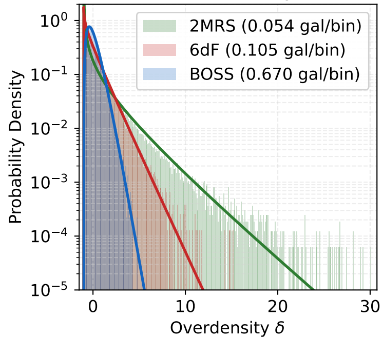
Initial Overdensity PDF
