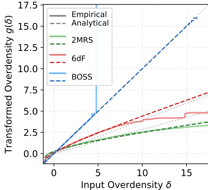
Transformation Function
