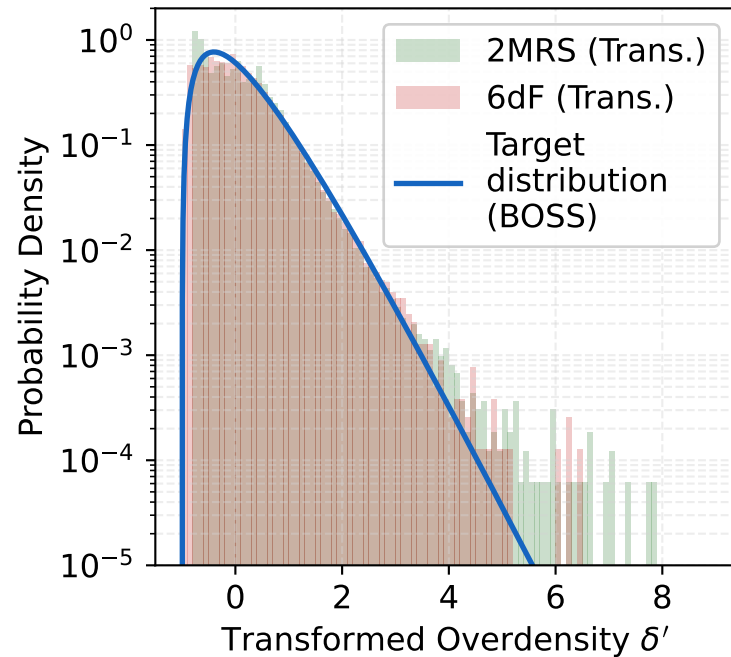
Transformed Distribution
