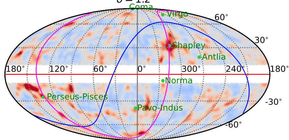
0.04 < z < 0.07 [0.03] 170 \text{ Mpc} < d < 295 \text{ Mpc} [125 Mpc] \sigma = 1.2^\circ
