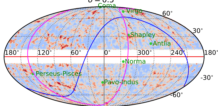
0.14 < z < 0.18 [0.04] 580 \text{ Mpc} < d < 739 \text{ Mpc} [158 Mpc] \sigma = 0.5^\circ
