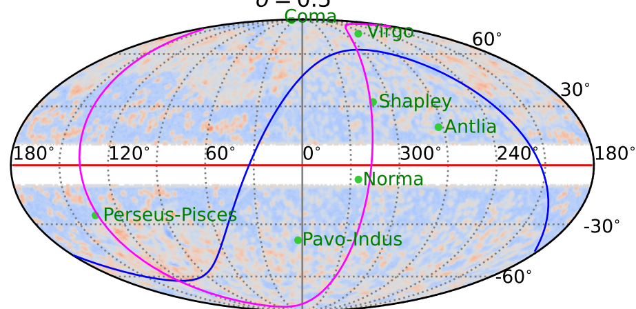
0.18 < z < 0.40 [0.22] 739 \text{ Mpc} < d < 1552 \text{ Mpc} [813 Mpc] \sigma = 0.5^\circ
