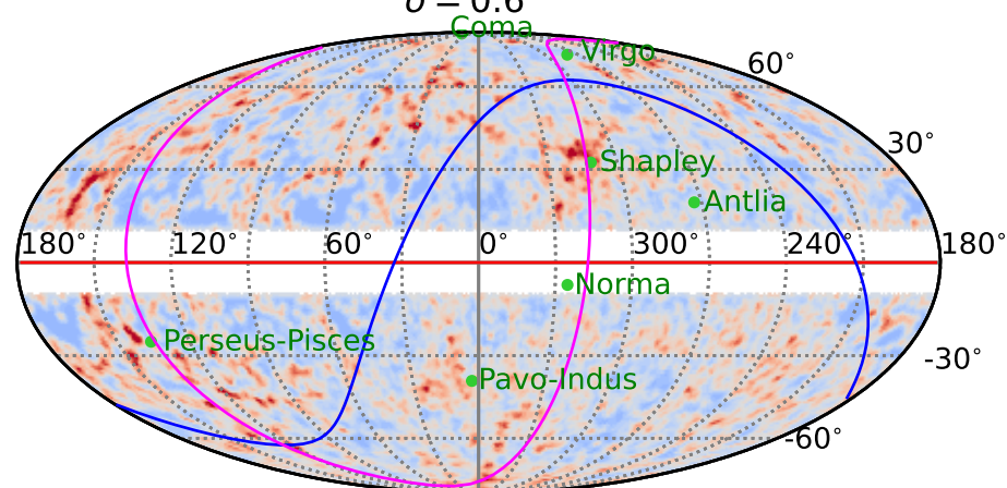
0.10 < z < 0.14 [0.04] 418 \text{ Mpc} < d < 580 \text{ Mpc} [162 Mpc] \sigma = 0.6^\circ
