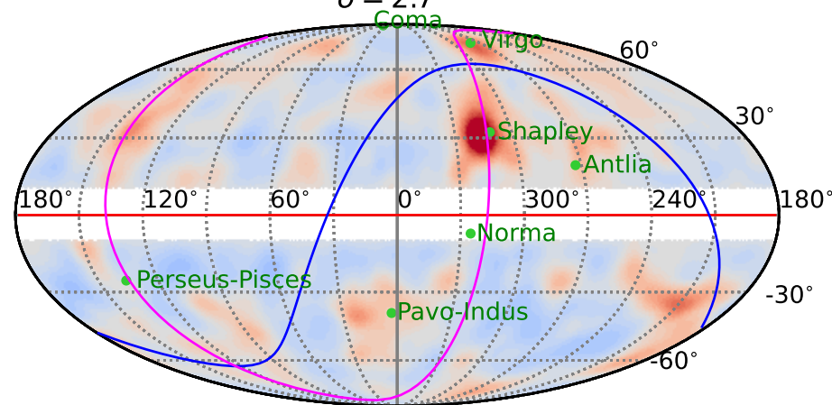
0.01 < z < 0.04 [0.03] 43 \text{ Mpc} < d < 170 \text{ Mpc} [127 Mpc] \sigma = 2.7^\circ
