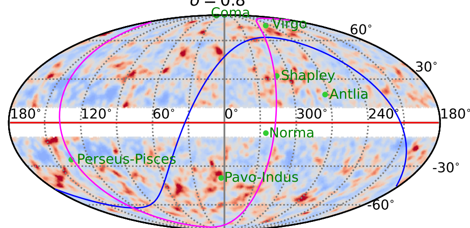
0.07 < z < 0.10 [0.03] 295 \text{ Mpc} < d < 418 \text{ Mpc} [123 Mpc] \sigma = 0.8^\circ
