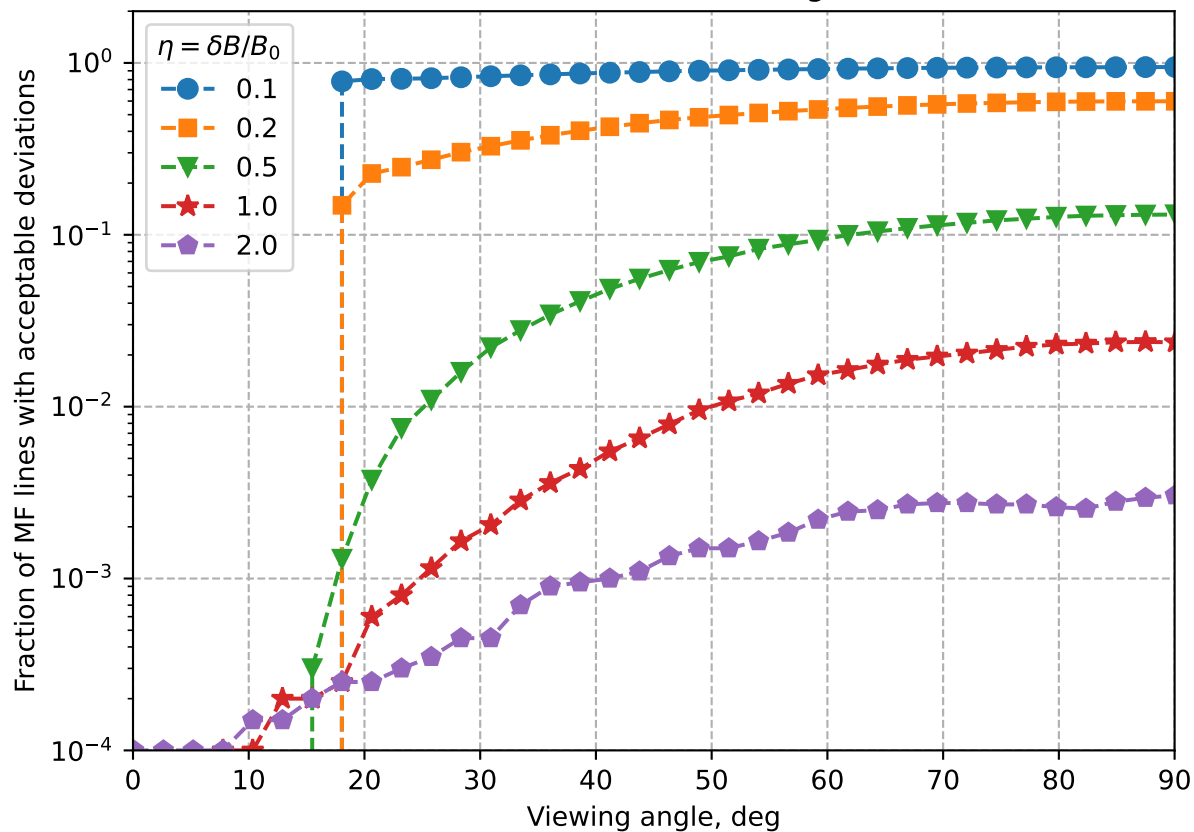
Fraction of lines within the Peanut rectangle [GS95 turbulence]
