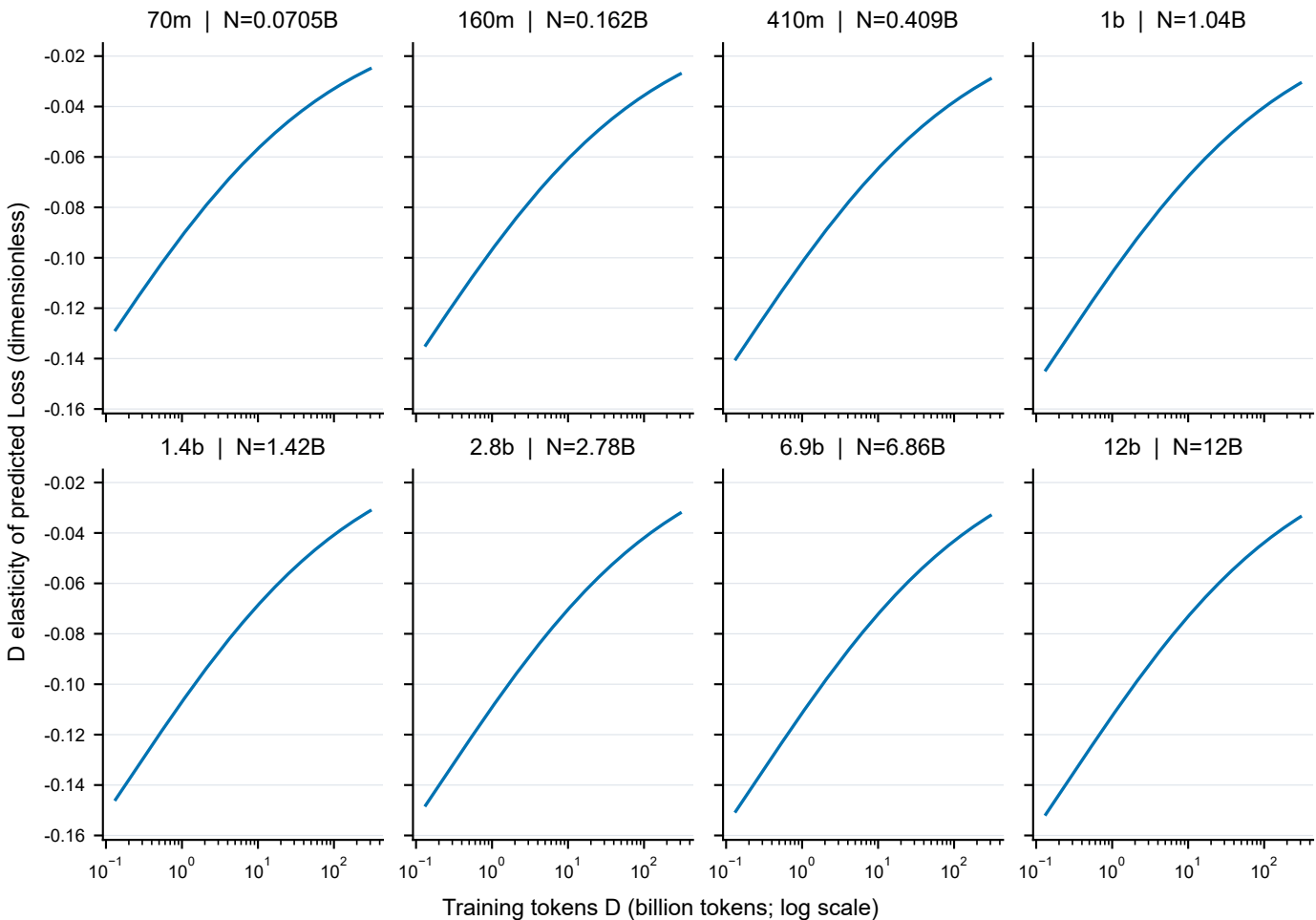
M0 elasticity with respect to D by model size Shading: pointwise 95% CI (1,000 bootstrap fits; 8 tracks)
