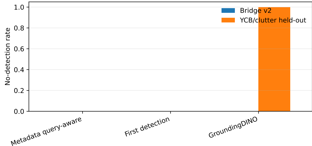
No-detection failure exposed by YCB/clutter held-out
