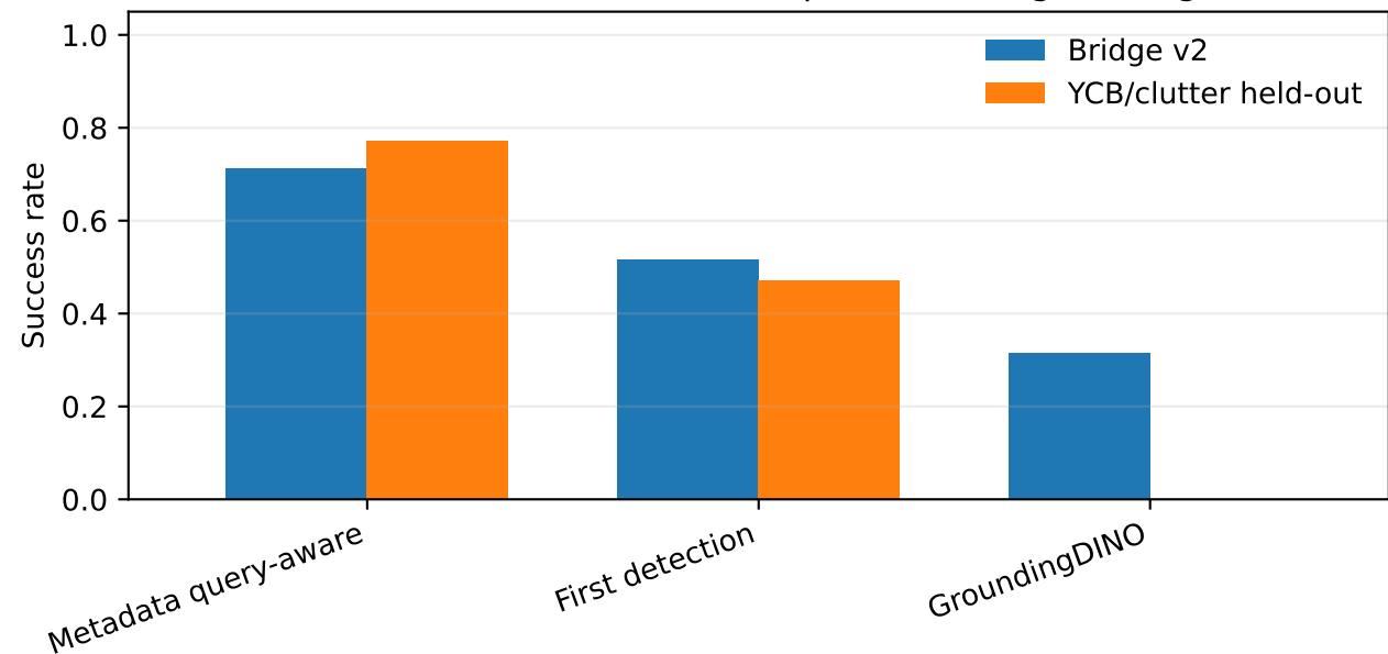
Detector transfer under crop-median target lifting
