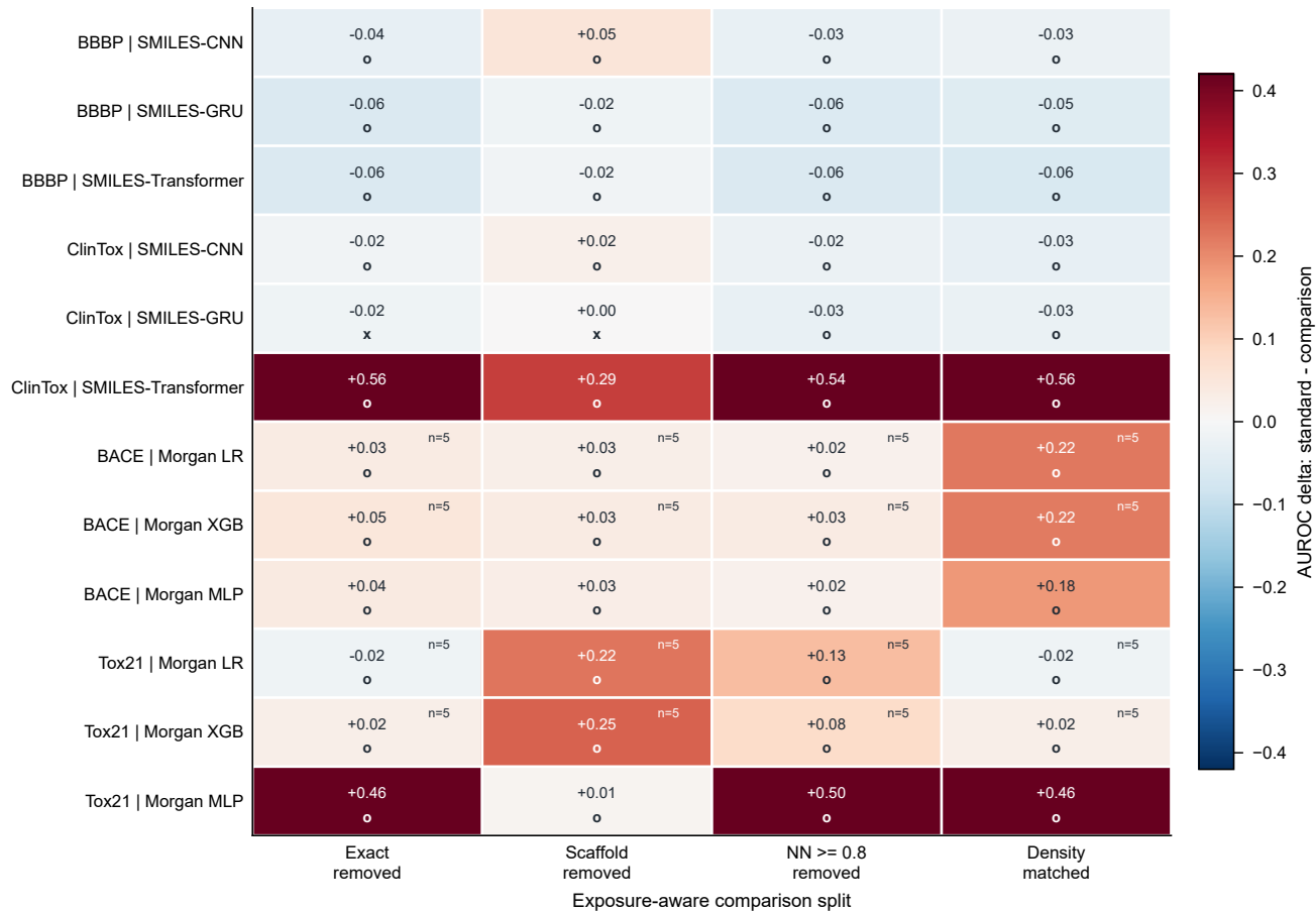
Fig. 4 | Exposure-adjusted AUROC deltas across benchmark tasks
