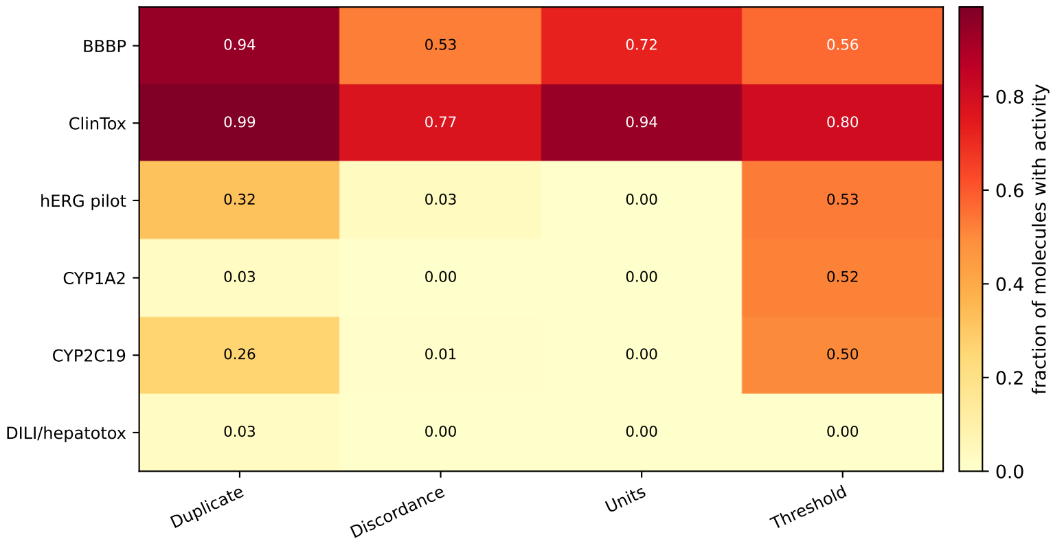
Assay-provenance heterogeneity rates
