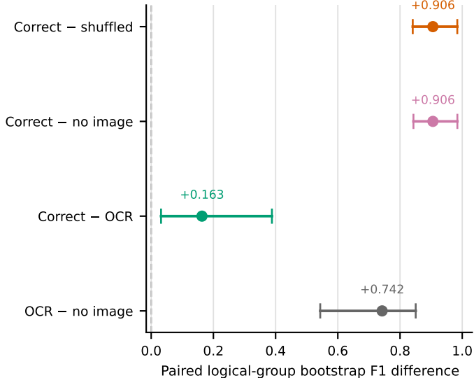
B Correct-image and OCR evidence contrasts
