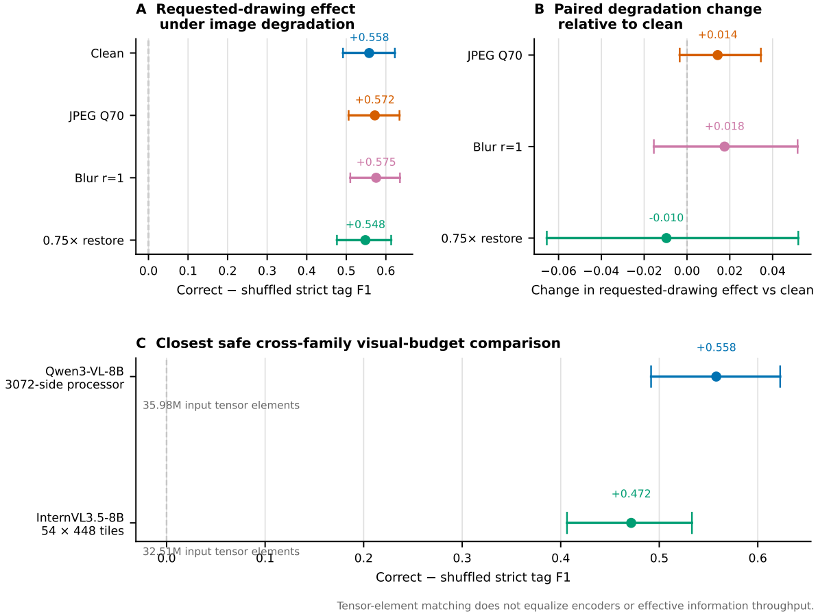
Figure 2: Qualified-budget robustness and cross-model visual-budget recovery. Panel A reports correct-minus-shuffled strict tag F1 under clean and three mild quality shifts. Panel B reports paired change relative to clean. Panel C shows InternVL requested-drawing effects at the closest-safe 54-tile setting. Whiskers are paired 95% source-bootstrap intervals; recorded tensor-element matching does not equalize encoders.
