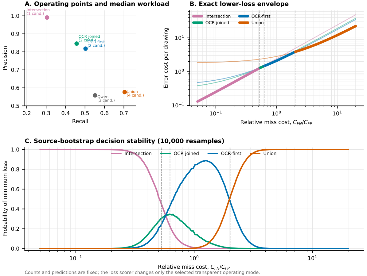
Figure 4: Cost-aware operation from fixed OCR–VLM outputs. Panel A shows precision–recall points with median candidate workload. Panel B highlights the exact lower-loss envelope for L = rFN + FP . Panel C gives each mode’s probability of minimum loss over 10,000 source-cluster resamples. Dashed lines mark point-estimate switches; scoring changes no prediction.
