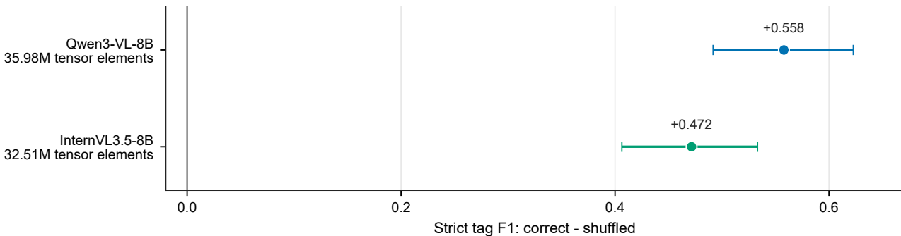
c Closest safe visual-budget comparison
