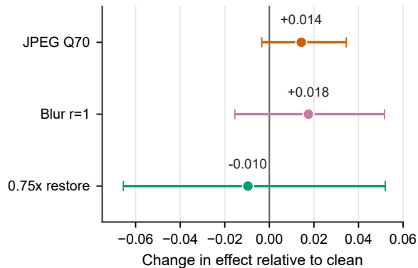
b Paired degradation change
