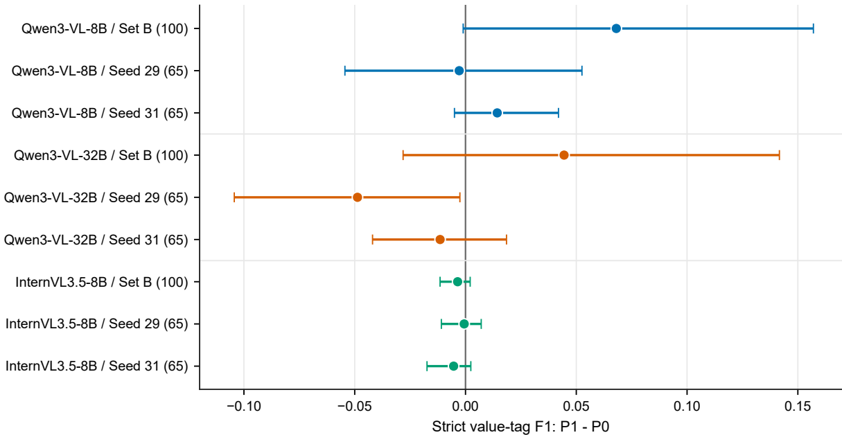
a Frozen-prompt sensitivity
