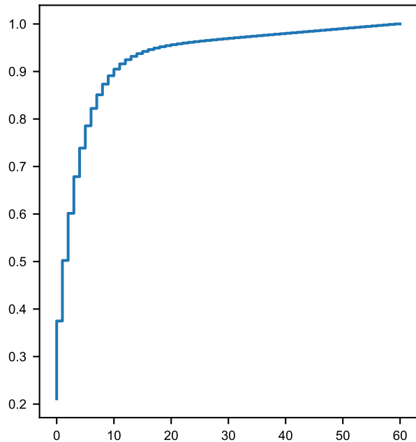
CDF
