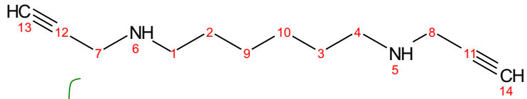
Predicted 1H NMR Spectrum
