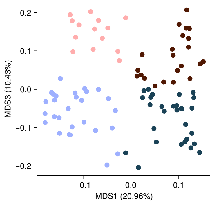
Functional Profiles (Genes/UniRef90s)
