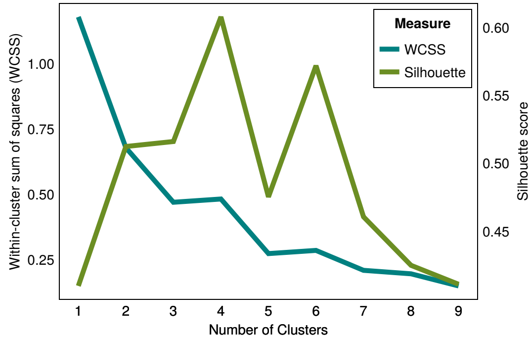
Clustering decision measures
