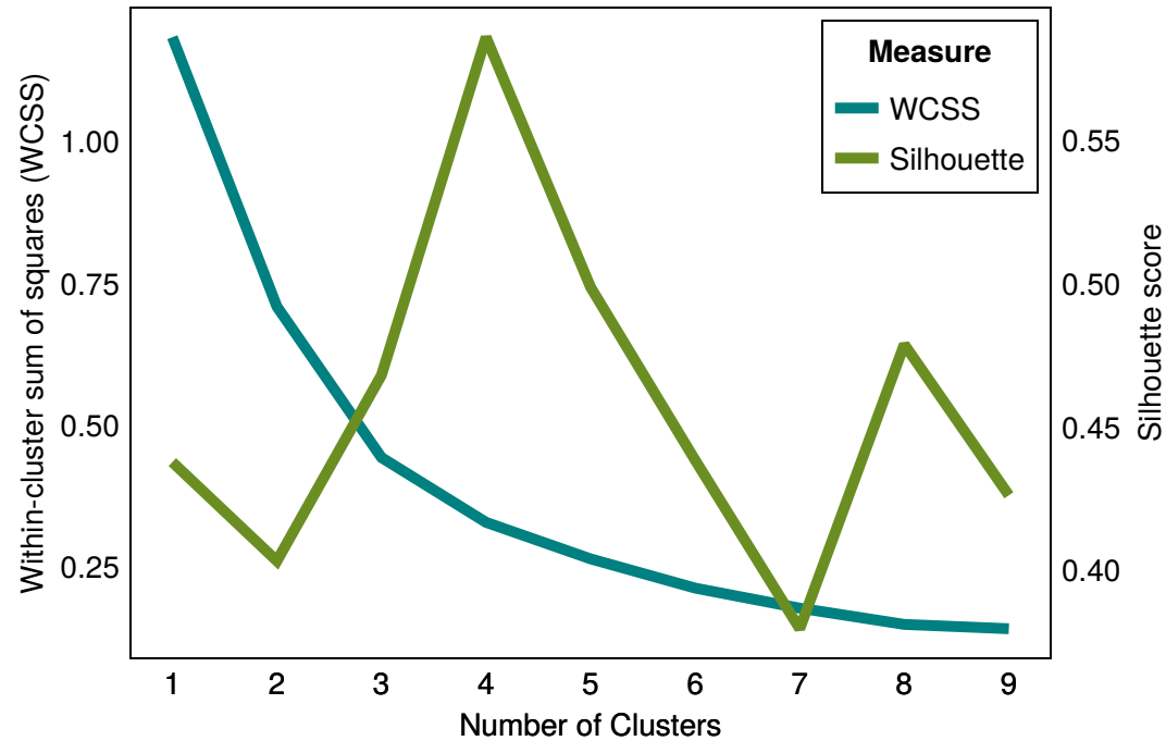
a Clustering decision measures
