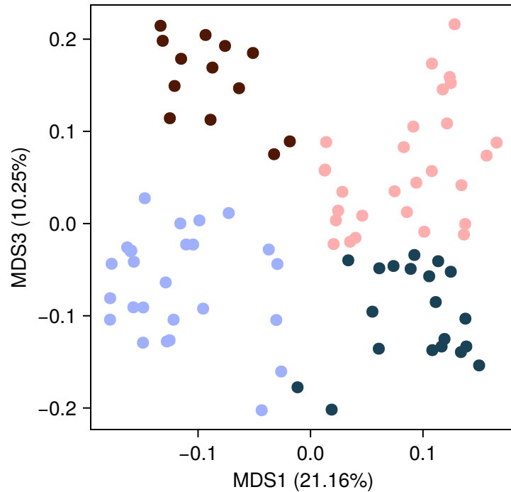
b Functional Profiles (Genes/UniRef90s)
