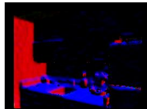
Normal (GT)
