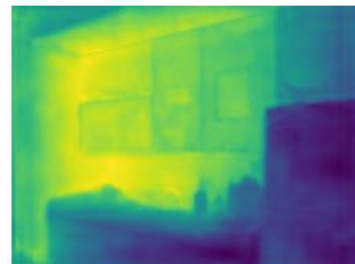
Depth
