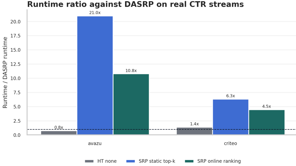
Figure 11: Avazu and Criteo datasets: Runtime ratio of selected real-stream baselines against DASRP. Values above 1 mean the baseline was slower than DASRP.
