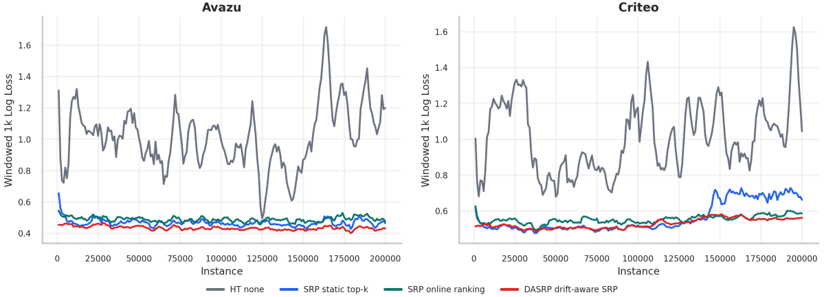
Figure 10: Left: Avazu dataset. Right: Criteo dataset. Windowed 1,000-instance Log Loss over time on real CTR streams:
