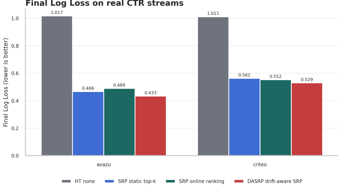
Figure 9: Final Log Loss comparison on Avazu and Criteo.
