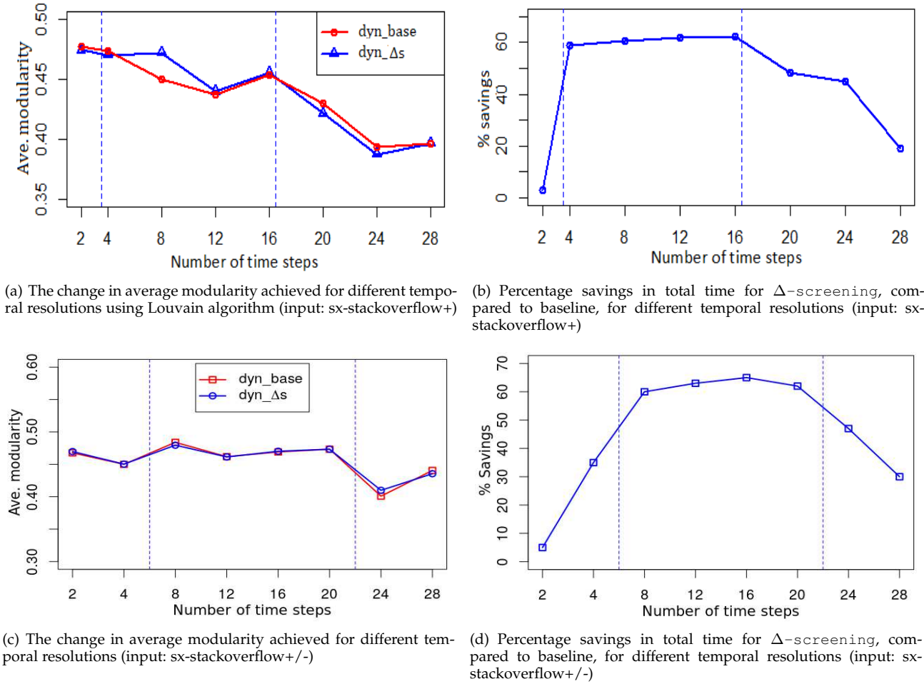
Fig. 9. Plots showing the effect of varying the temporal resolution— as measured by the number of temporal bins (i.e., time steps) used to partition the input graph stream. The resolution of partitioning changes from coarser to finer, from left to right on the x-axis.
