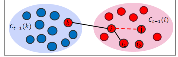
Fig. 2. Figure showing the impact of a deleted edge (i, j) , shown in red dotted line. Representative cases of candidate vertices for potential inclusion in \mathcal{R}_t are shown highlighted as labelled vertices. Note that we follow the naming convention of denoting the community containing a vertex i by C(i) . Also, note that not all edges are shown.
