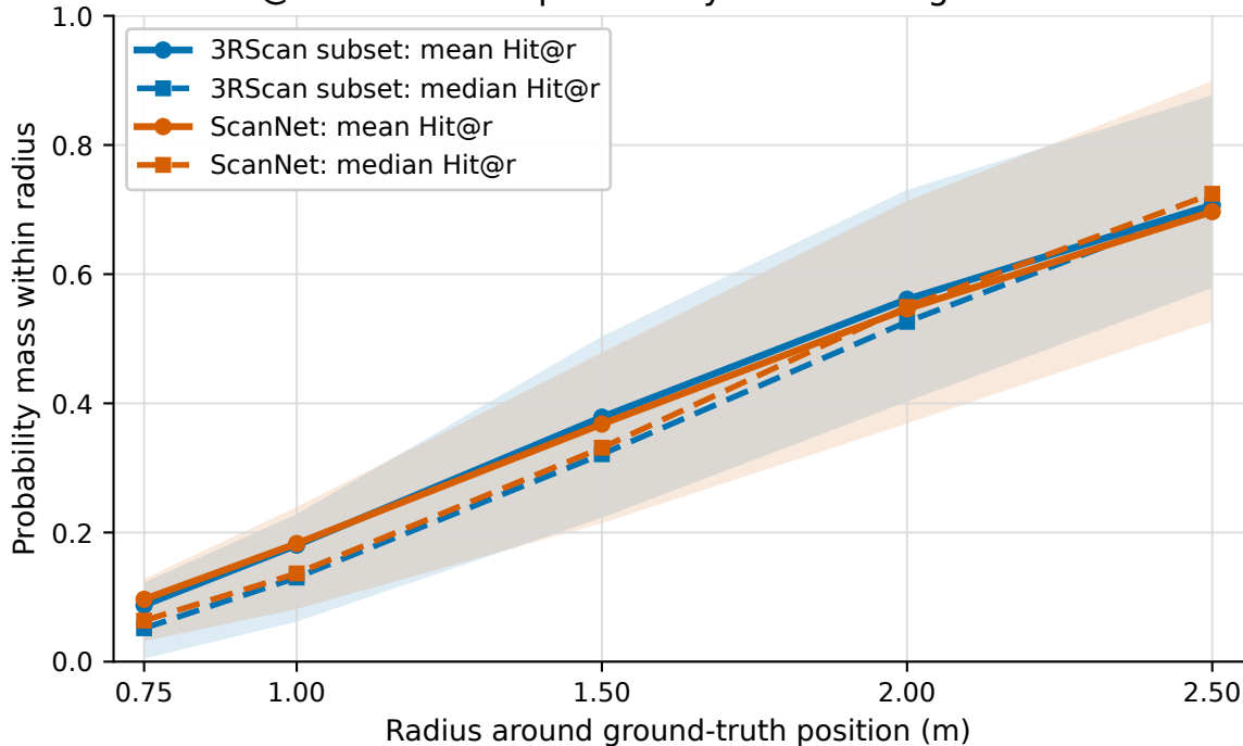
Hit@r: localization probability mass near ground truth
