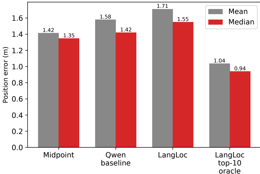
Mean vs median (skew = mean – median)
