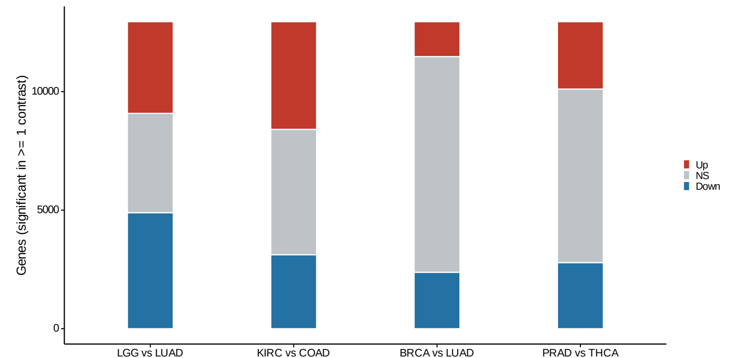
E Direction of change across contrasts
