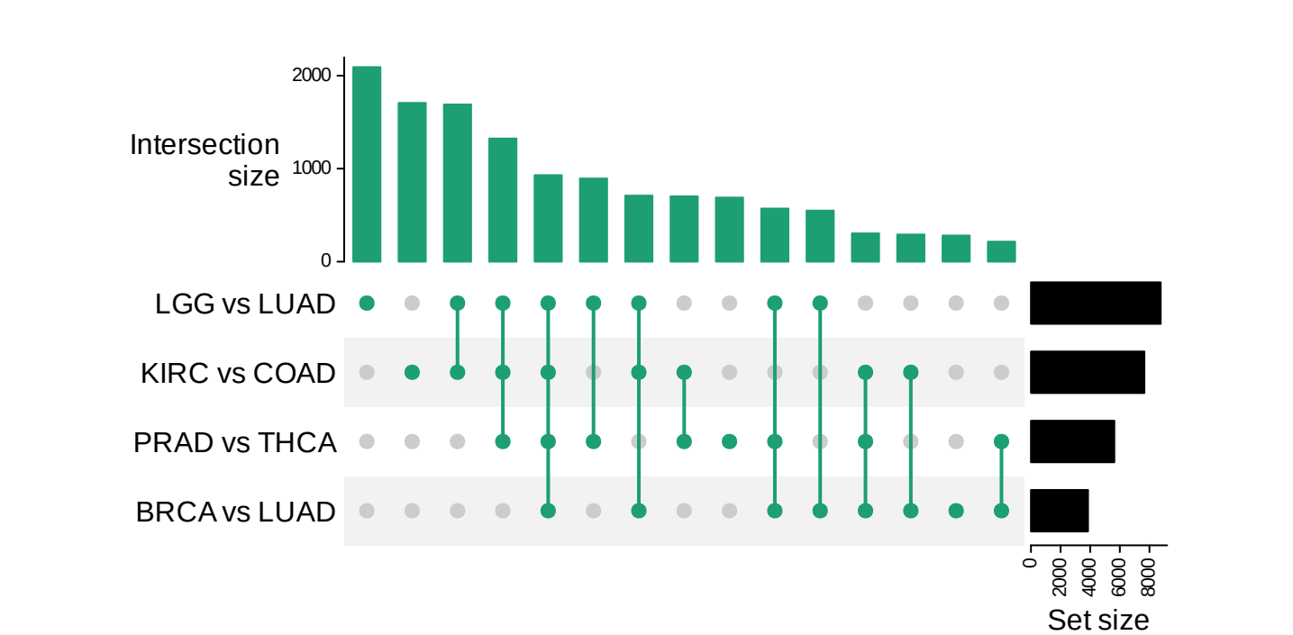
B Significant-gene overlap (UpSet)
