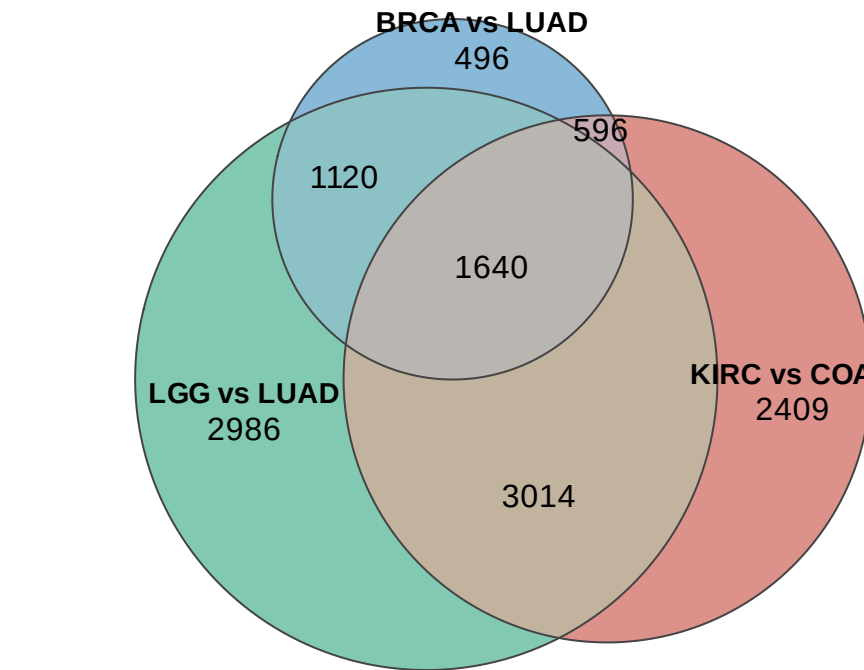
C Significant-gene overlap (Venn)
