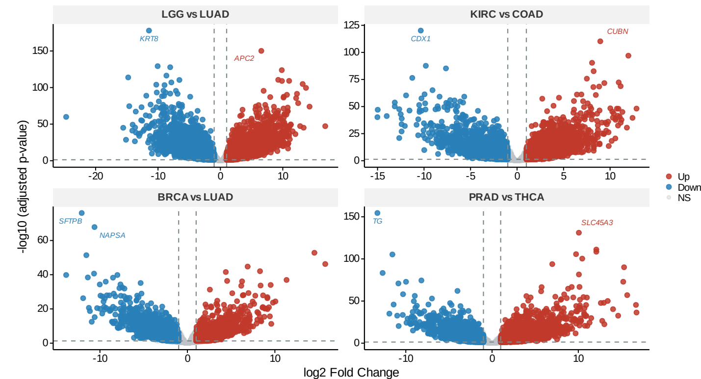
A Pairwise differential expression (TCGA)
