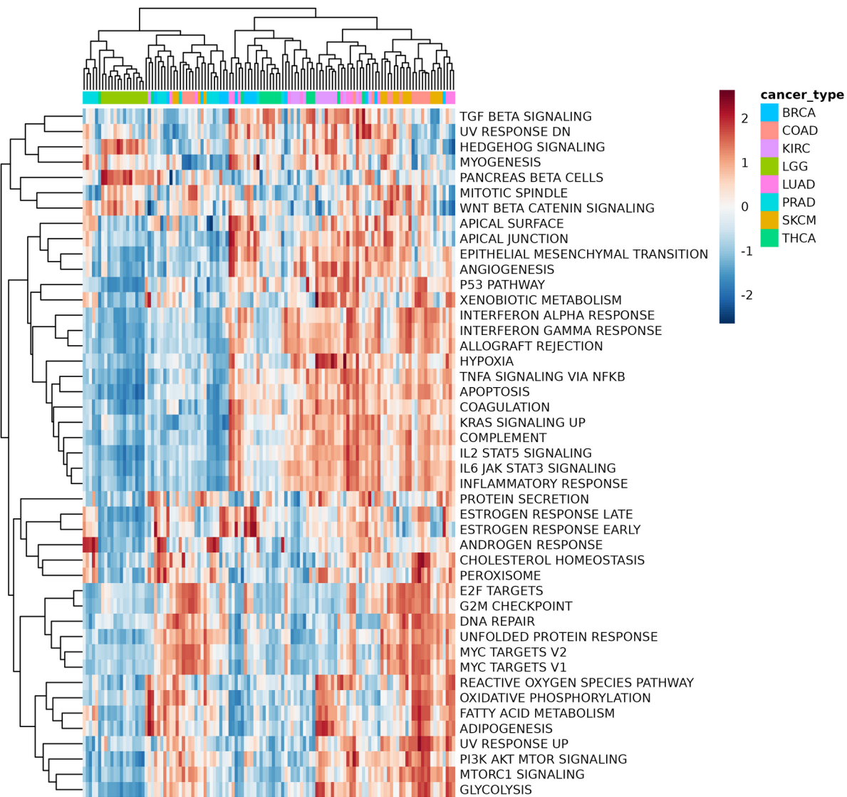
a Per-sample GSVA signatures (Hallmark)
