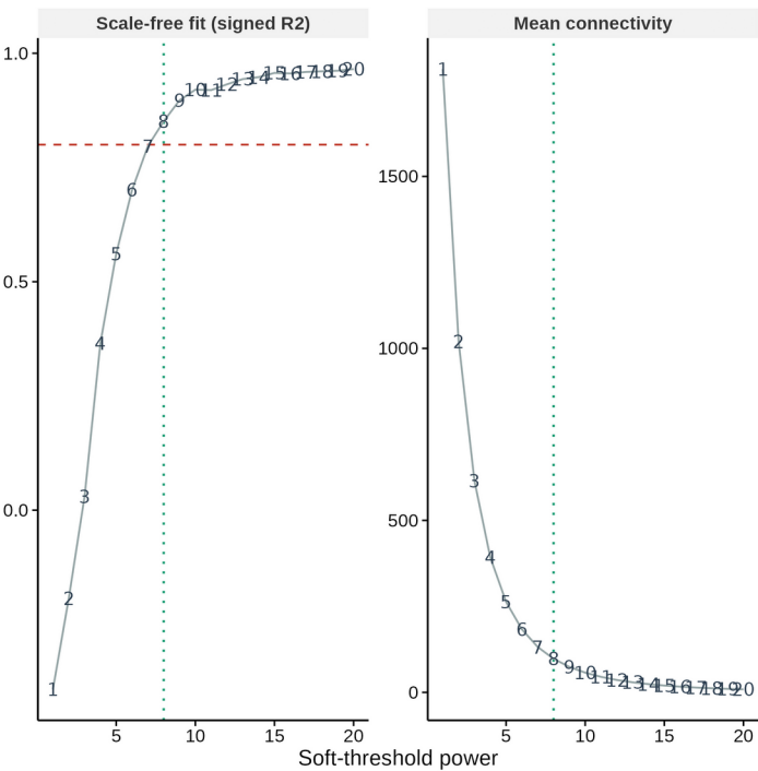
c Soft-threshold selection
