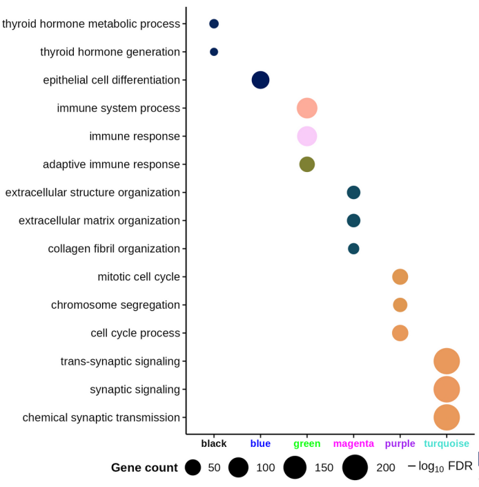
e Module enrichment (GO BP)
