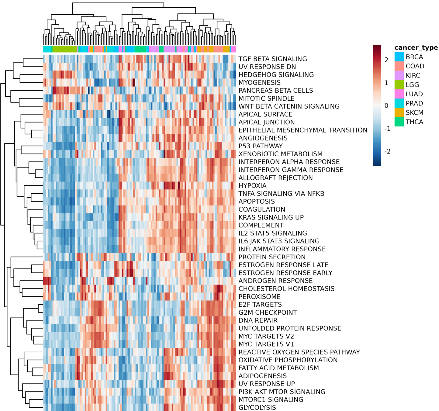
a Per-sample GSVA signatures (Hallmark)
