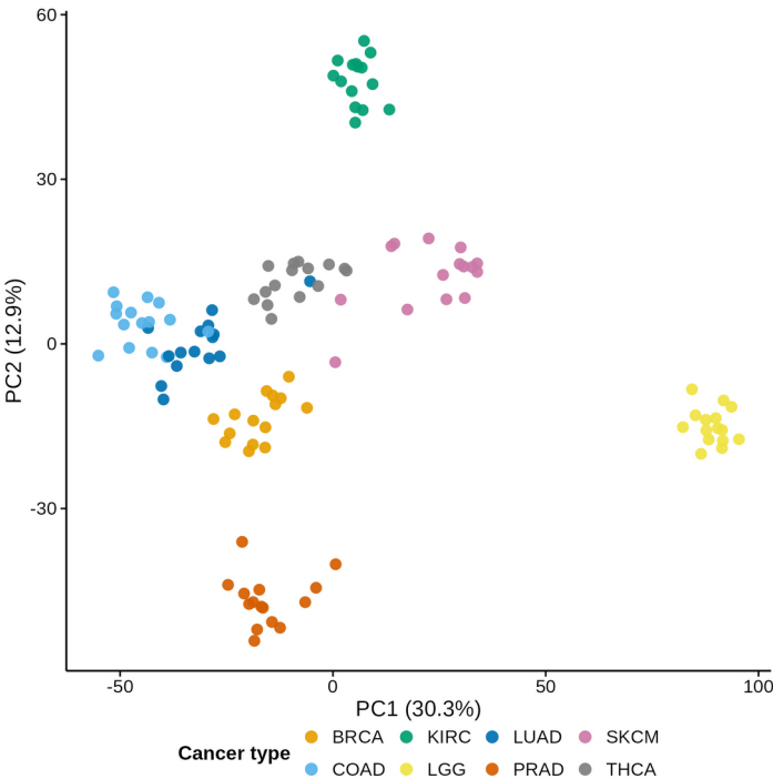
b Principal-component analysis
