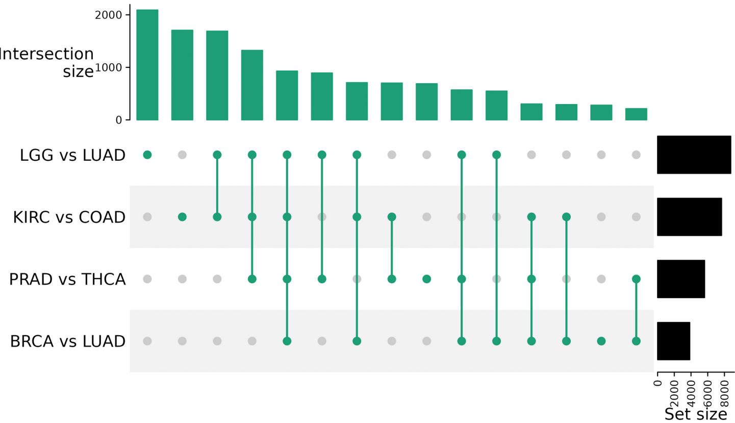
b Significant-gene overlap (UpSet)
