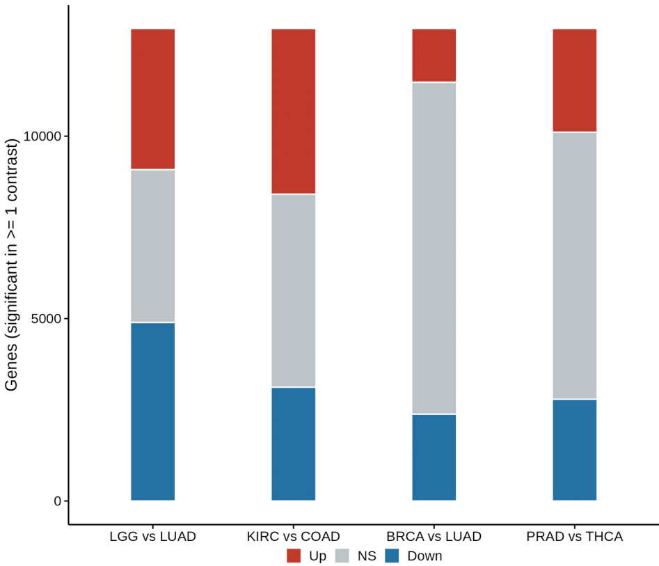
e Direction of change across contrasts
