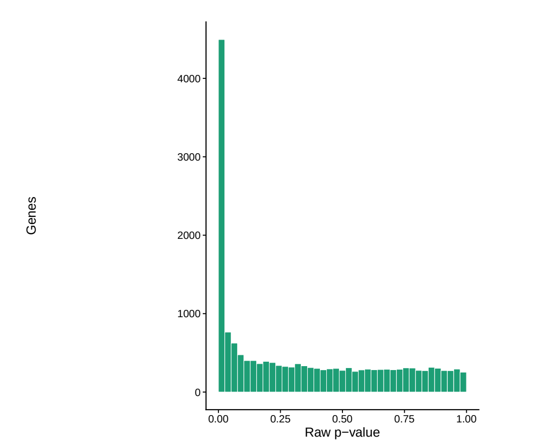
C P-value distribution (airway)
