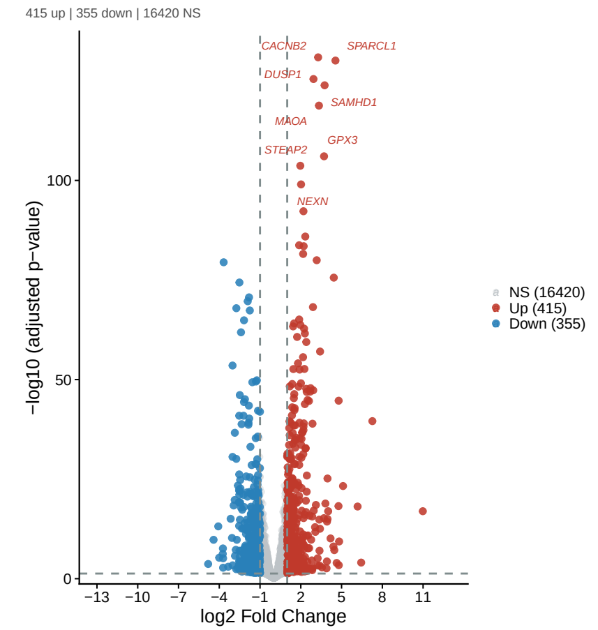
A Differential expression: dexamethasone vs control (airway)
