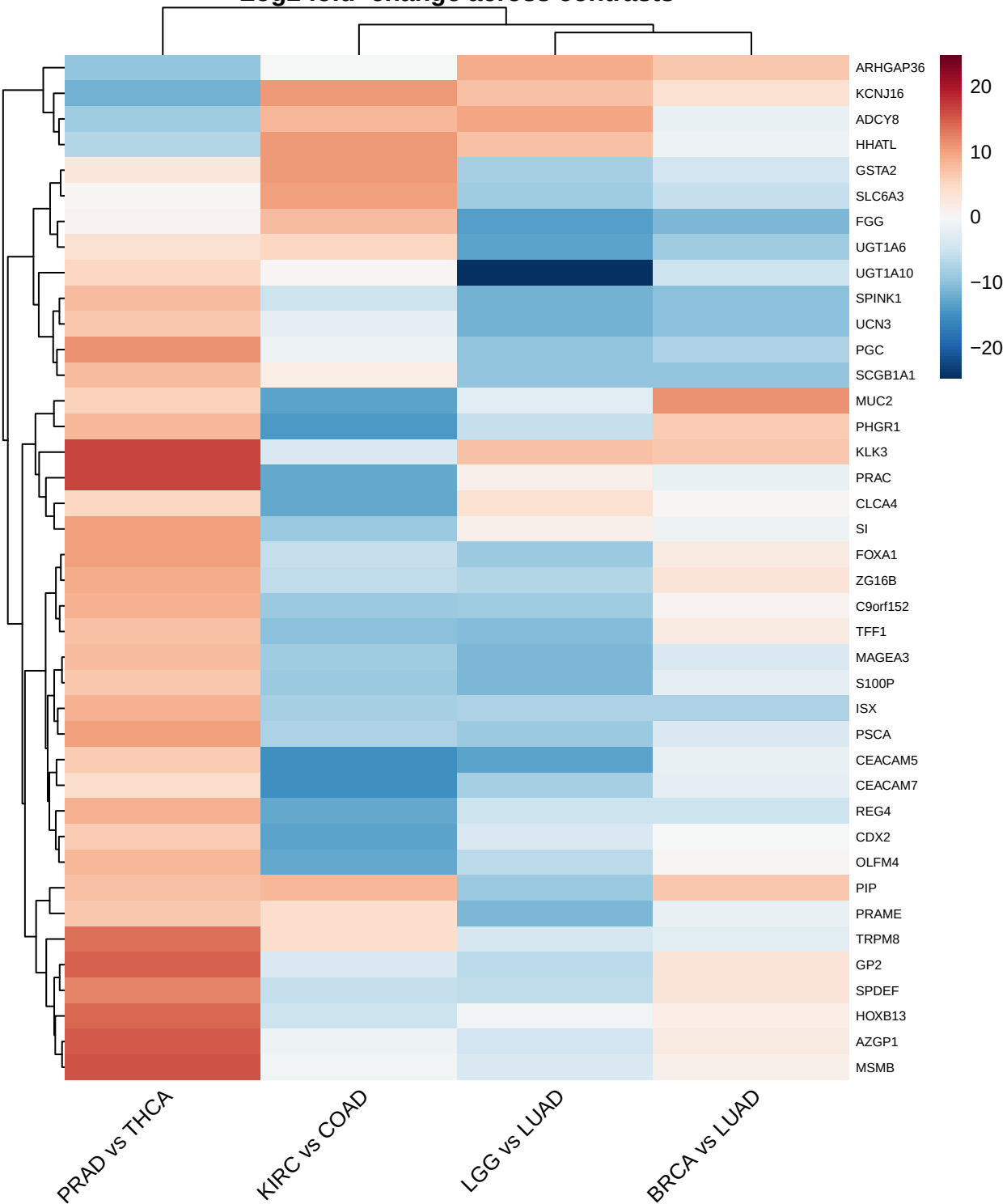
Log2 fold-change across contrasts
