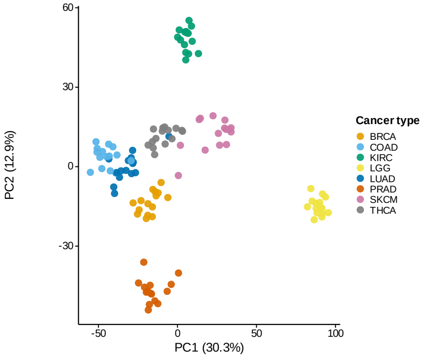
Principal-component analysis
