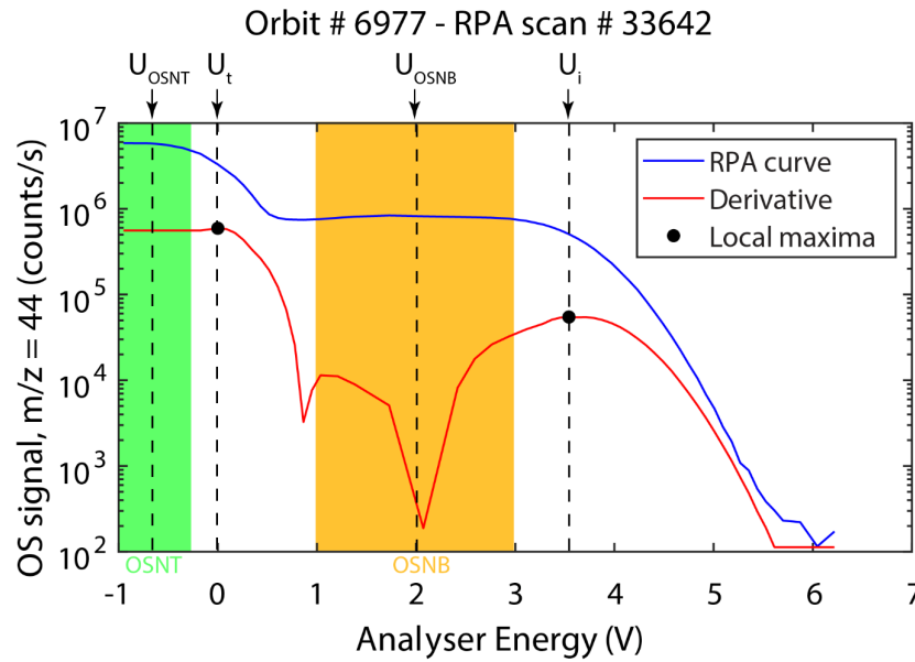
Figure 9: Example of RPA curve (blue) collected during orbit #6977 of wind campaign #23. Its derivative is in red.
