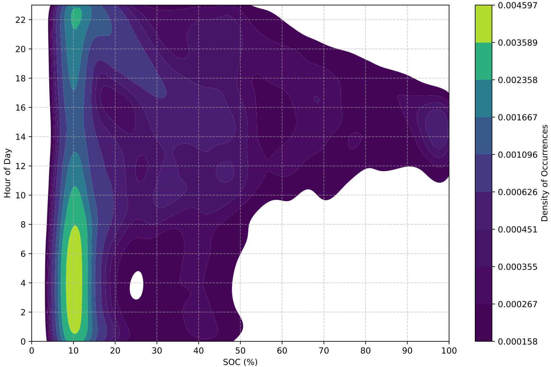
SOC Density Plot - 50kWh (Capacity: 50.0 kWh)
