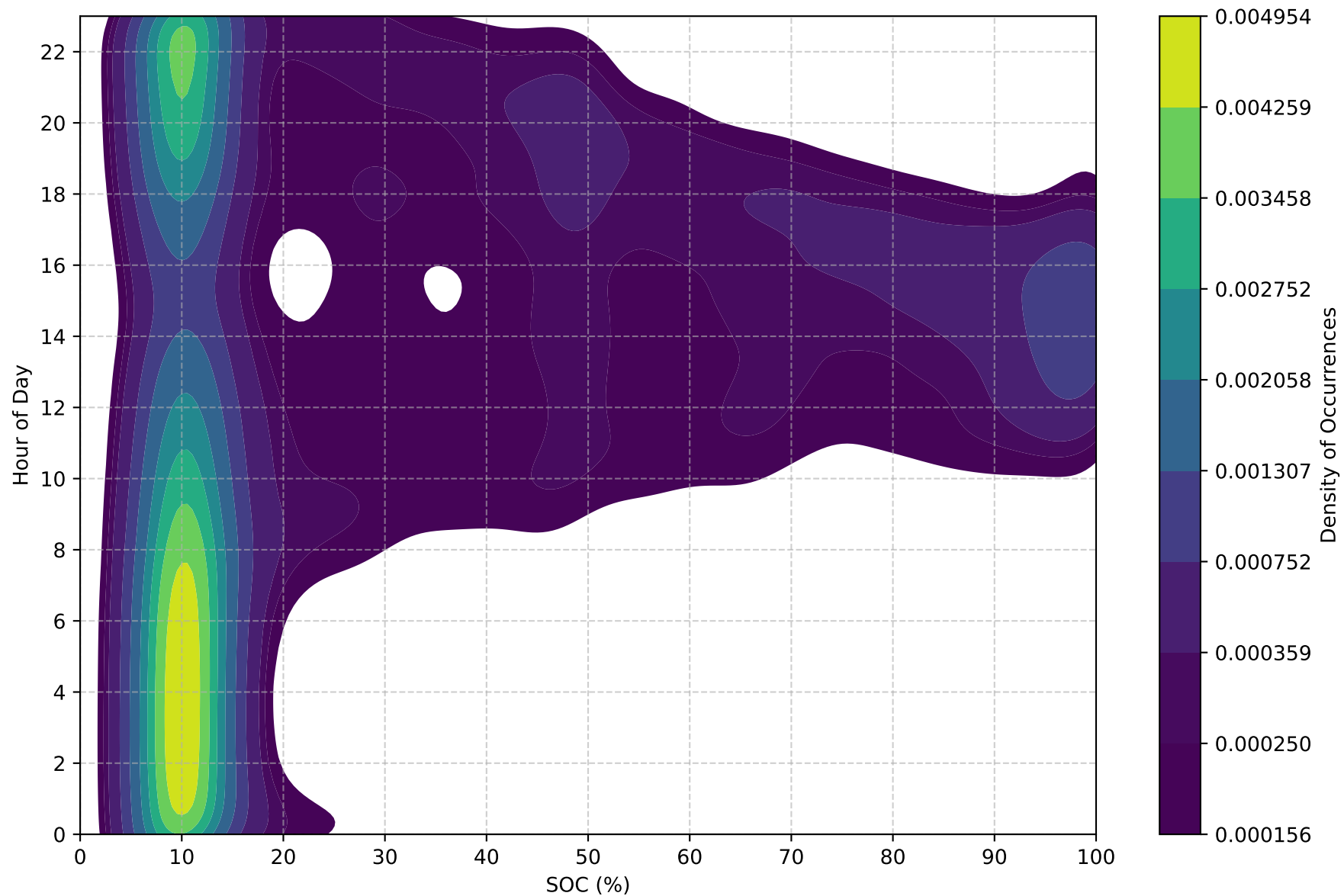
SOC Density Plot - 12kWh (Capacity: 12.0 kWh)
