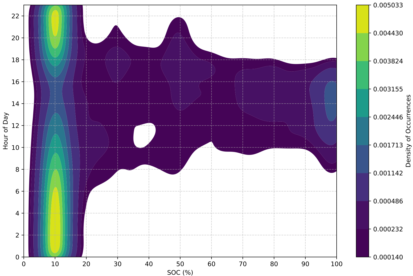
SOC Density Plot - 5kWh (Capacity: 5.0 kWh)
