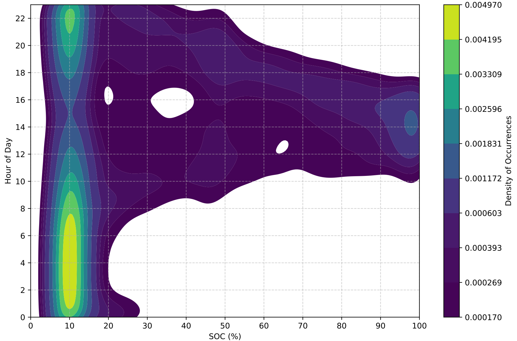
SOC Density Plot - 15kWh (Capacity: 15.0 kWh)
