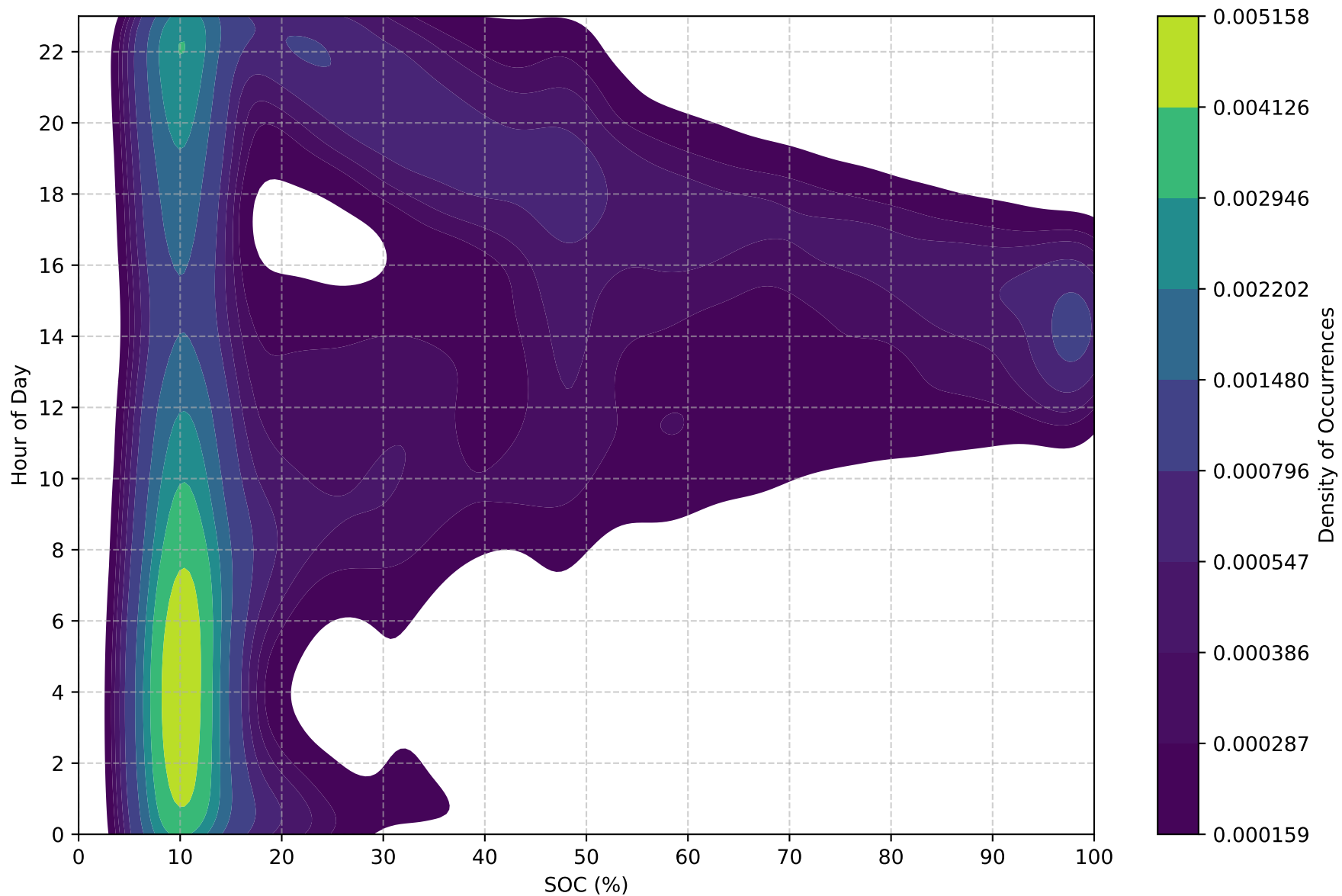
SOC Density Plot - 26kWh (Capacity: 26.0 kWh)
