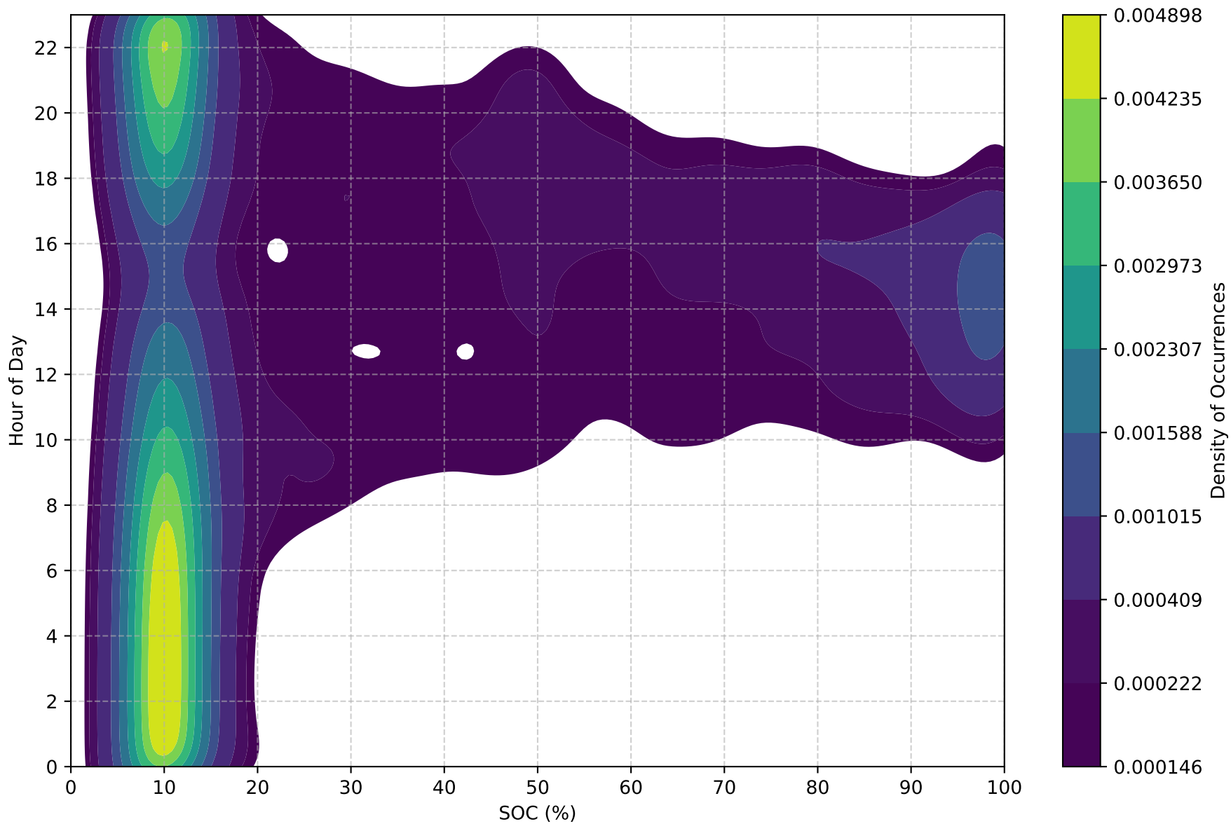
SOC Density Plot - 8kWh (Capacity: 8.0 kWh)
