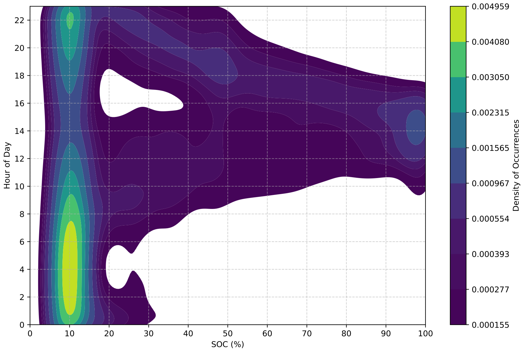
SOC Density Plot - 20kWh (Capacity: 20.0 kWh)
