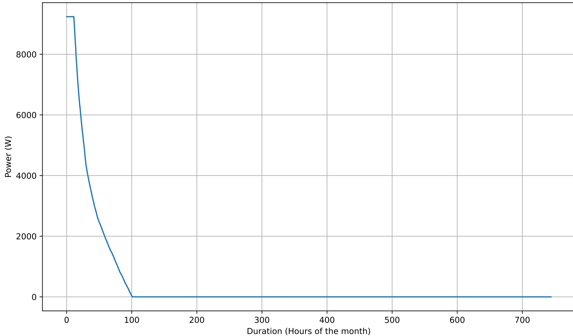
Battery Charging Power Duration Curve - 12kWh - Jul
