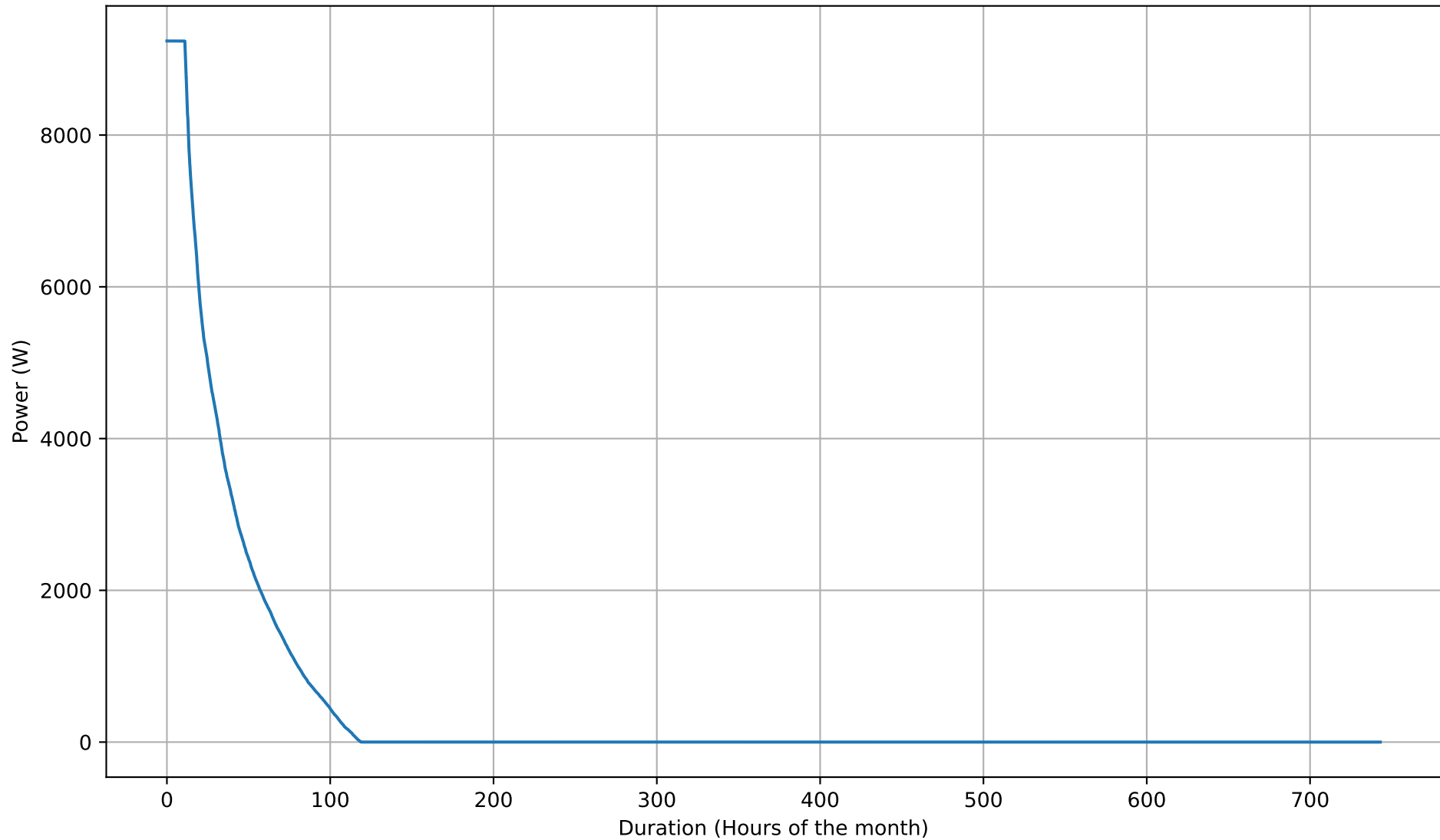
Battery Charging Power Duration Curve - 12kWh - Mar
