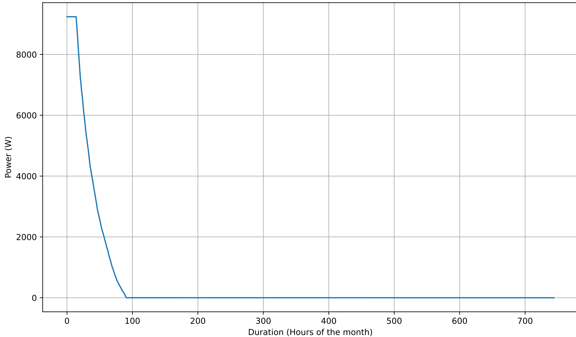
Battery Charging Power Duration Curve - 12kWh - Aug
