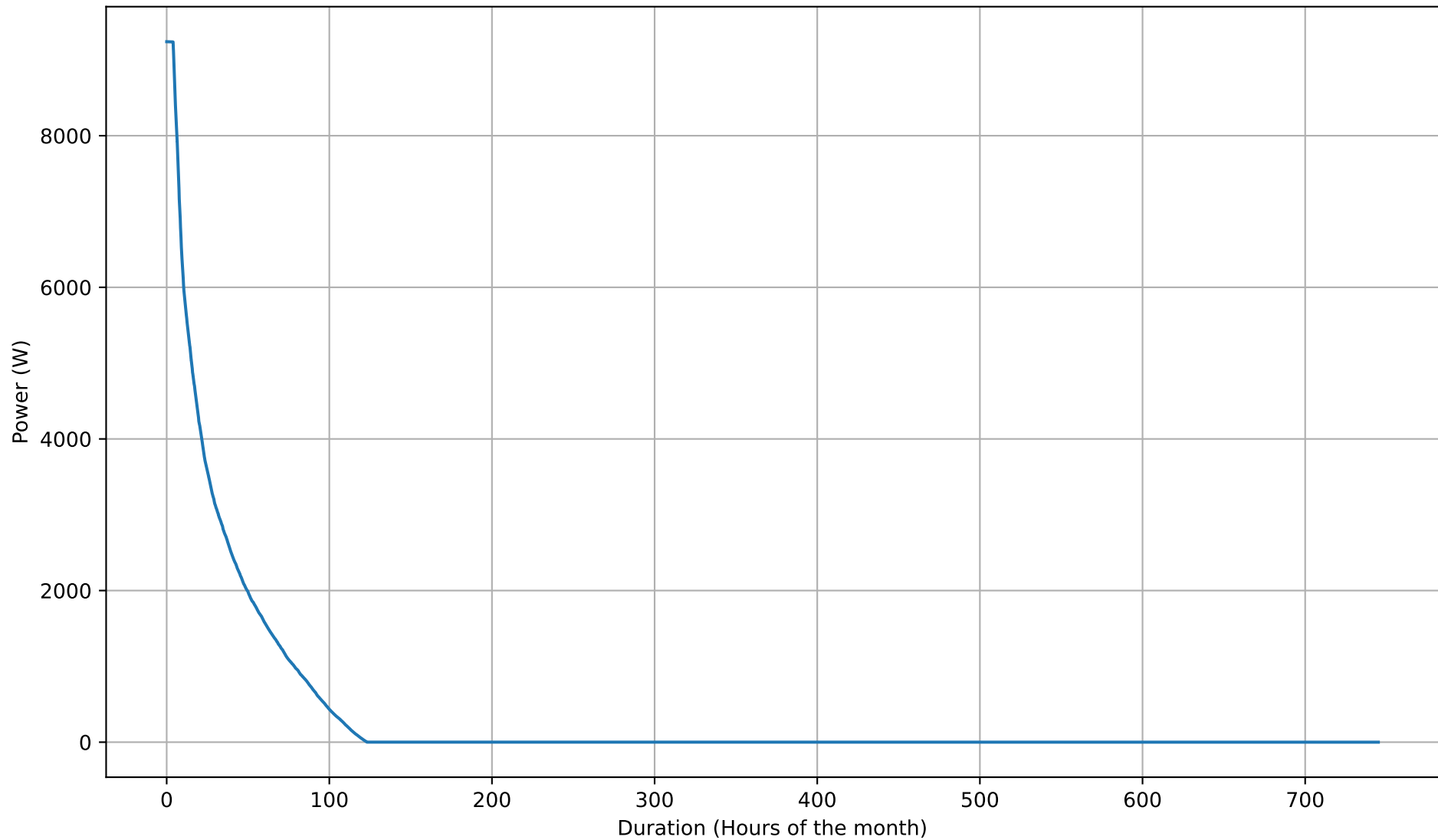
Battery Charging Power Duration Curve - 12kWh - Oct
