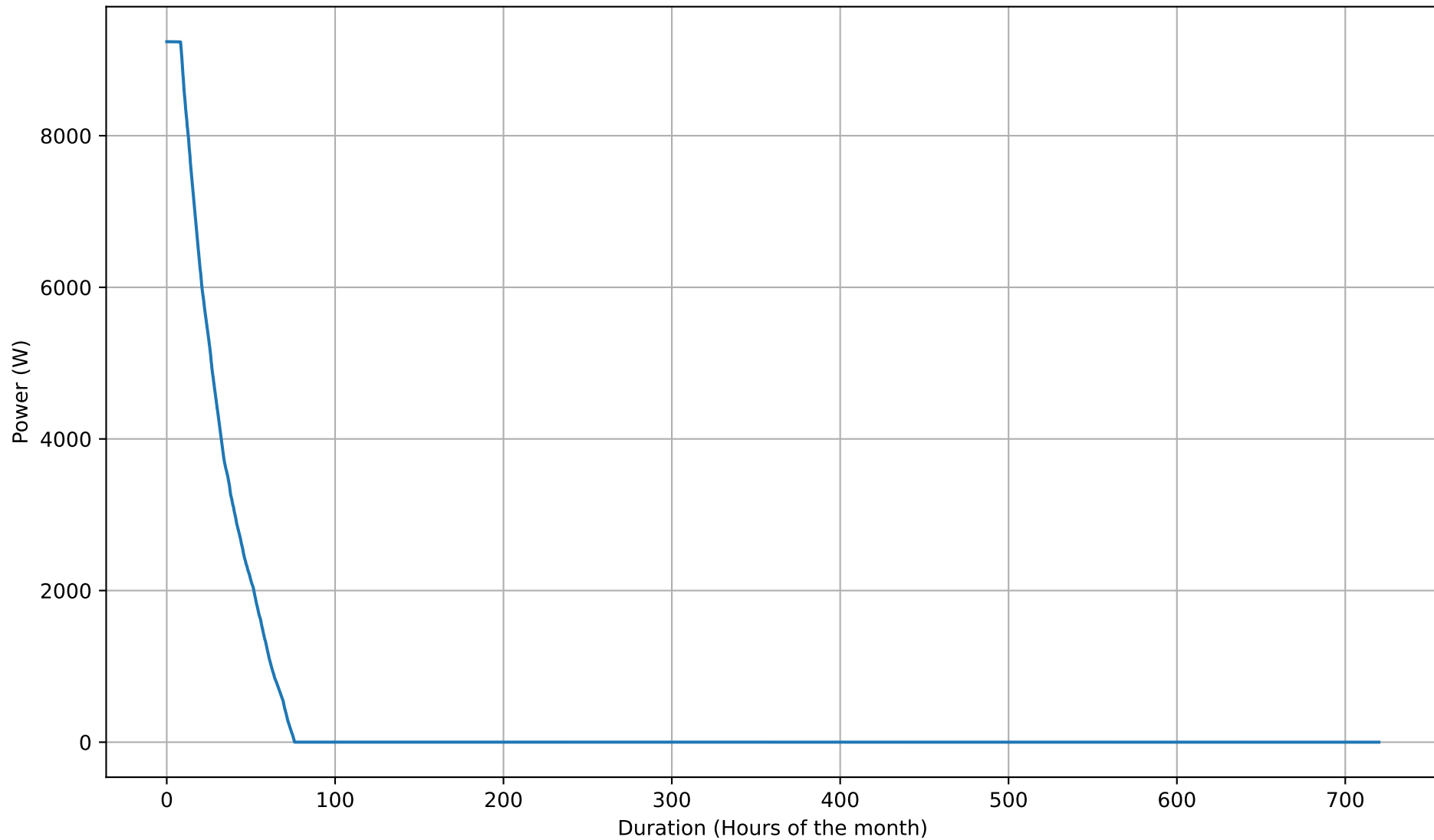
Battery Charging Power Duration Curve - 12kWh - Jun
