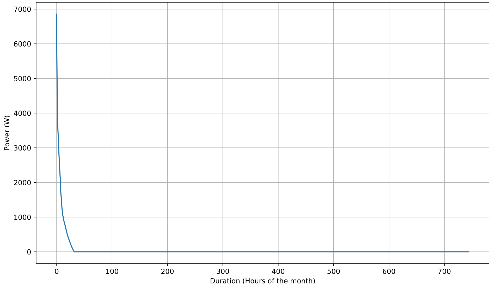
Battery Charging Power Duration Curve - 12kWh - Dec
