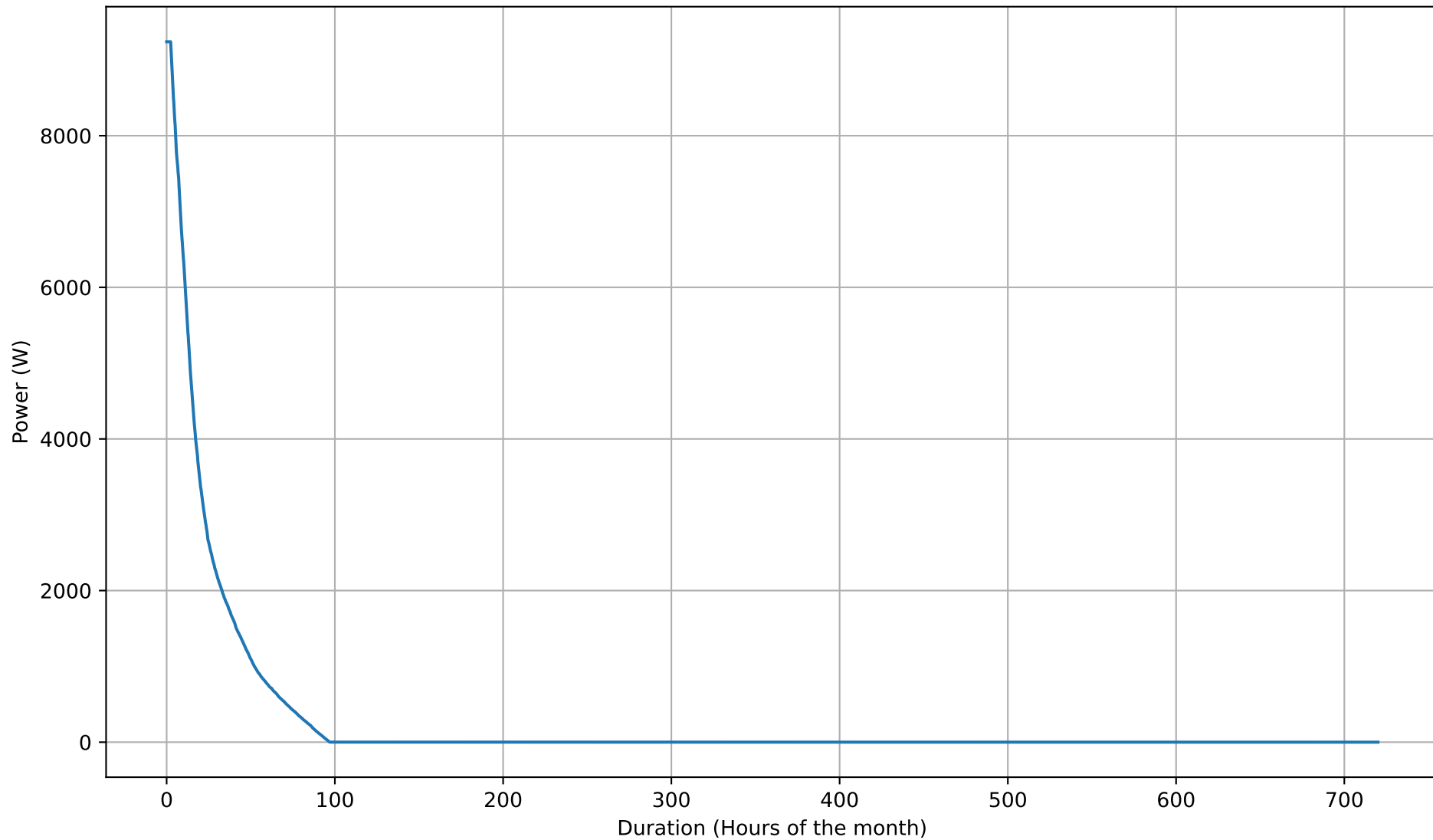
Battery Charging Power Duration Curve - 12kWh - Nov
