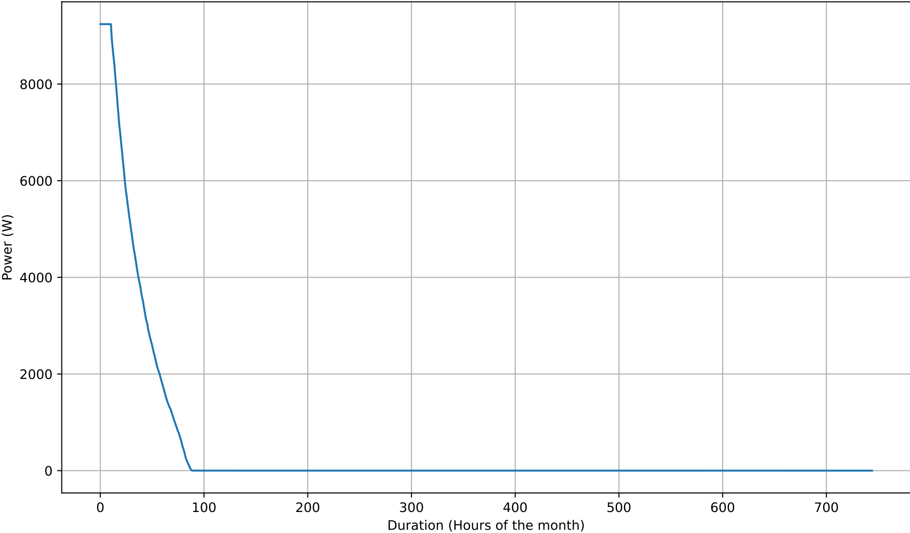
Battery Charging Power Duration Curve - 12kWh - May
