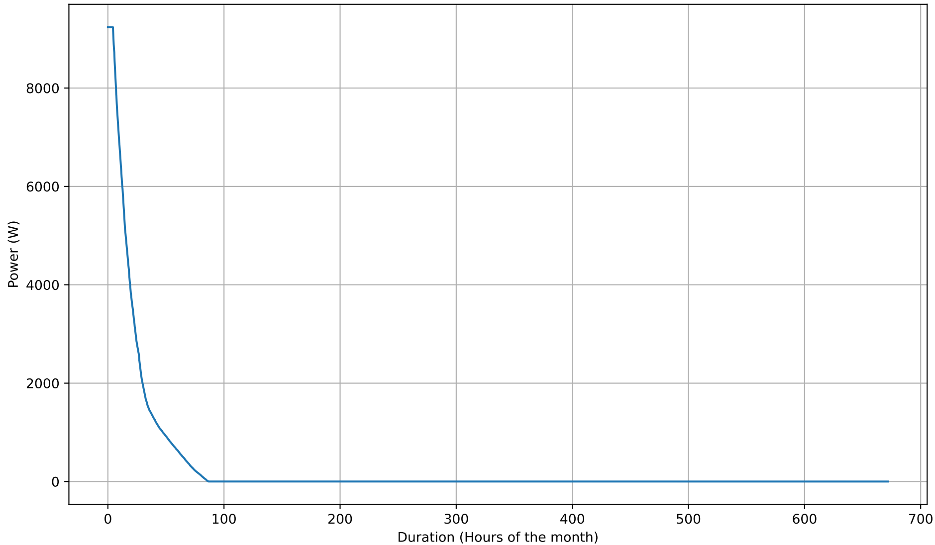
Battery Charging Power Duration Curve - 12kWh - Feb
