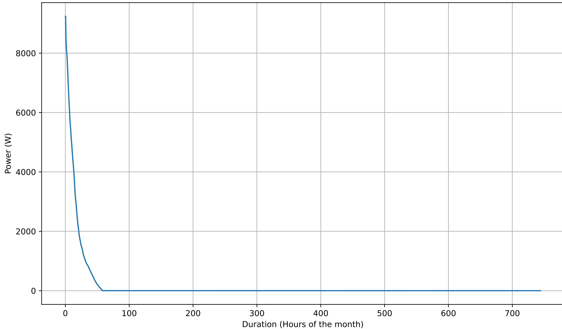
Battery Charging Power Duration Curve - 12kWh - Jan
