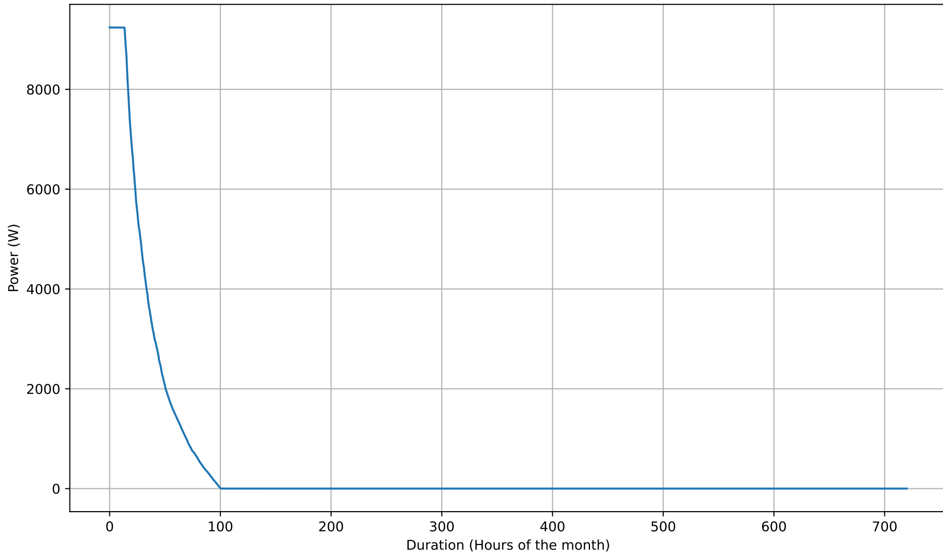
Battery Charging Power Duration Curve - 12kWh - Apr
