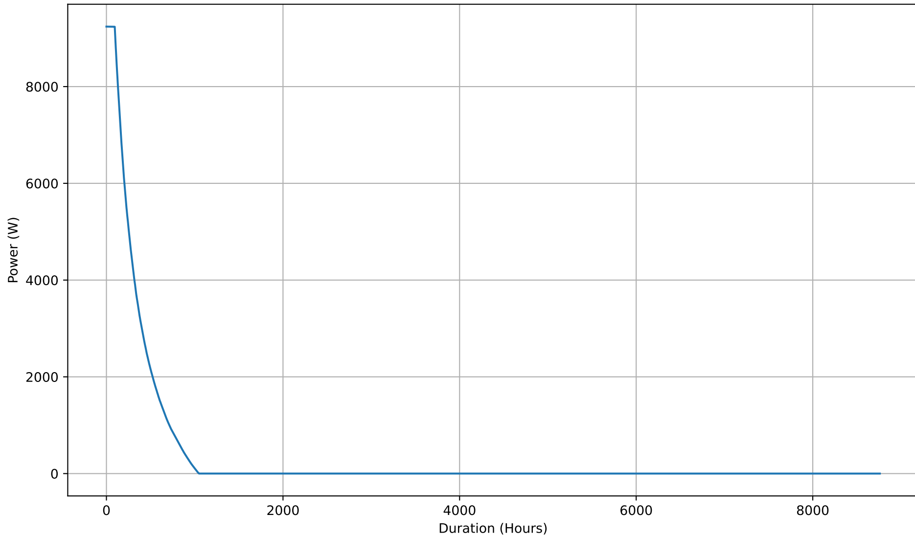
Yearly Battery Charging Power Duration Curve - 12kWh
