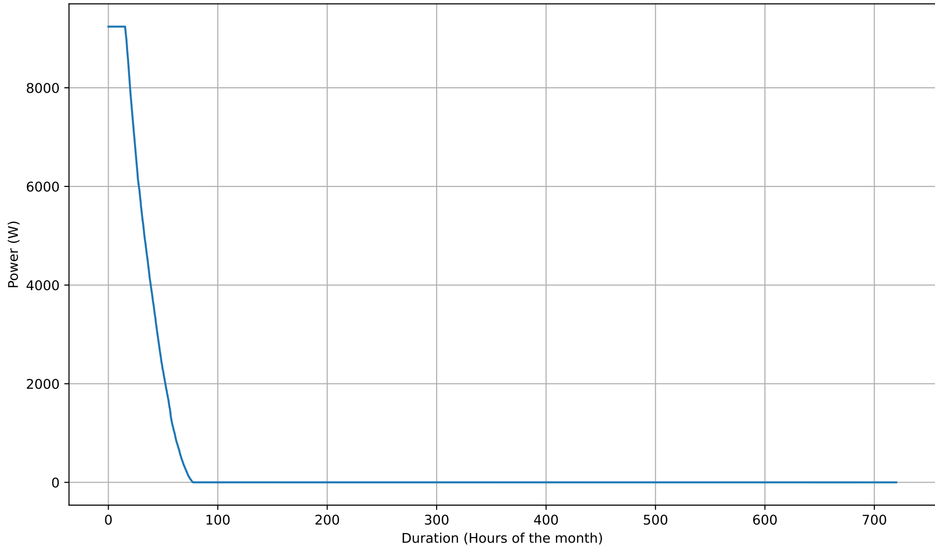
Battery Charging Power Duration Curve - 12kWh - Sep
