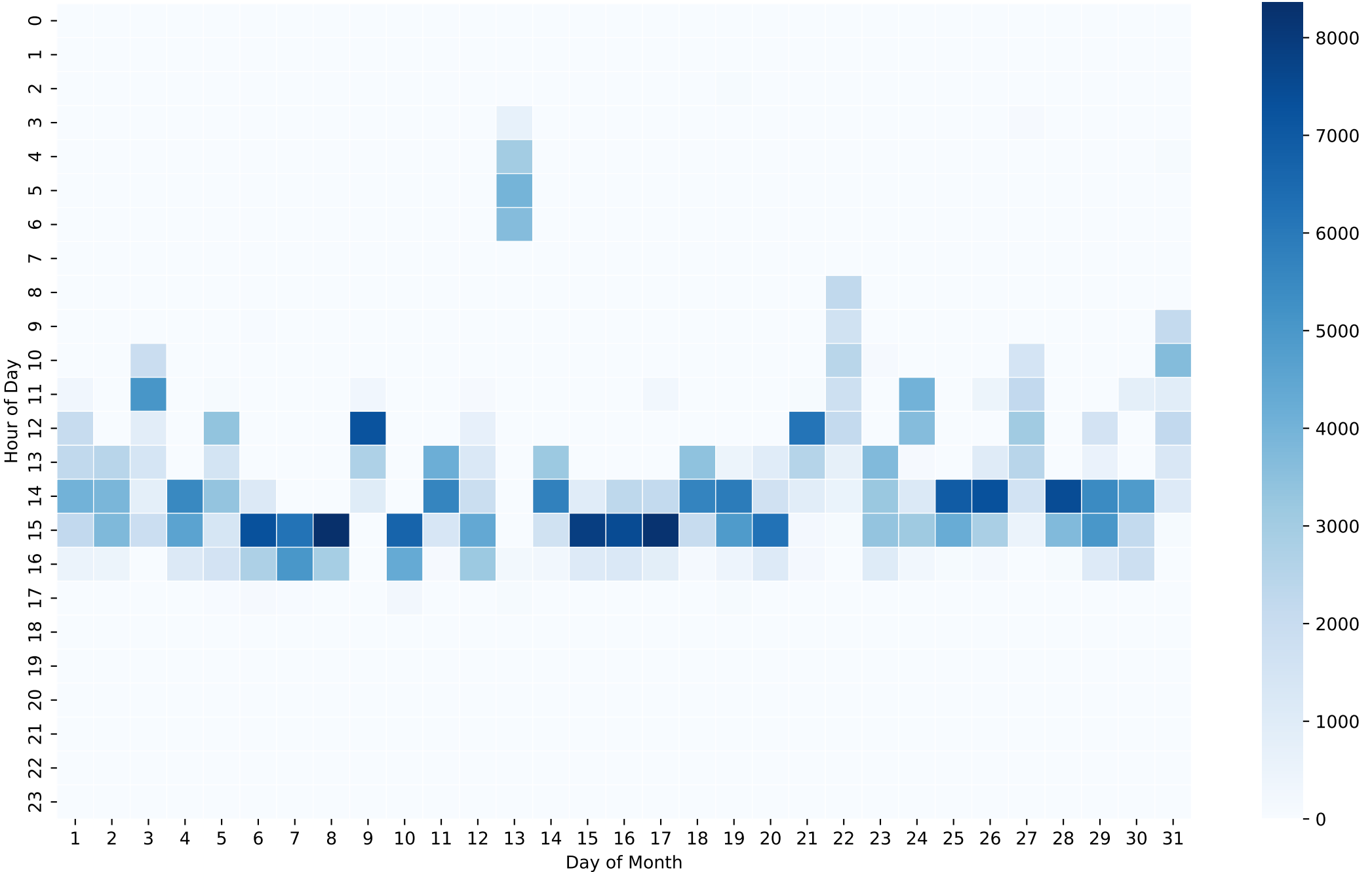
Battery Charging Power Heatmap (Wh/Hour) - 12kWh - Jul
