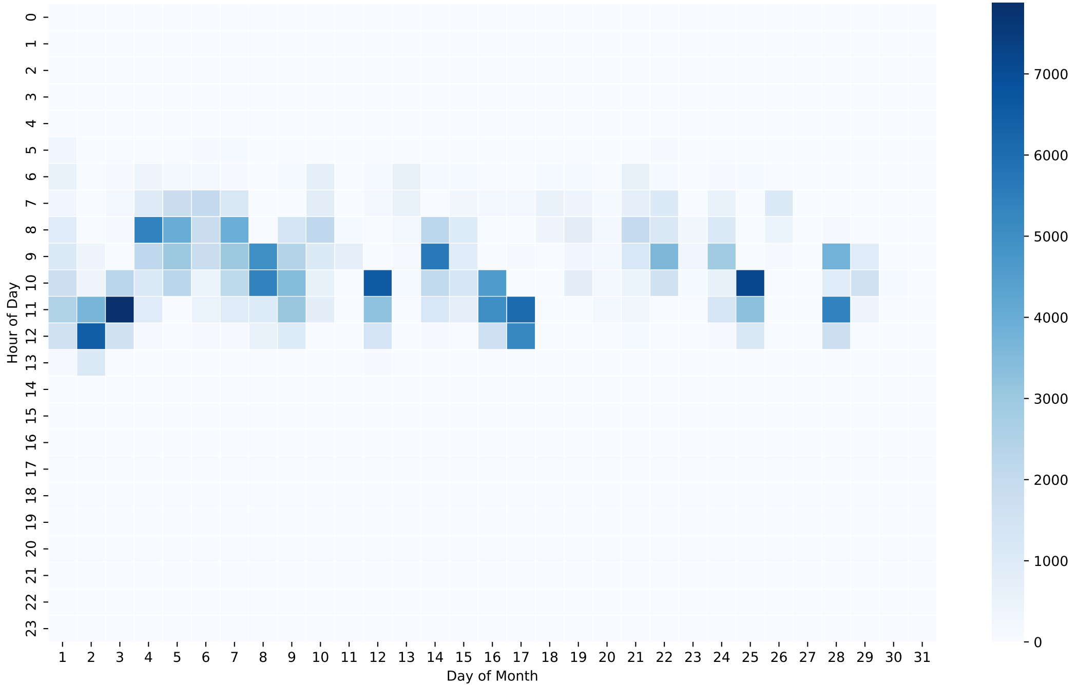
Battery Charging Power Heatmap (Wh/Hour) - 12kWh - Nov
