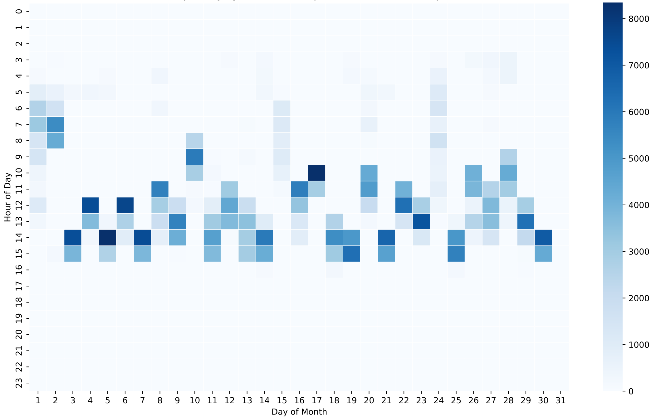
Battery Charging Power Heatmap (Wh/Hour) - 12kWh - Apr
