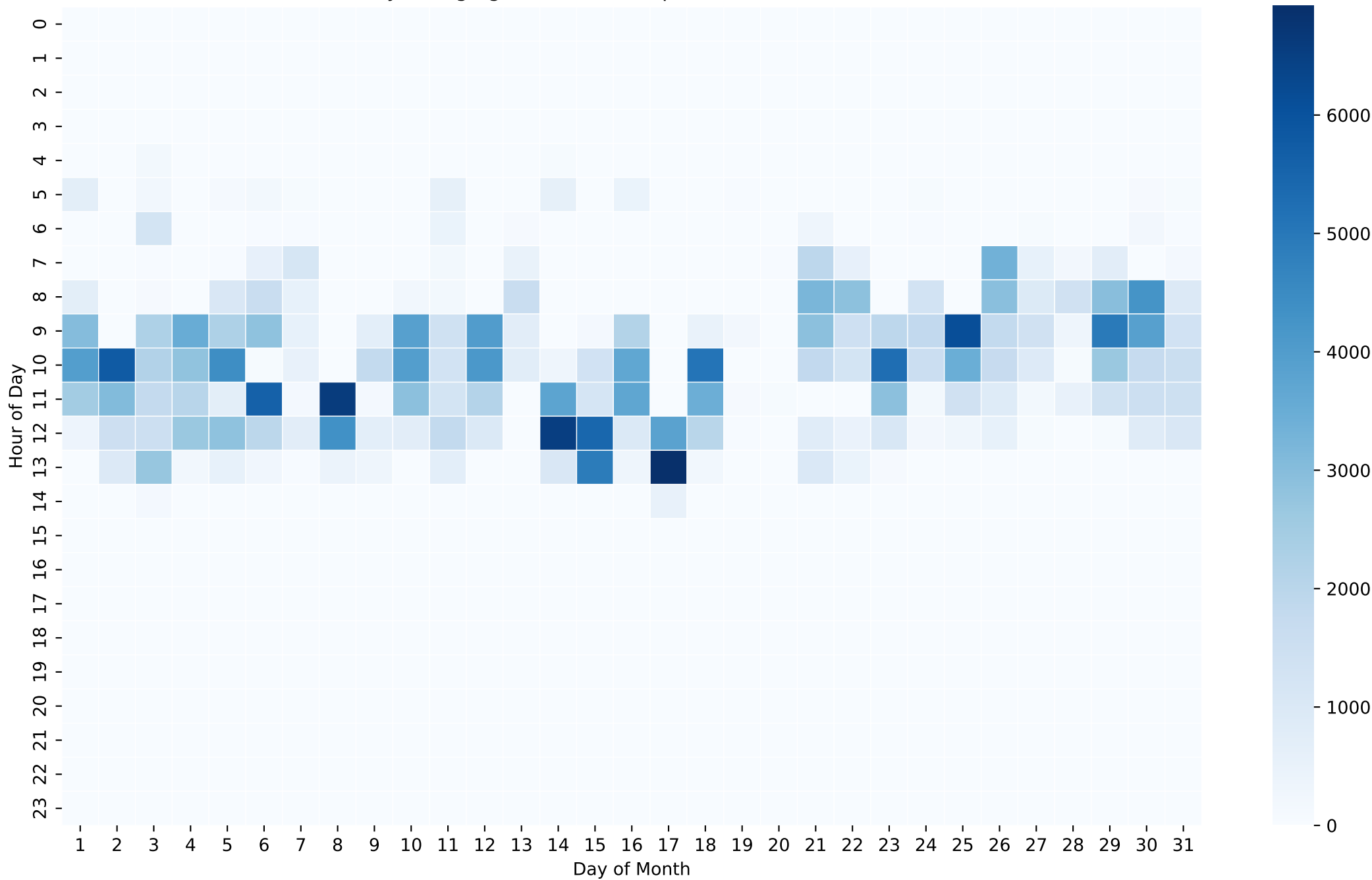
Battery Charging Power Heatmap (Wh/Hour) - 12kWh - Oct
