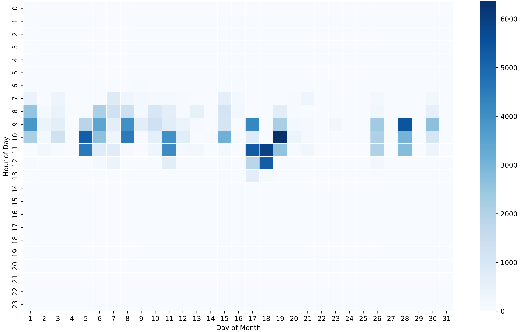
Battery Charging Power Heatmap (Wh/Hour) - 12kWh - Jan
