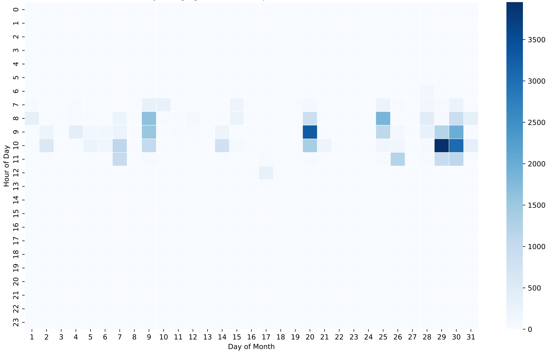
Battery Charging Power Heatmap (Wh/Hour) - 12kWh - Dec
