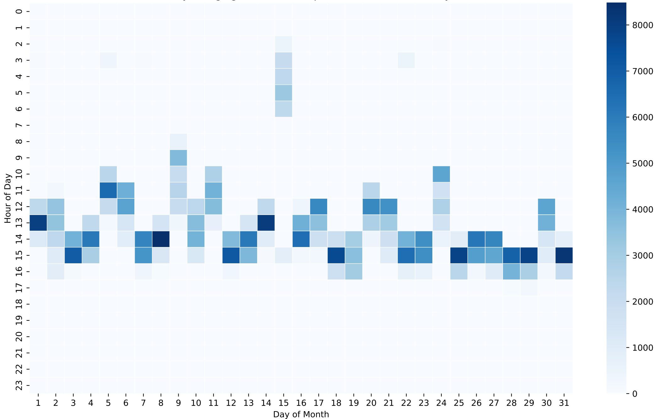
Battery Charging Power Heatmap (Wh/Hour) - 12kWh - May
