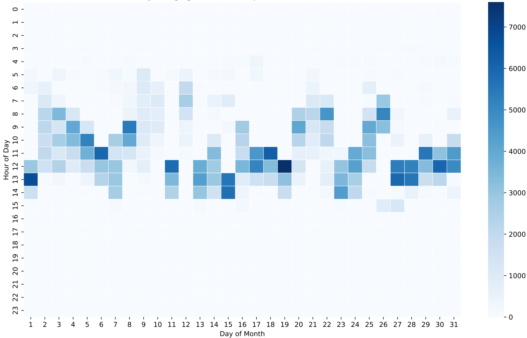
Battery Charging Power Heatmap (Wh/Hour) - 12kWh - Mar
