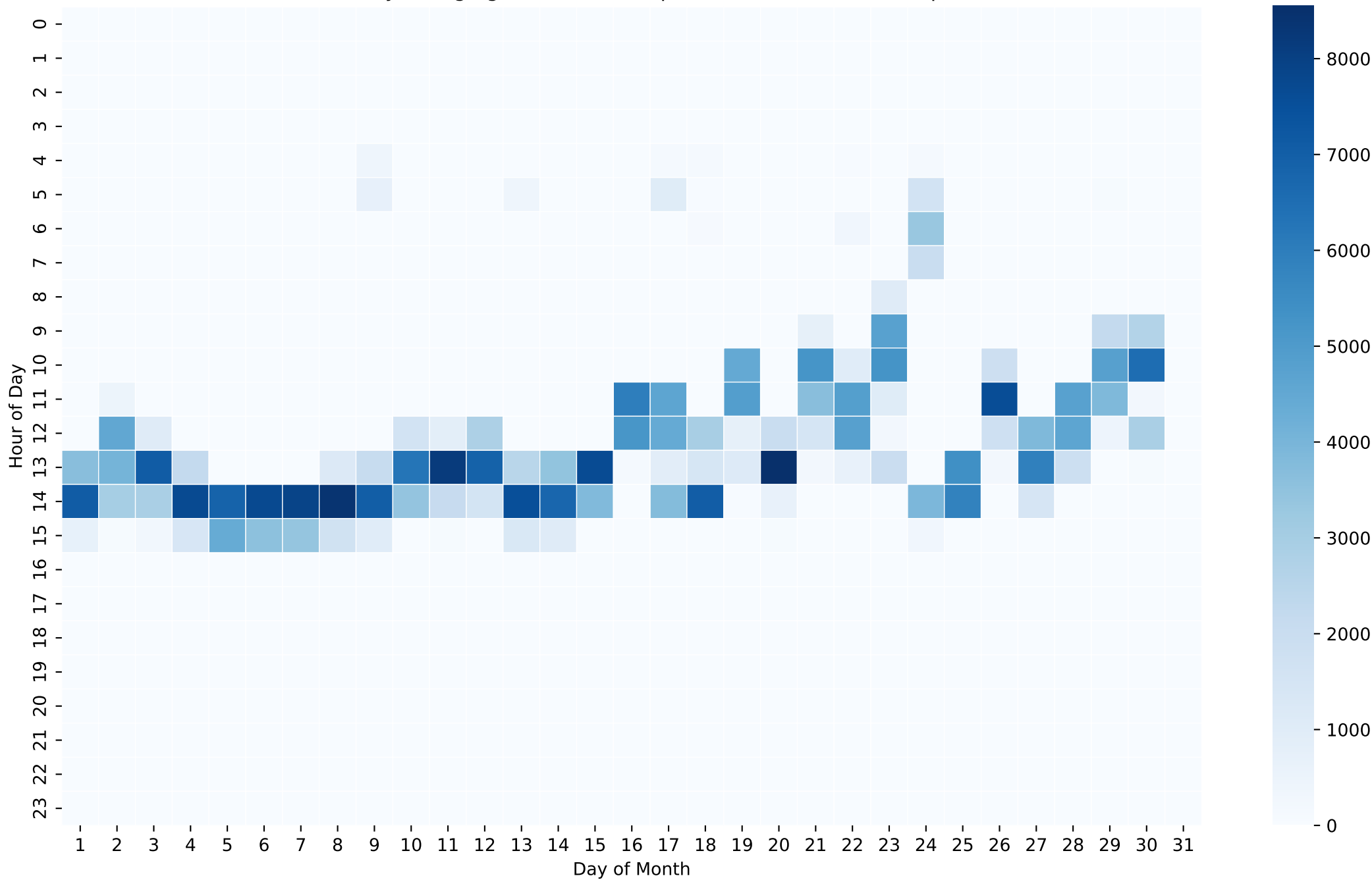
Battery Charging Power Heatmap (Wh/Hour) - 12kWh - Sep
