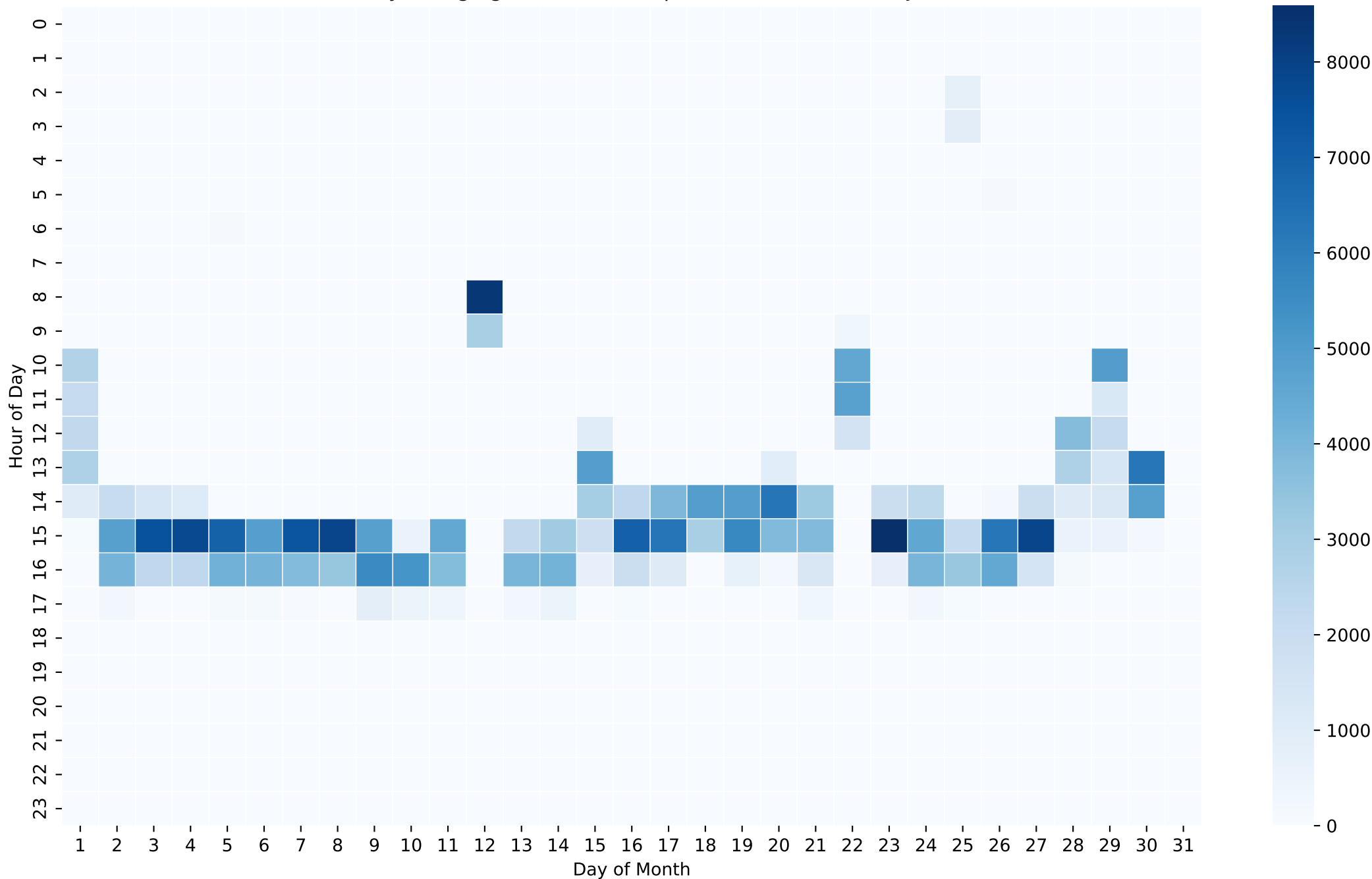
Battery Charging Power Heatmap (Wh/Hour) - 12kWh - Jun
