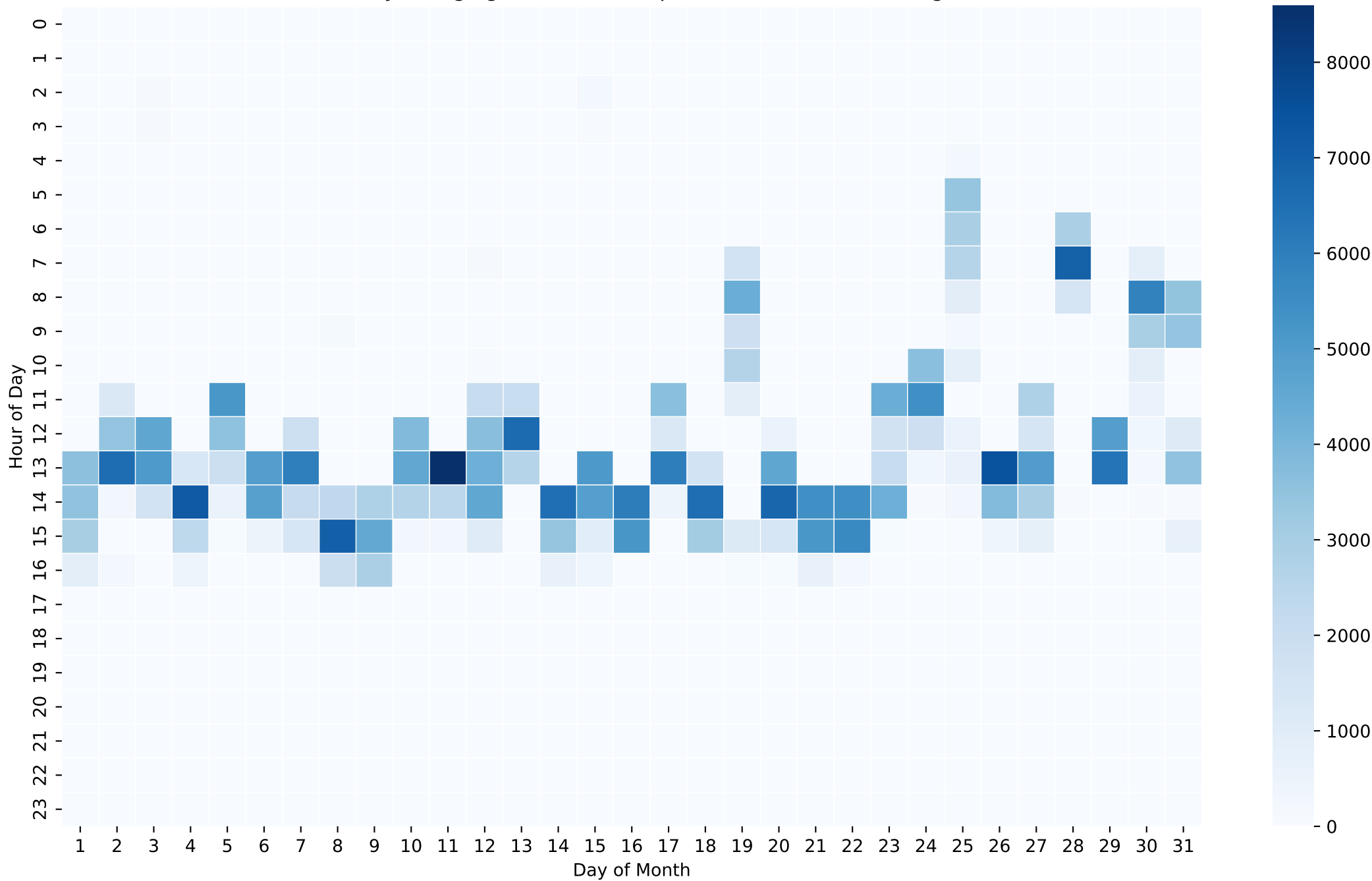
Battery Charging Power Heatmap (Wh/Hour) - 12kWh - Aug
