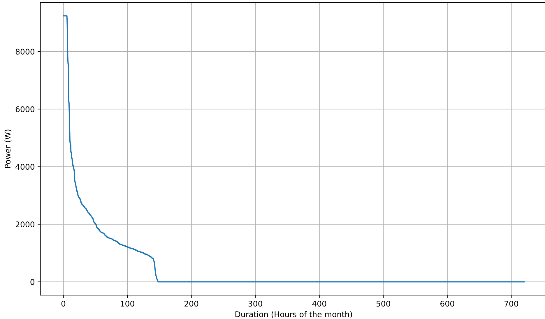
Battery Discharging Power Duration Curve - 12kWh - Sep
