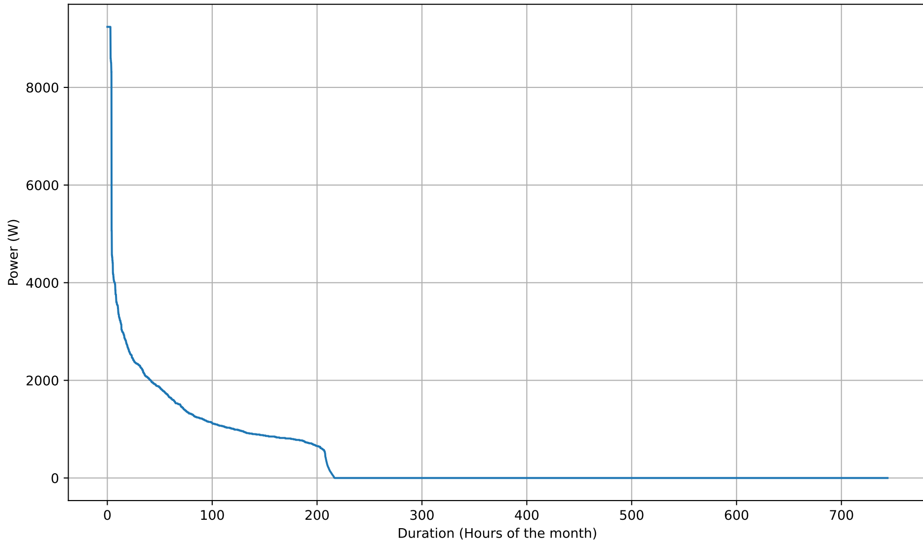
Battery Discharging Power Duration Curve - 12kWh - Jul
