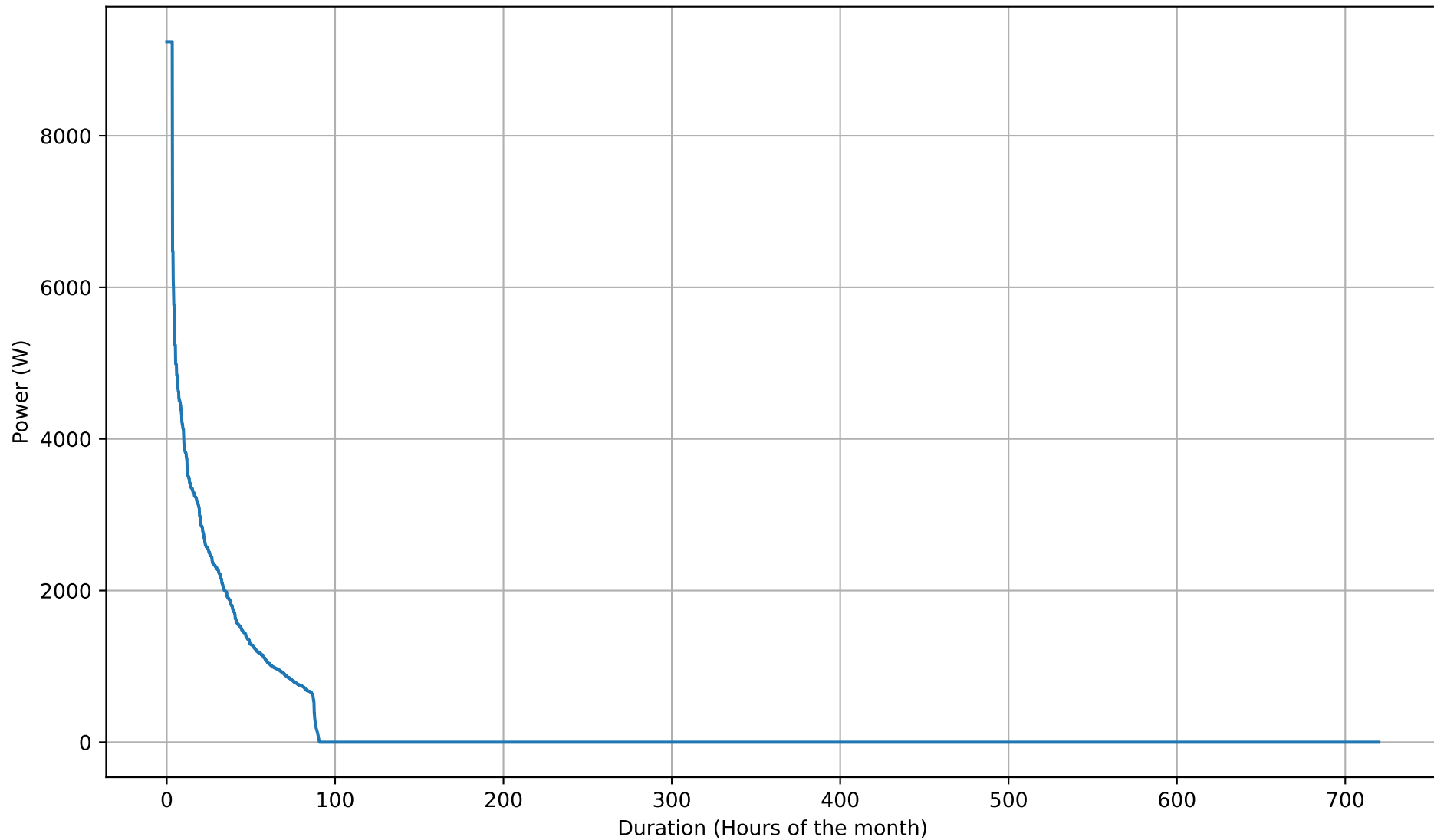
Battery Discharging Power Duration Curve - 12kWh - Nov
