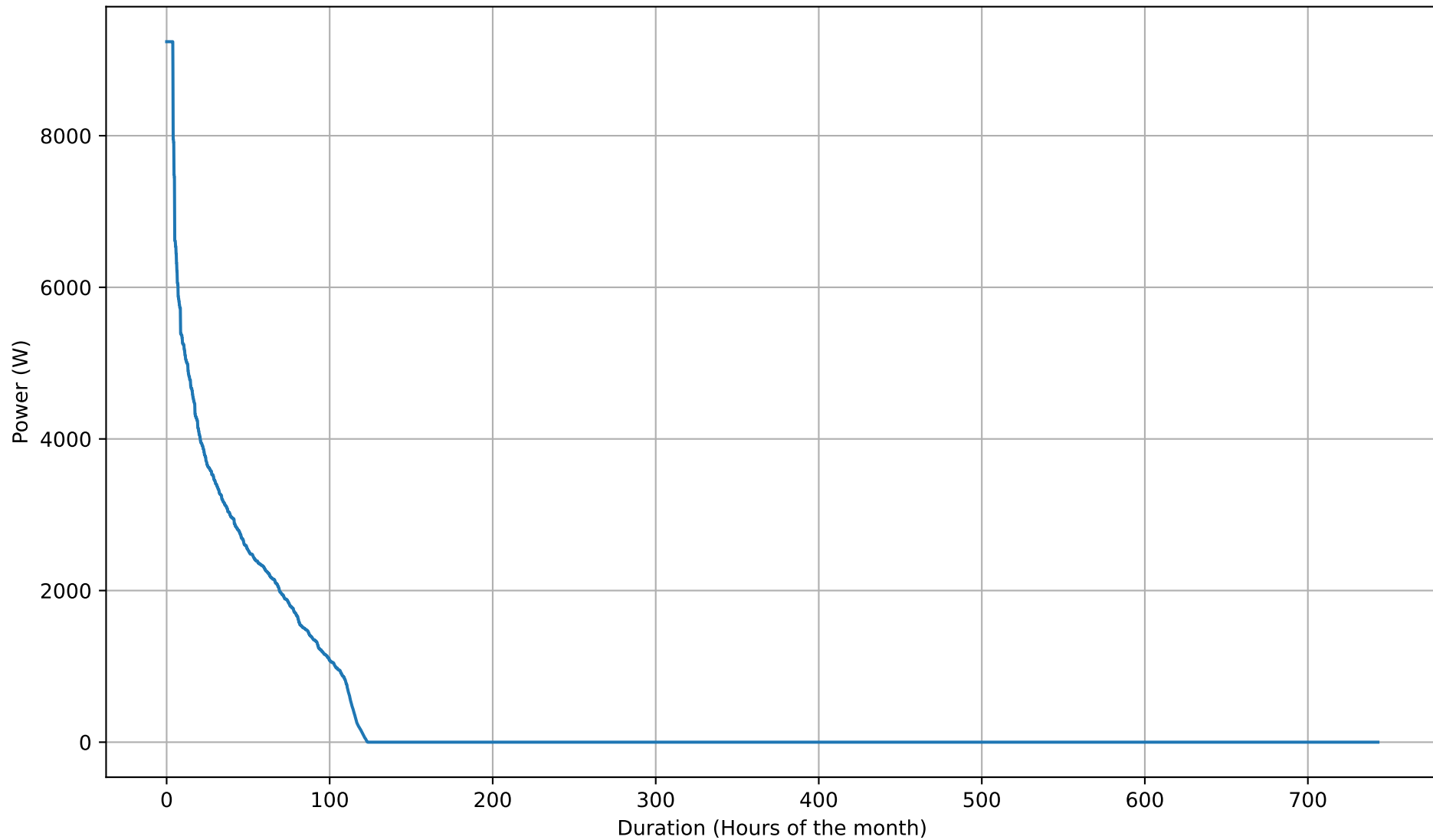
Battery Discharging Power Duration Curve - 12kWh - Mar
