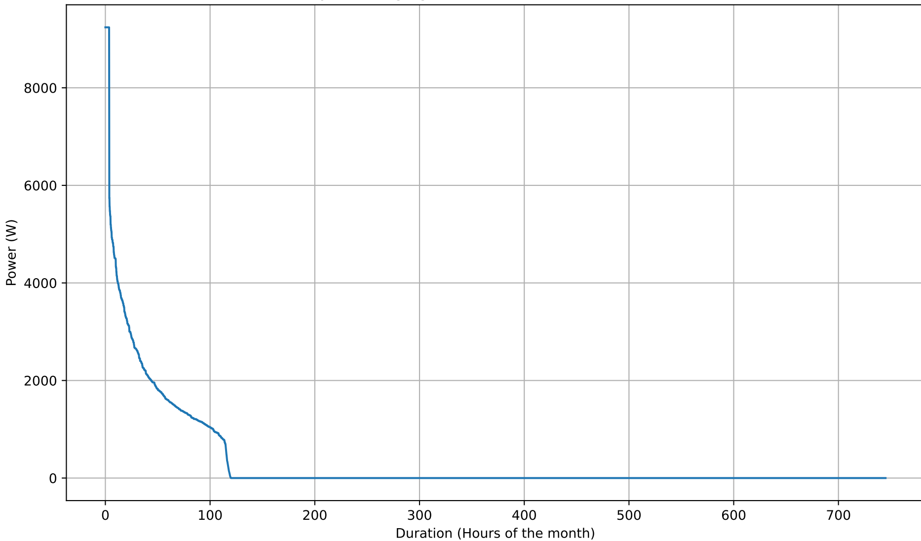
Battery Discharging Power Duration Curve - 12kWh - Oct
