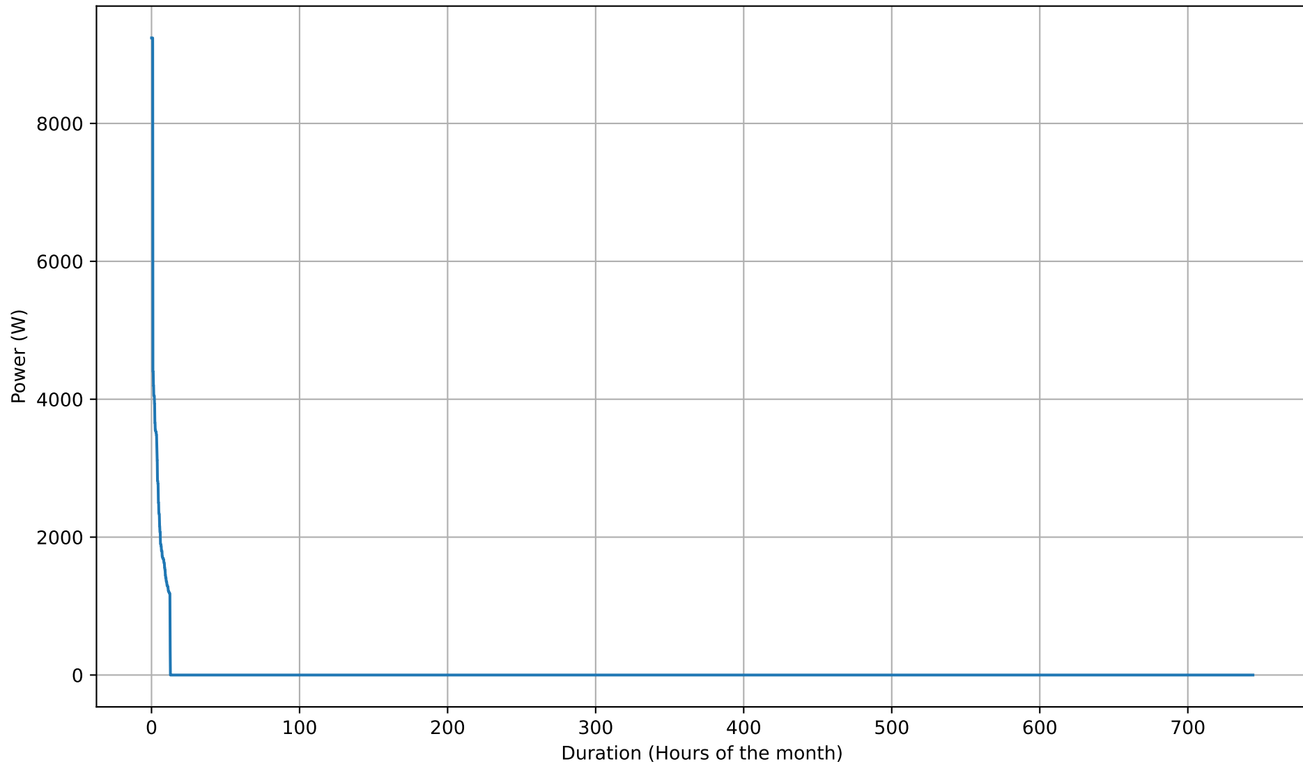
Battery Discharging Power Duration Curve - 12kWh - Dec
