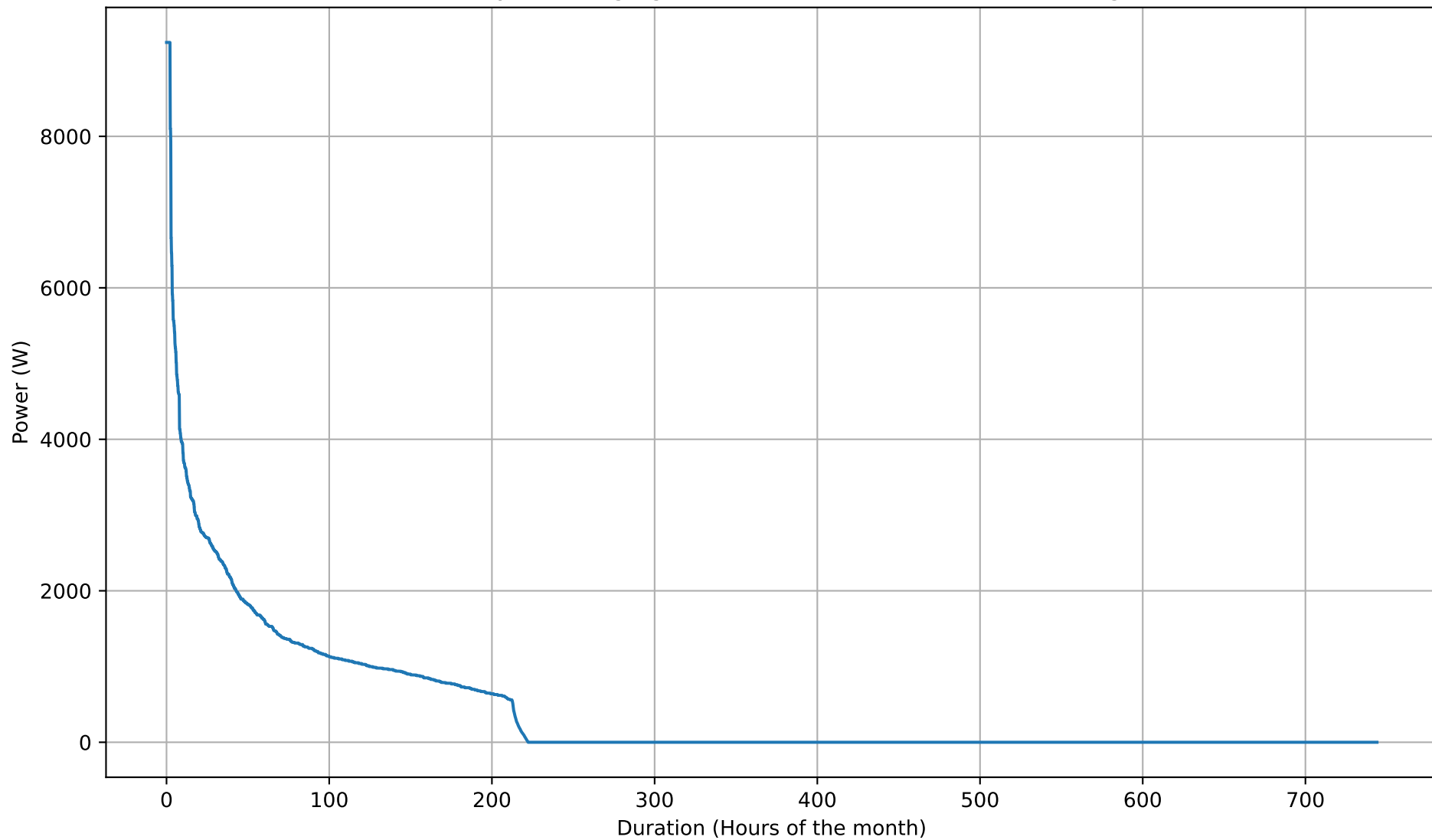
Battery Discharging Power Duration Curve - 12kWh - Aug
