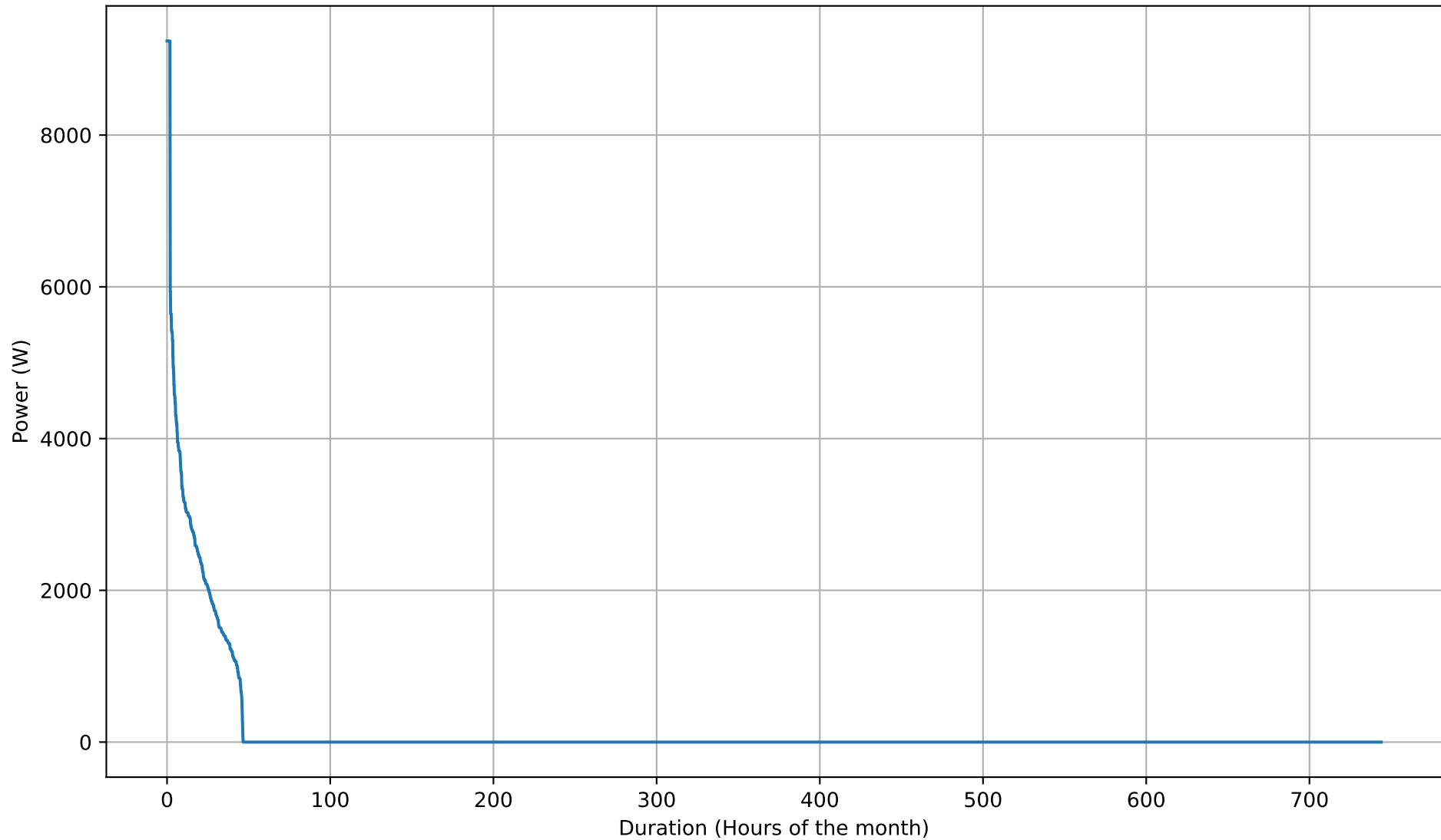
Battery Discharging Power Duration Curve - 12kWh - Jan
