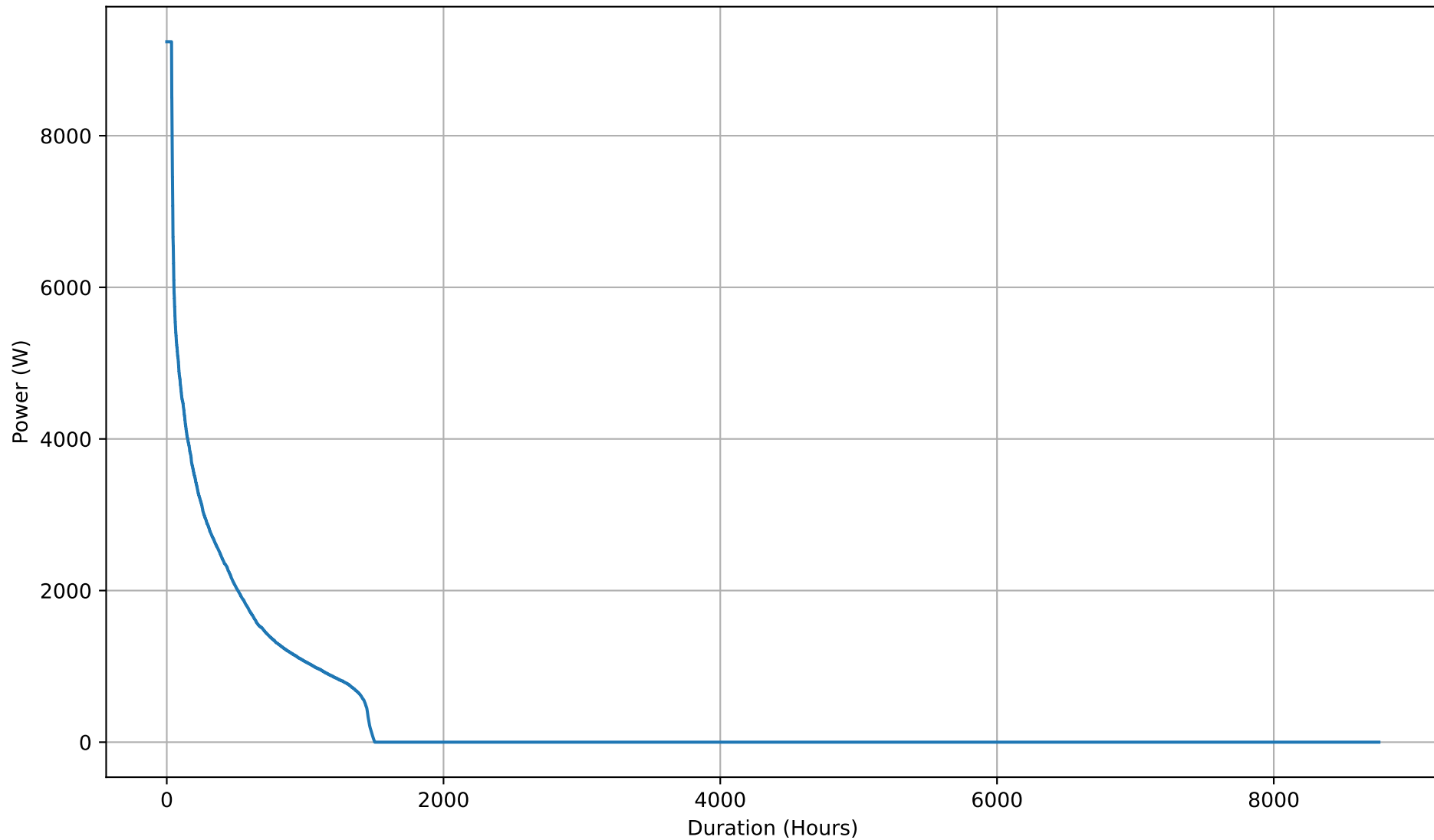
Yearly Battery Discharging Power Duration Curve - 12kWh
