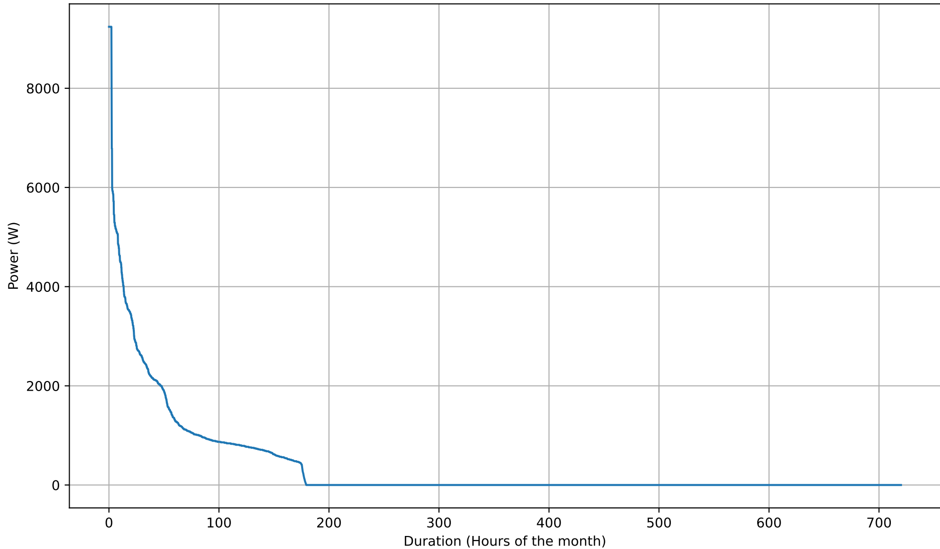
Battery Discharging Power Duration Curve - 12kWh - Jun
