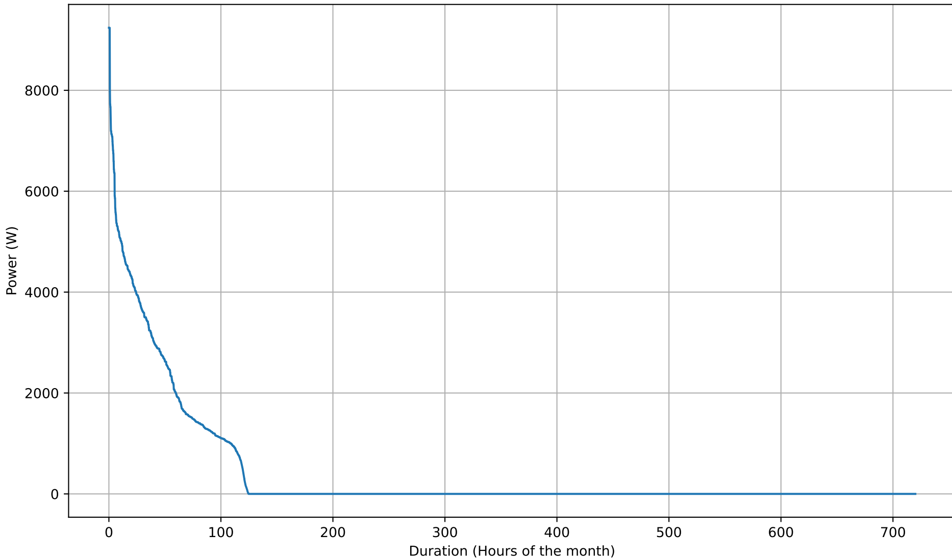
Battery Discharging Power Duration Curve - 12kWh - Apr
