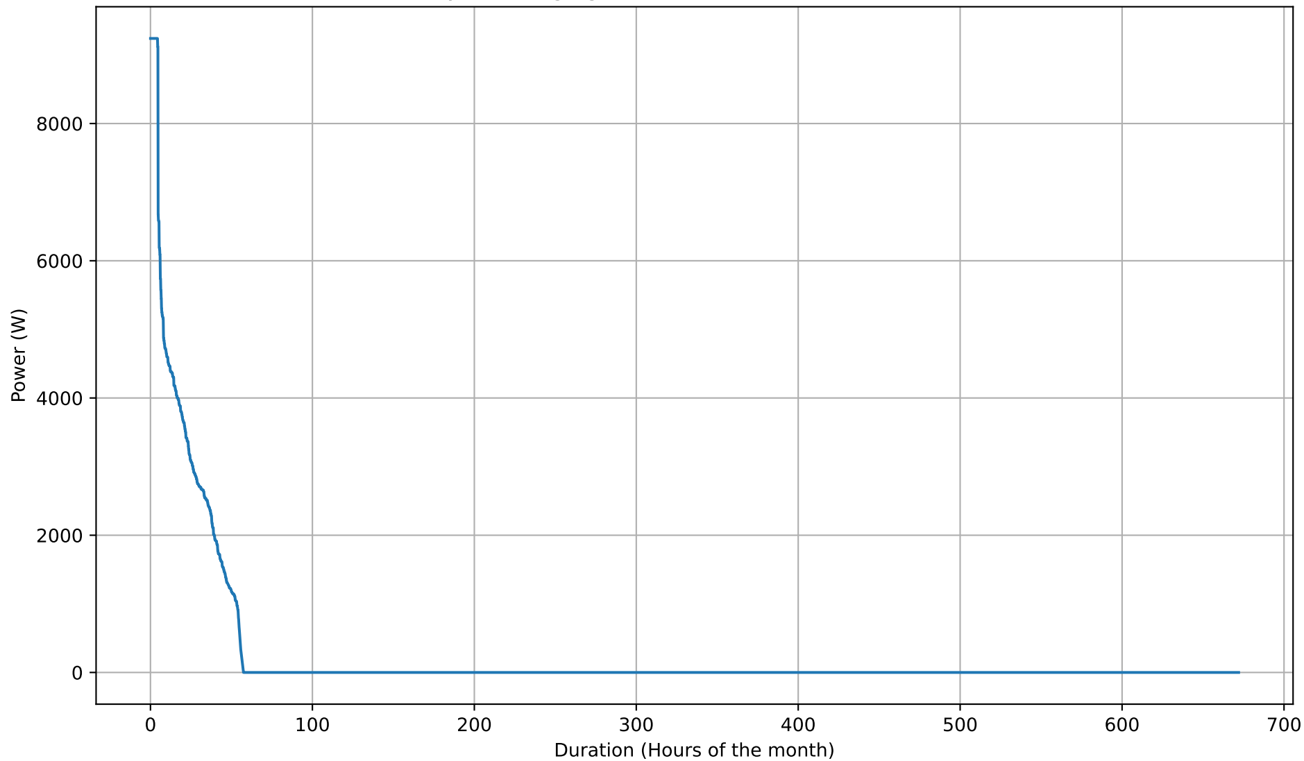
Battery Discharging Power Duration Curve - 12kWh - Feb
