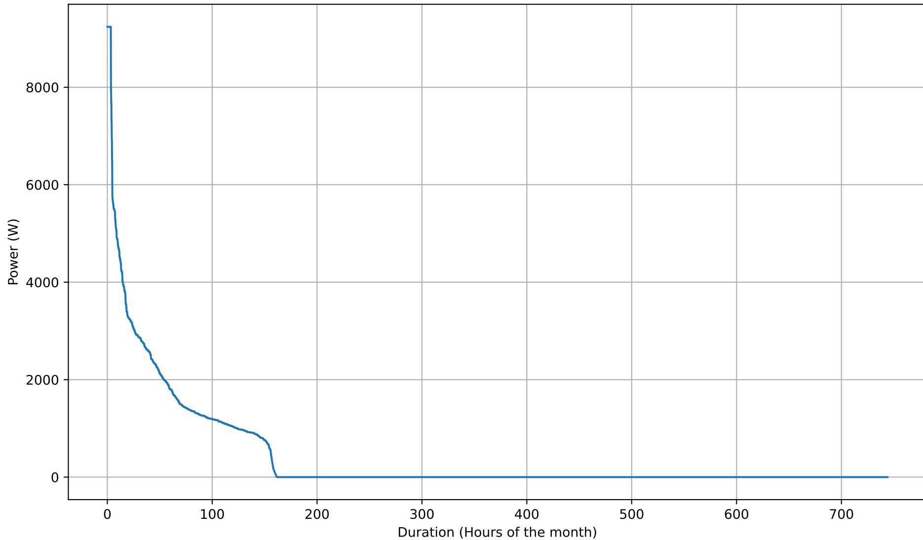
Battery Discharging Power Duration Curve - 12kWh - May
