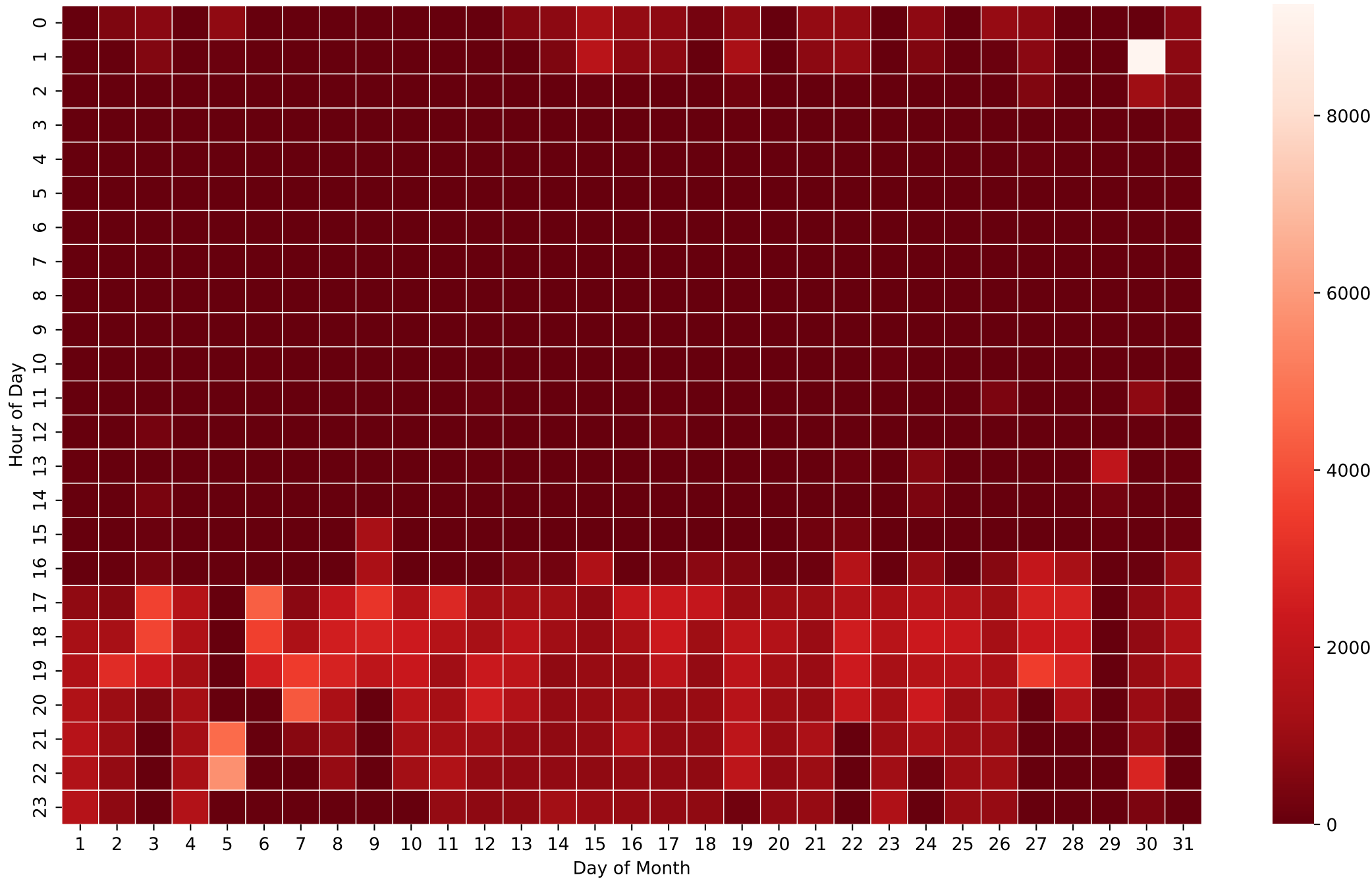
Battery Discharging Power Heatmap (Wh/Hour) - 12kWh - Jul
