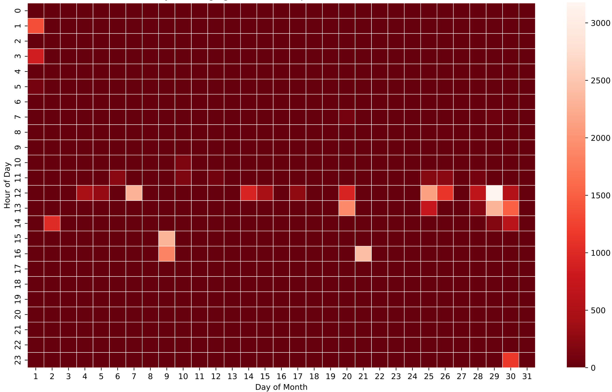
Battery Discharging Power Heatmap (Wh/Hour) - 12kWh - Dec
