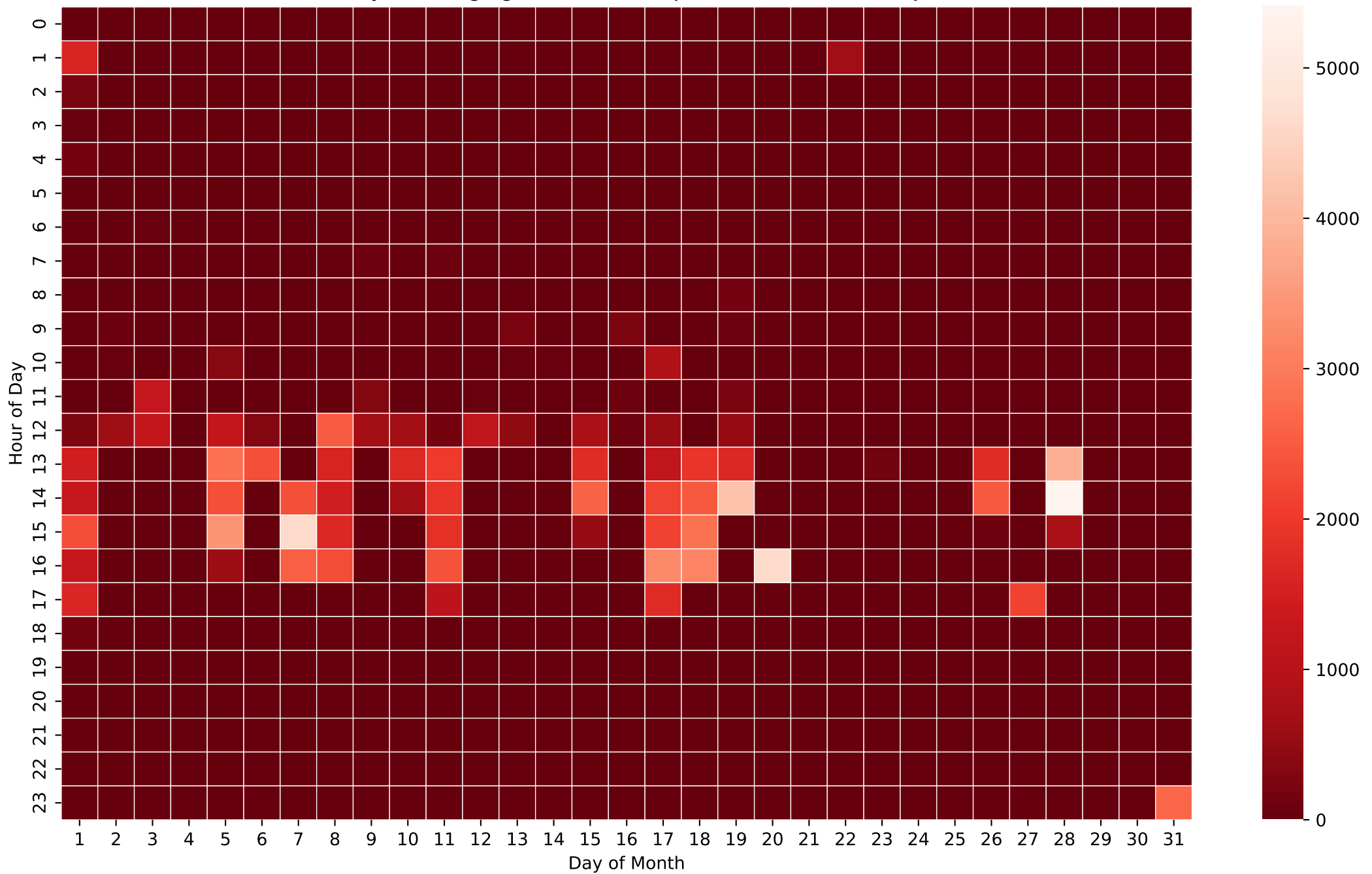
Battery Discharging Power Heatmap (Wh/Hour) - 12kWh - Jan
