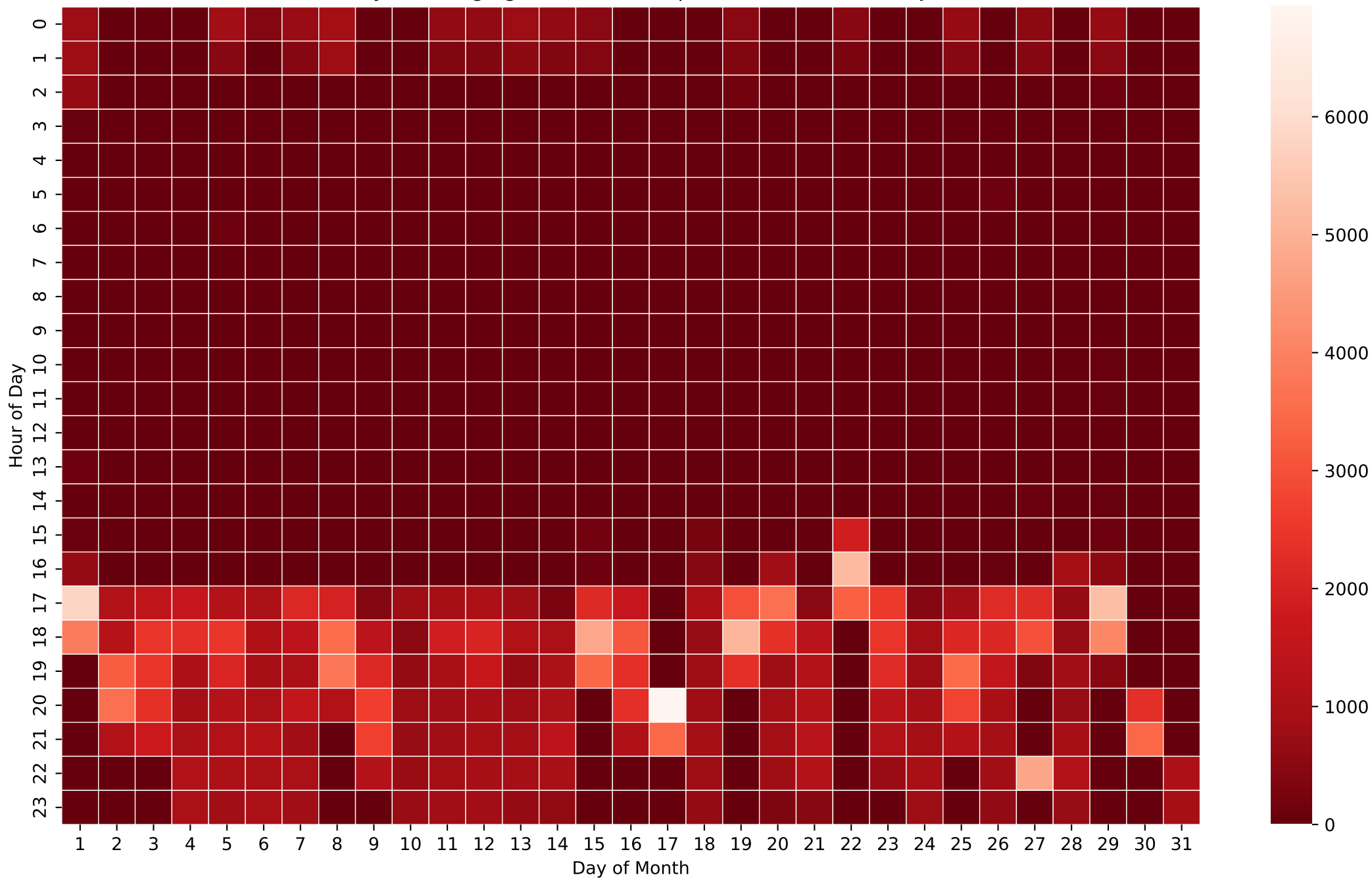
Battery Discharging Power Heatmap (Wh/Hour) - 12kWh - Jun
