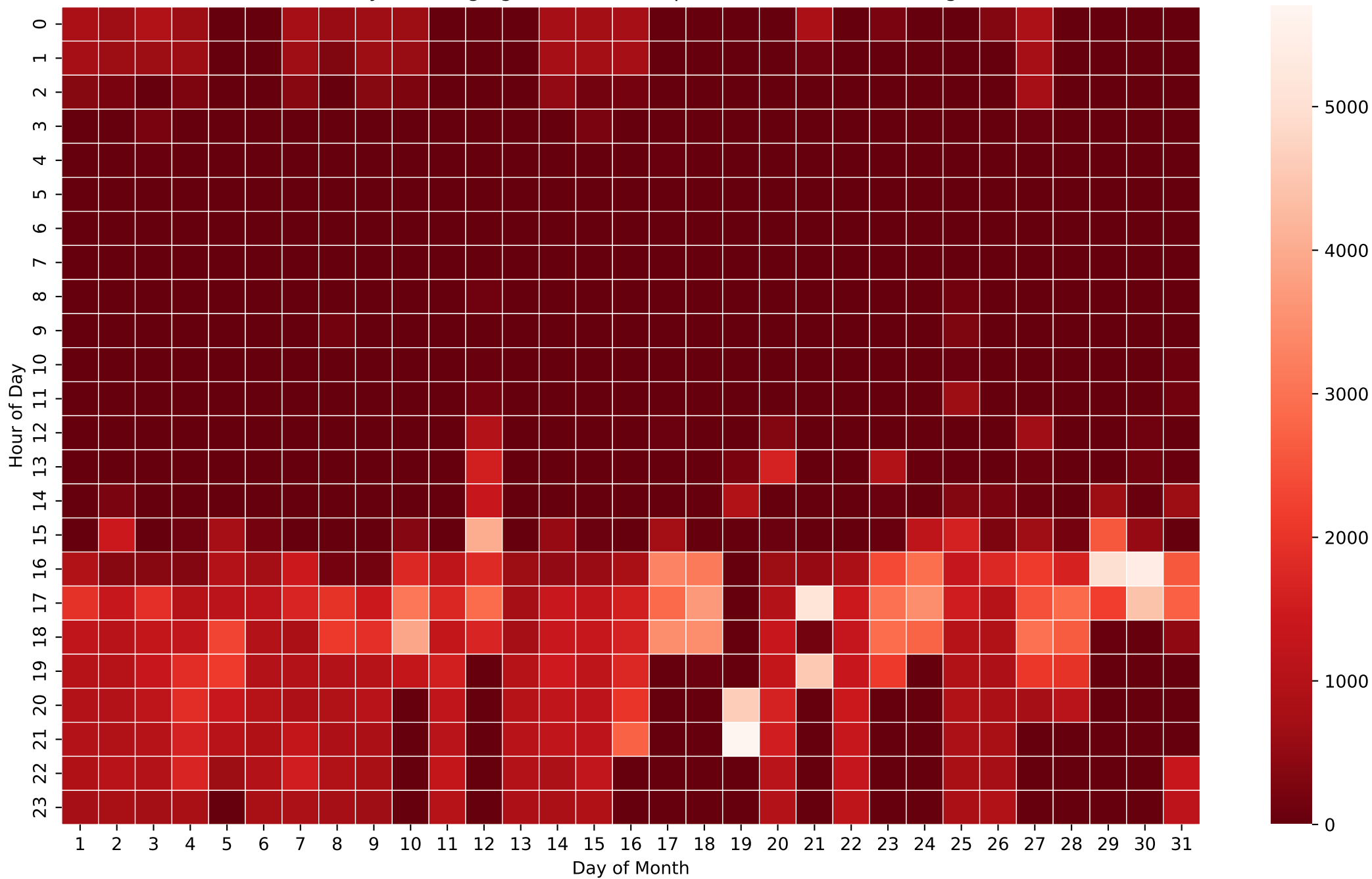
Battery Discharging Power Heatmap (Wh/Hour) - 12kWh - Aug
