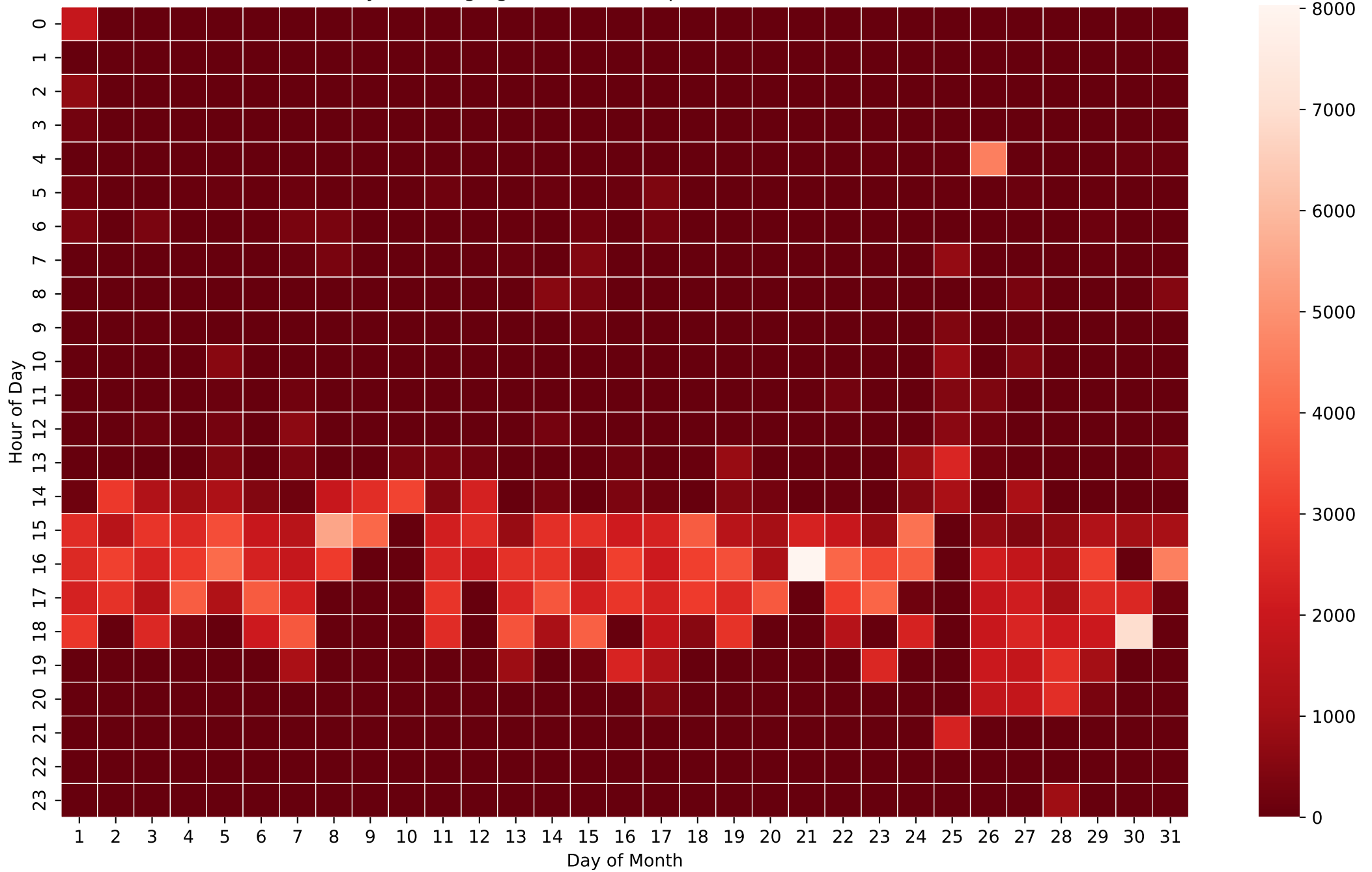
Battery Discharging Power Heatmap (Wh/Hour) - 12kWh - Mar
