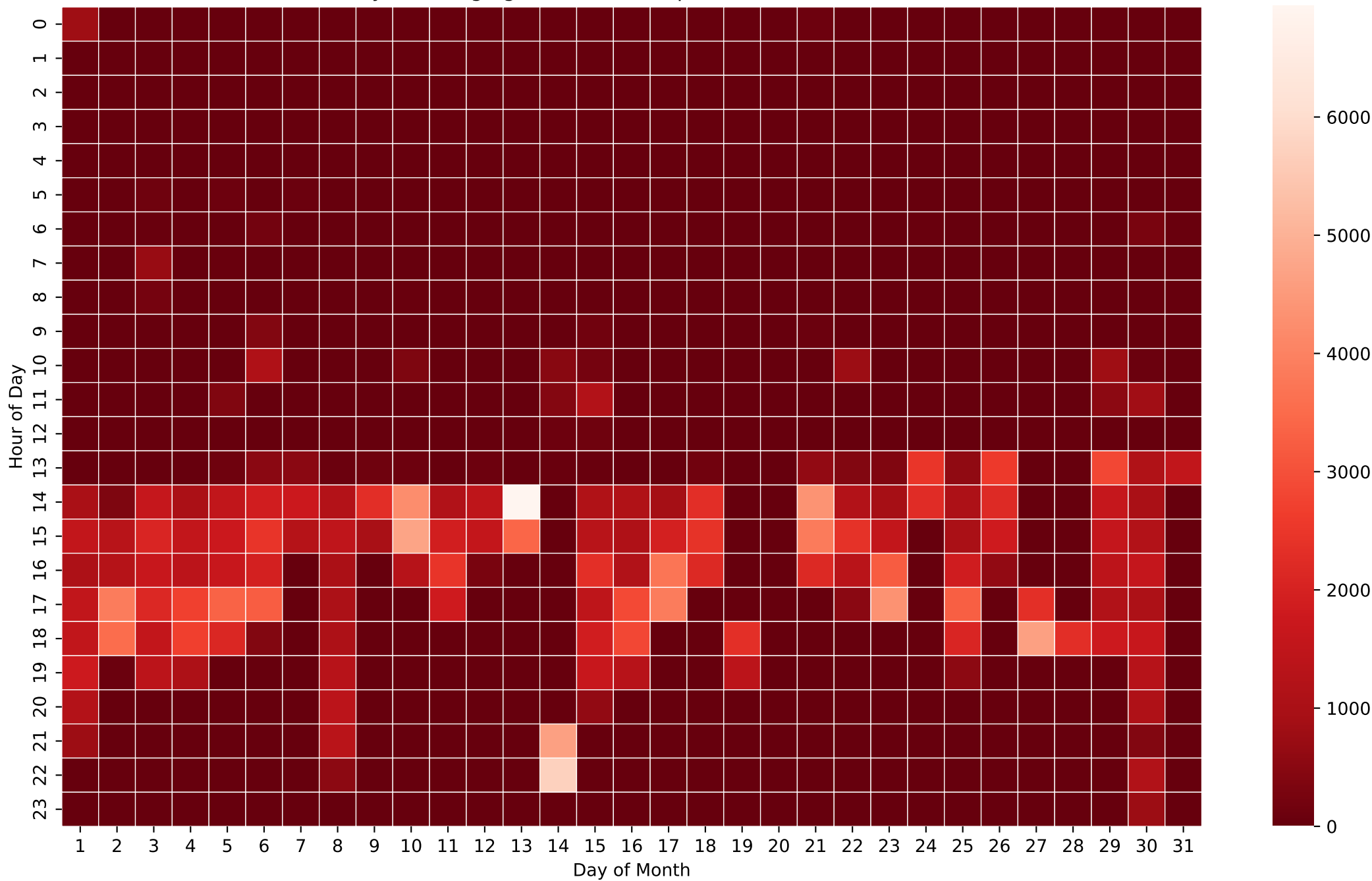
Battery Discharging Power Heatmap (Wh/Hour) - 12kWh - Oct
