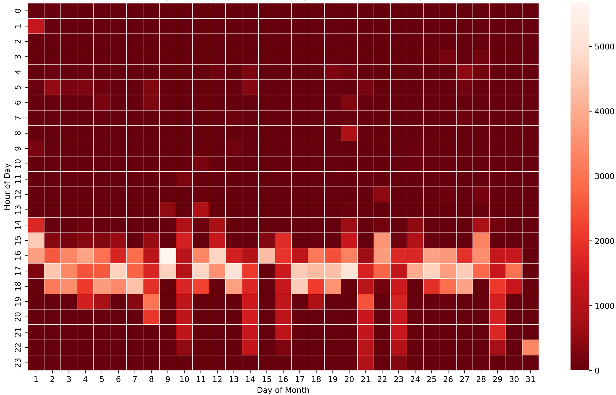
Battery Discharging Power Heatmap (Wh/Hour) - 12kWh - Apr
