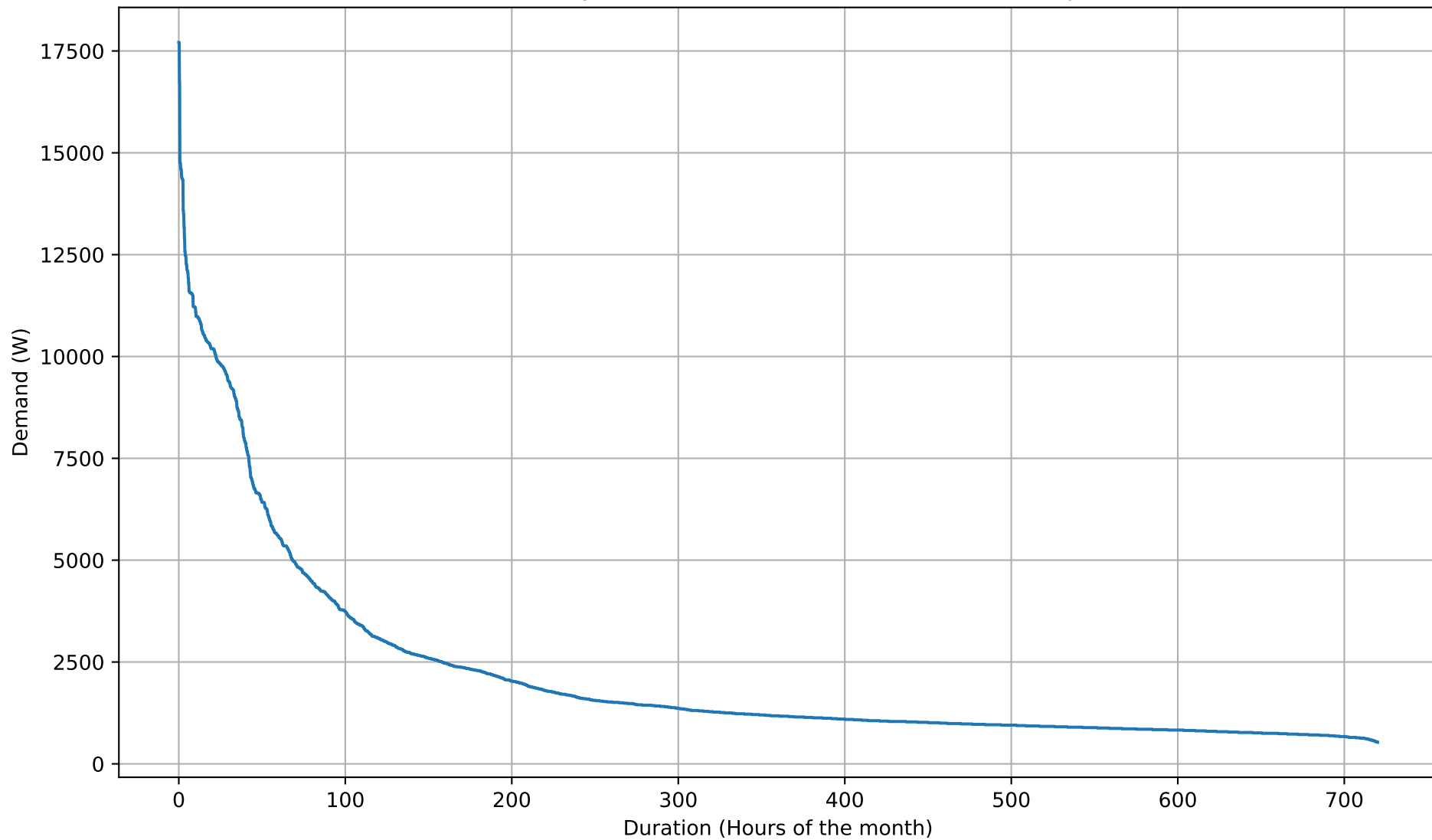
Electricity Demand Duration Curve - 12kWh - Sep
