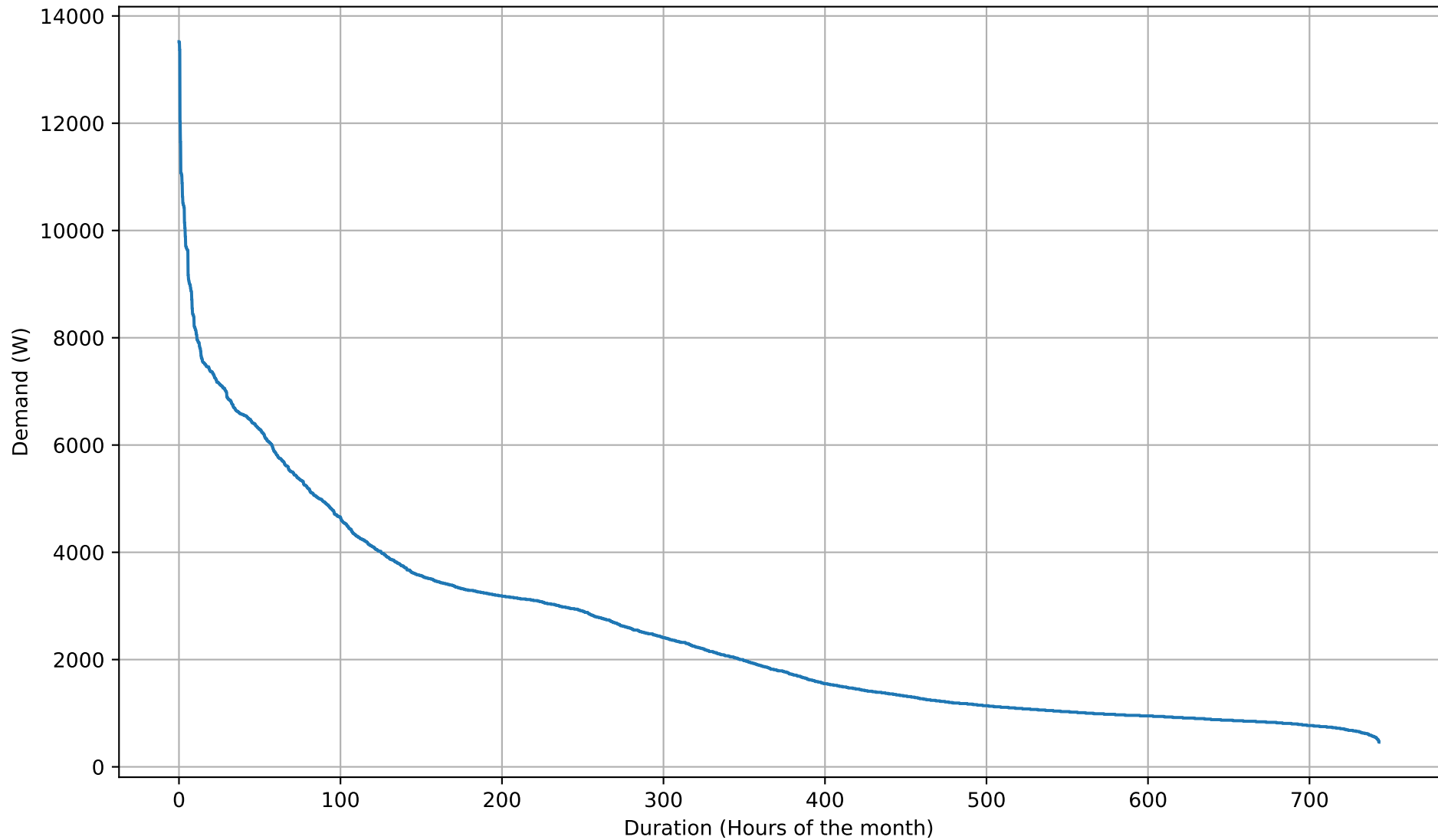
Electricity Demand Duration Curve - 12kWh - Mar
