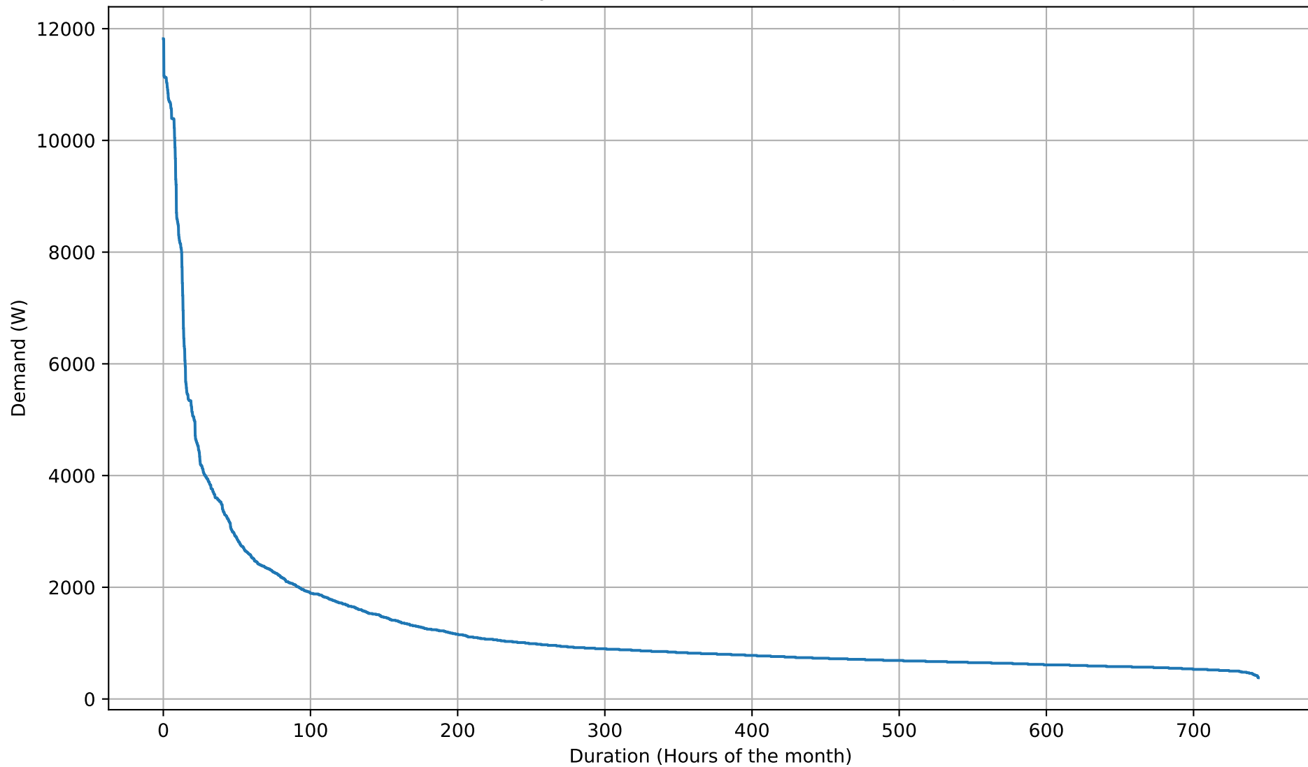
Electricity Demand Duration Curve - 12kWh - Jul
