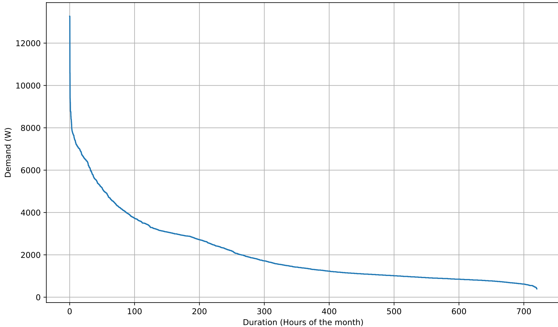
Electricity Demand Duration Curve - 12kWh - Apr
