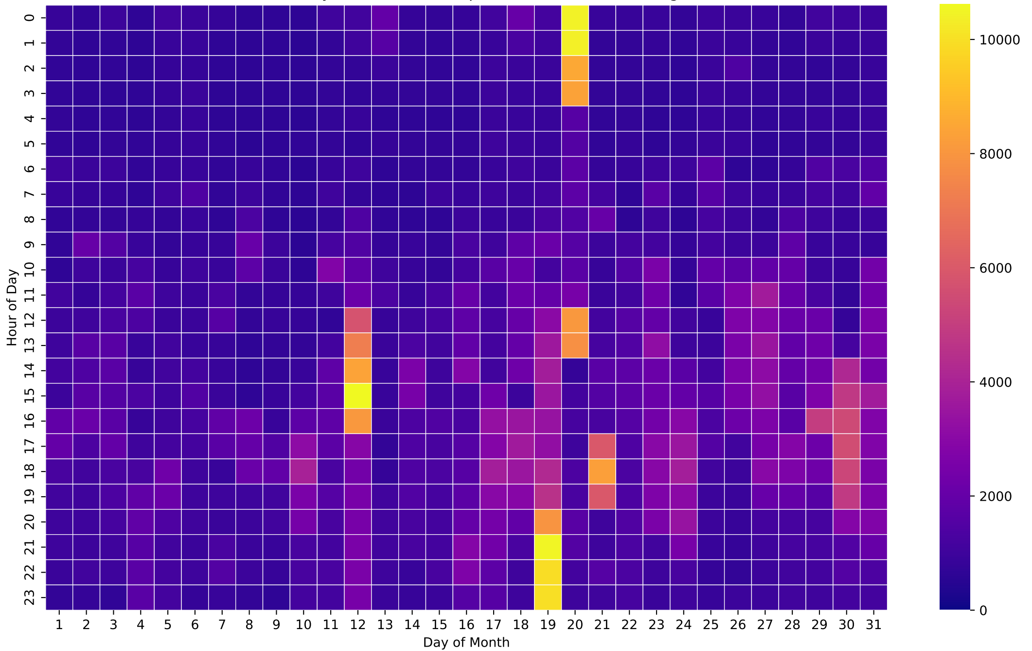
Electricity Demand Heatmap (Wh/Hour) - 12kWh - Aug
