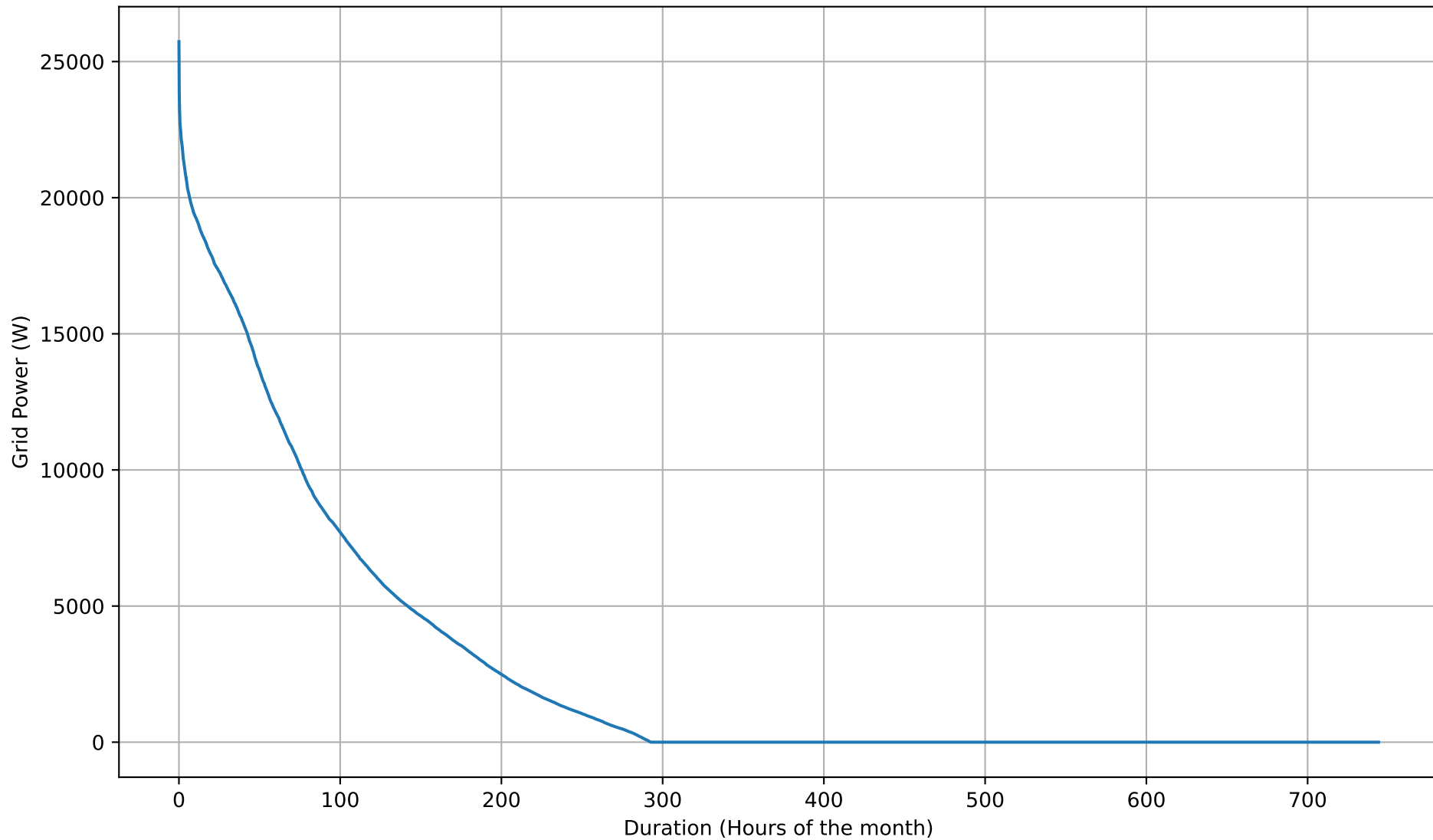
Grid Export Duration Curve - 12kWh - Aug
