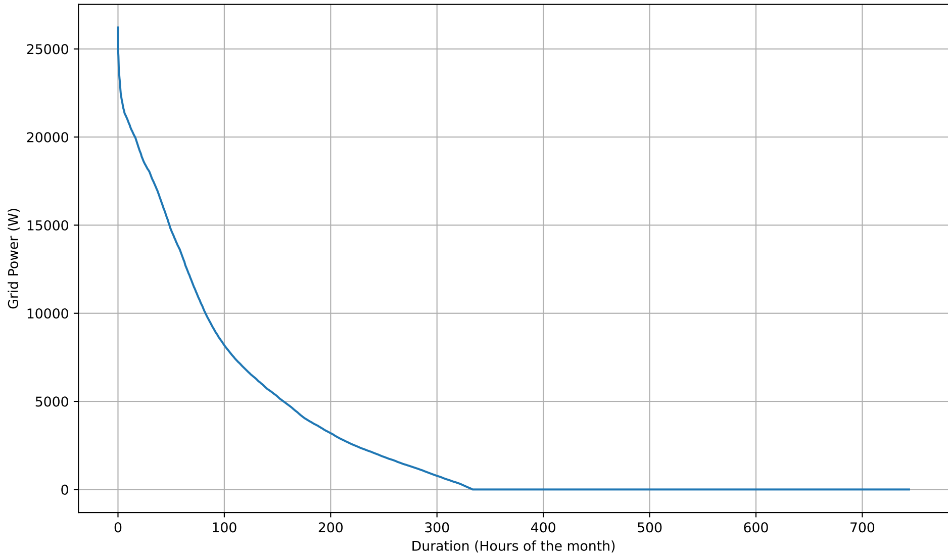
Grid Export Duration Curve - 12kWh - Jul
