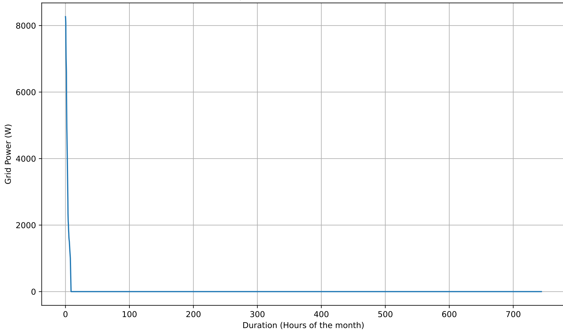
Grid Export Duration Curve - 12kWh - Jan
