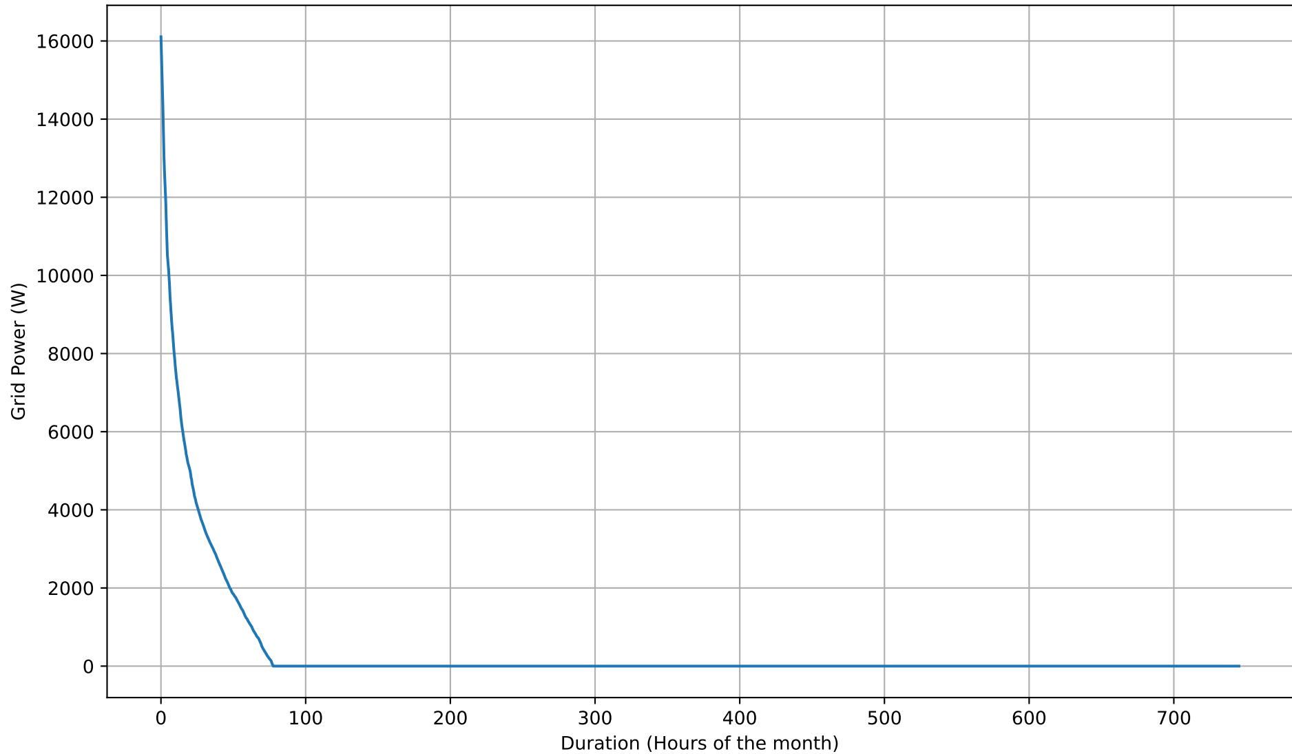
Grid Export Duration Curve - 12kWh - Oct
