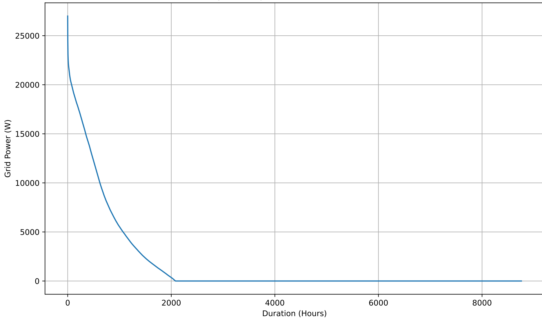
Yearly Grid Export Duration Curve - 12kWh
