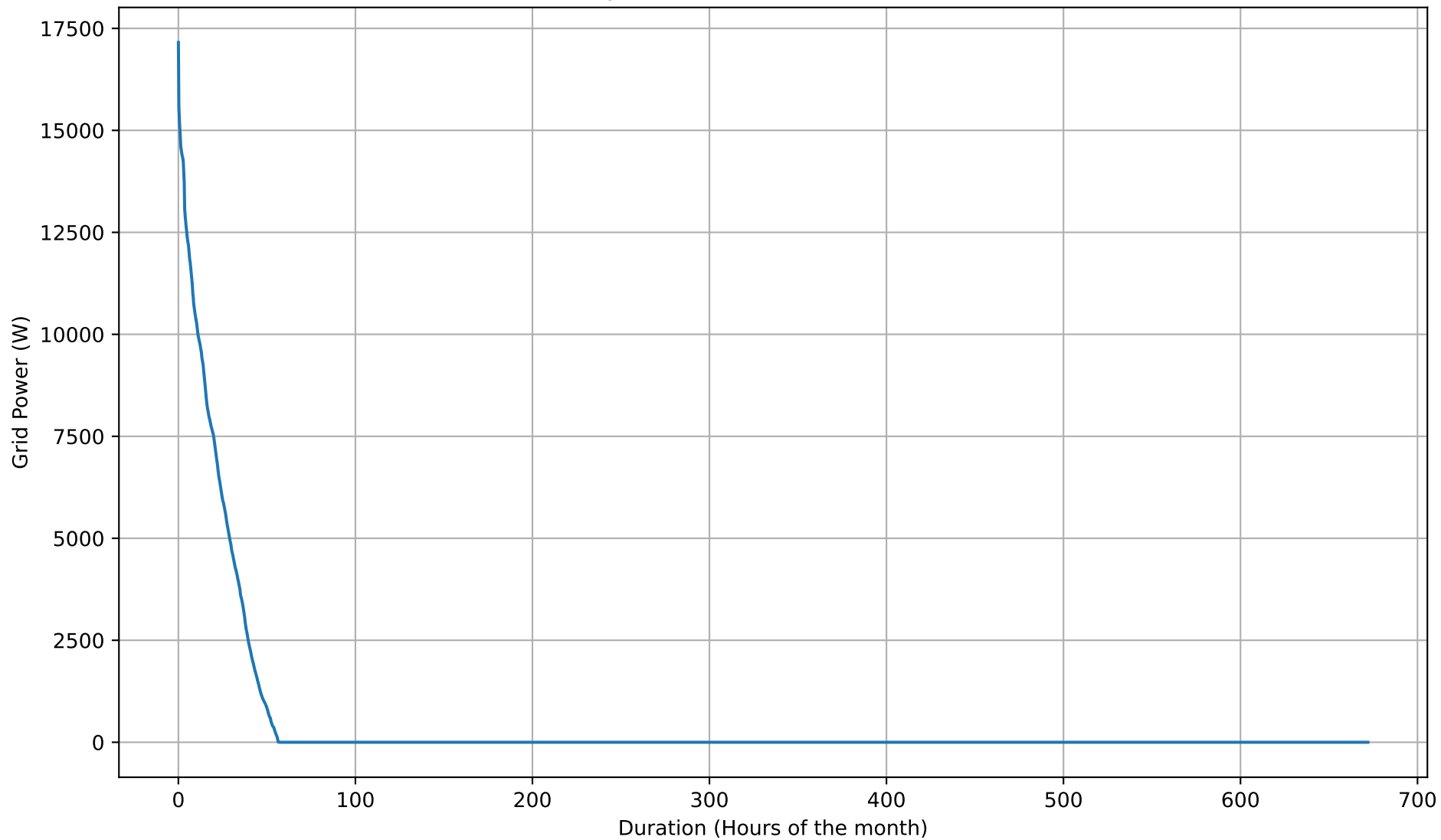
Grid Export Duration Curve - 12kWh - Feb
