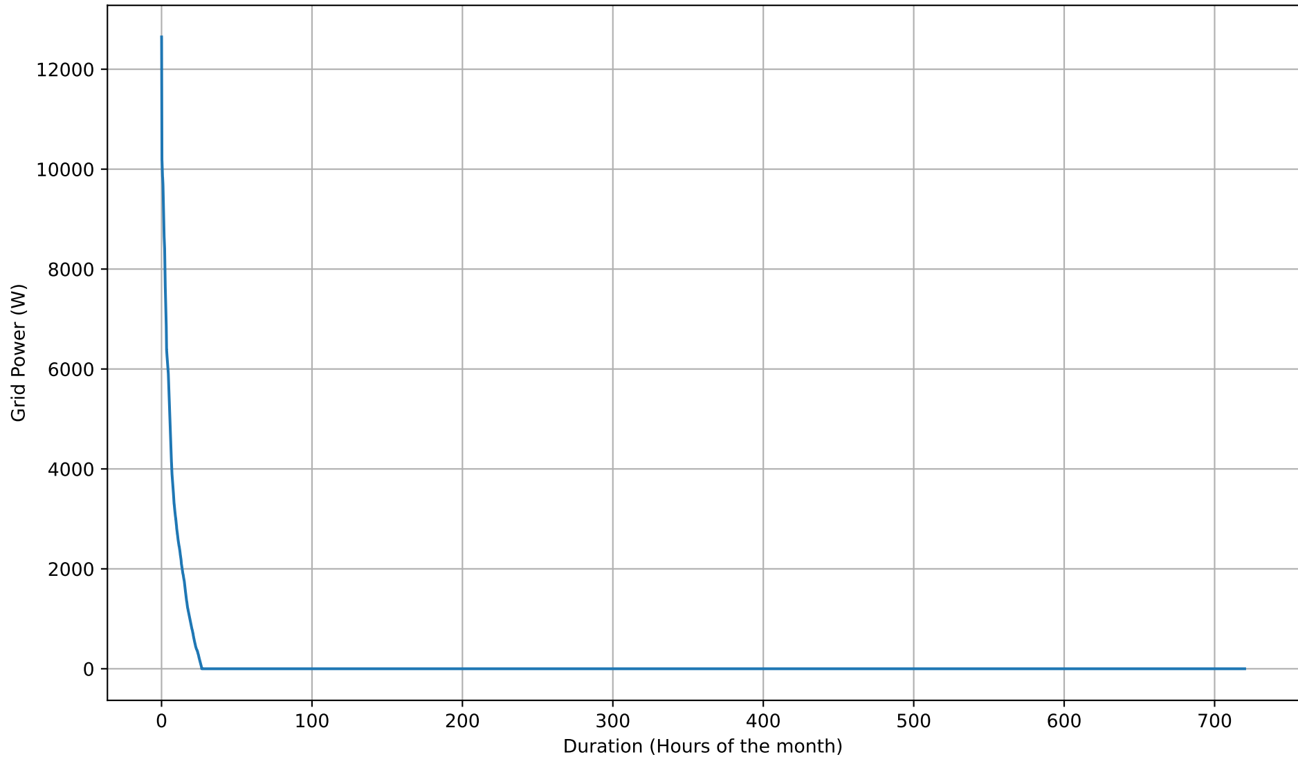
Grid Export Duration Curve - 12kWh - Nov
