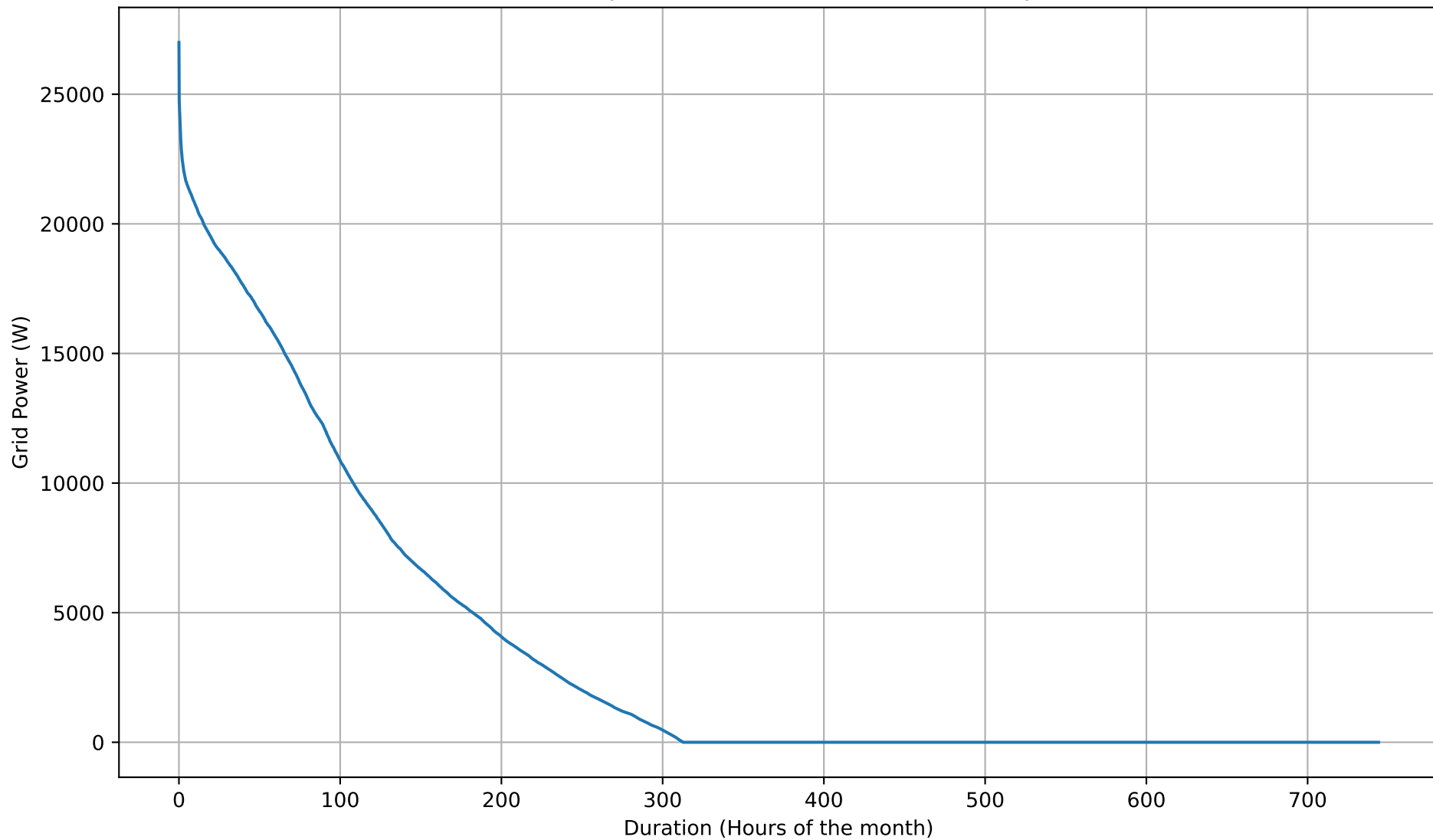
Grid Export Duration Curve - 12kWh - May
