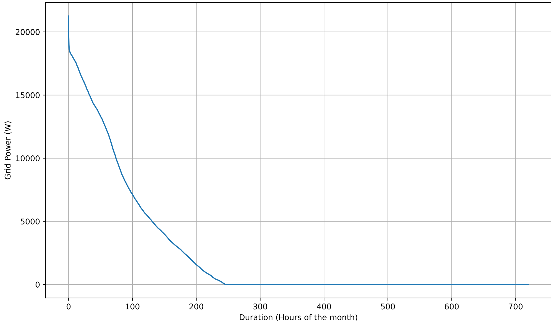
Grid Export Duration Curve - 12kWh - Sep
