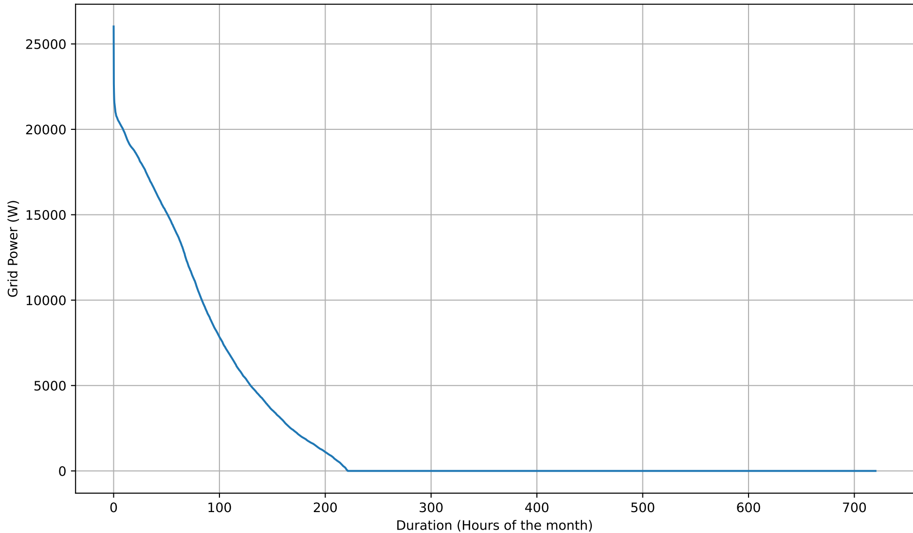
Grid Export Duration Curve - 12kWh - Apr
