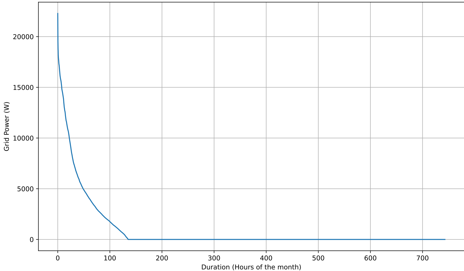
Grid Export Duration Curve - 12kWh - Mar
