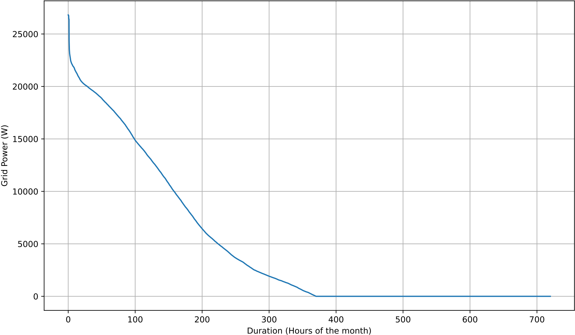
Grid Export Duration Curve - 12kWh - Jun
