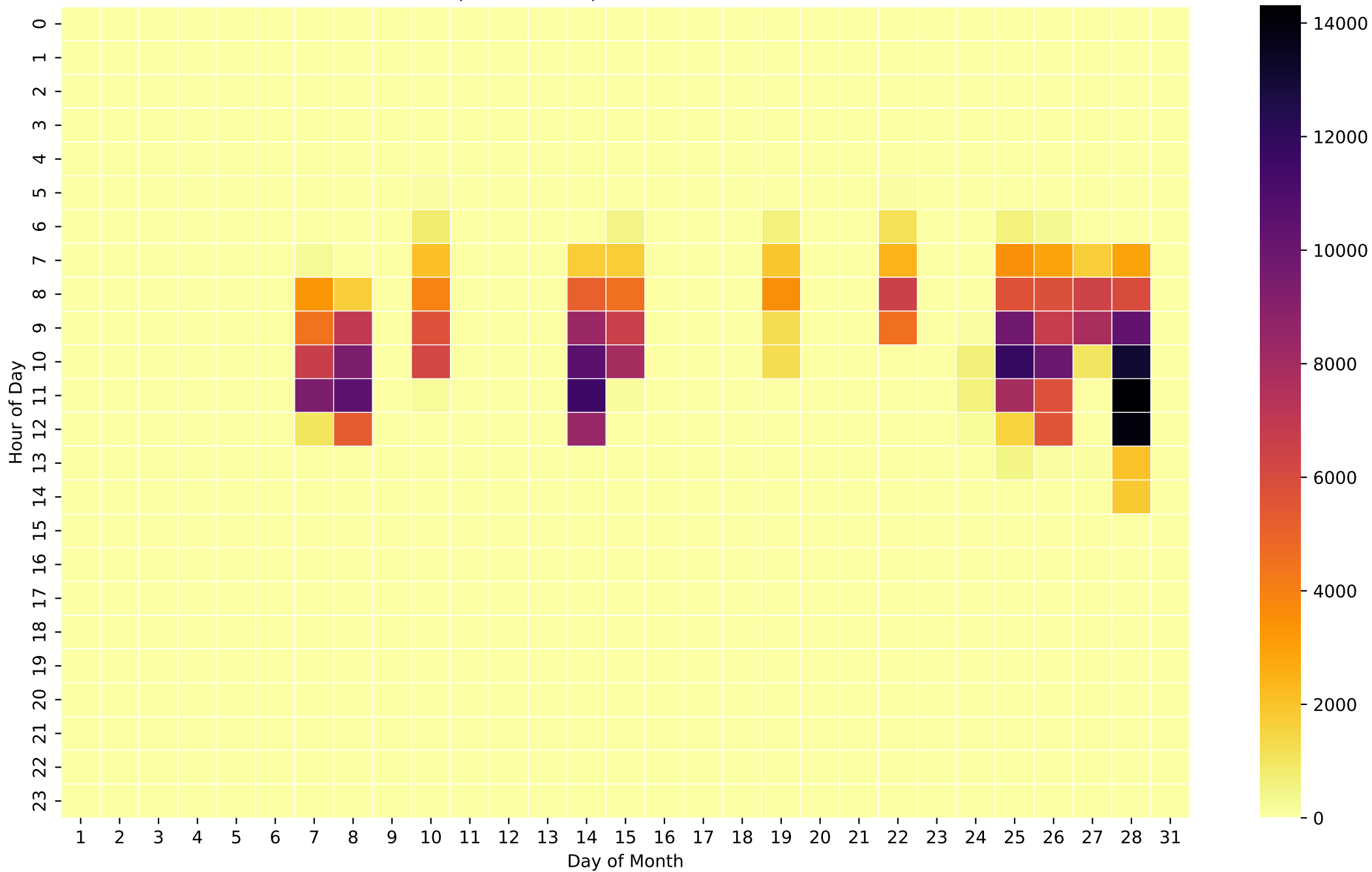
Grid Export Heatmap (Wh/Hour) - 12kWh - Feb
