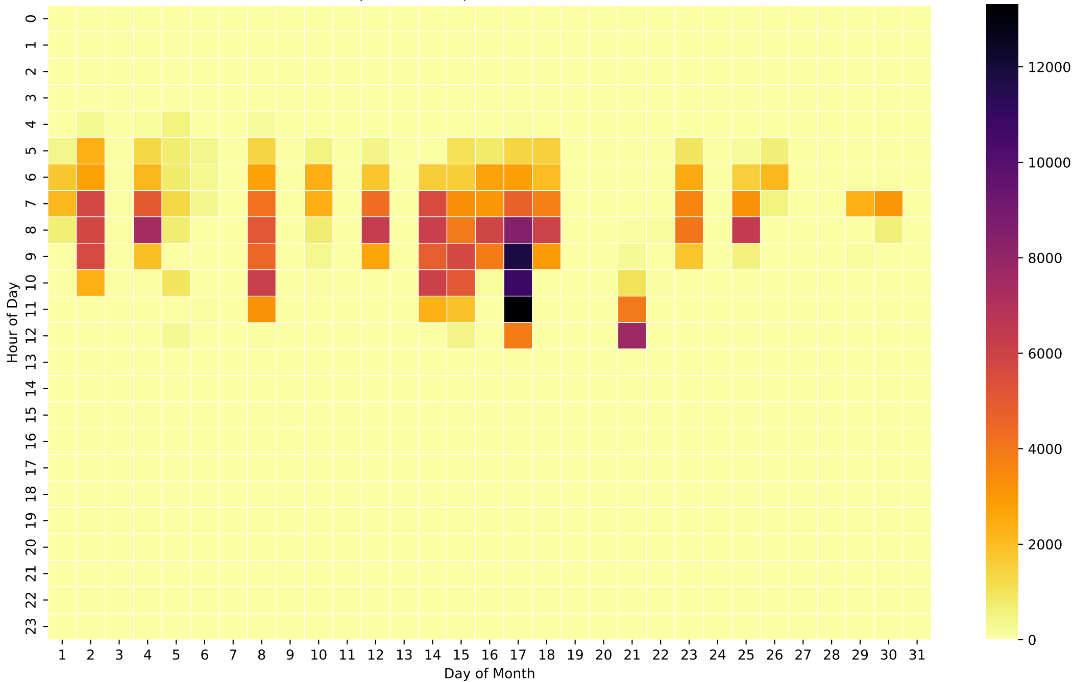
Grid Export Heatmap (Wh/Hour) - 12kWh - Oct
