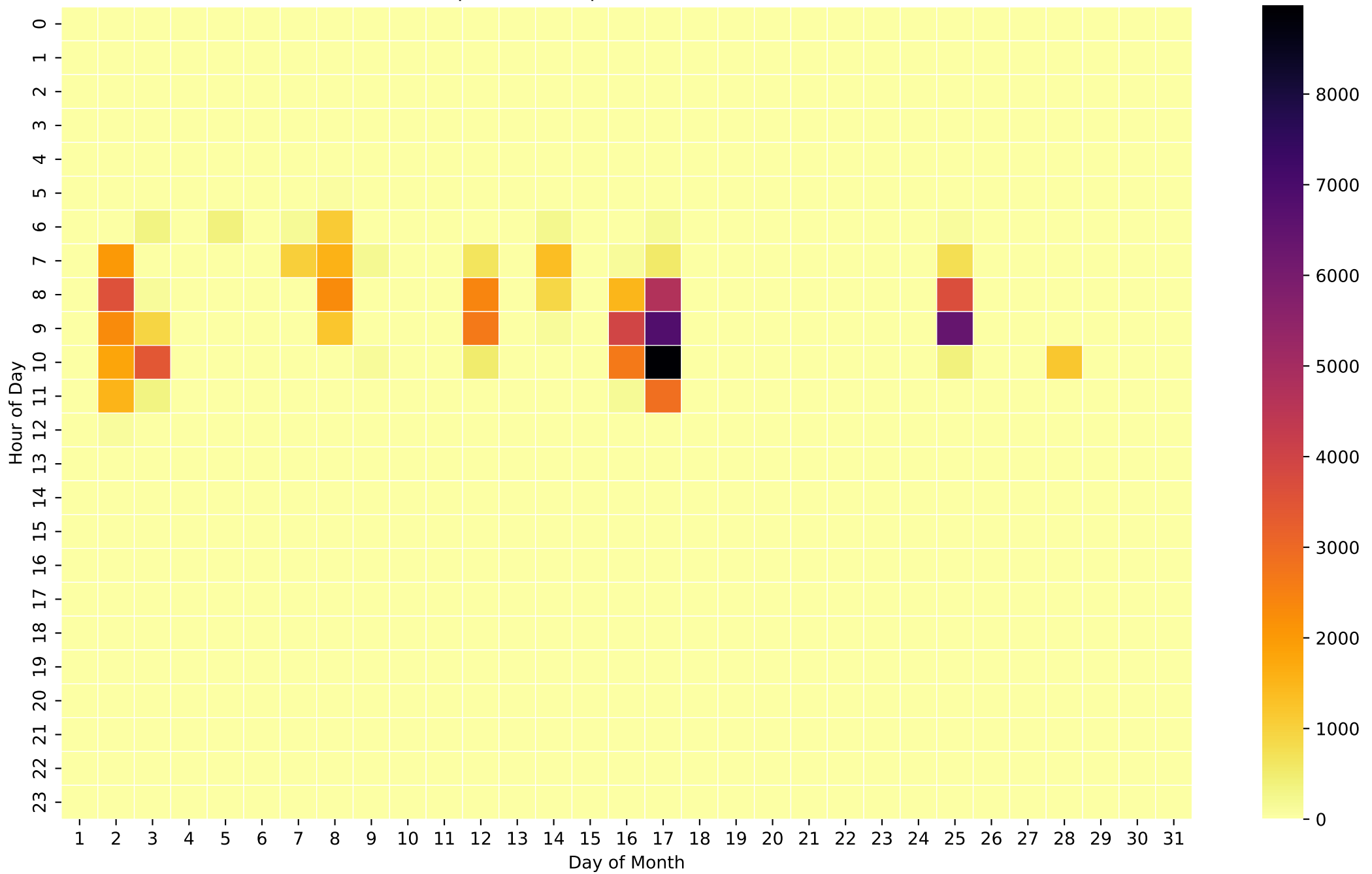
Grid Export Heatmap (Wh/Hour) - 12kWh - Nov
