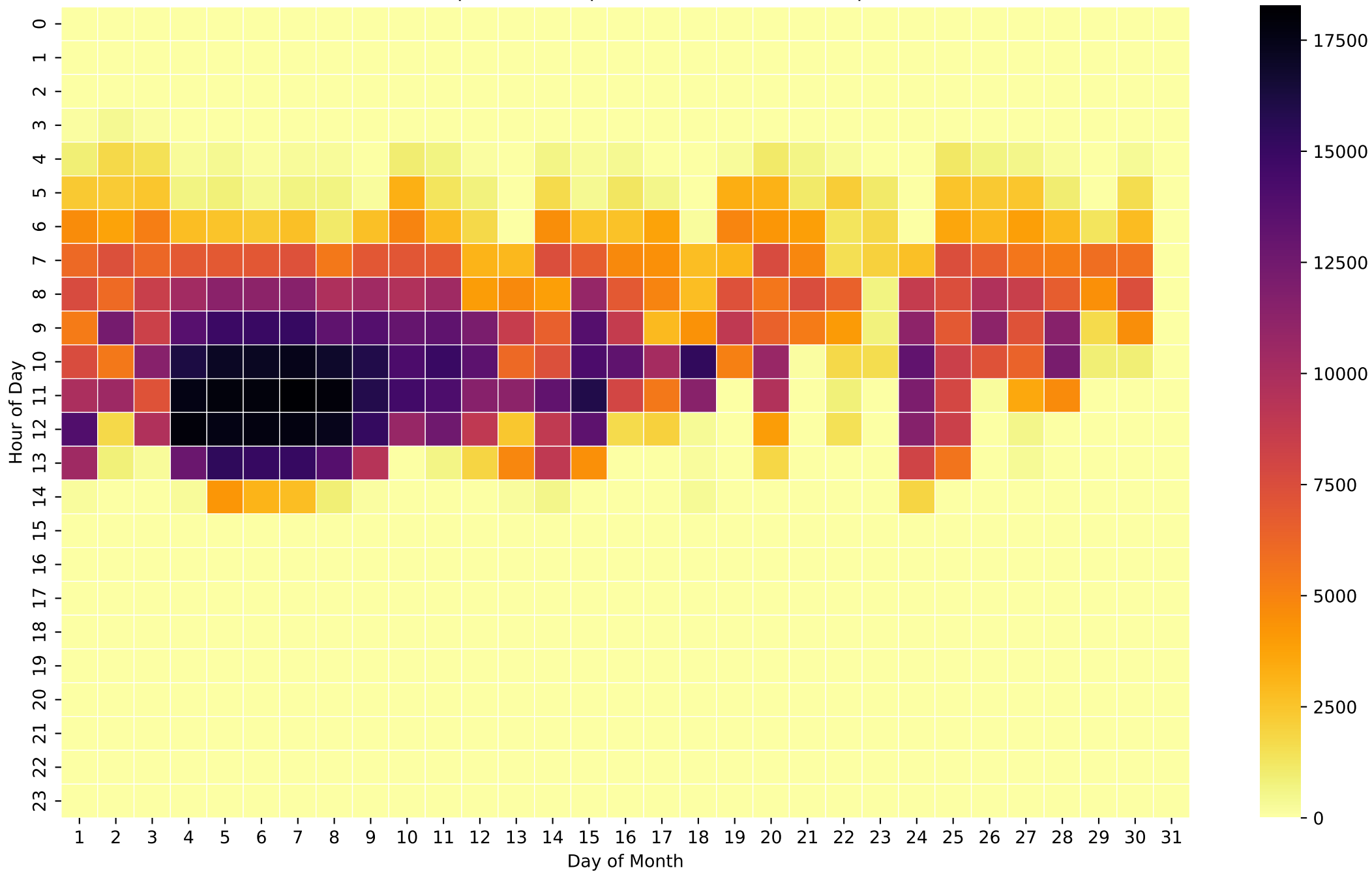
Grid Export Heatmap (Wh/Hour) - 12kWh - Sep
