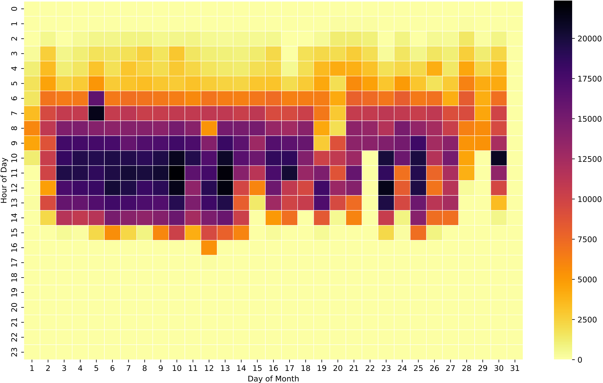
Grid Export Heatmap (Wh/Hour) - 12kWh - Jun
