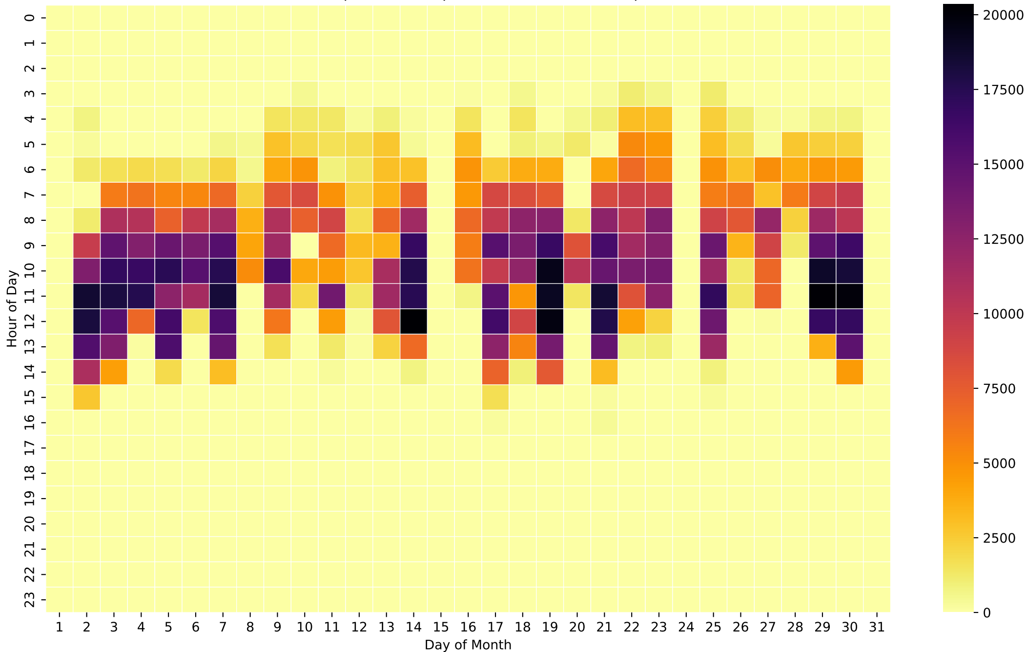
Grid Export Heatmap (Wh/Hour) - 12kWh - Apr
