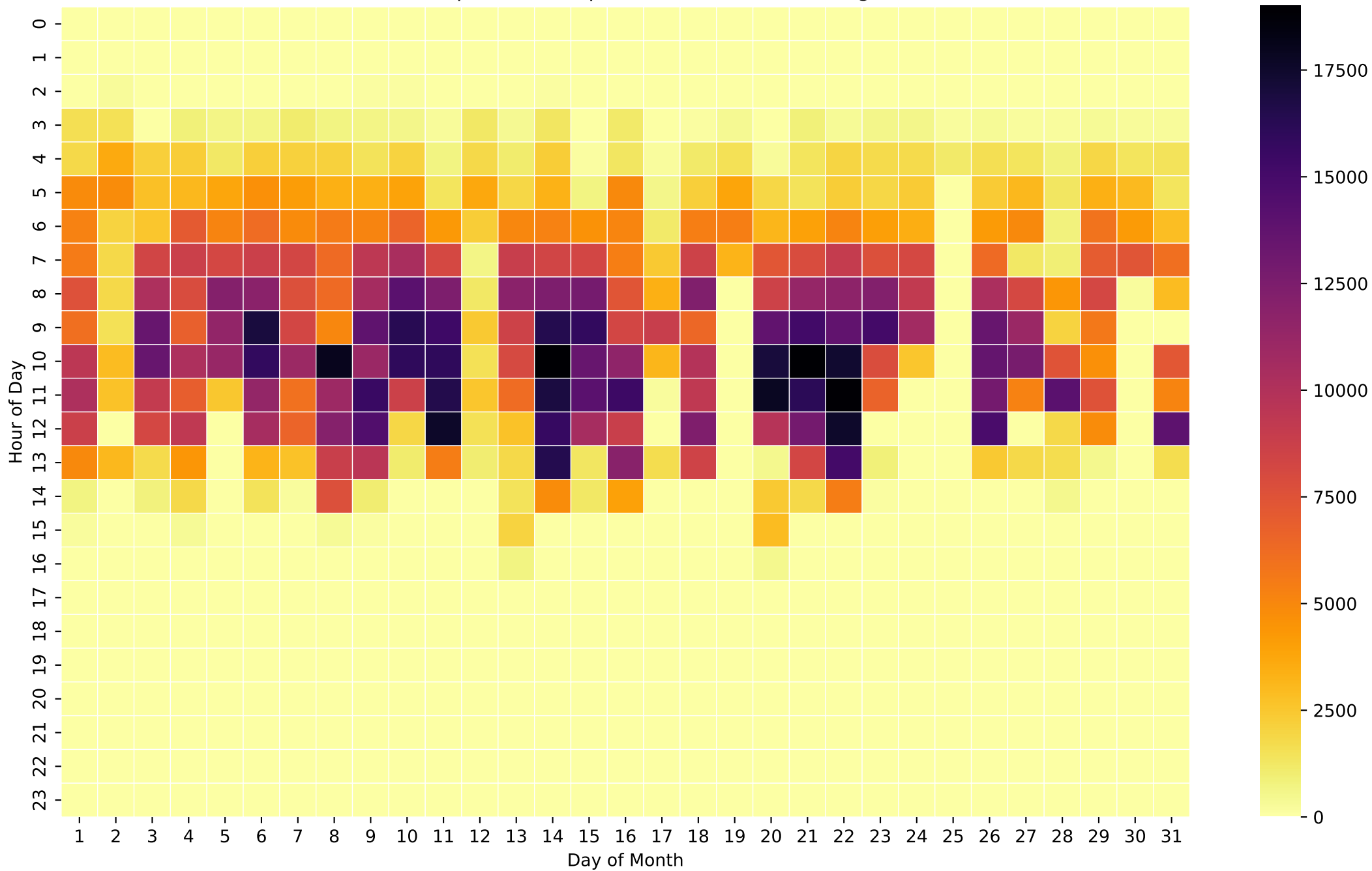
Grid Export Heatmap (Wh/Hour) - 12kWh - Aug
