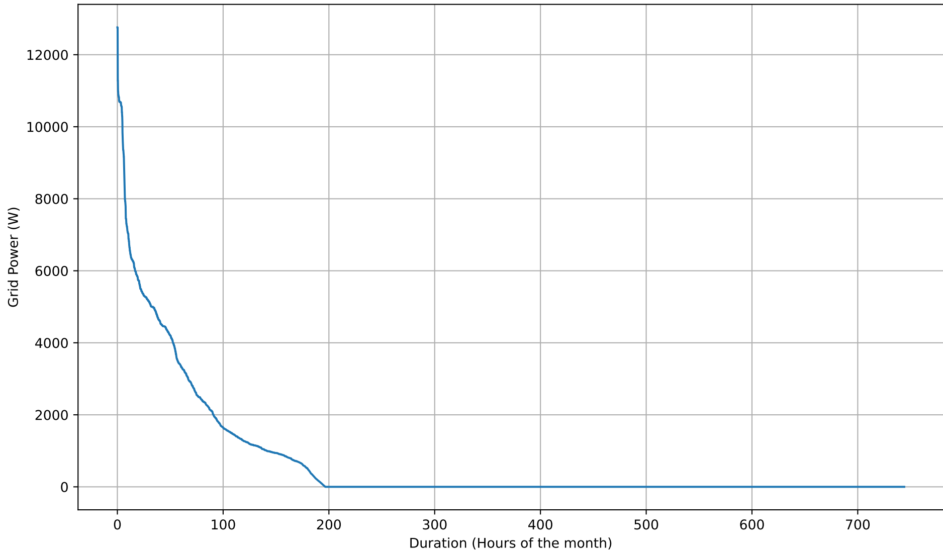
Grid Import Duration Curve - 12kWh - May
