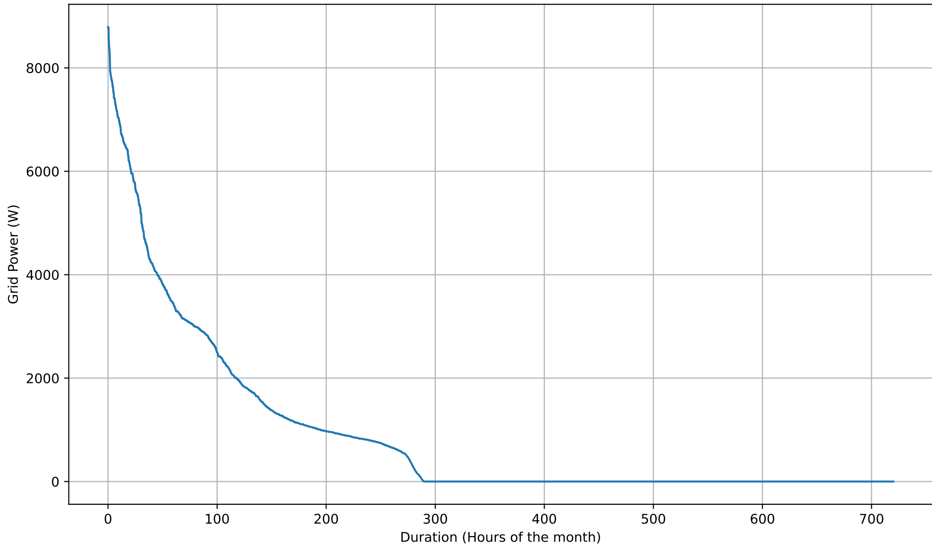
Grid Import Duration Curve - 12kWh - Apr
