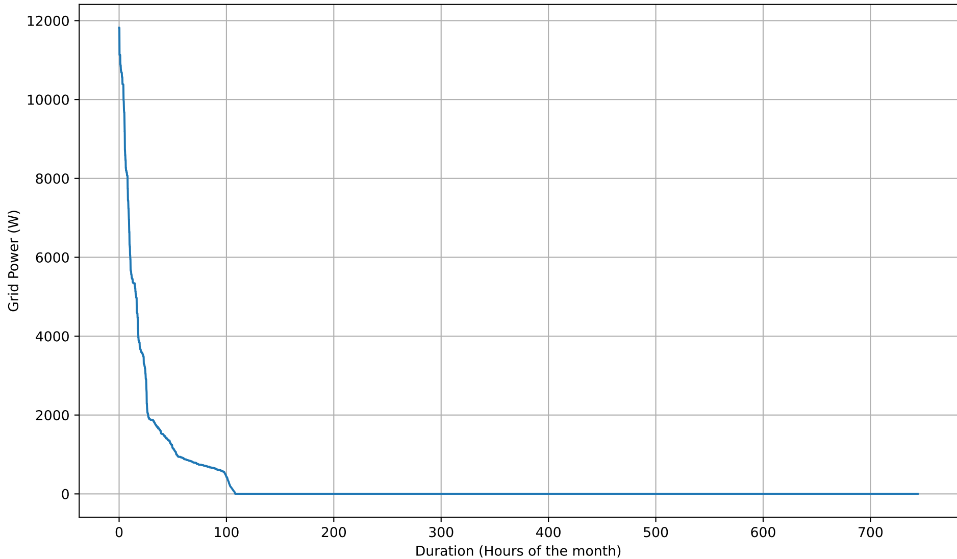
Grid Import Duration Curve - 12kWh - Jul
