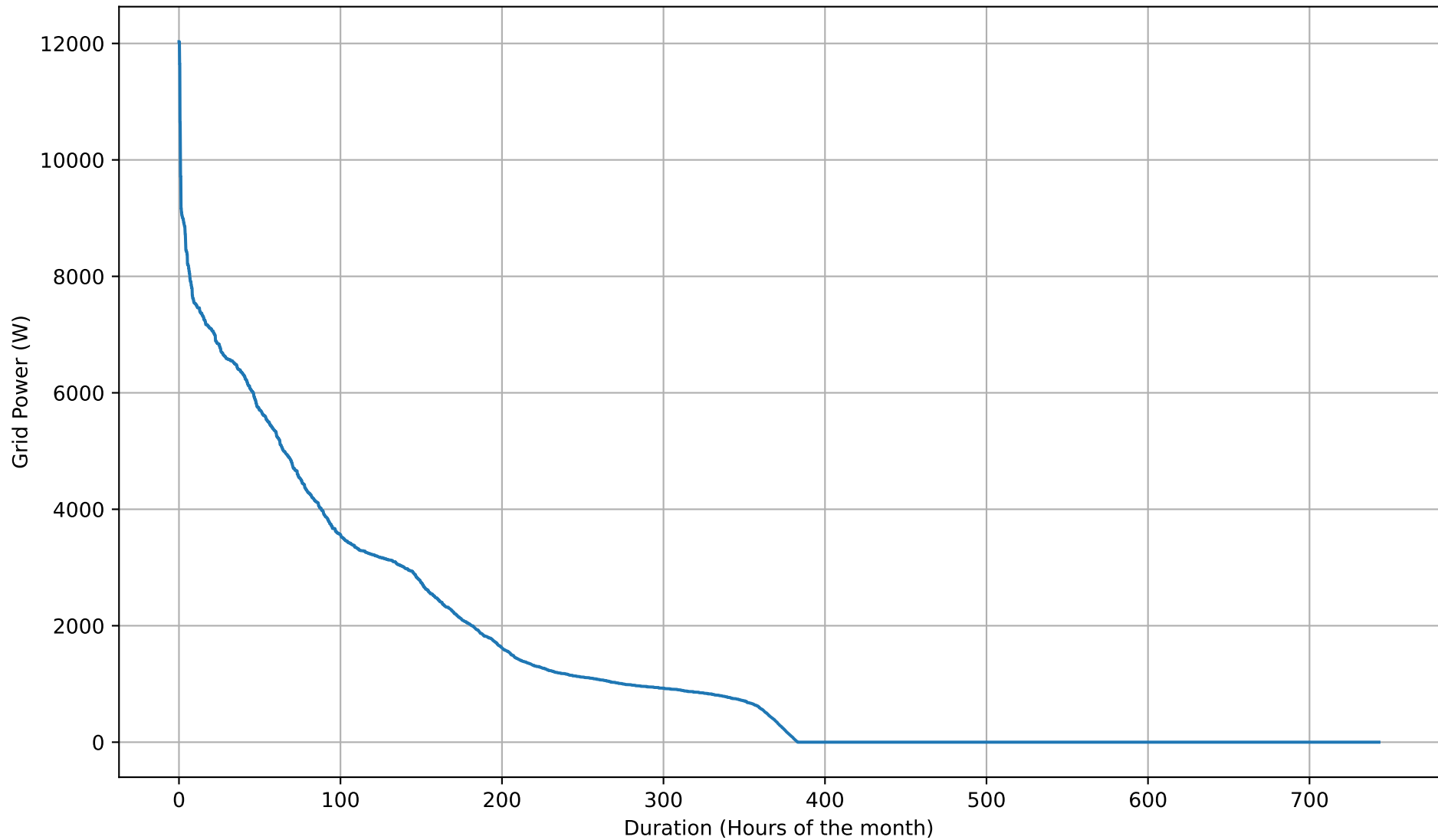
Grid Import Duration Curve - 12kWh - Mar
