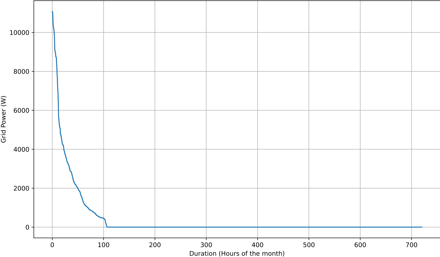
Grid Import Duration Curve - 12kWh - Jun
