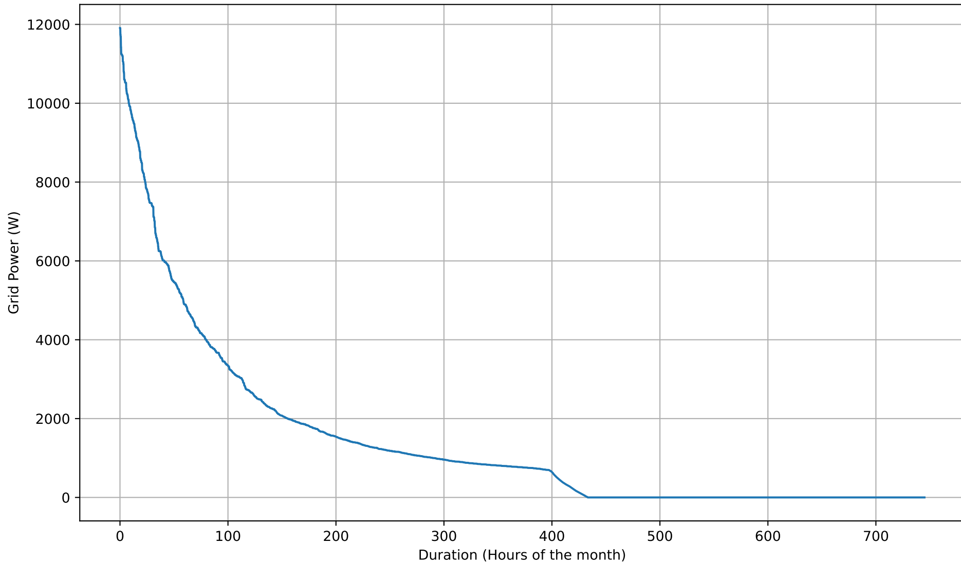
Grid Import Duration Curve - 12kWh - Oct
