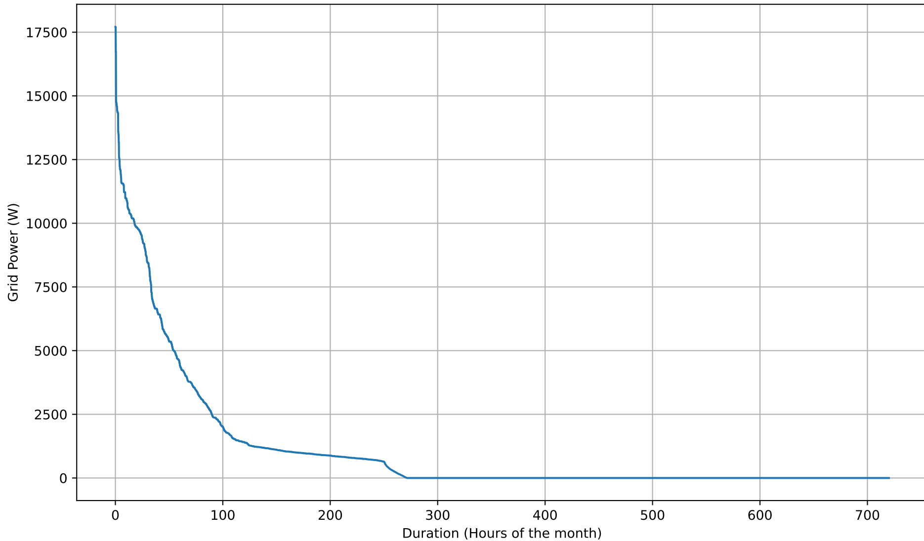
Grid Import Duration Curve - 12kWh - Sep
