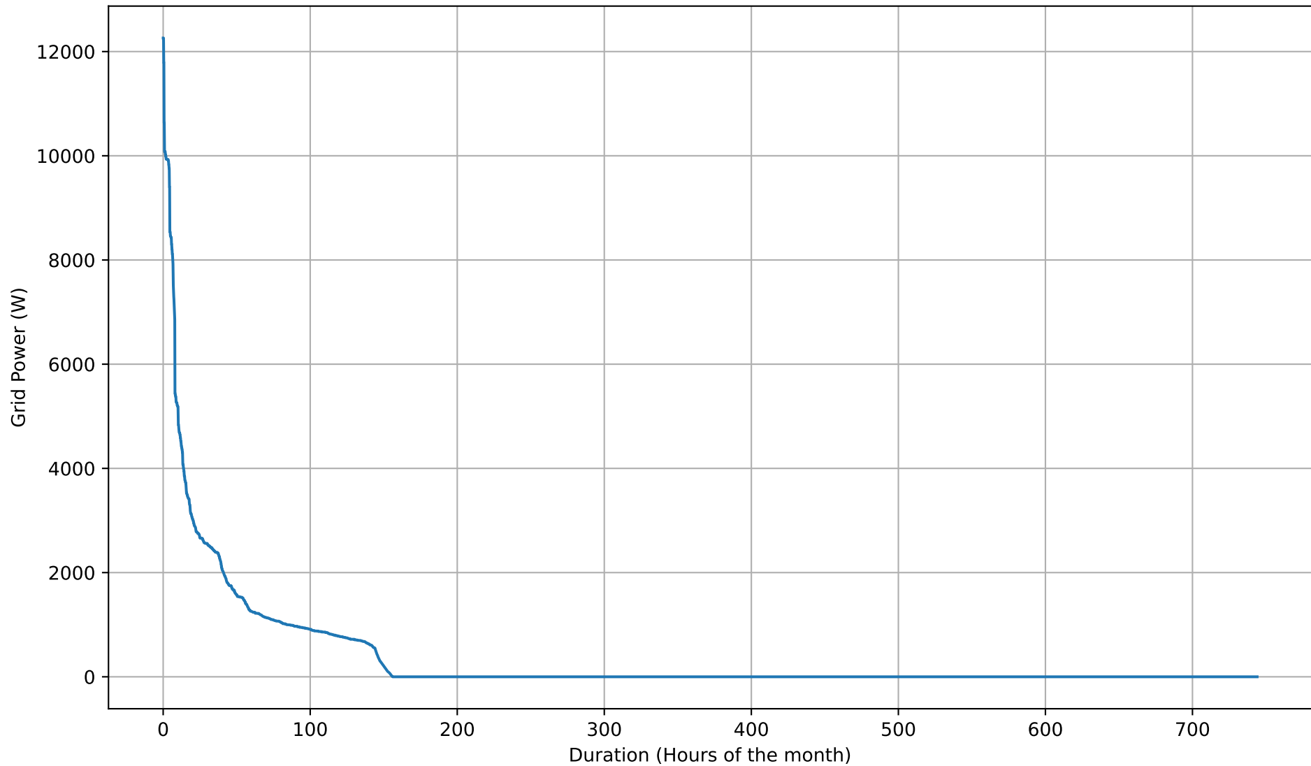
Grid Import Duration Curve - 12kWh - Aug
