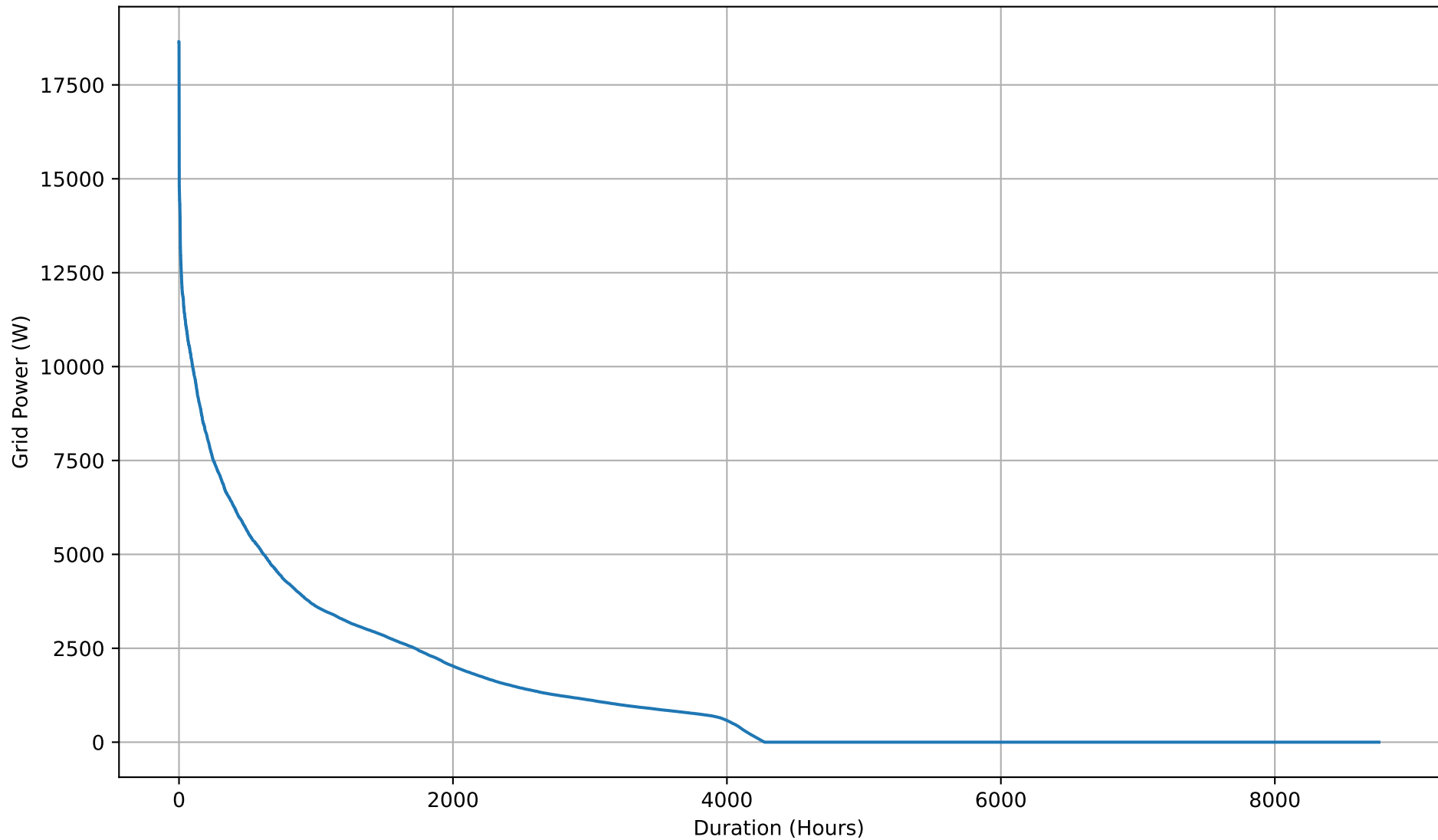
Yearly Grid Import Duration Curve - 12kWh
