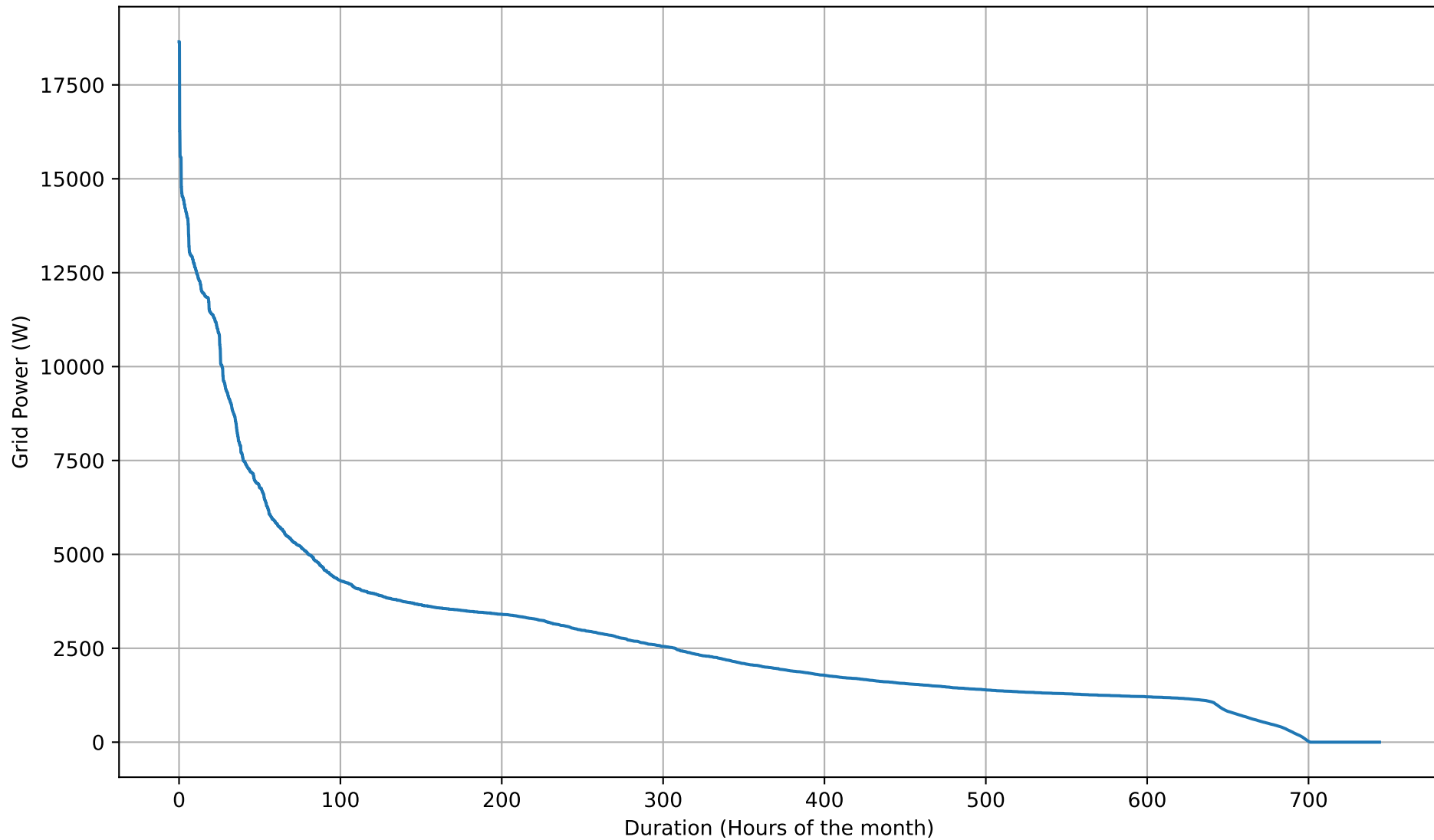
Grid Import Duration Curve - 12kWh - Dec
