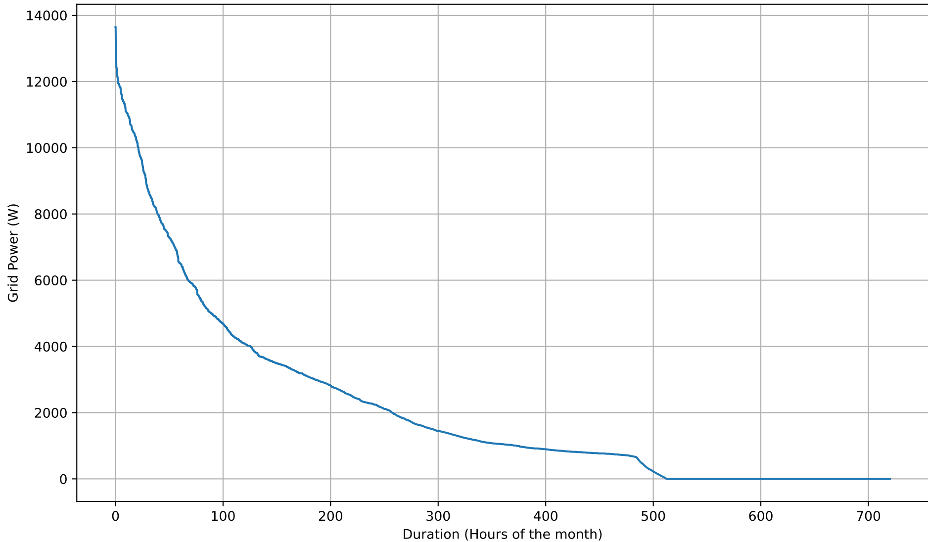
Grid Import Duration Curve - 12kWh - Nov
