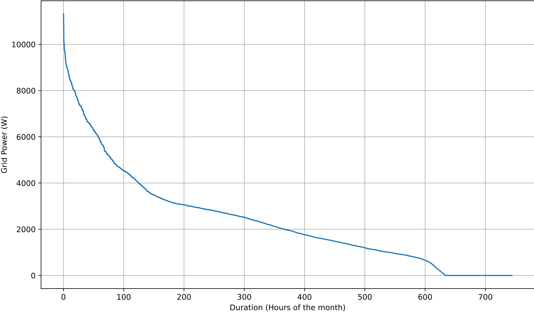
Grid Import Duration Curve - 12kWh - Jan
