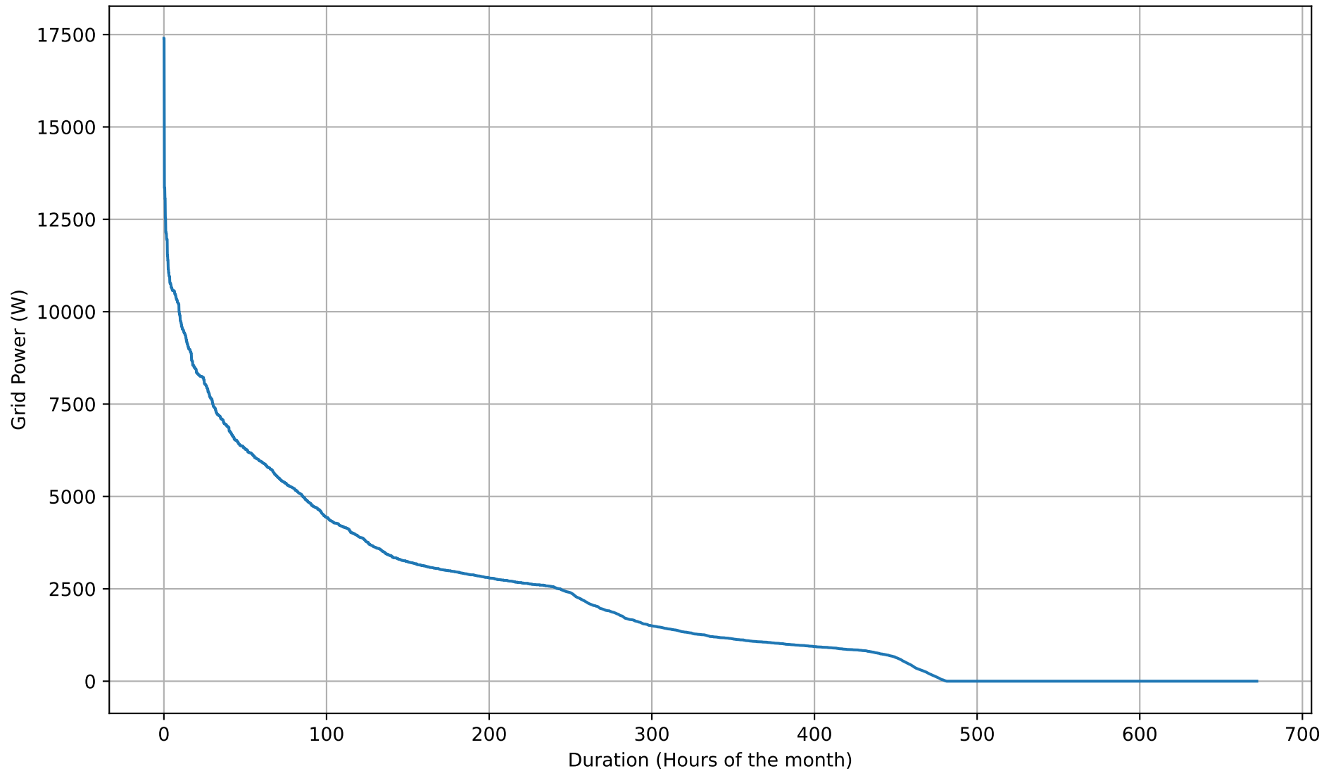
Grid Import Duration Curve - 12kWh - Feb
