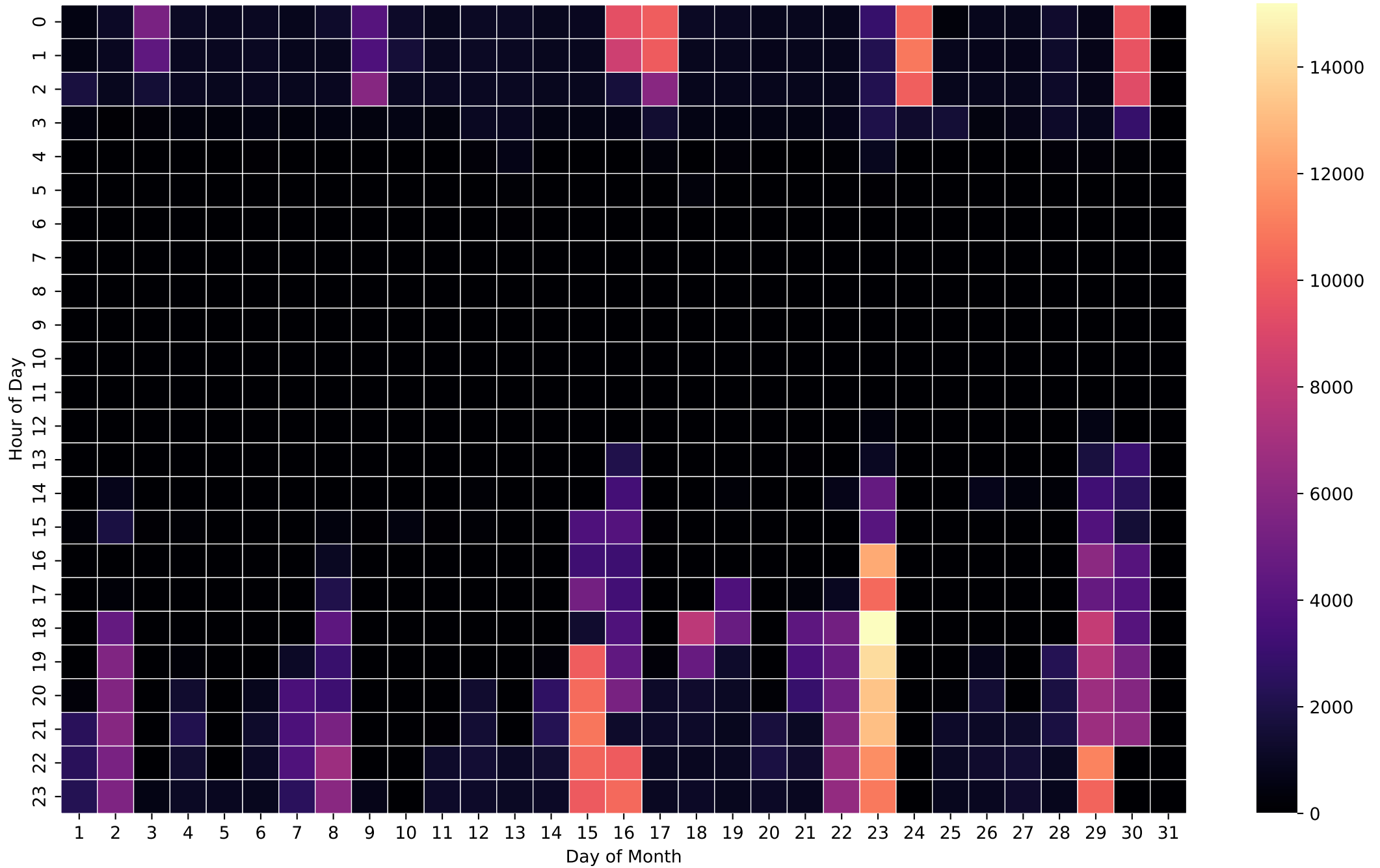
Grid Import Heatmap (Wh/Hour) - 12kWh - Sep
