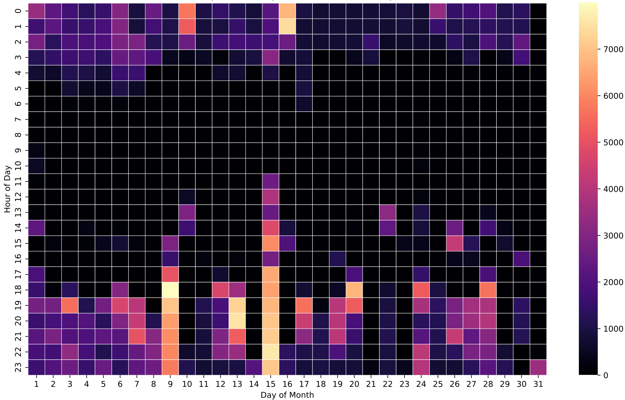
Grid Import Heatmap (Wh/Hour) - 12kWh - Apr
