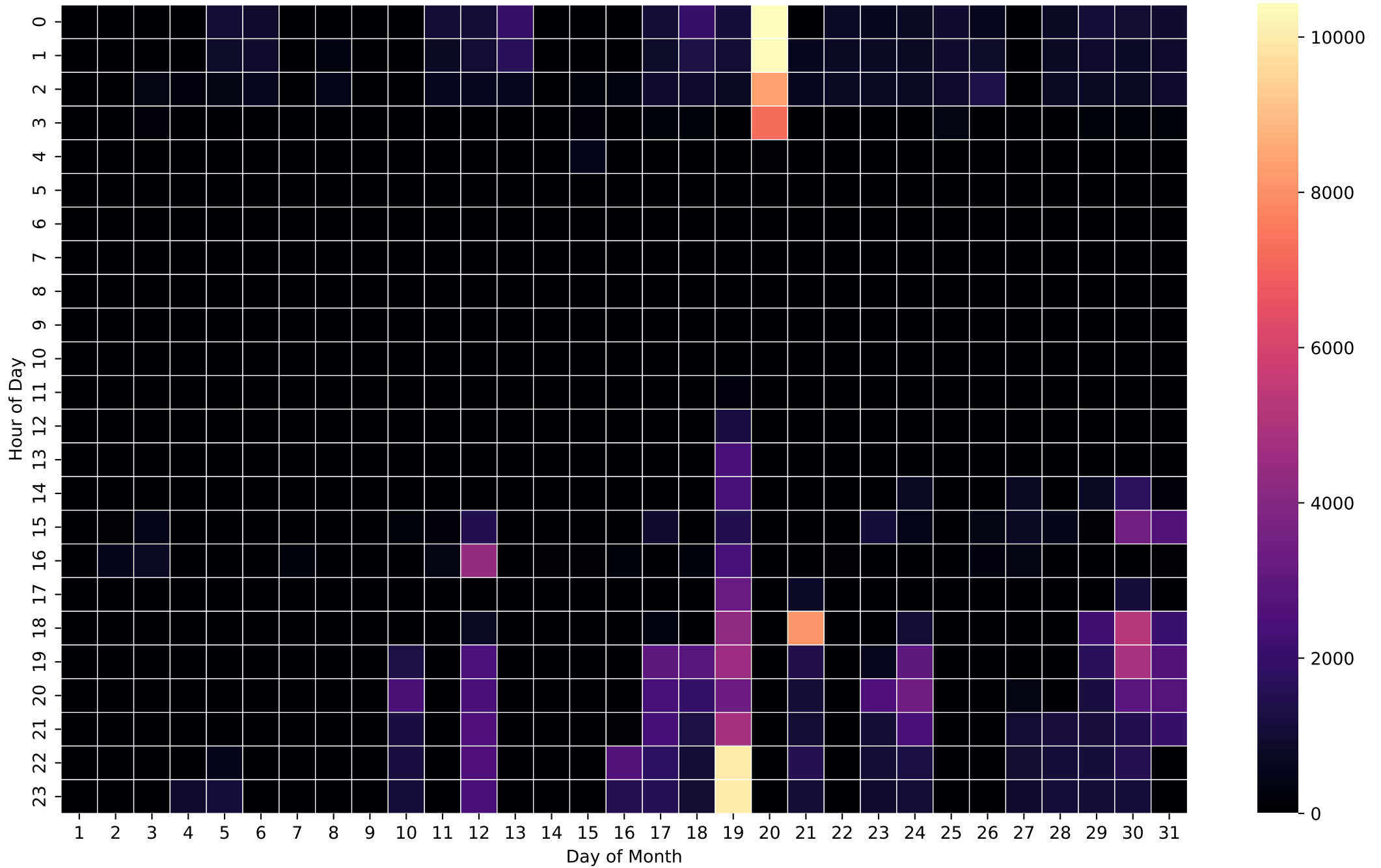
Grid Import Heatmap (Wh/Hour) - 12kWh - Aug
