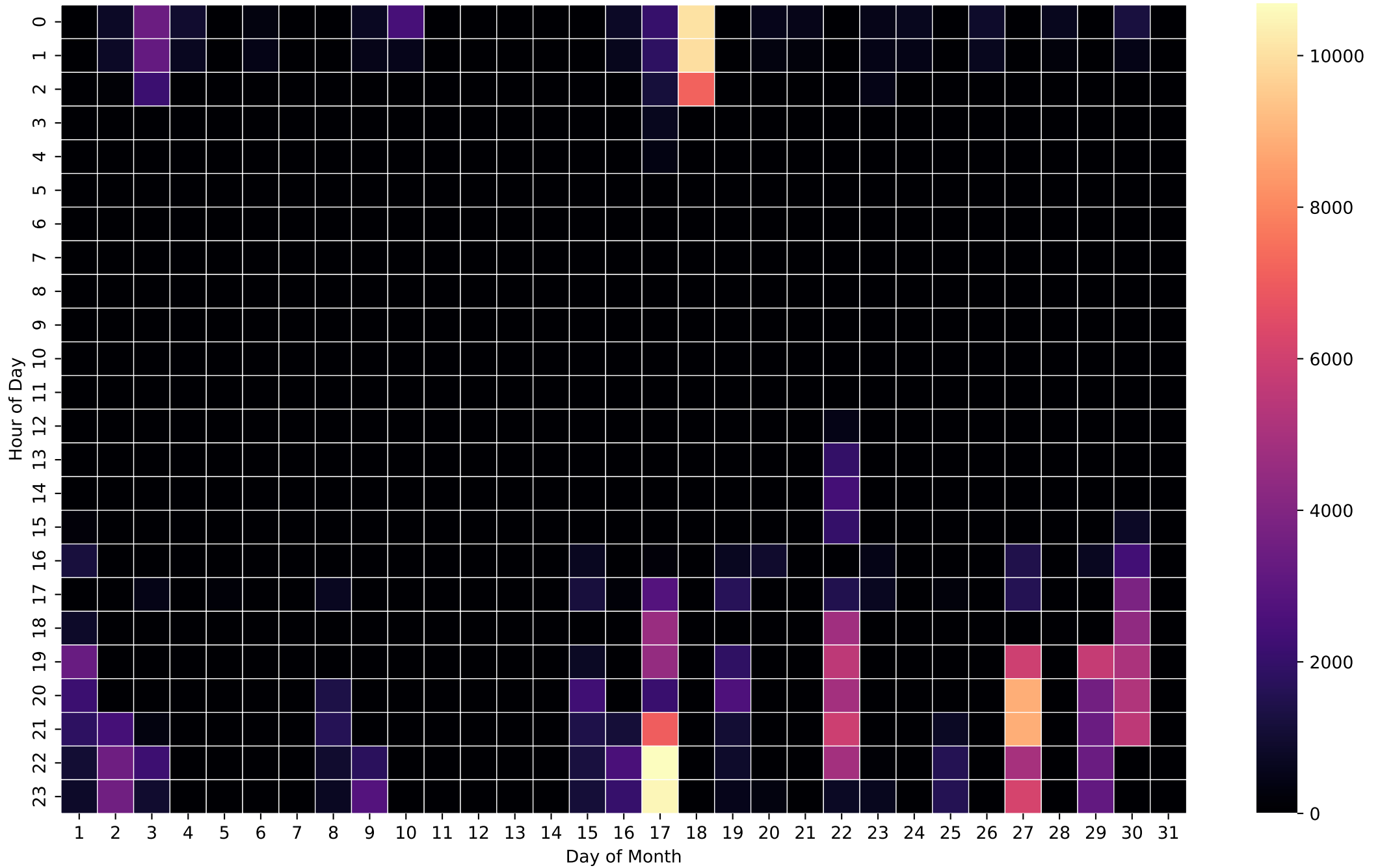
Grid Import Heatmap (Wh/Hour) - 12kWh - Jun
