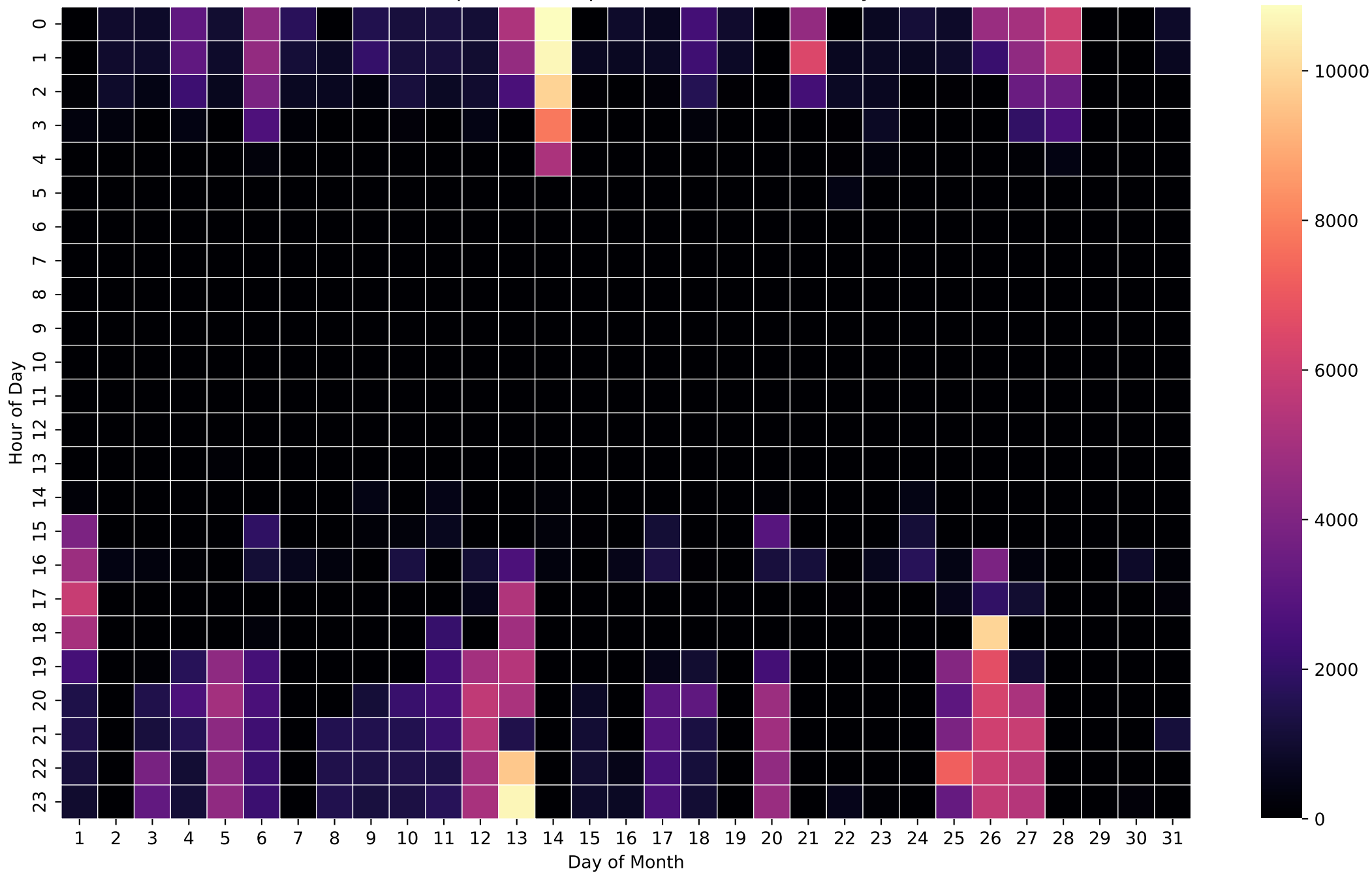
Grid Import Heatmap (Wh/Hour) - 12kWh - May
