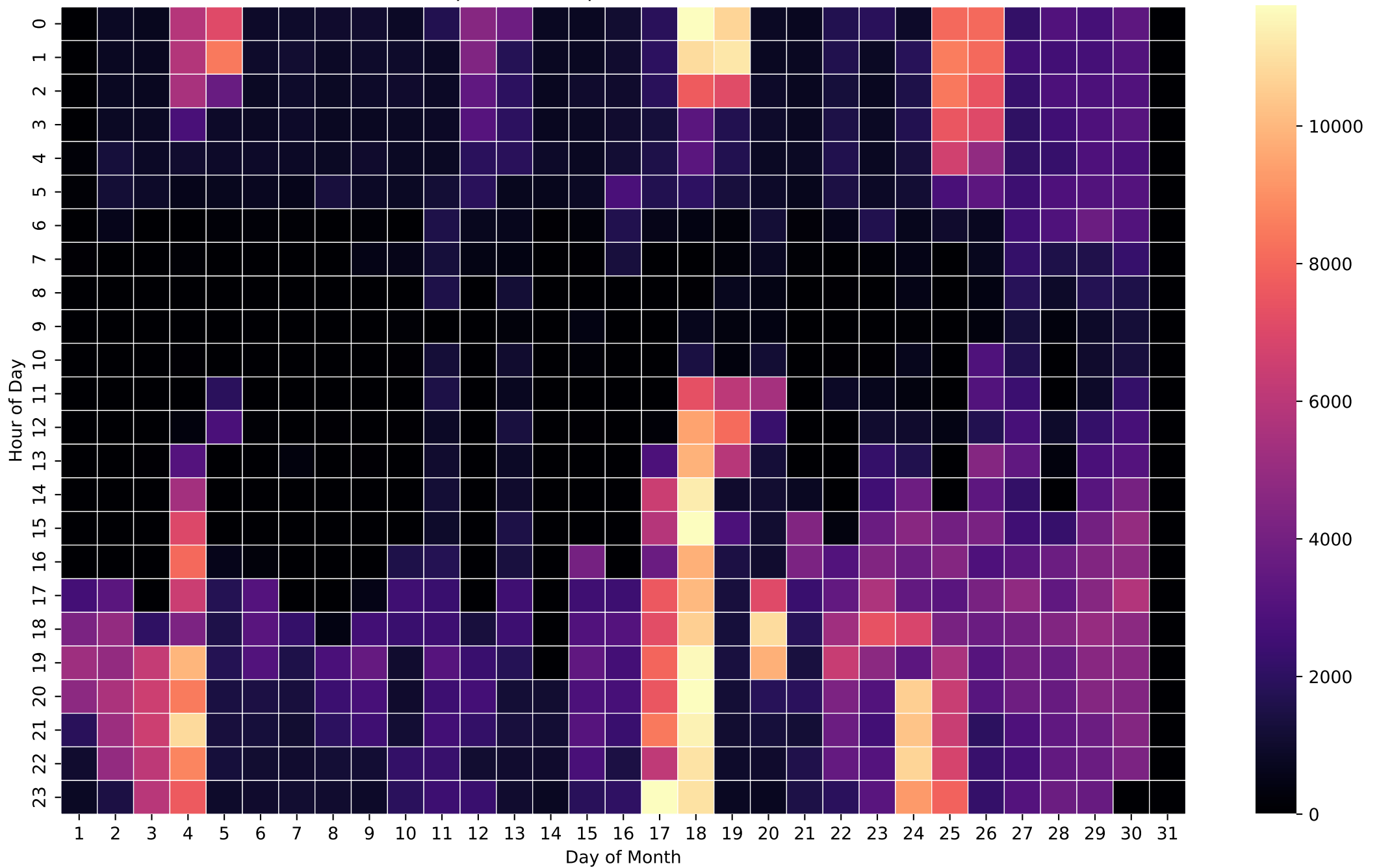
Grid Import Heatmap (Wh/Hour) - 12kWh - Nov
