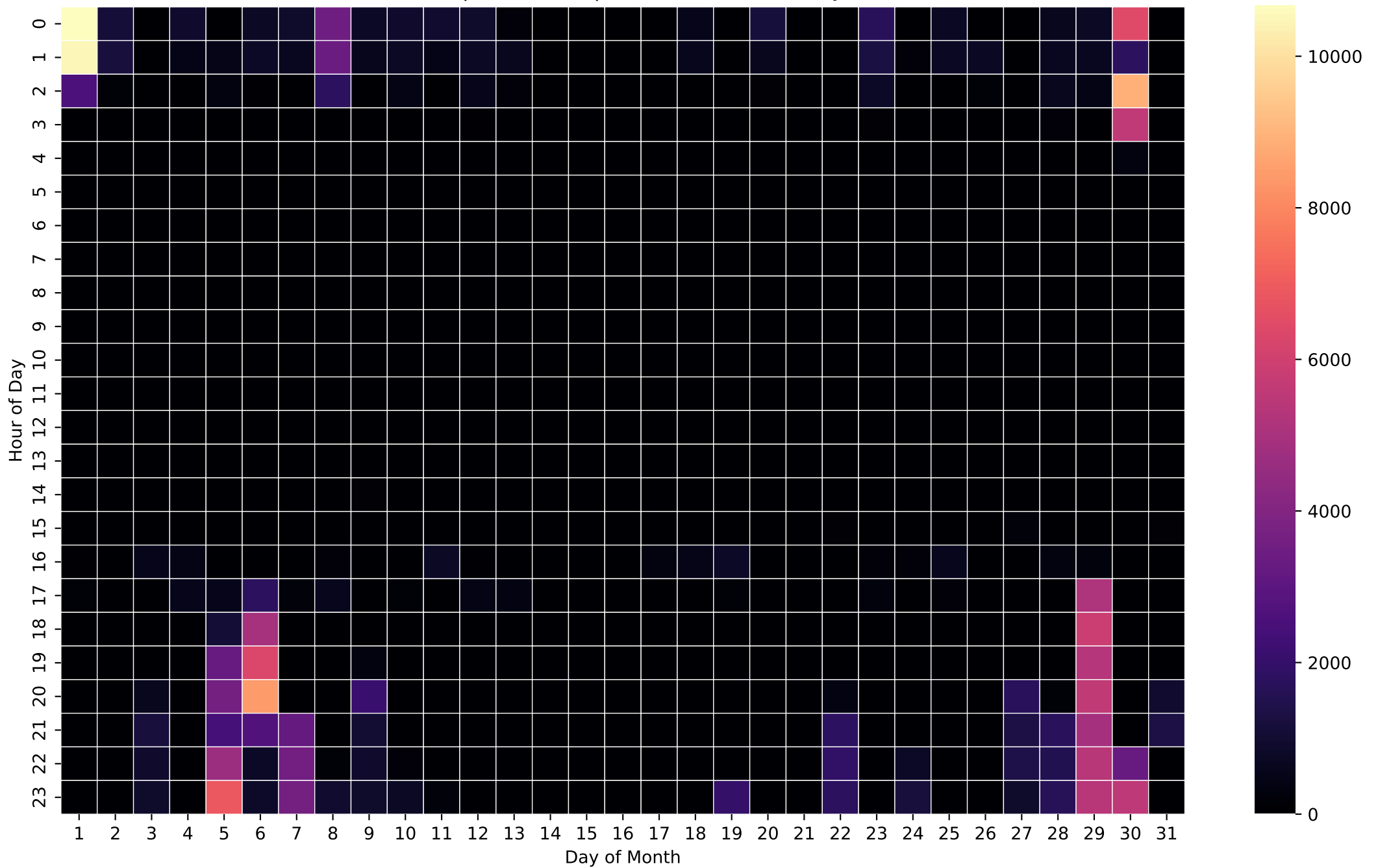
Grid Import Heatmap (Wh/Hour) - 12kWh - Jul
