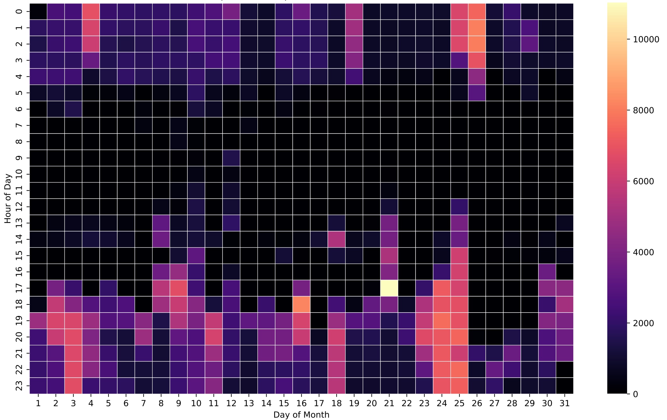
Grid Import Heatmap (Wh/Hour) - 12kWh - Mar
