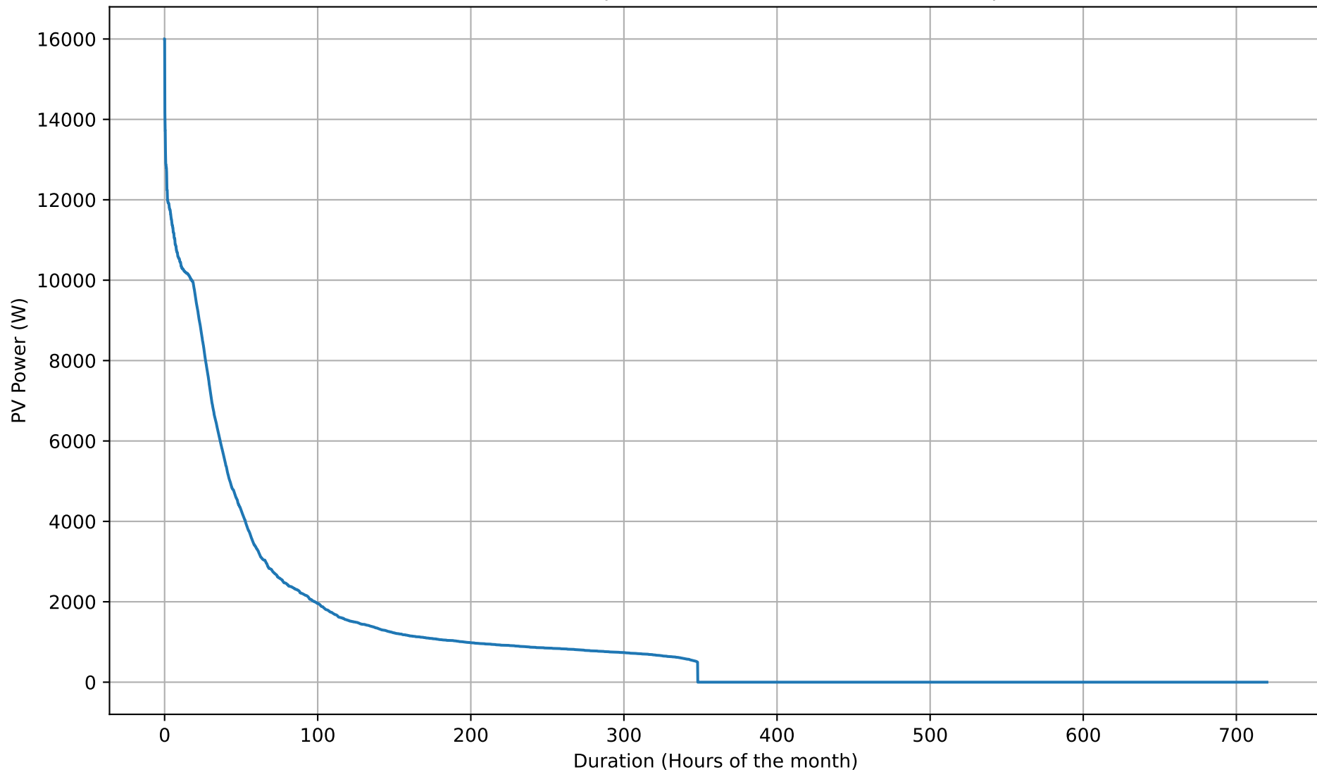
PV Self-Consumption Duration Curve - 12kWh - Sep
