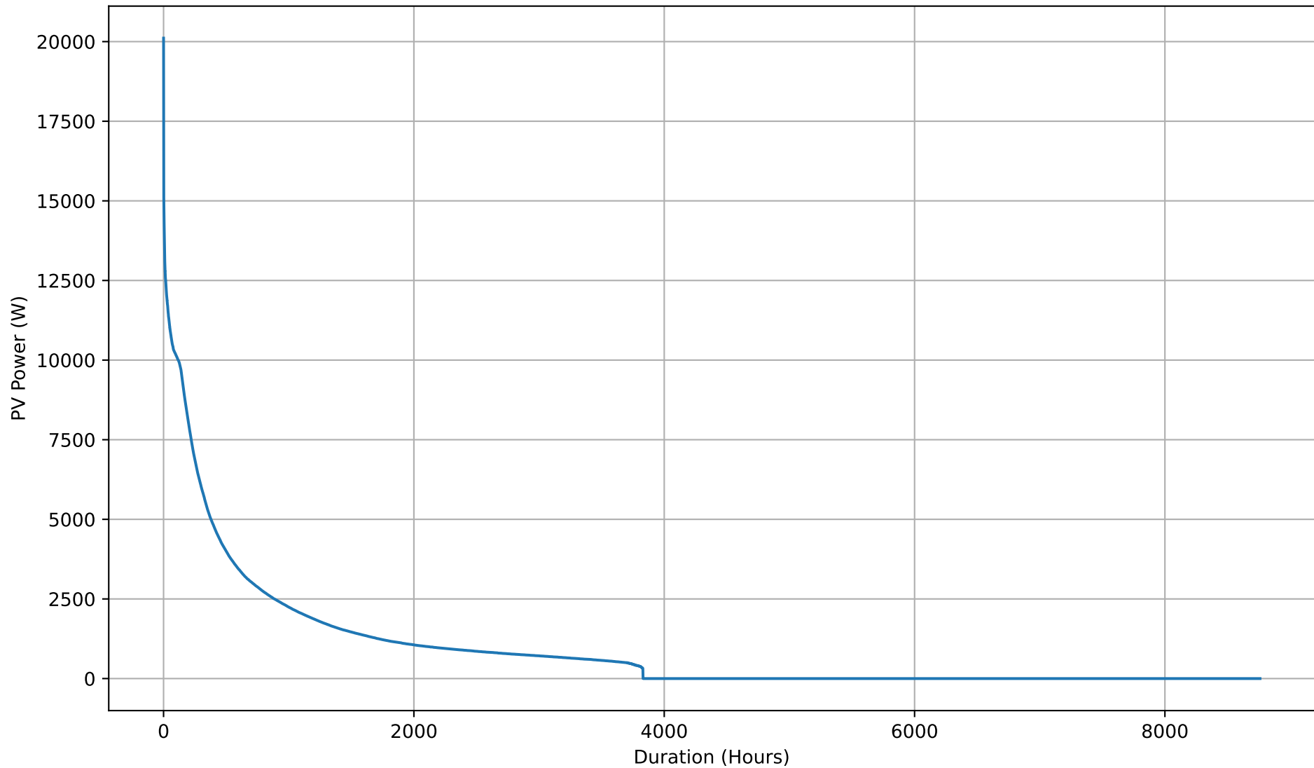
Yearly PV Self-Consumption Duration Curve - 12kWh
