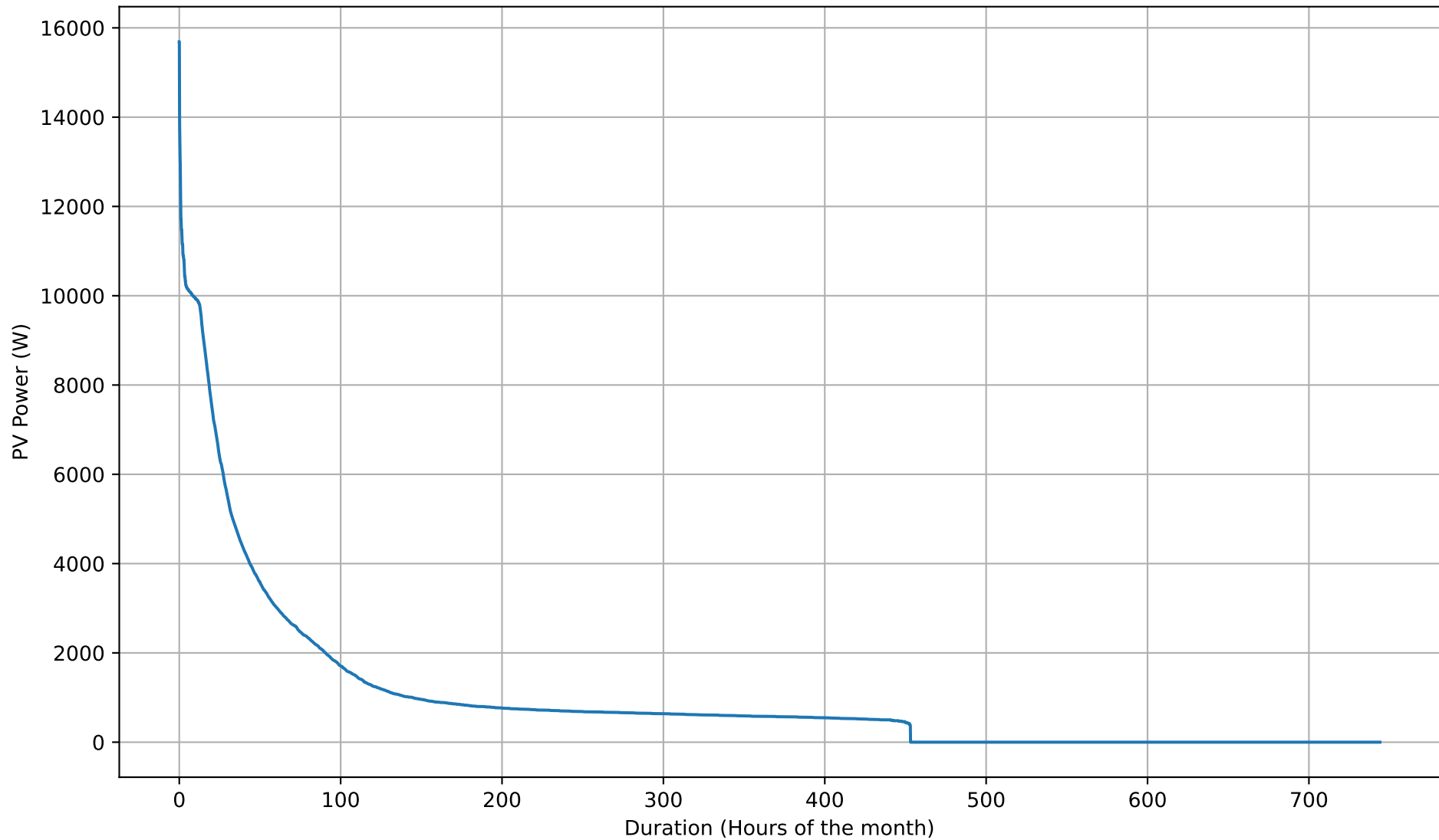
PV Self-Consumption Duration Curve - 12kWh - Jul
