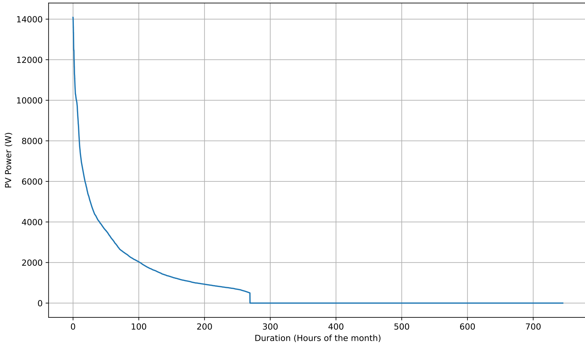
PV Self-Consumption Duration Curve - 12kWh - Oct
