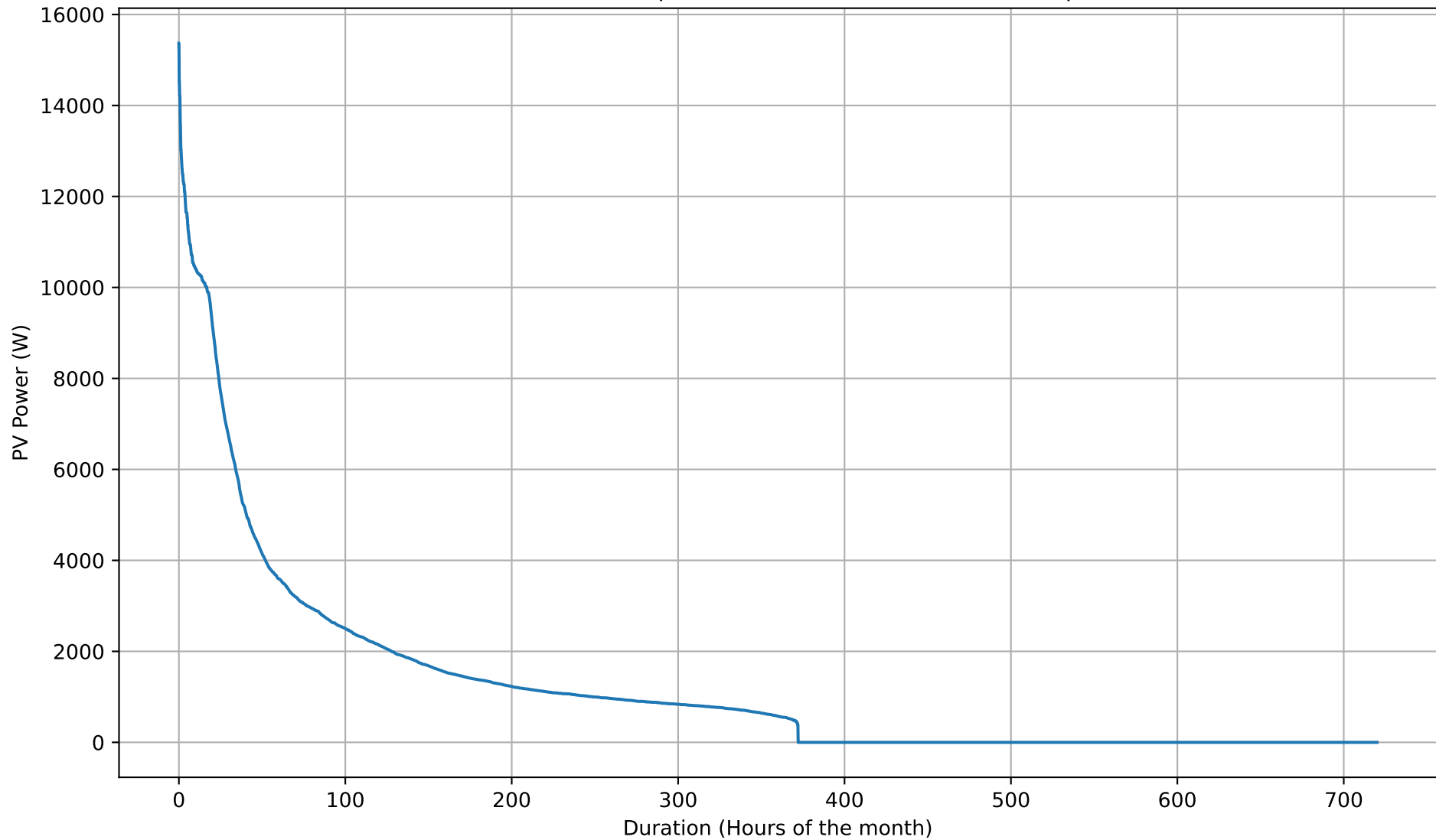
PV Self-Consumption Duration Curve - 12kWh - Apr
