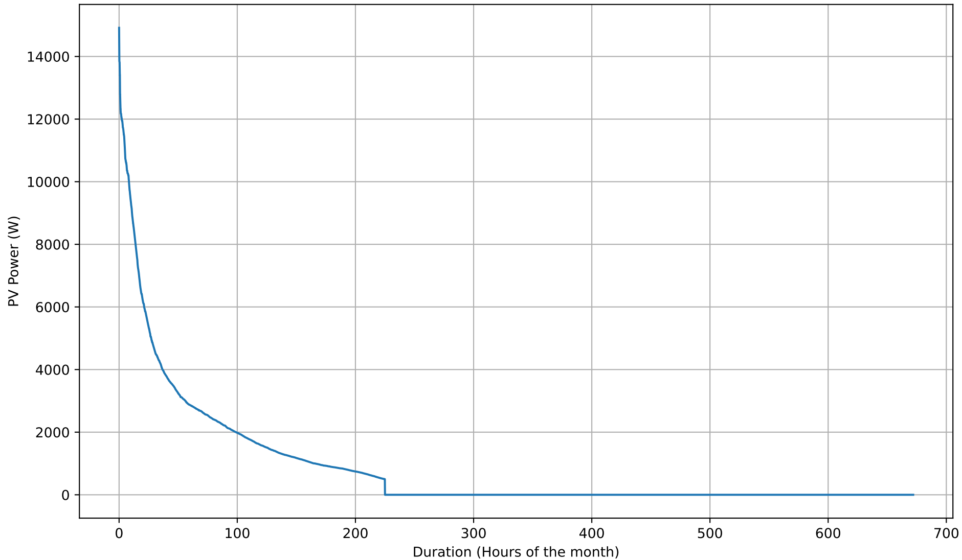
PV Self-Consumption Duration Curve - 12kWh - Feb
