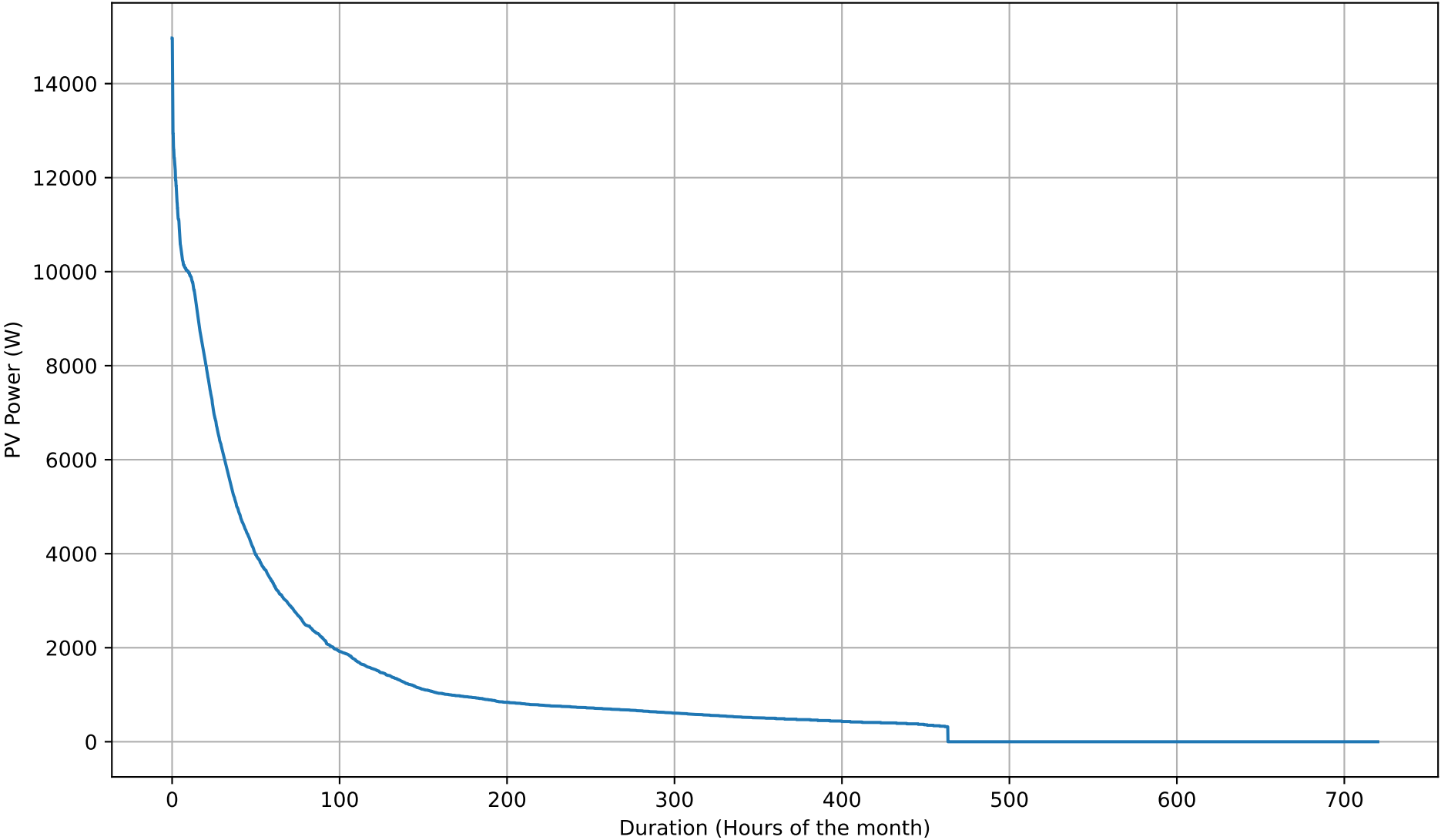
PV Self-Consumption Duration Curve - 12kWh - Jun
