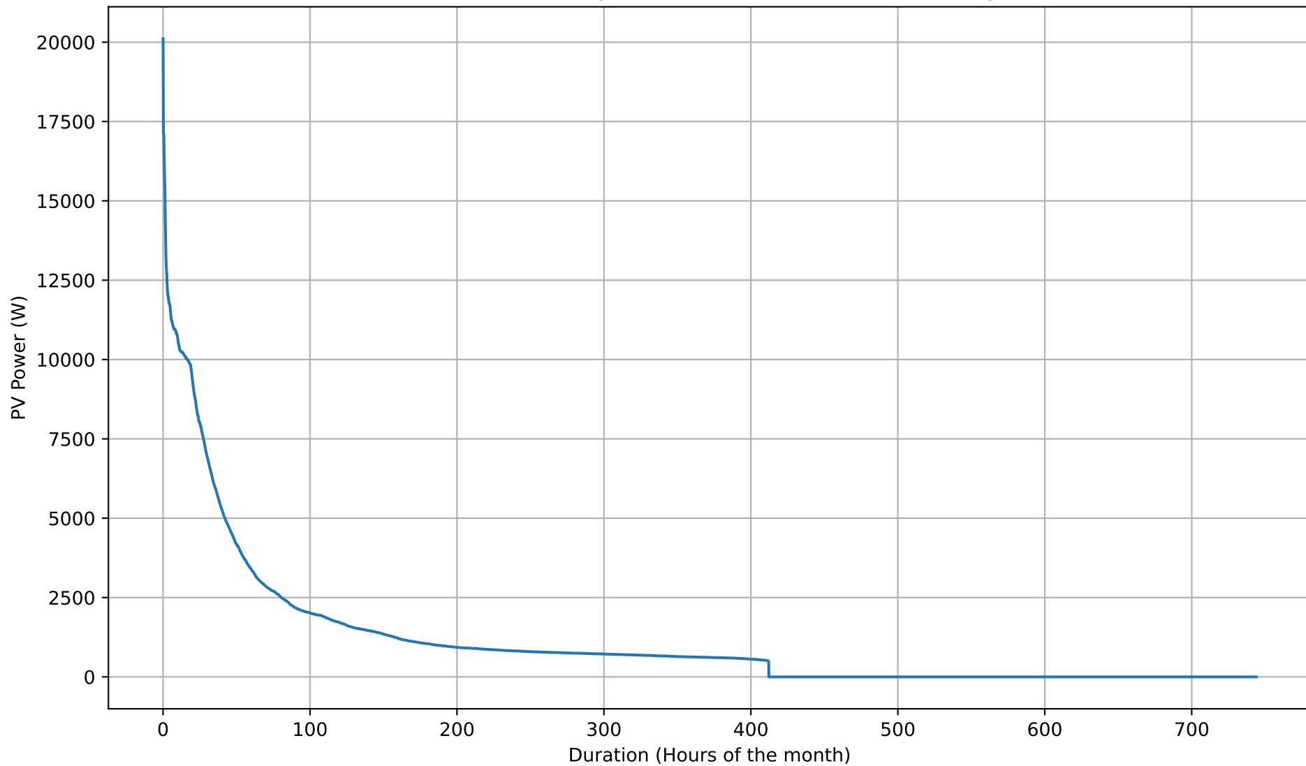
PV Self-Consumption Duration Curve - 12kWh - Aug
