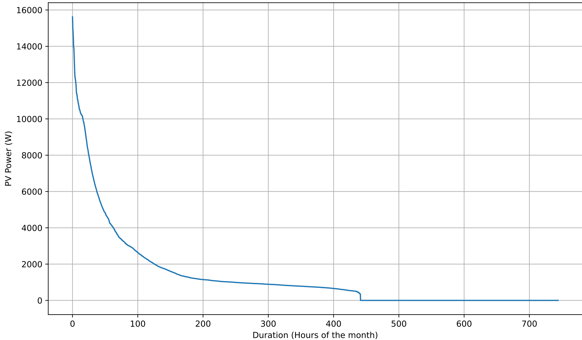
PV Self-Consumption Duration Curve - 12kWh - May
