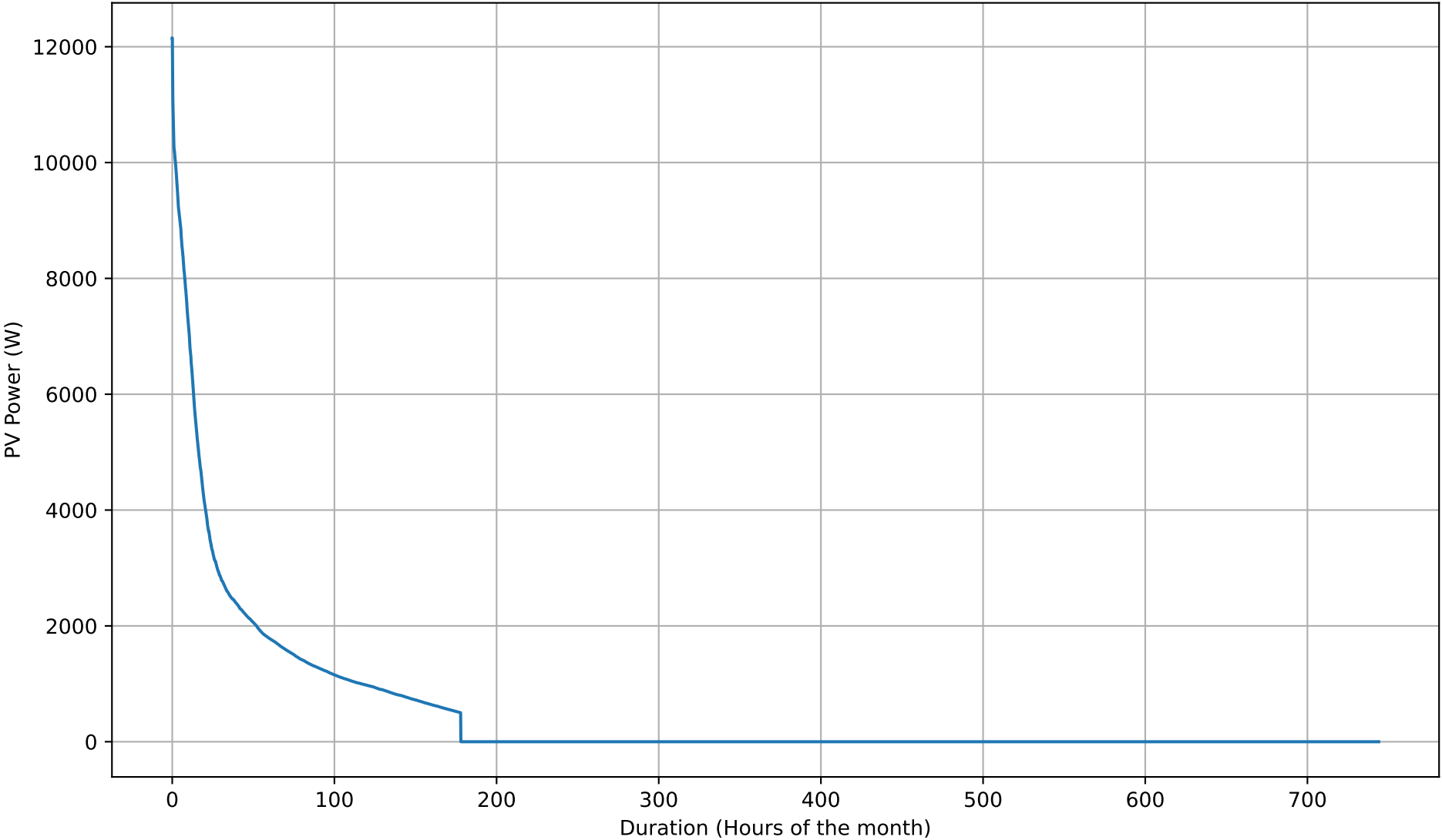
PV Self-Consumption Duration Curve - 12kWh - Jan
