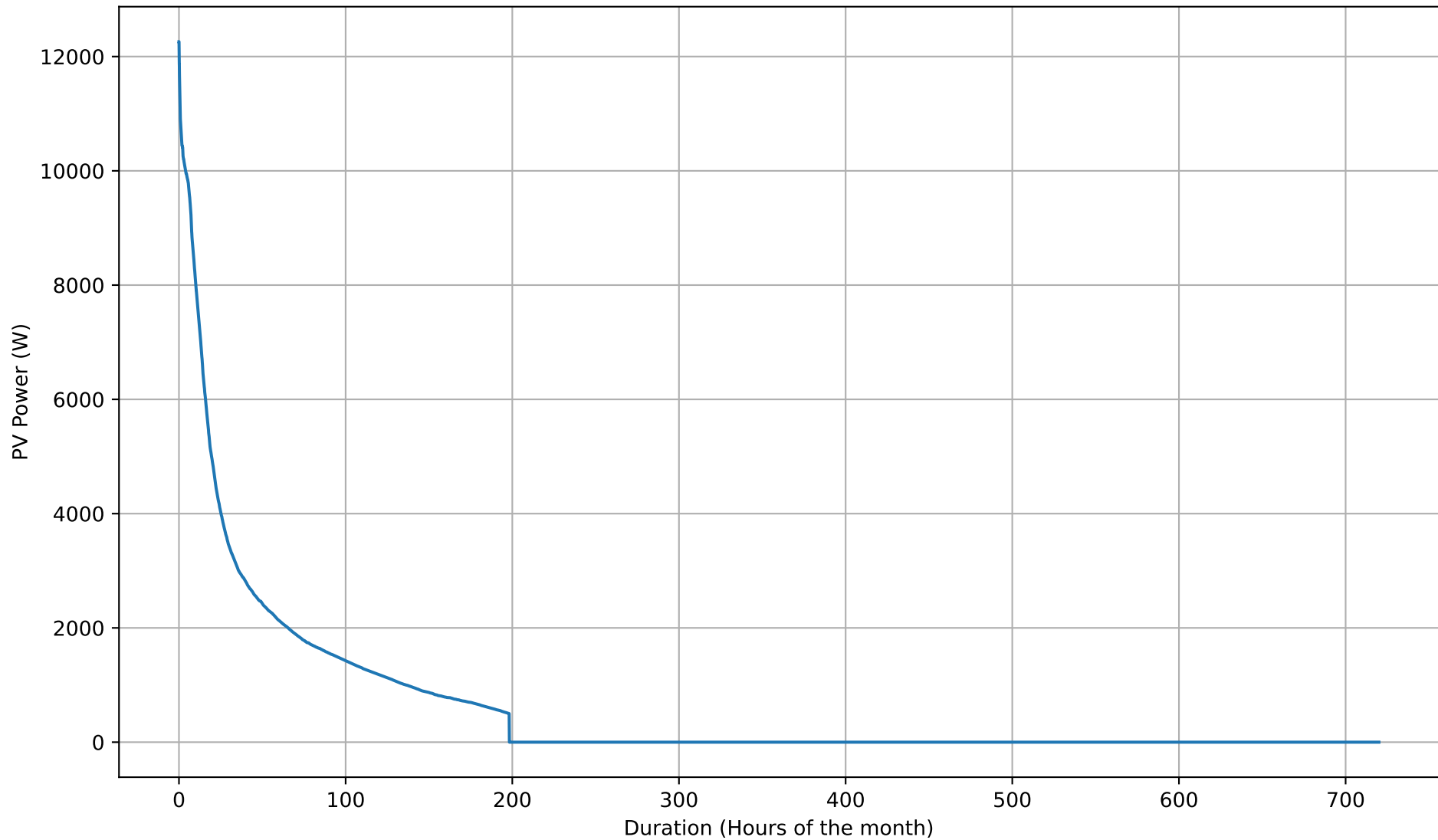
PV Self-Consumption Duration Curve - 12kWh - Nov
