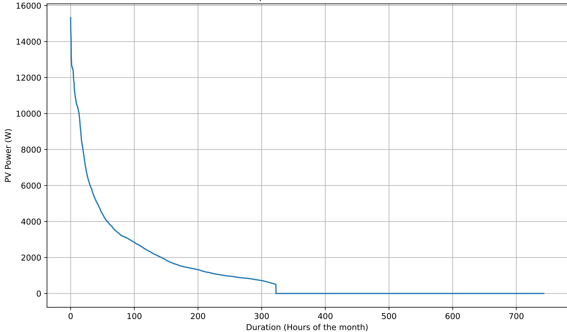
PV Self-Consumption Duration Curve - 12kWh - Mar
