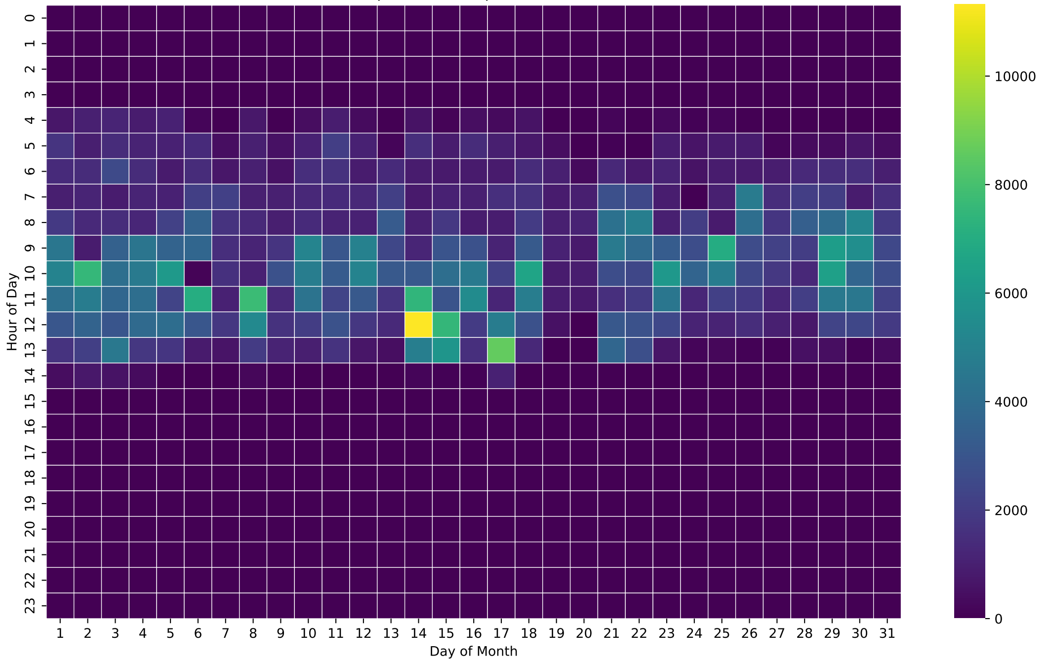
PV Self-Consumption Heatmap (Wh/Hour) - 12kWh - Oct
