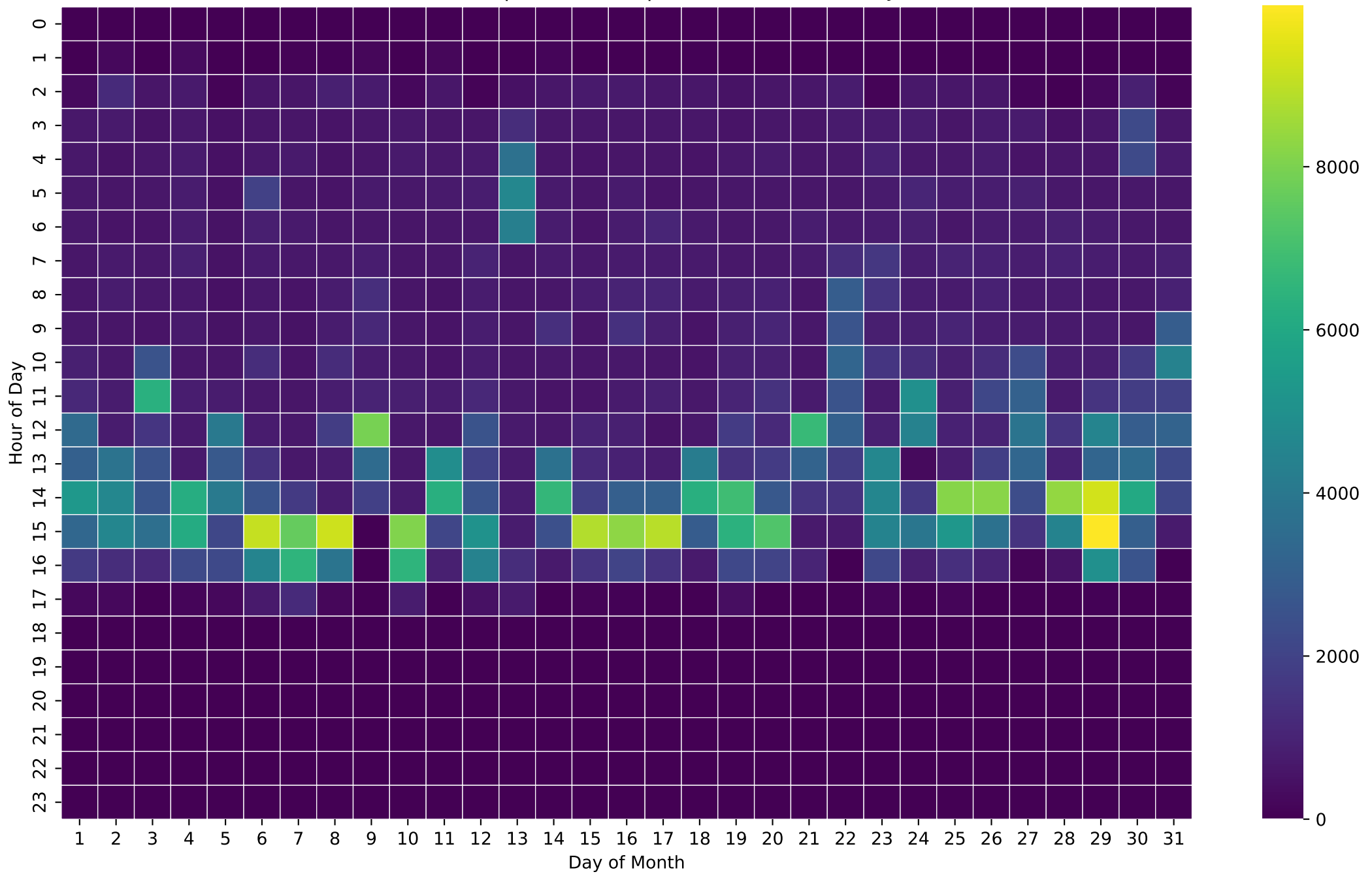
PV Self-Consumption Heatmap (Wh/Hour) - 12kWh - Jul
