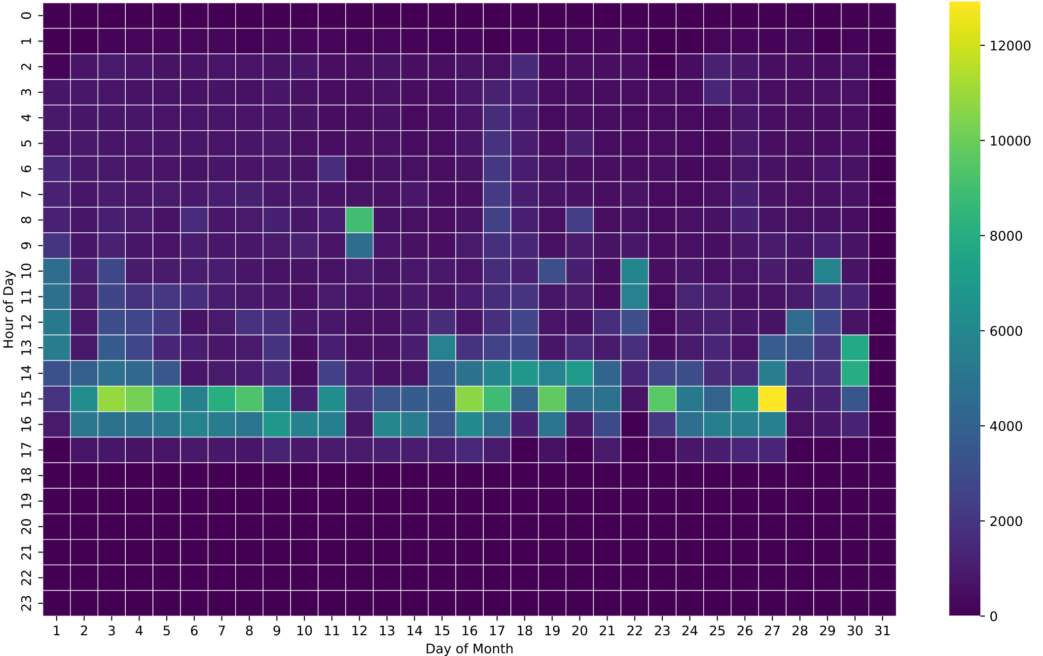
PV Self-Consumption Heatmap (Wh/Hour) - 12kWh - Jun
