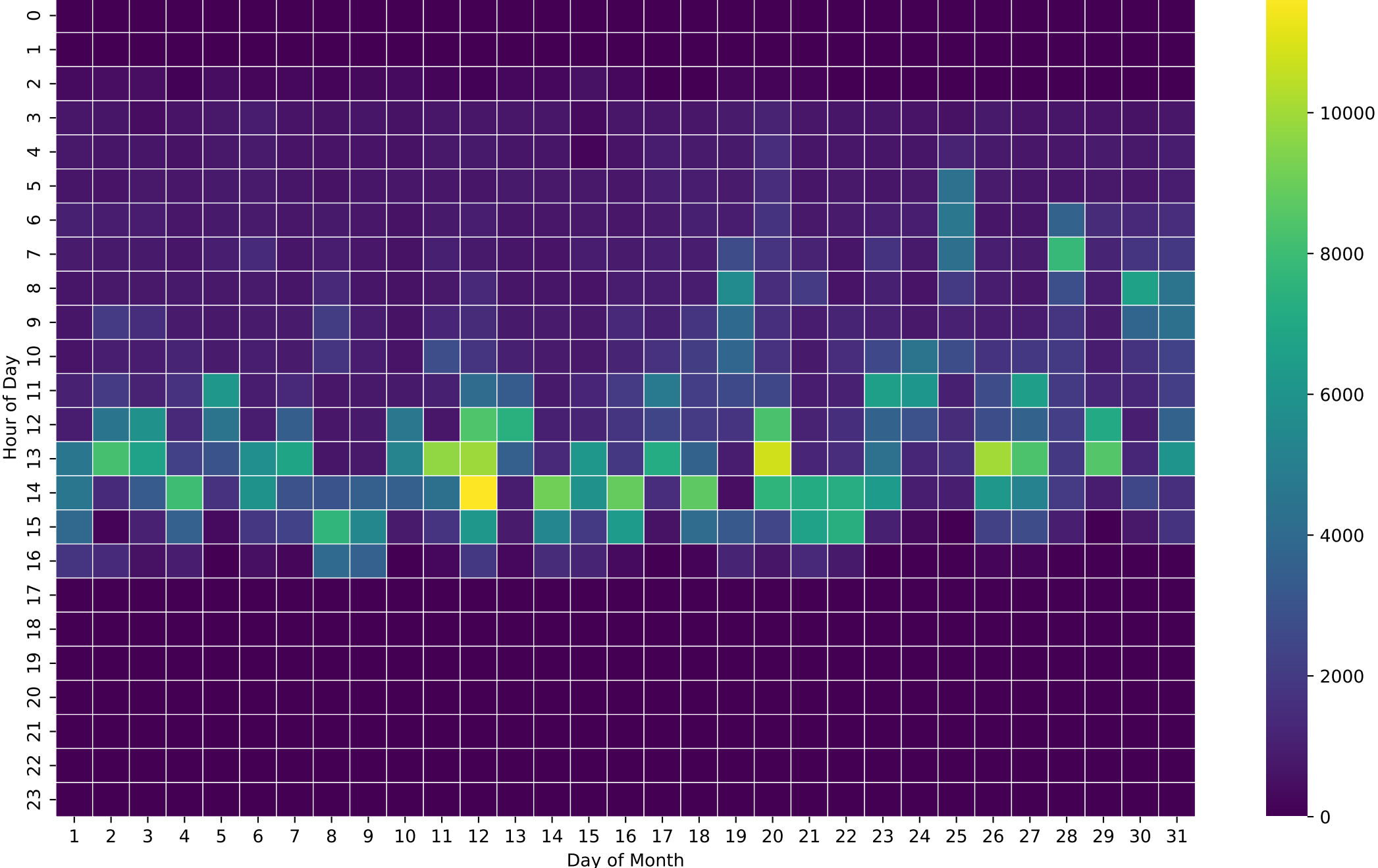
PV Self-Consumption Heatmap (Wh/Hour) - 12kWh - Aug
