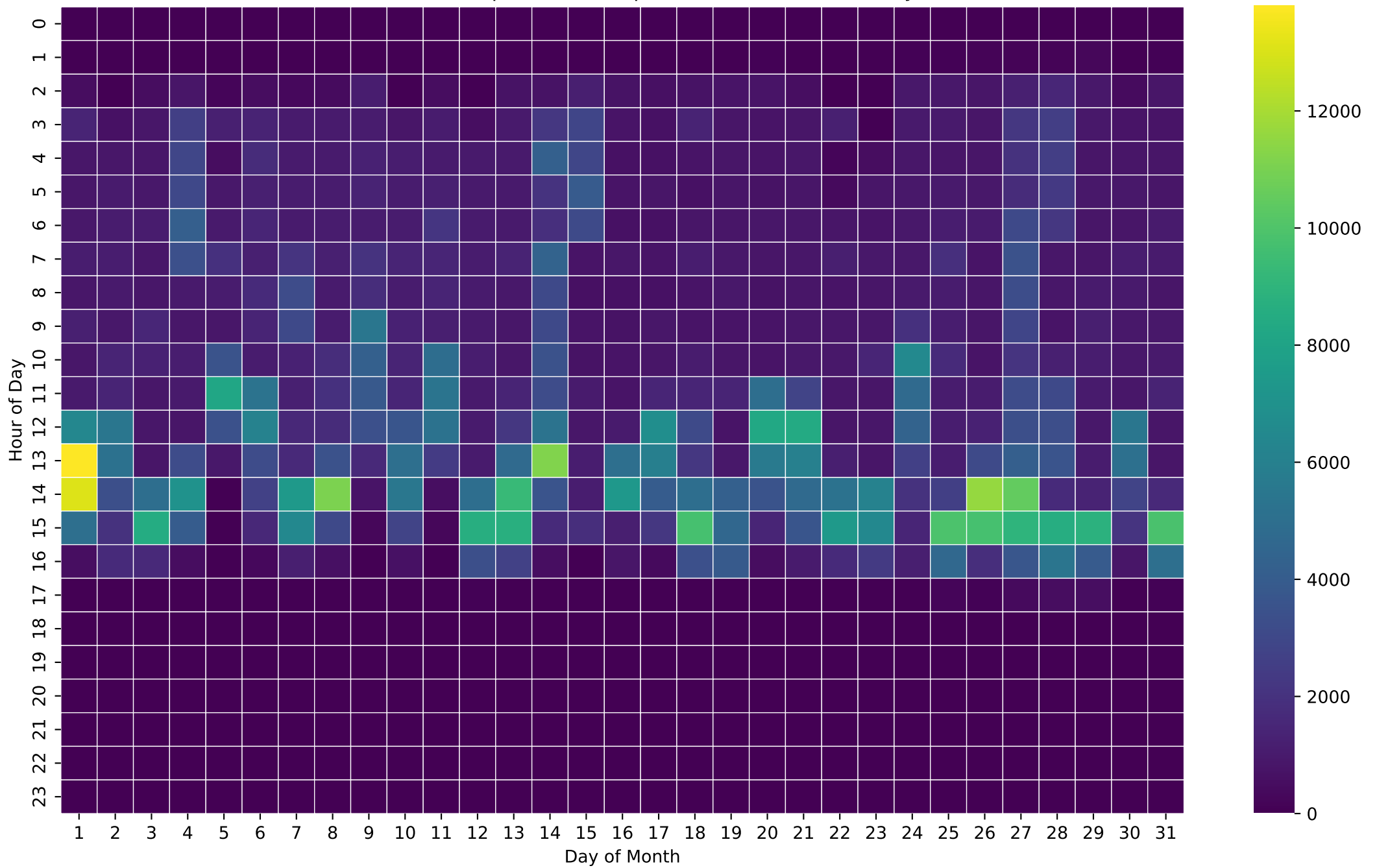
PV Self-Consumption Heatmap (Wh/Hour) - 12kWh - May
