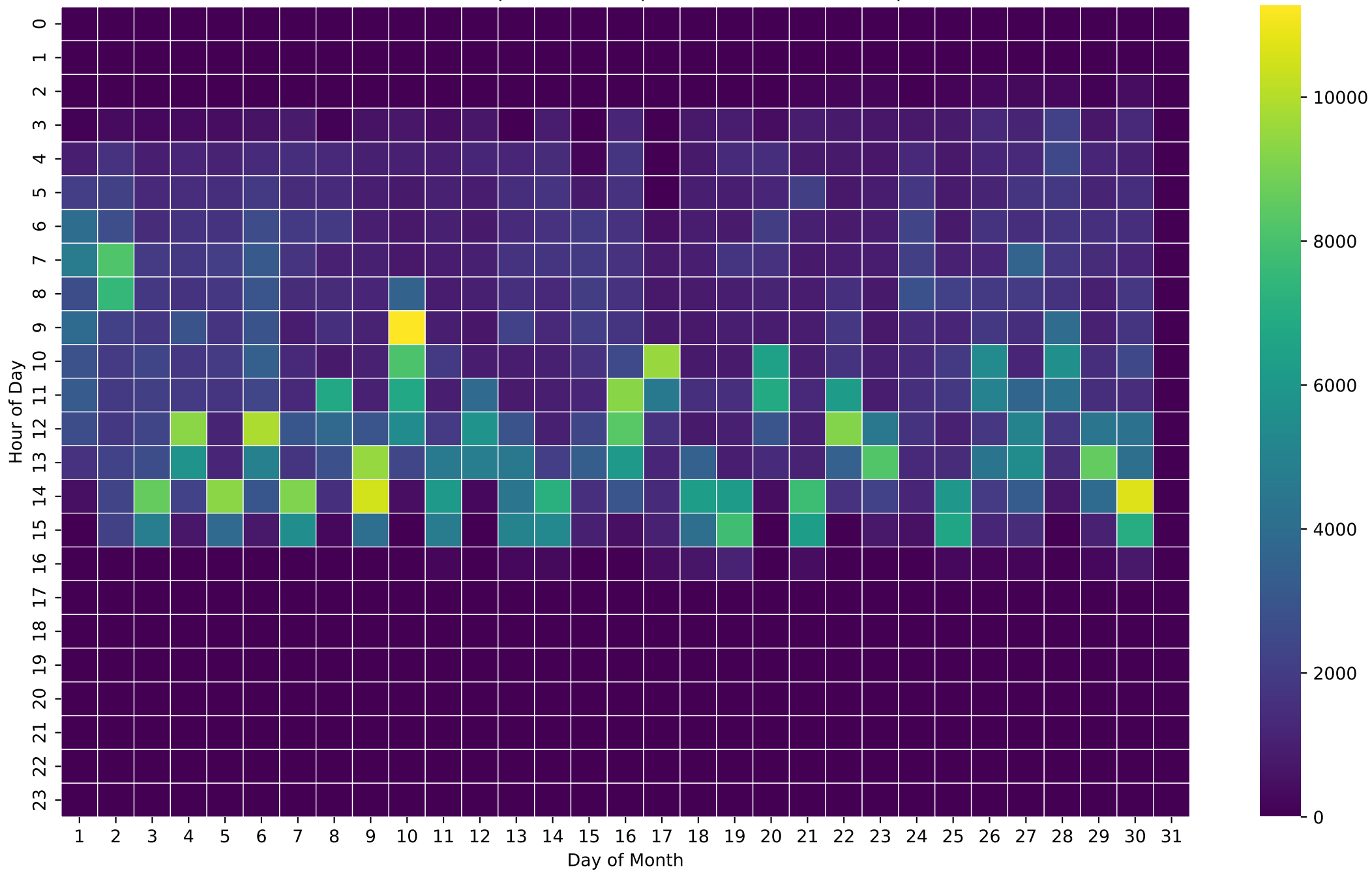
PV Self-Consumption Heatmap (Wh/Hour) - 12kWh - Apr
