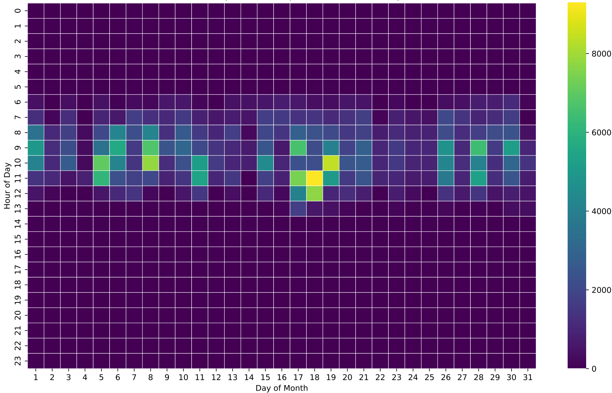
PV Self-Consumption Heatmap (Wh/Hour) - 12kWh - Jan
