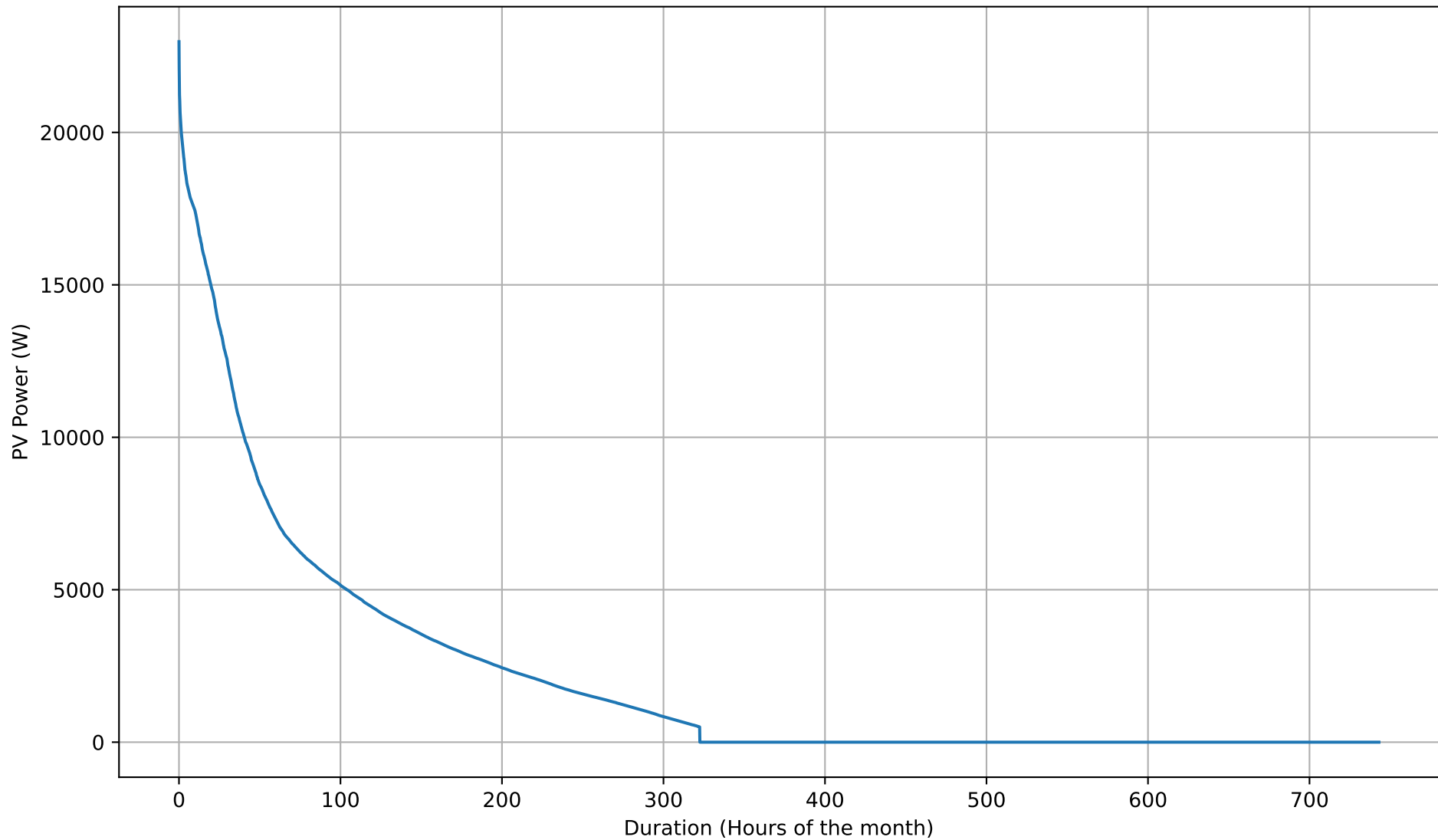
PV Production Duration Curve - 12kWh - Mar
