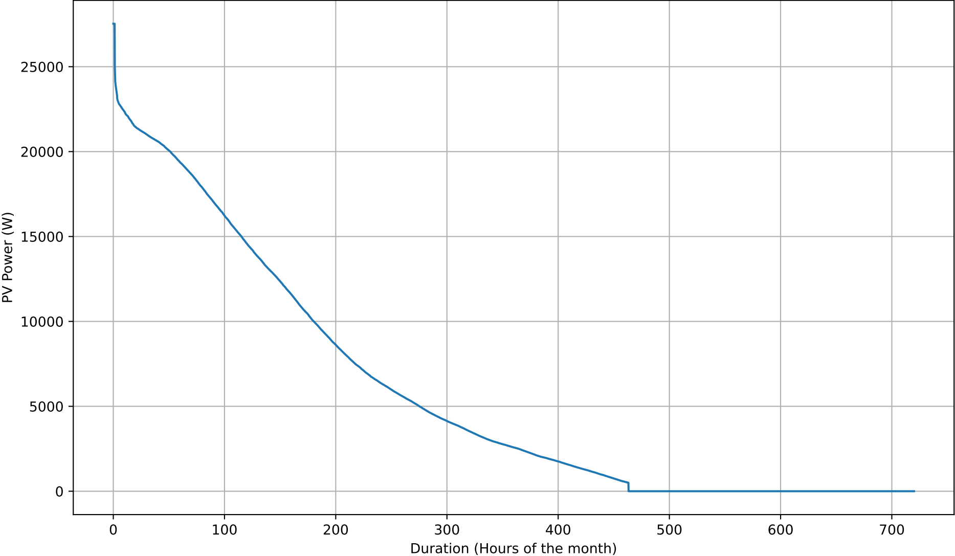
PV Production Duration Curve - 12kWh - Jun
