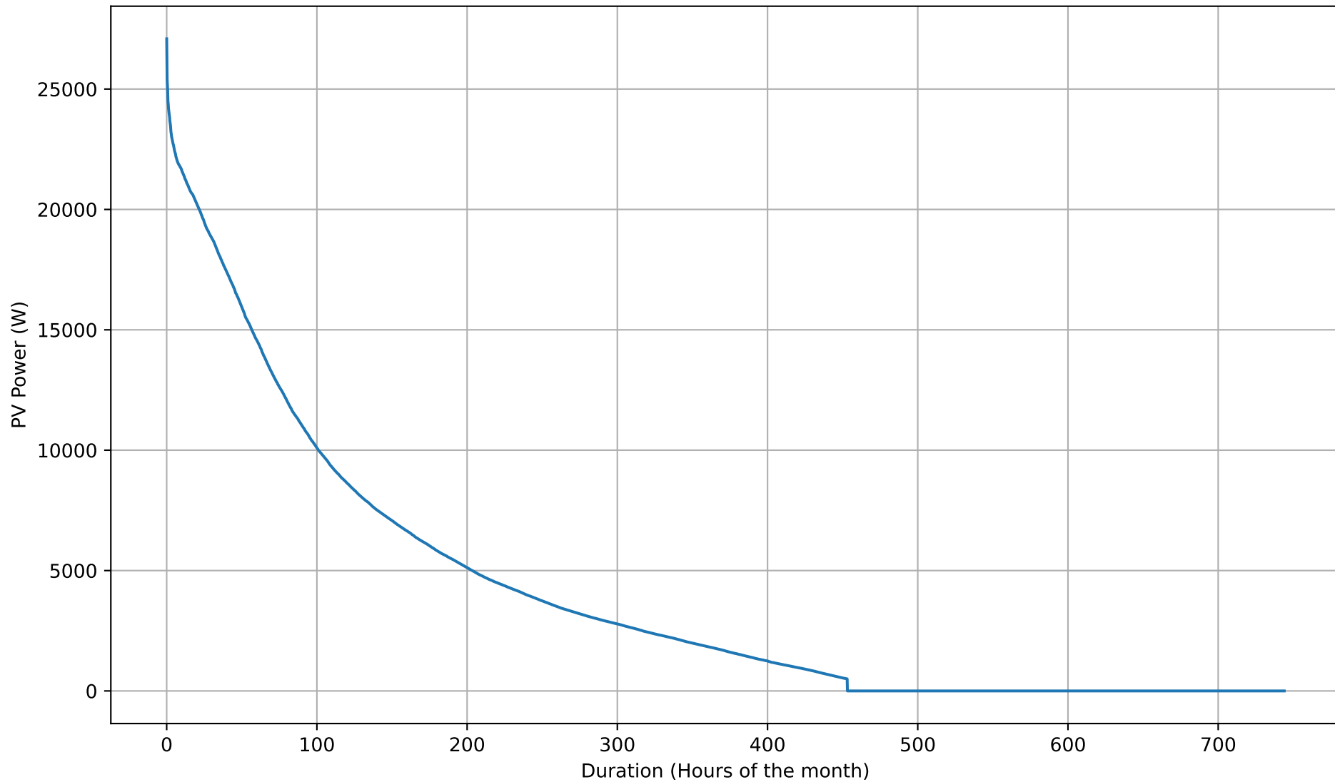
PV Production Duration Curve - 12kWh - Jul
