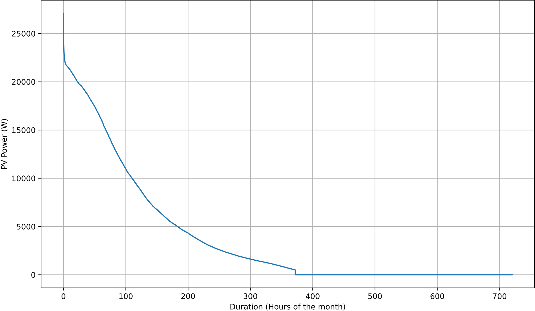
PV Production Duration Curve - 12kWh - Apr
