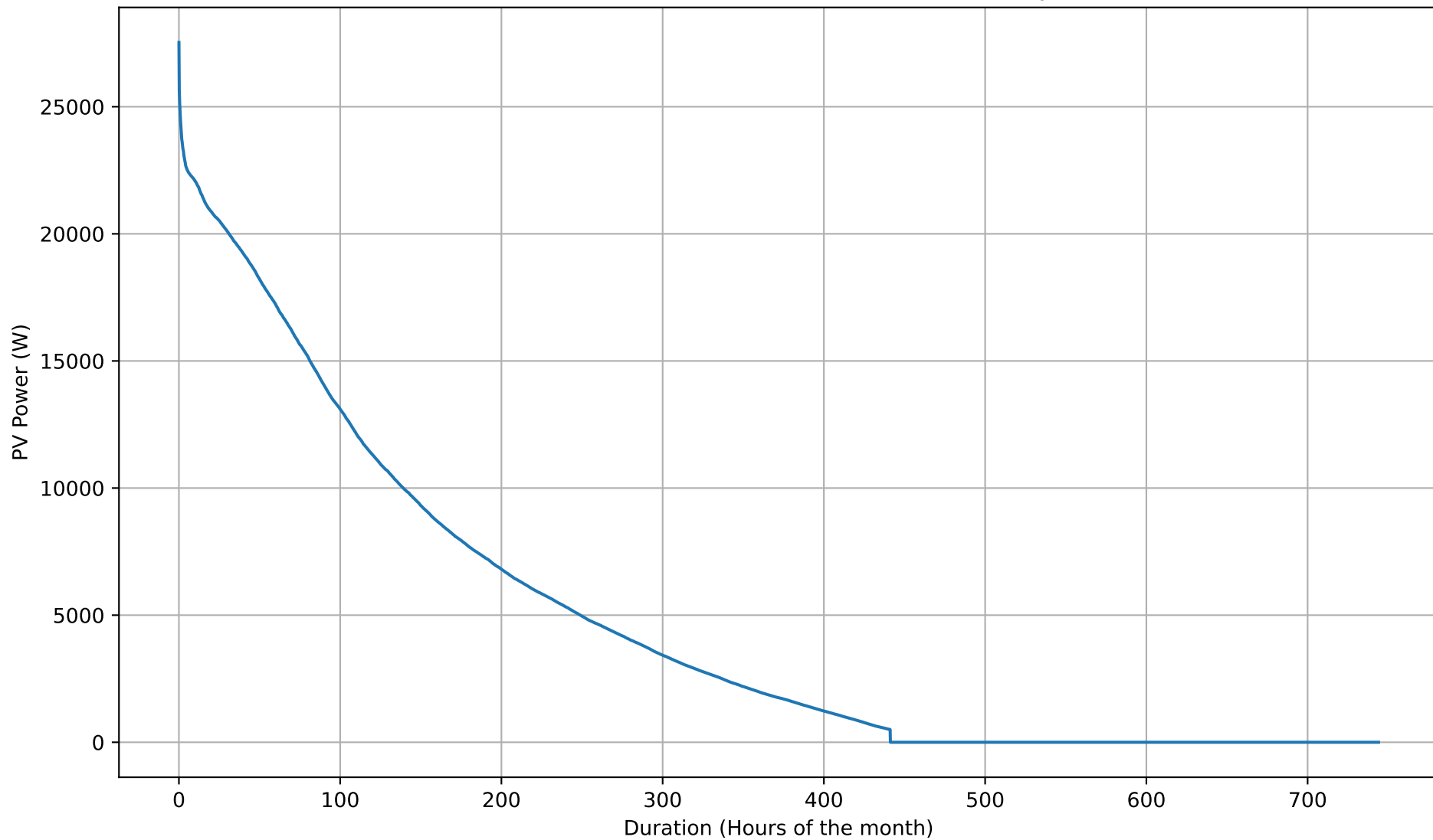
PV Production Duration Curve - 12kWh - May
