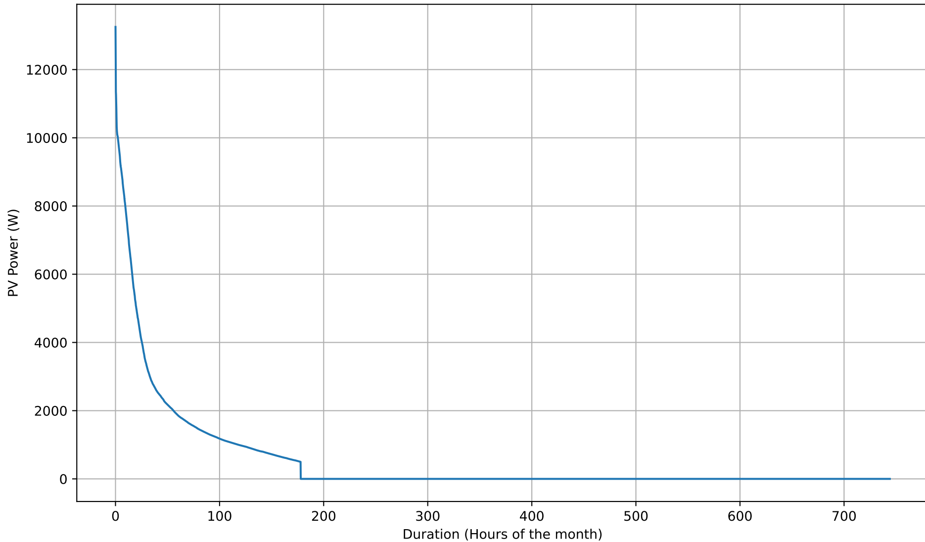
PV Production Duration Curve - 12kWh - Jan
