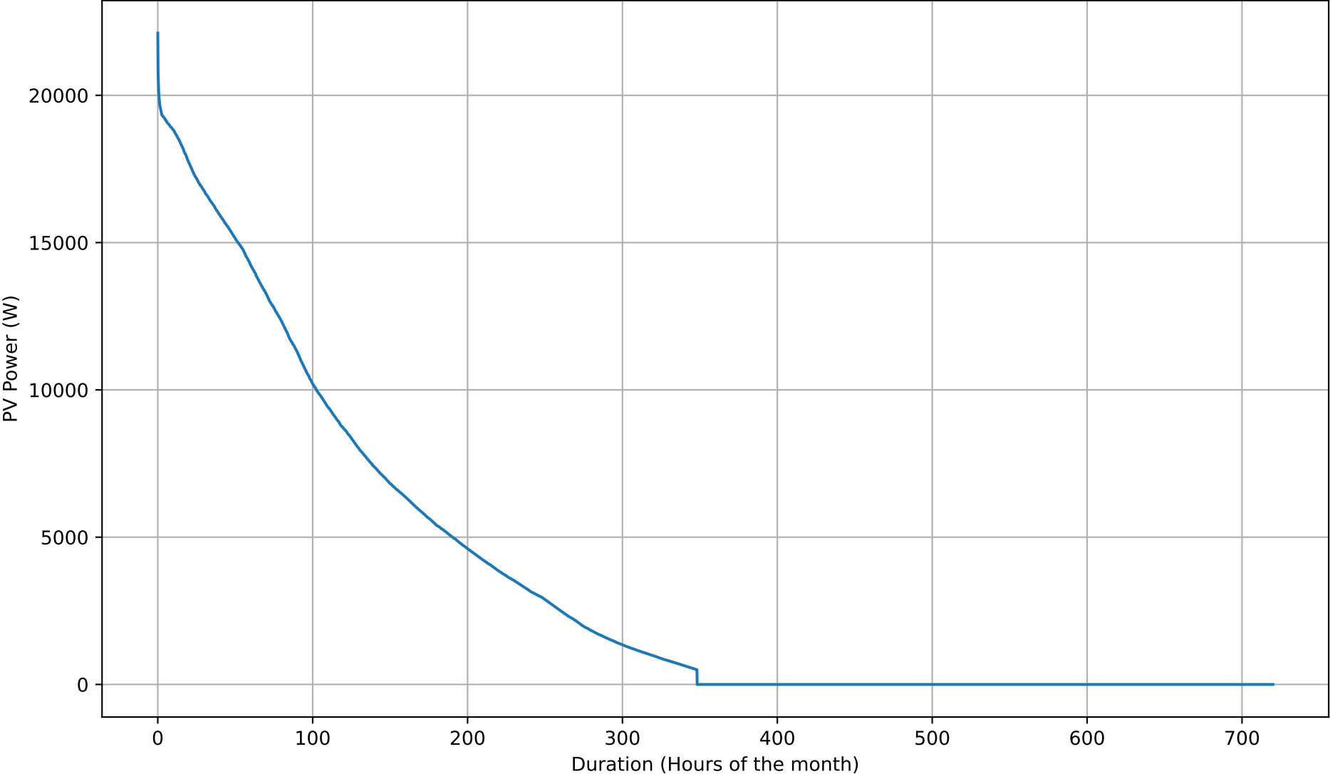
PV Production Duration Curve - 12kWh - Sep
