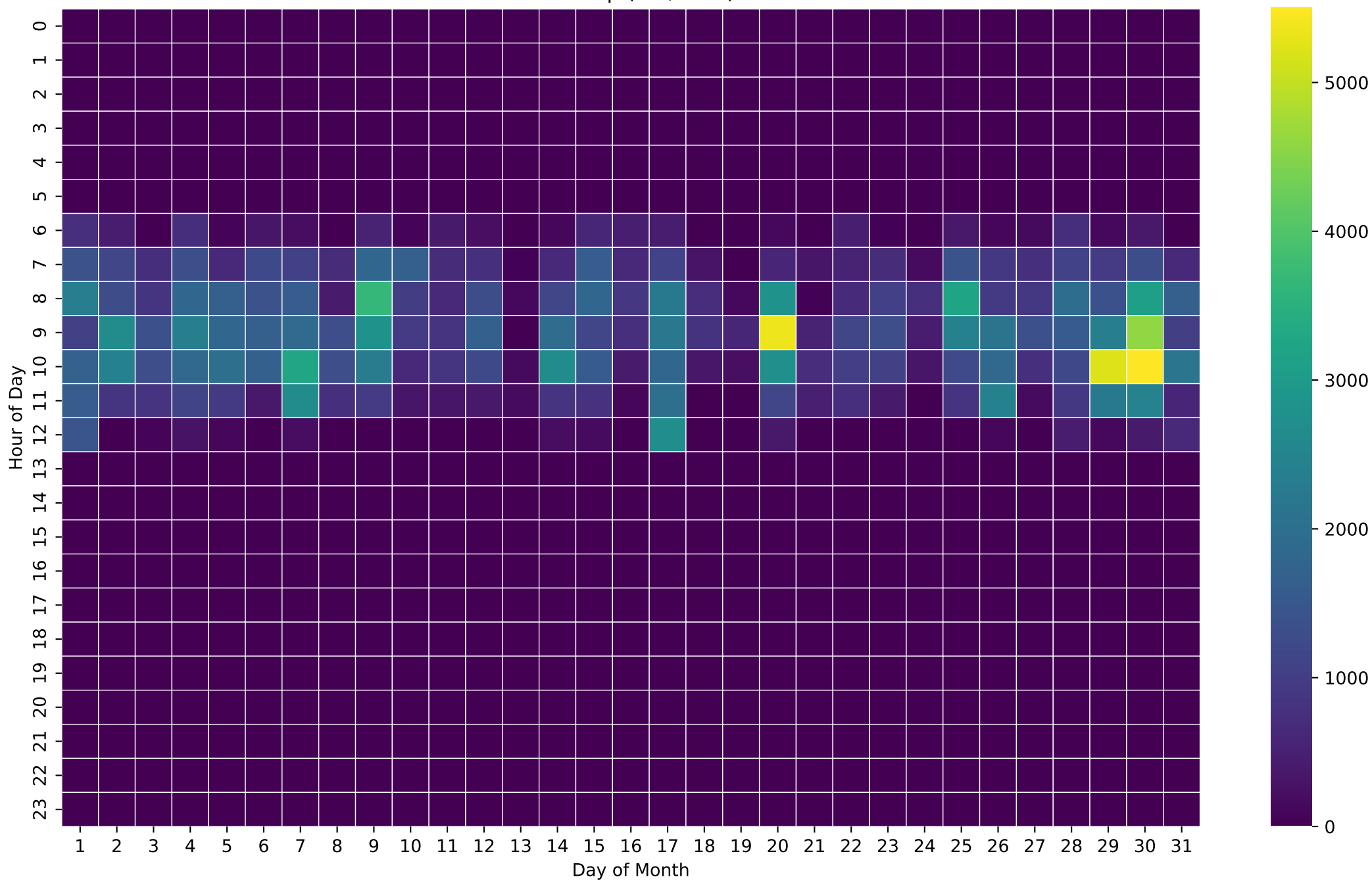
PV Production Heatmap (Wh/Hour) - 12kWh - Dec
