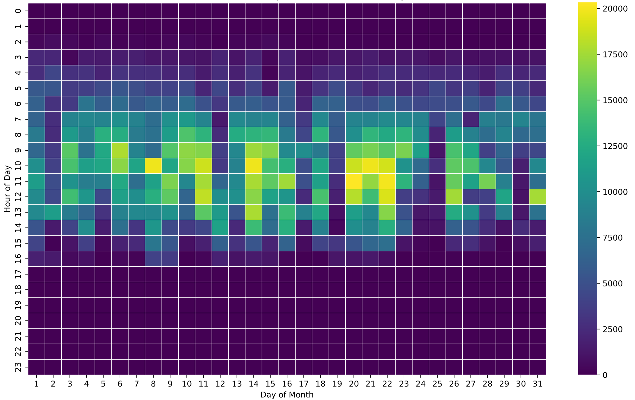
PV Production Heatmap (Wh/Hour) - 12kWh - Aug
