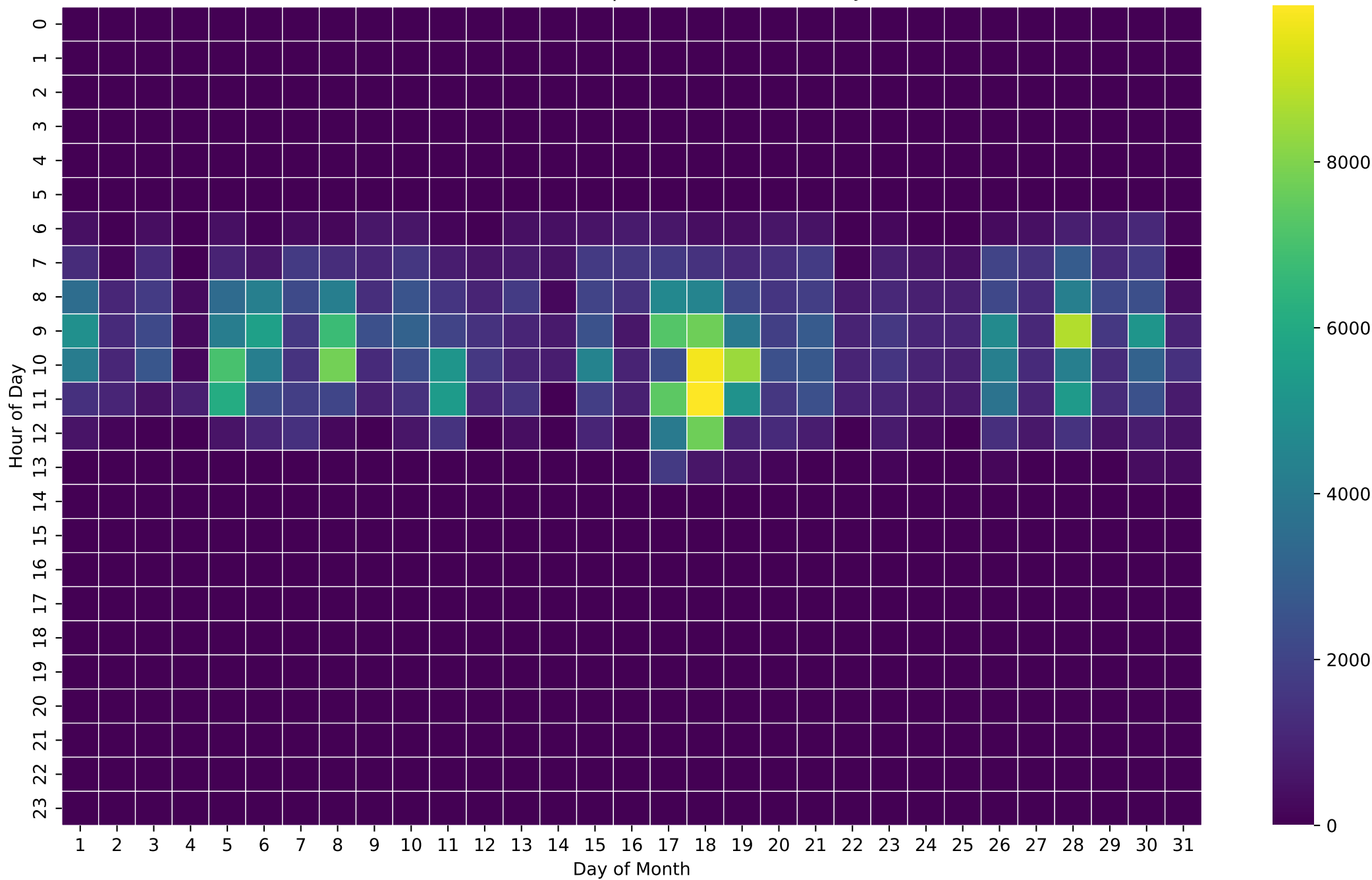
PV Production Heatmap (Wh/Hour) - 12kWh - Jan
