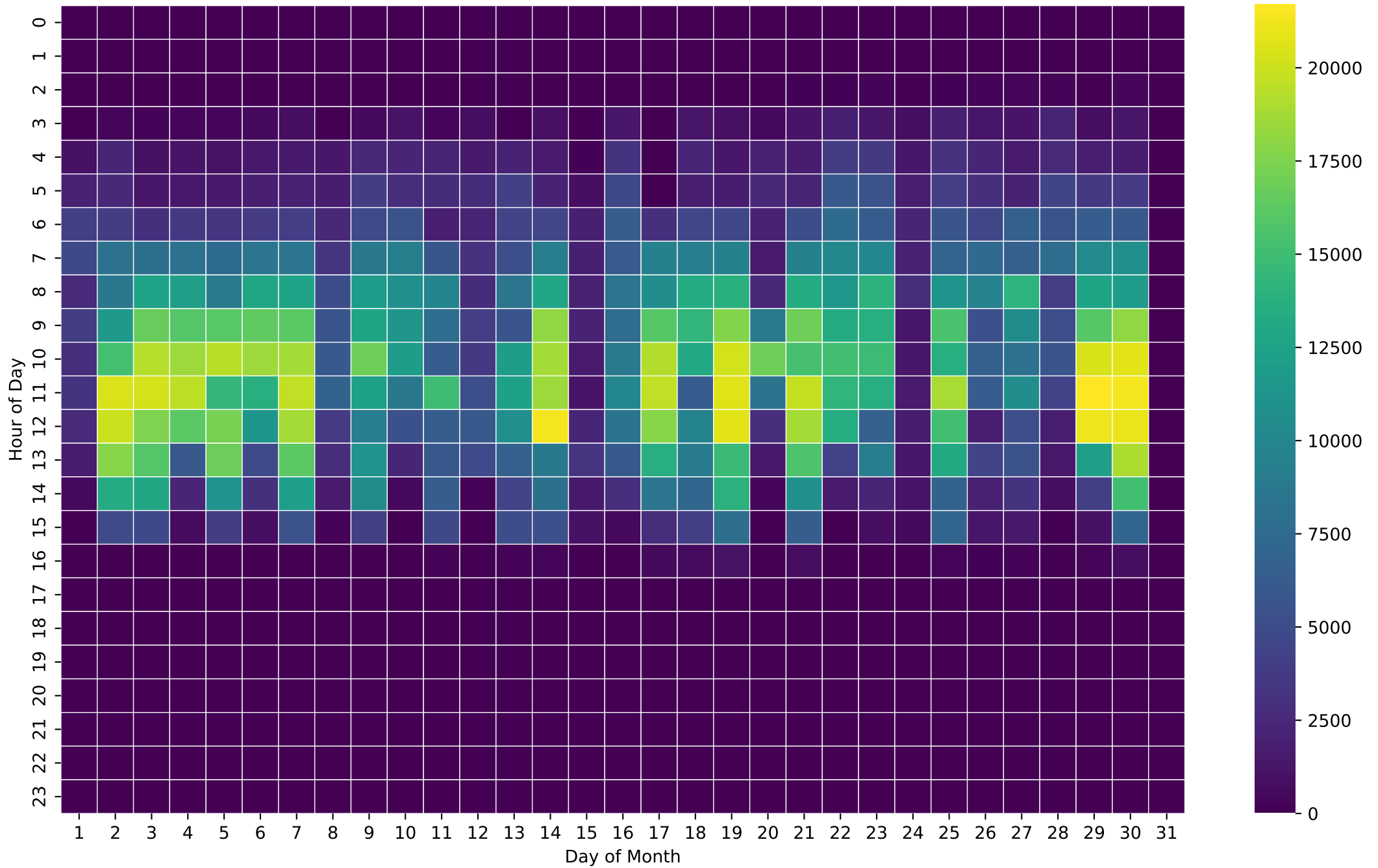
PV Production Heatmap (Wh/Hour) - 12kWh - Apr
