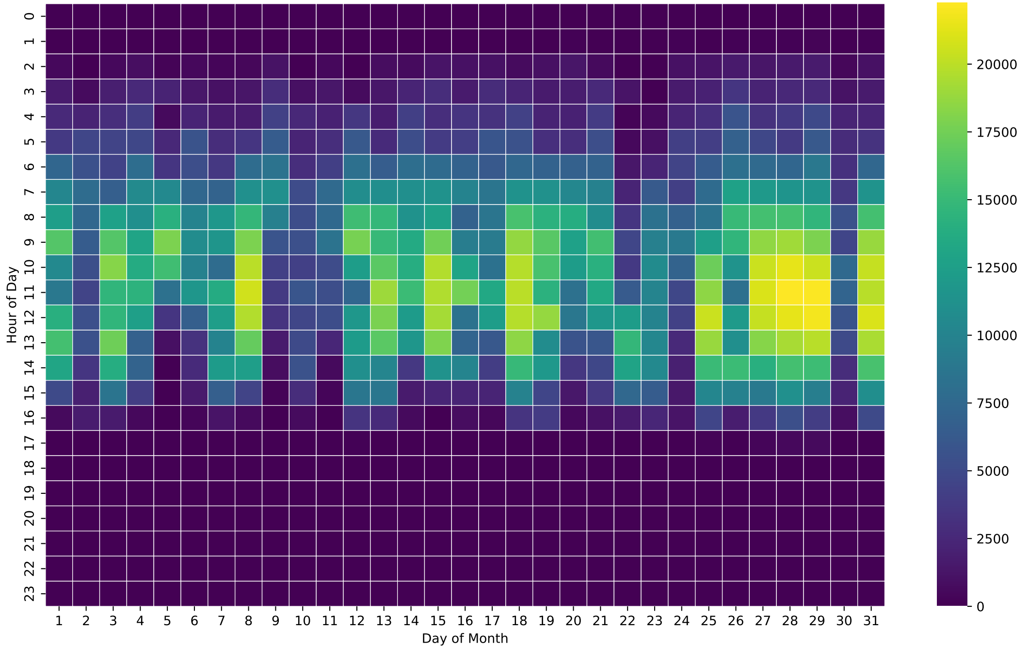
PV Production Heatmap (Wh/Hour) - 12kWh - May
