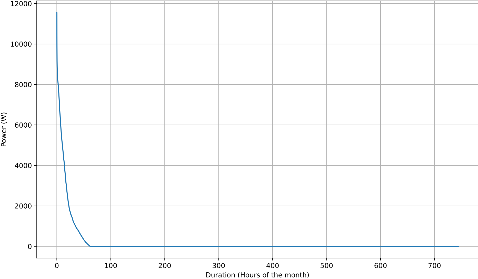
Battery Charging Power Duration Curve - 15kWh - Jan
