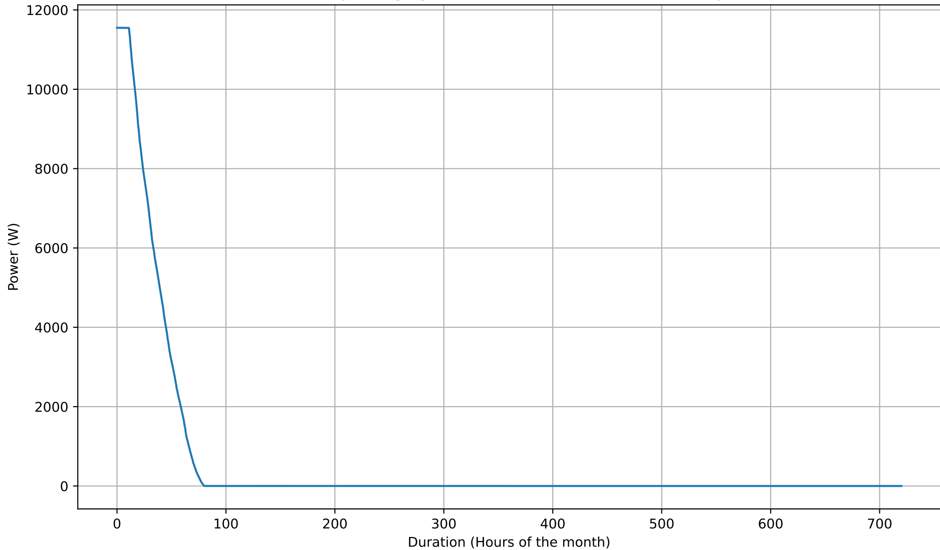
Battery Charging Power Duration Curve - 15kWh - Sep
