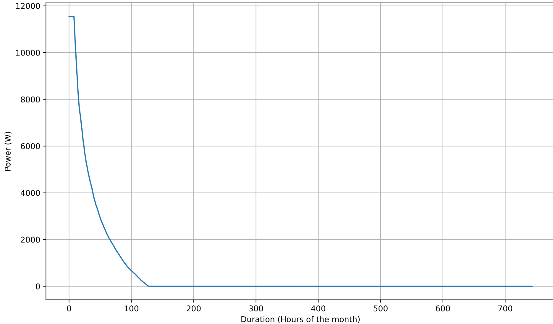
Battery Charging Power Duration Curve - 15kWh - Mar
