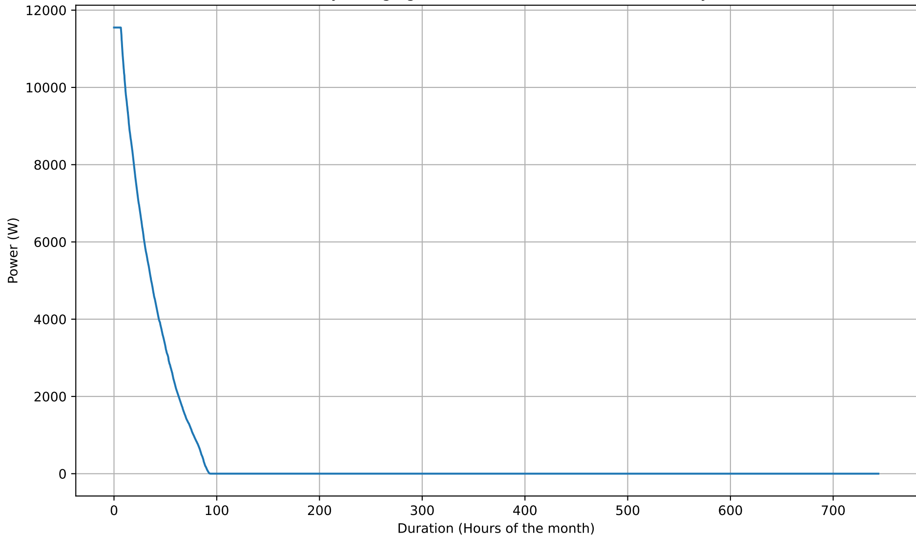
Battery Charging Power Duration Curve - 15kWh - May
