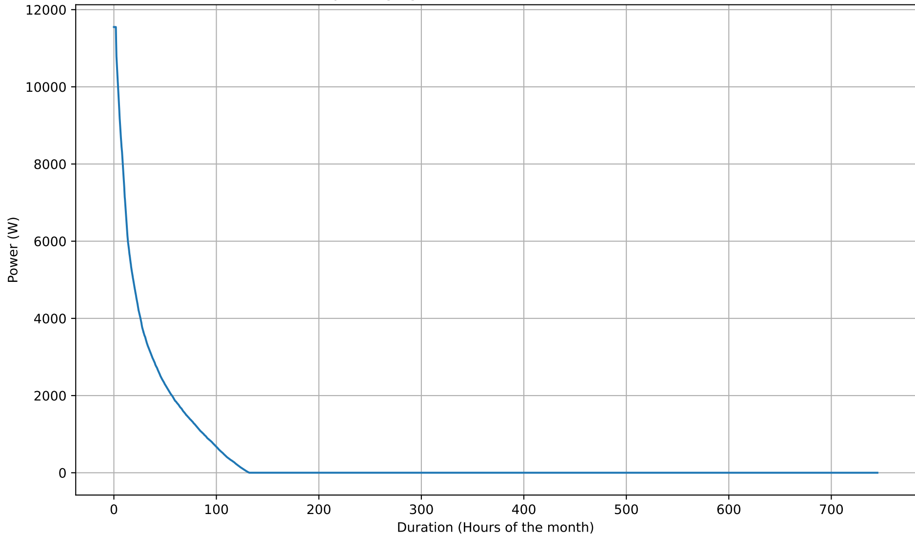
Battery Charging Power Duration Curve - 15kWh - Oct
