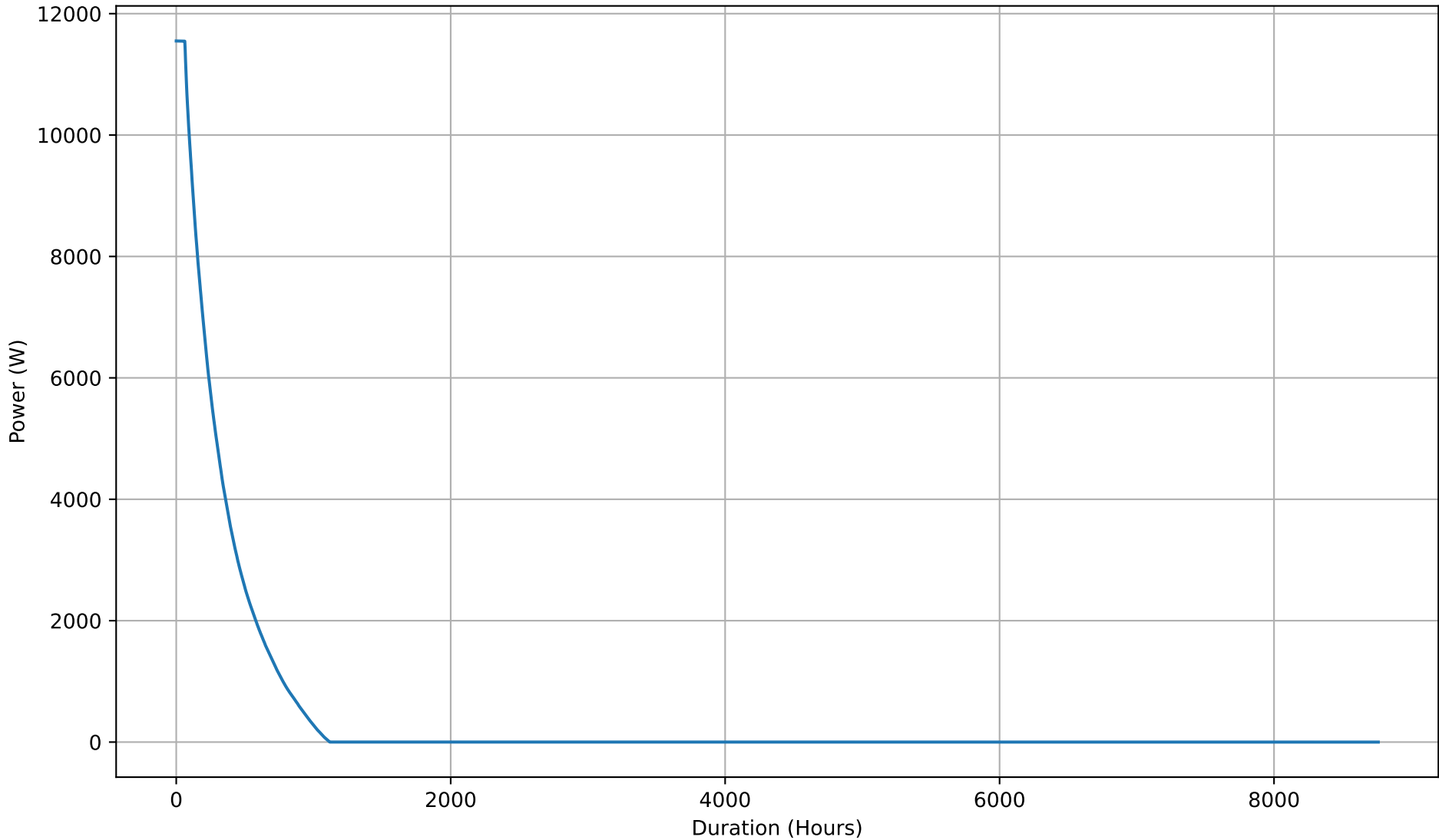
Yearly Battery Charging Power Duration Curve - 15kWh
