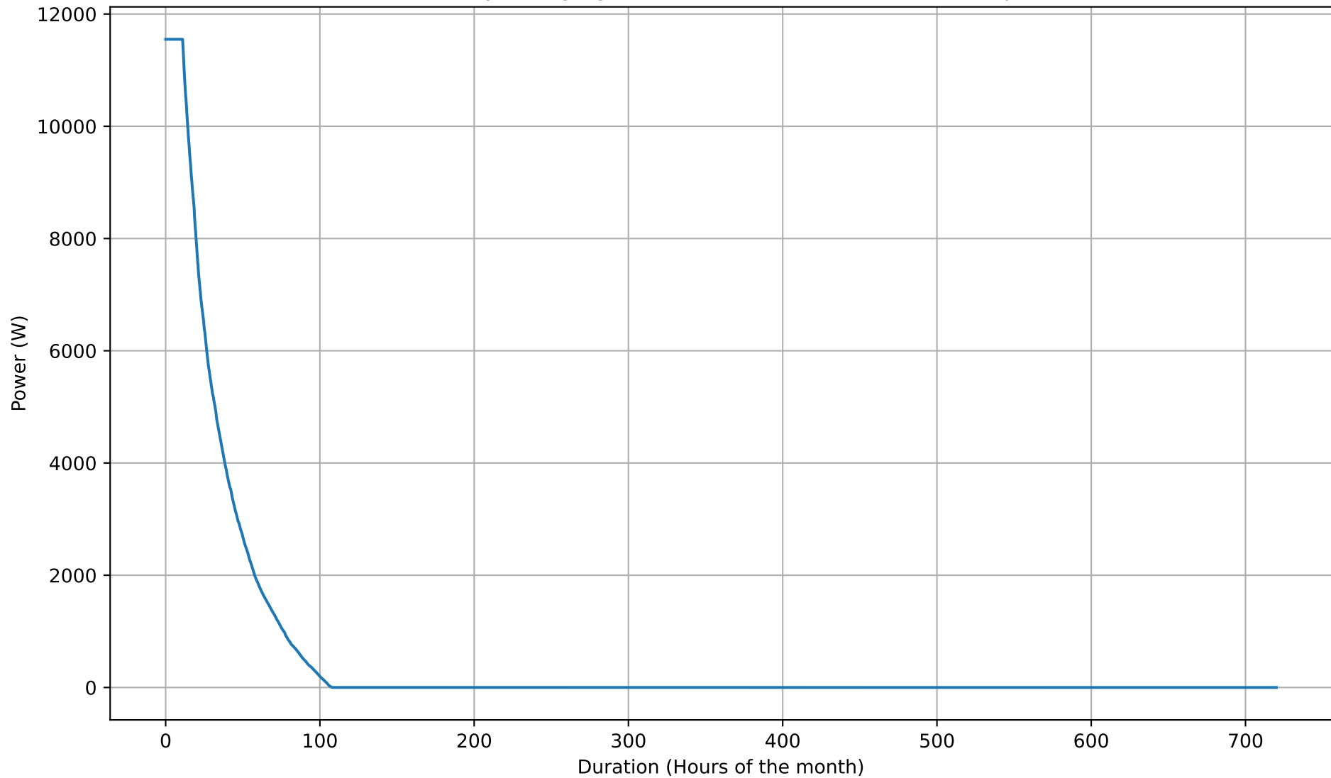
Battery Charging Power Duration Curve - 15kWh - Apr
