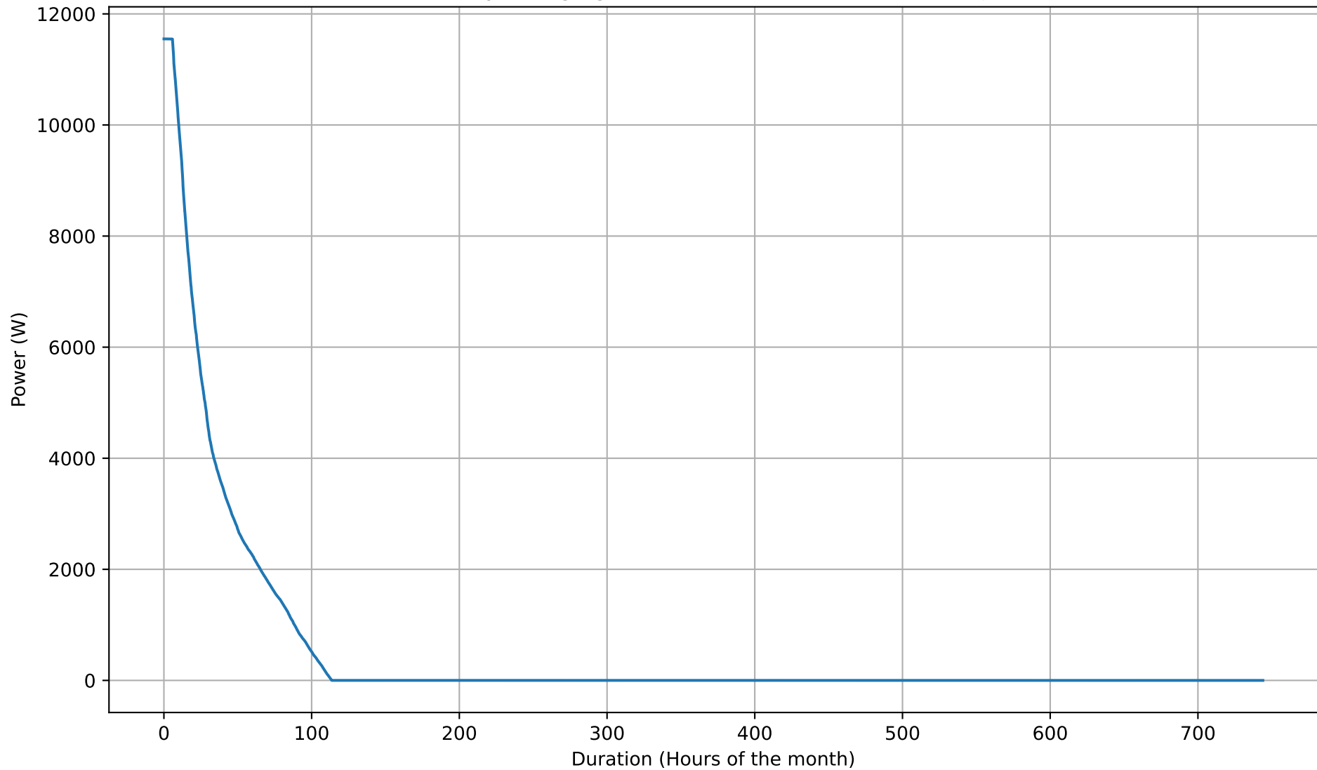
Battery Charging Power Duration Curve - 15kWh - Jul
