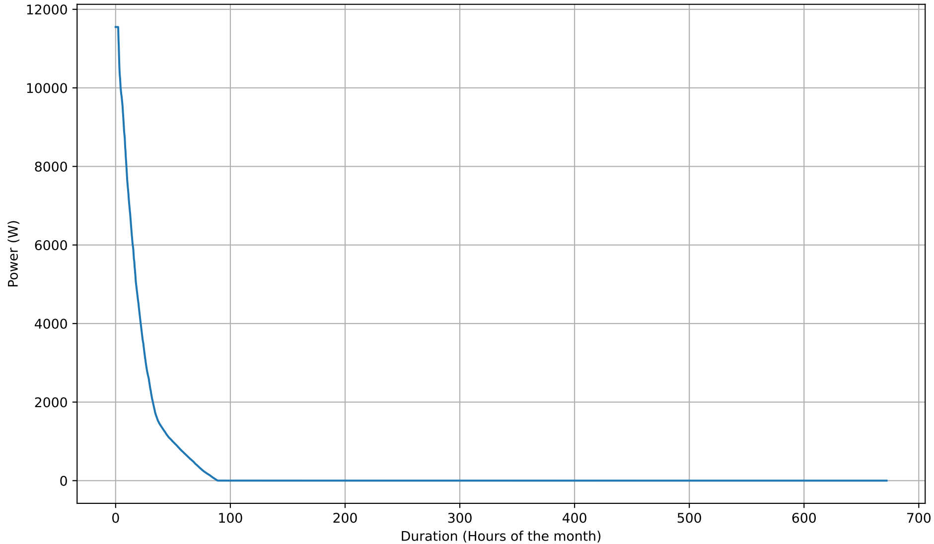
Battery Charging Power Duration Curve - 15kWh - Feb
