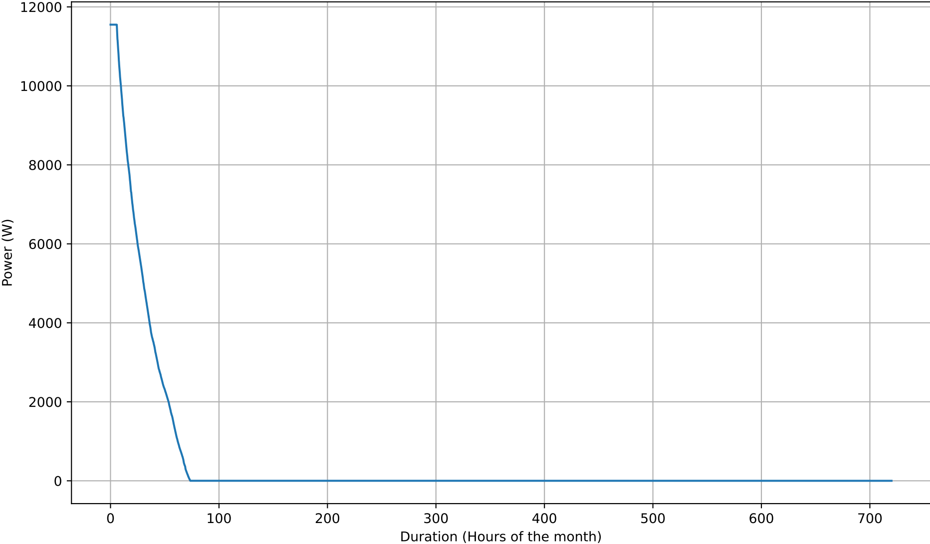
Battery Charging Power Duration Curve - 15kWh - Jun
