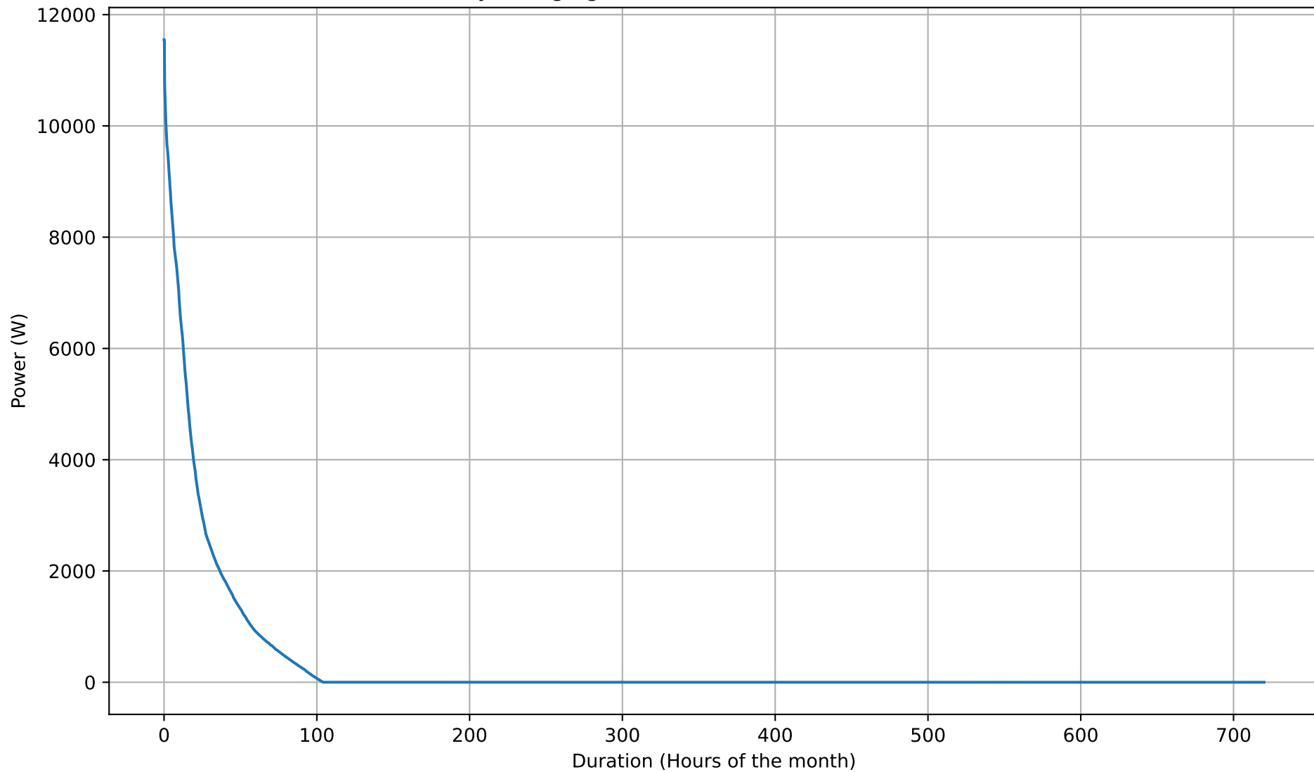
Battery Charging Power Duration Curve - 15kWh - Nov
