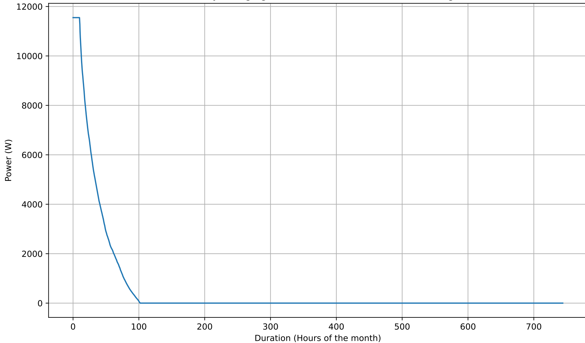
Battery Charging Power Duration Curve - 15kWh - Aug
