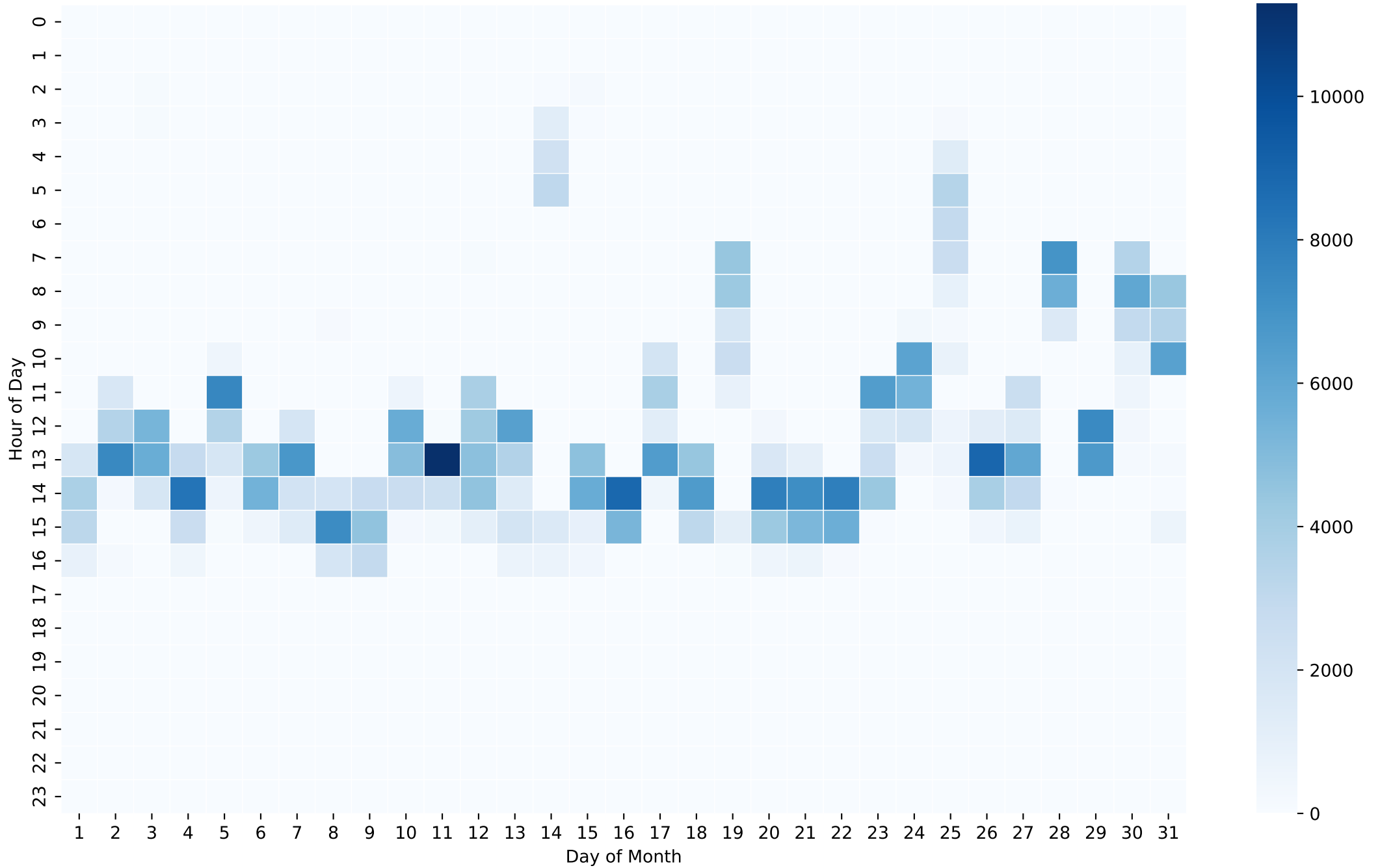
Battery Charging Power Heatmap (Wh/Hour) - 15kWh - Aug
