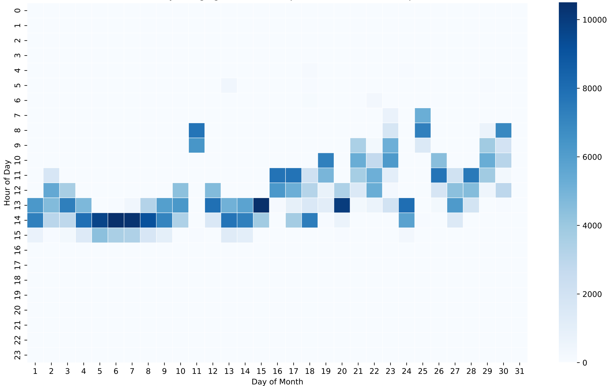
Battery Charging Power Heatmap (Wh/Hour) - 15kWh - Sep
