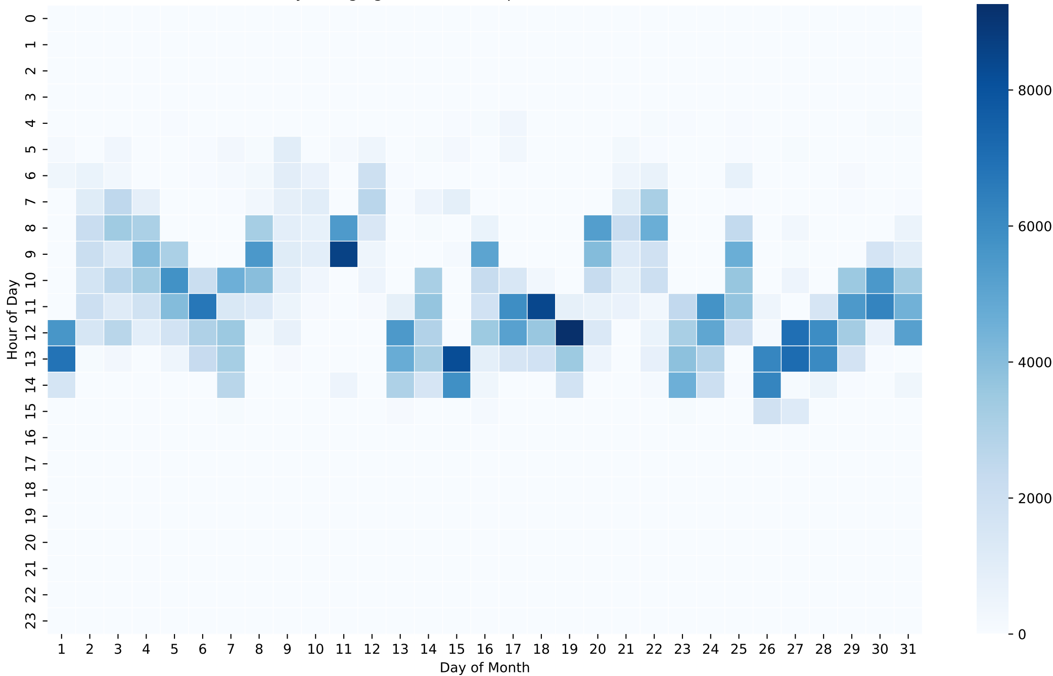
Battery Charging Power Heatmap (Wh/Hour) - 15kWh - Mar
