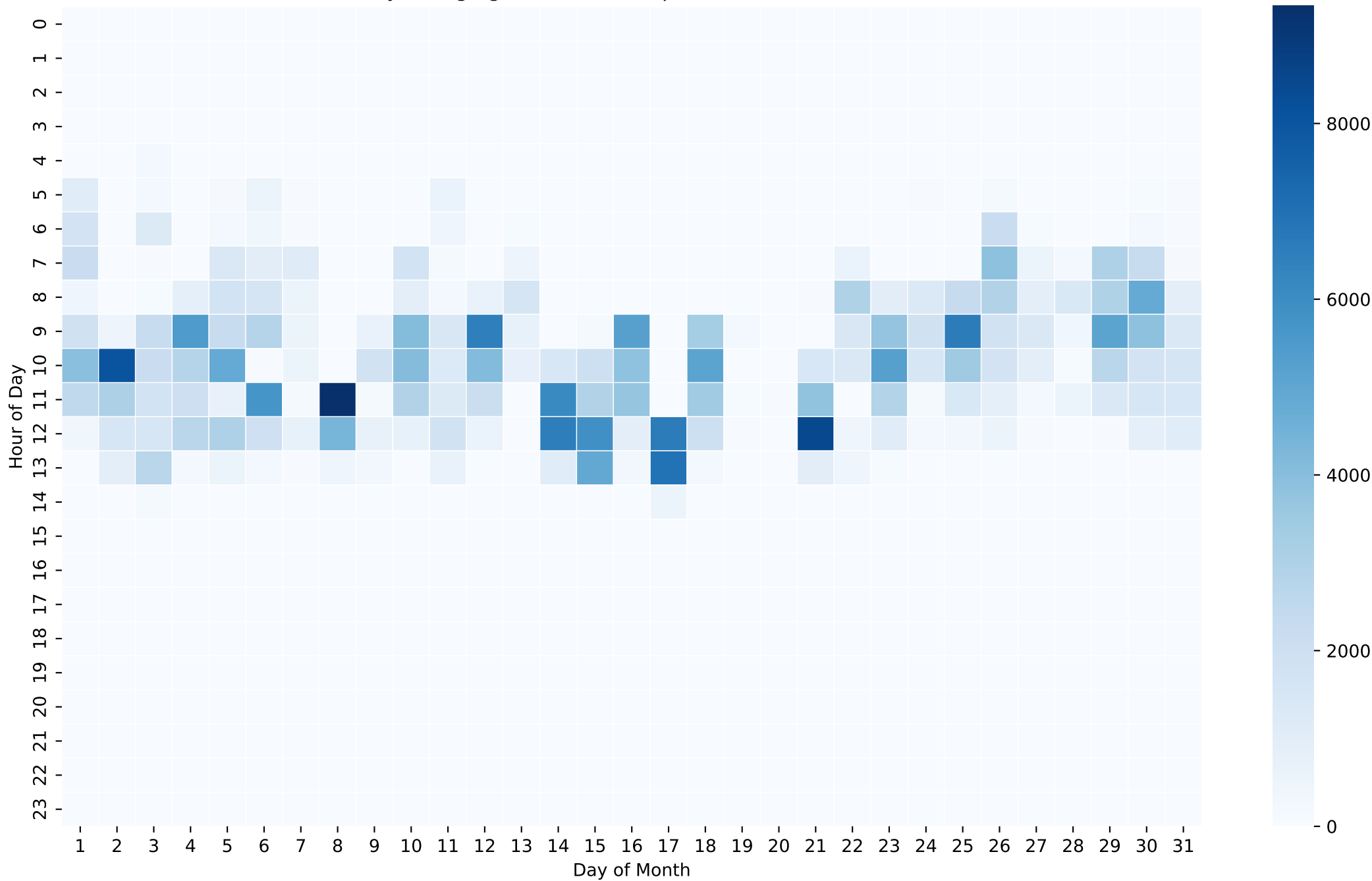
Battery Charging Power Heatmap (Wh/Hour) - 15kWh - Oct
