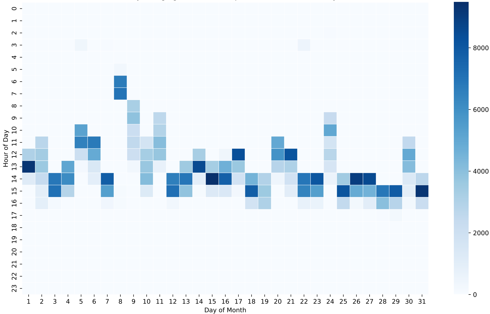
Battery Charging Power Heatmap (Wh/Hour) - 15kWh - May
