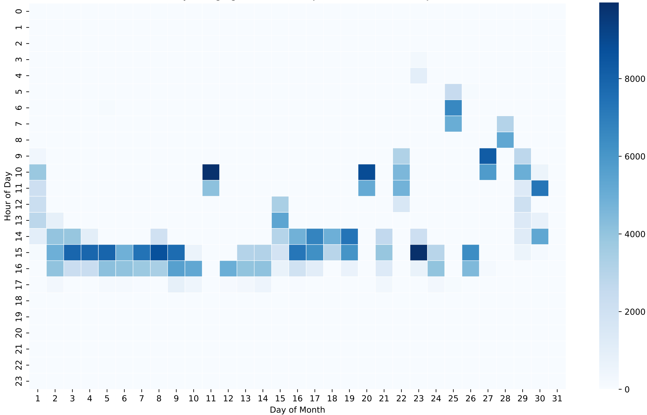
Battery Charging Power Heatmap (Wh/Hour) - 15kWh - Jun
