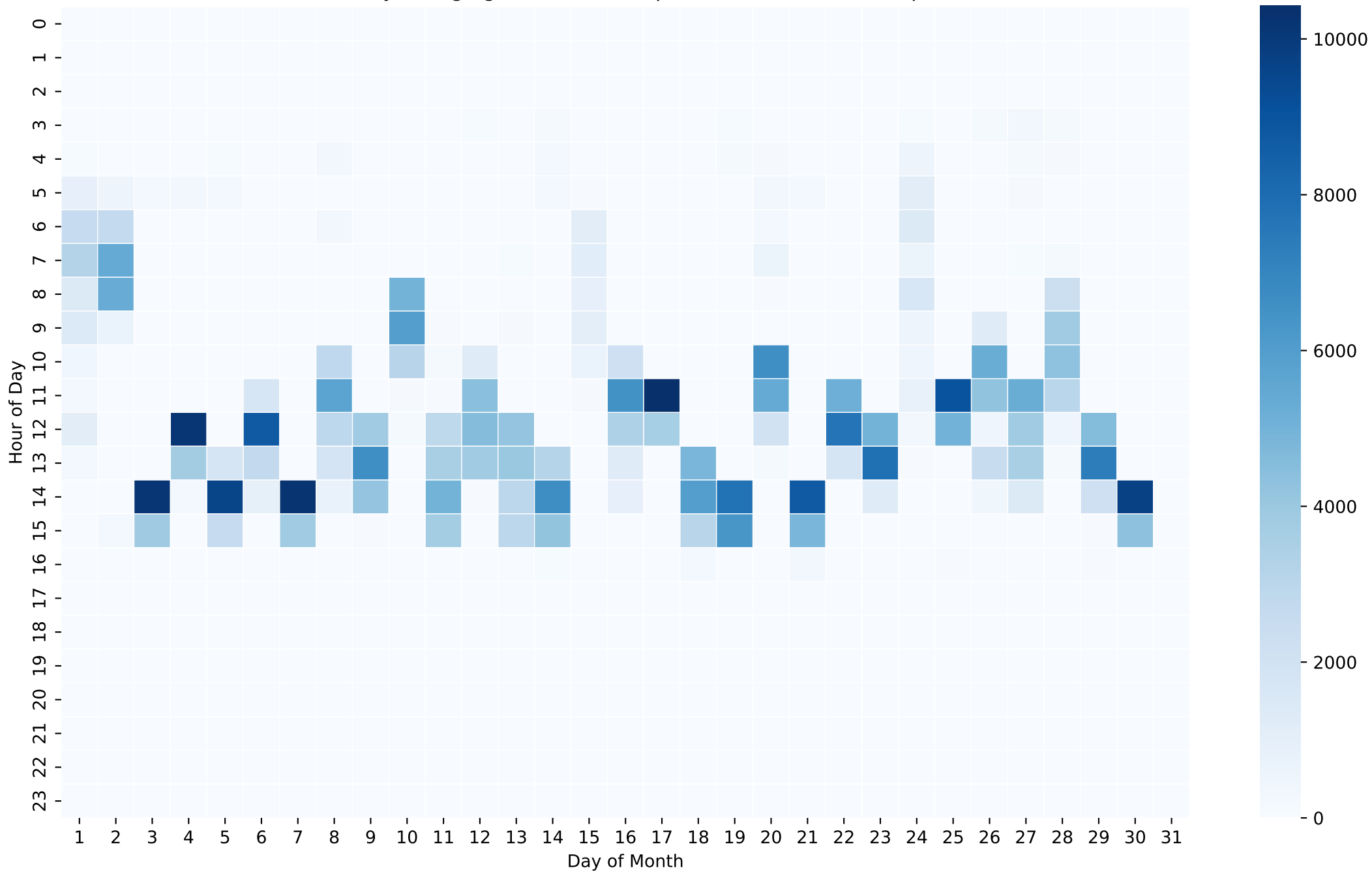
Battery Charging Power Heatmap (Wh/Hour) - 15kWh - Apr
