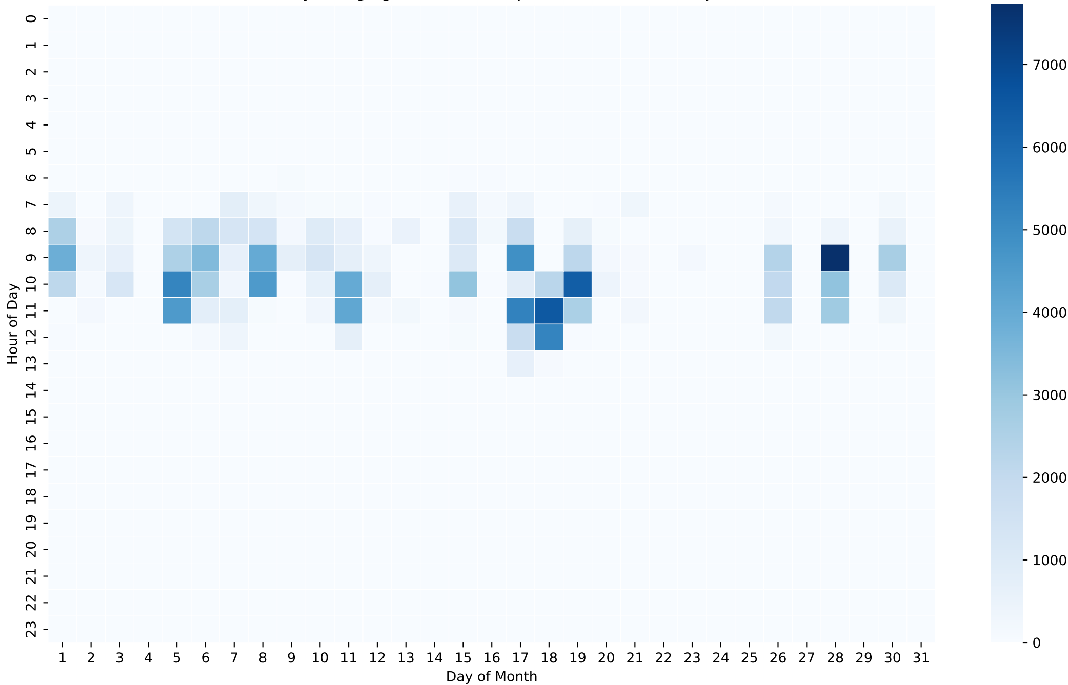
Battery Charging Power Heatmap (Wh/Hour) - 15kWh - Jan
