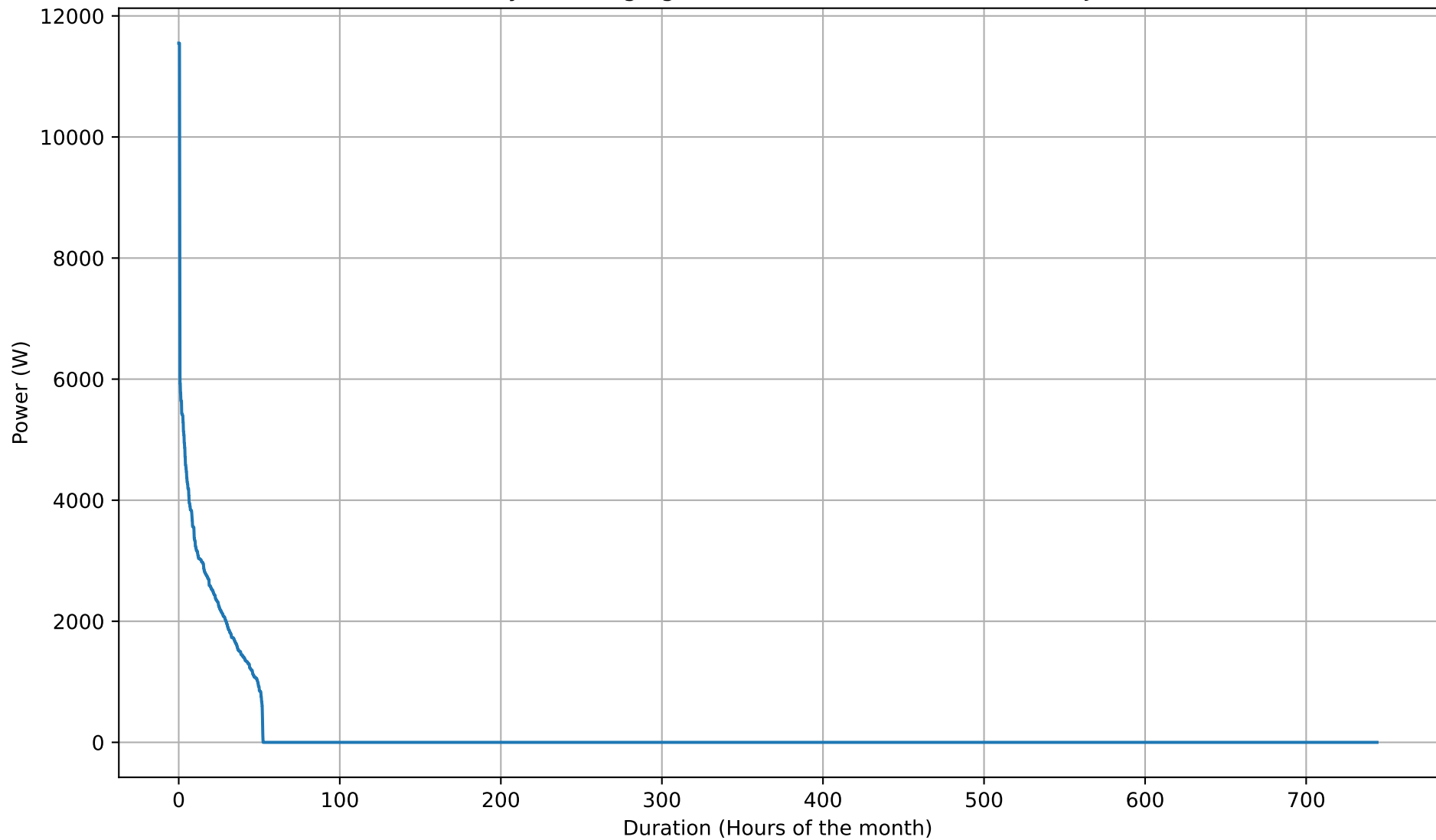
Battery Discharging Power Duration Curve - 15kWh - Jan
