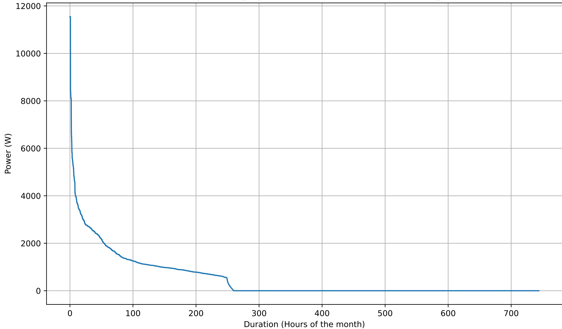
Battery Discharging Power Duration Curve - 15kWh - Aug
