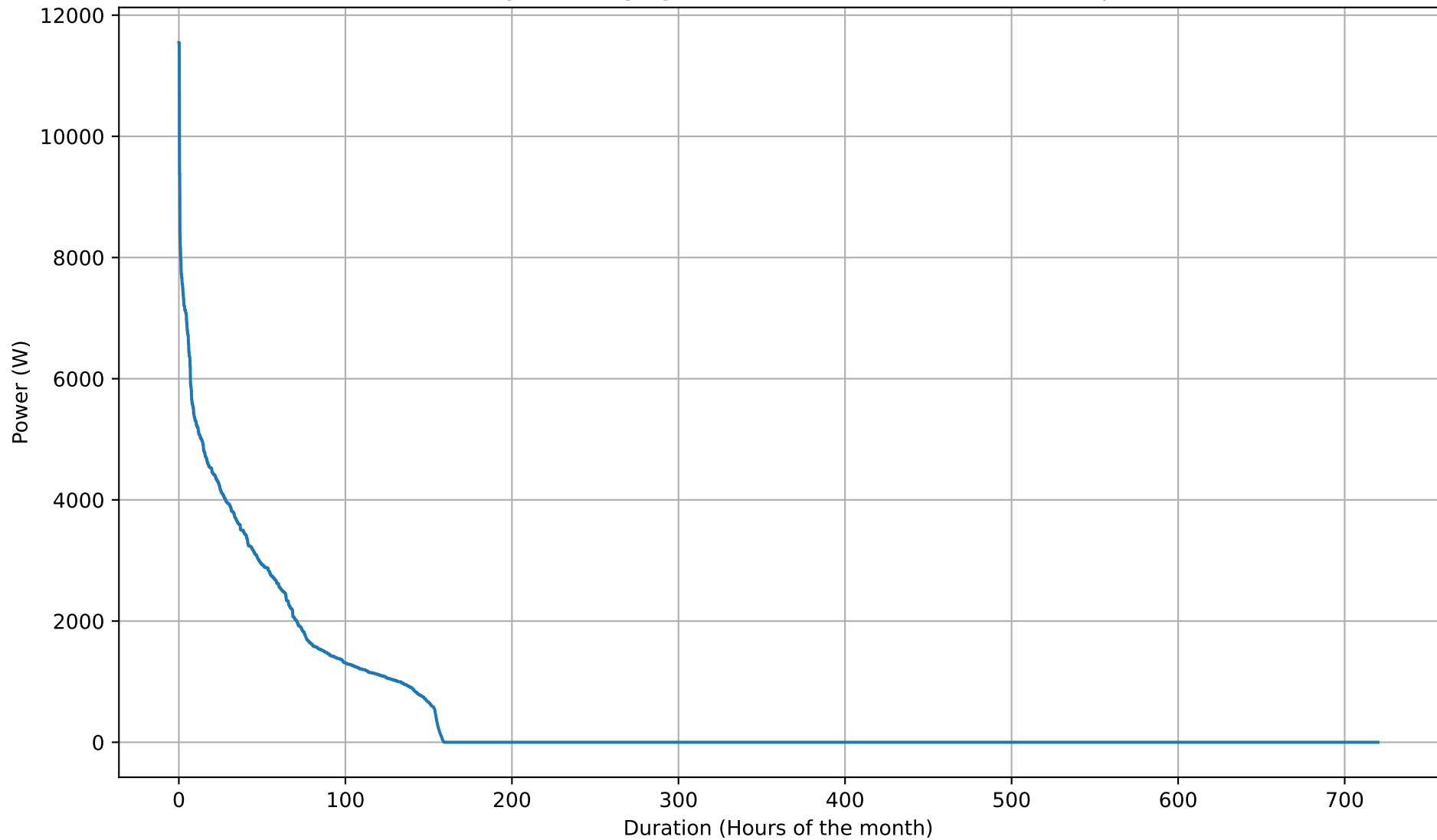
Battery Discharging Power Duration Curve - 15kWh - Apr
