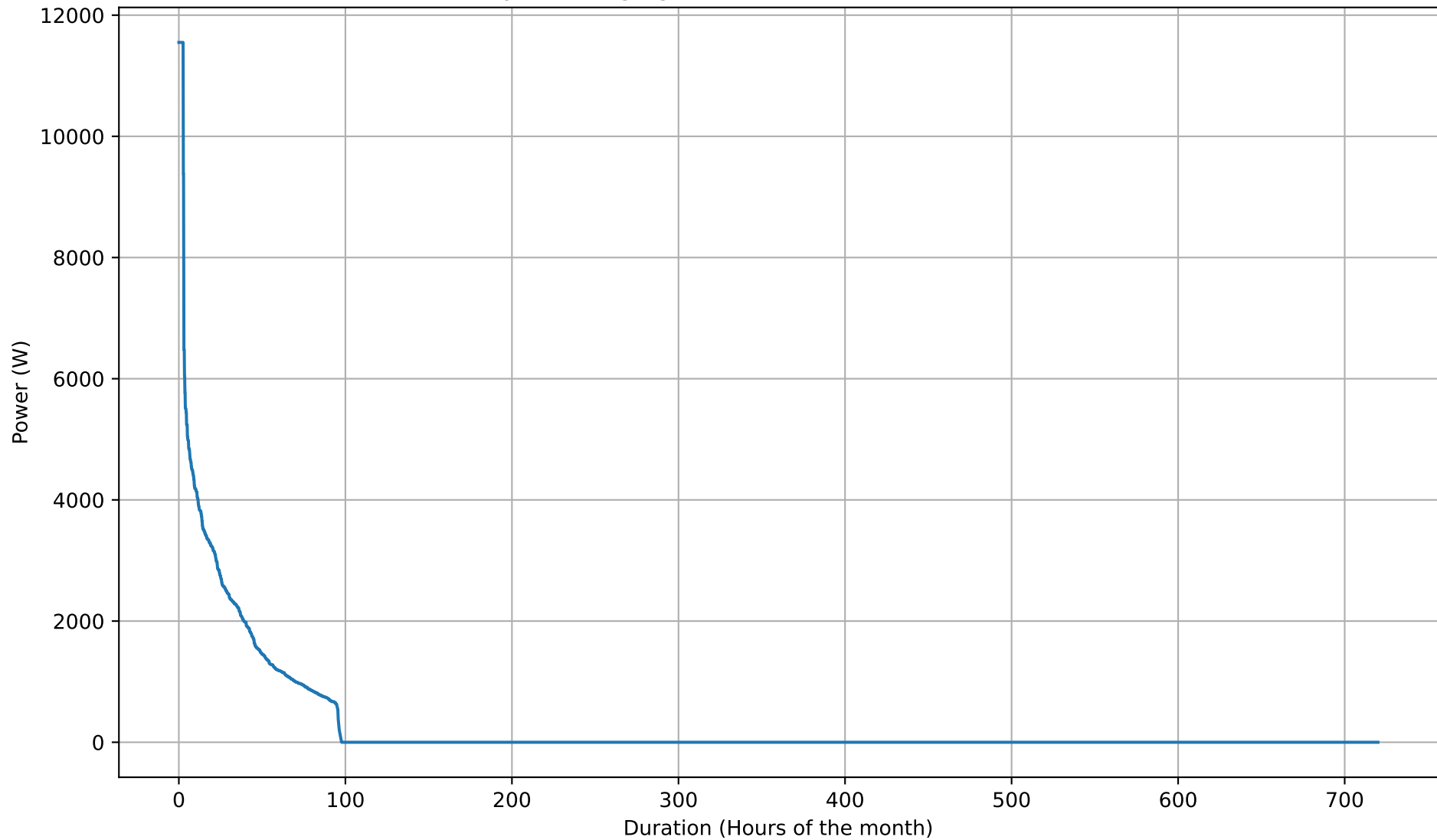
Battery Discharging Power Duration Curve - 15kWh - Nov
