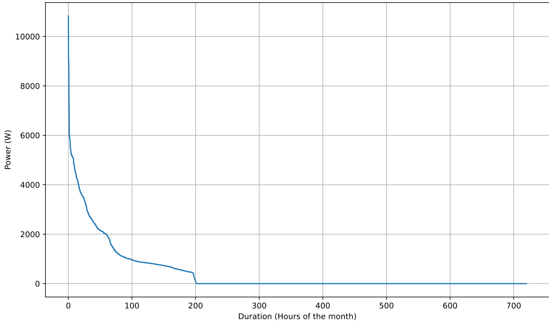
Battery Discharging Power Duration Curve - 15kWh - Jun
