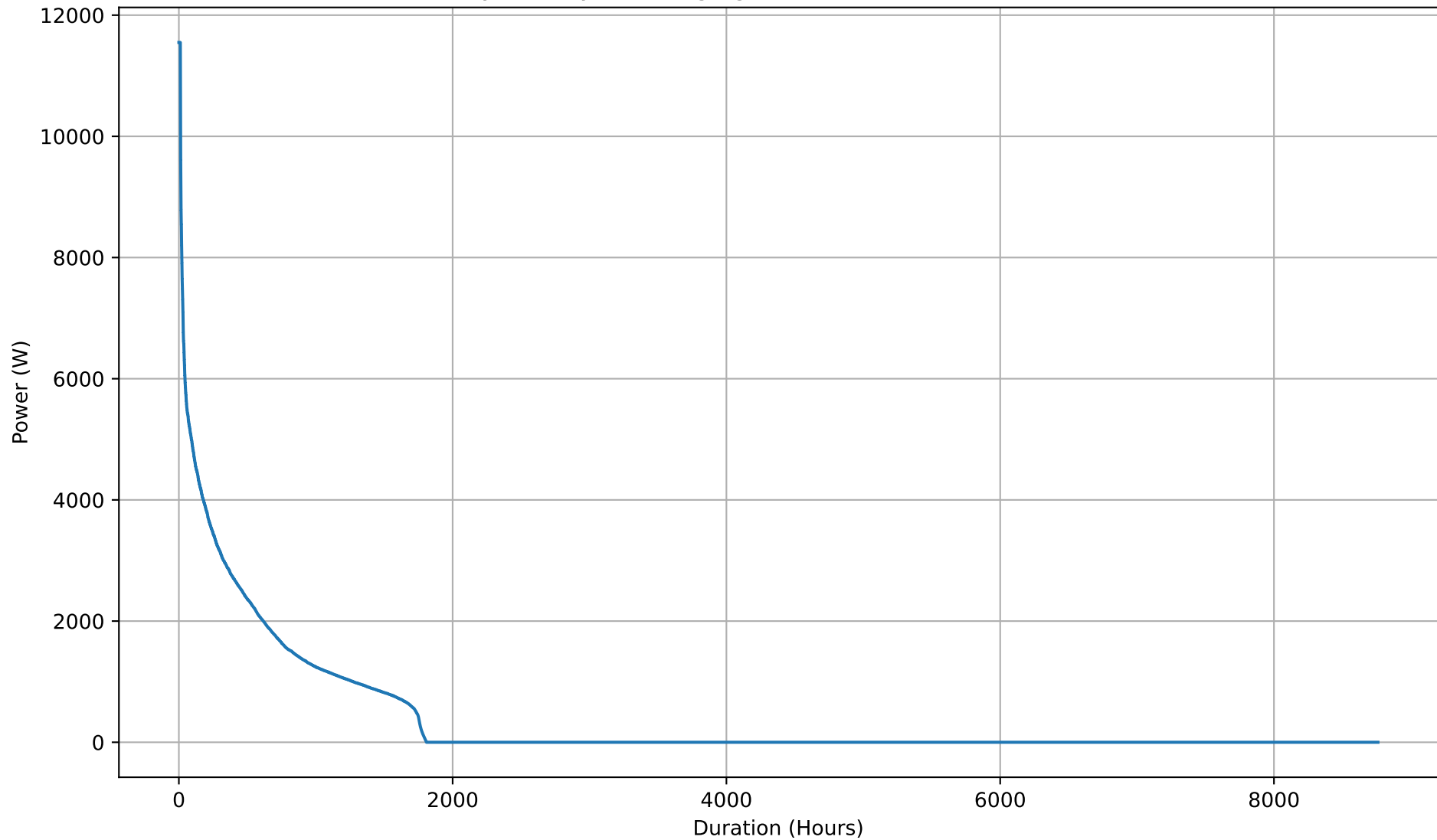
Yearly Battery Discharging Power Duration Curve - 15kWh
