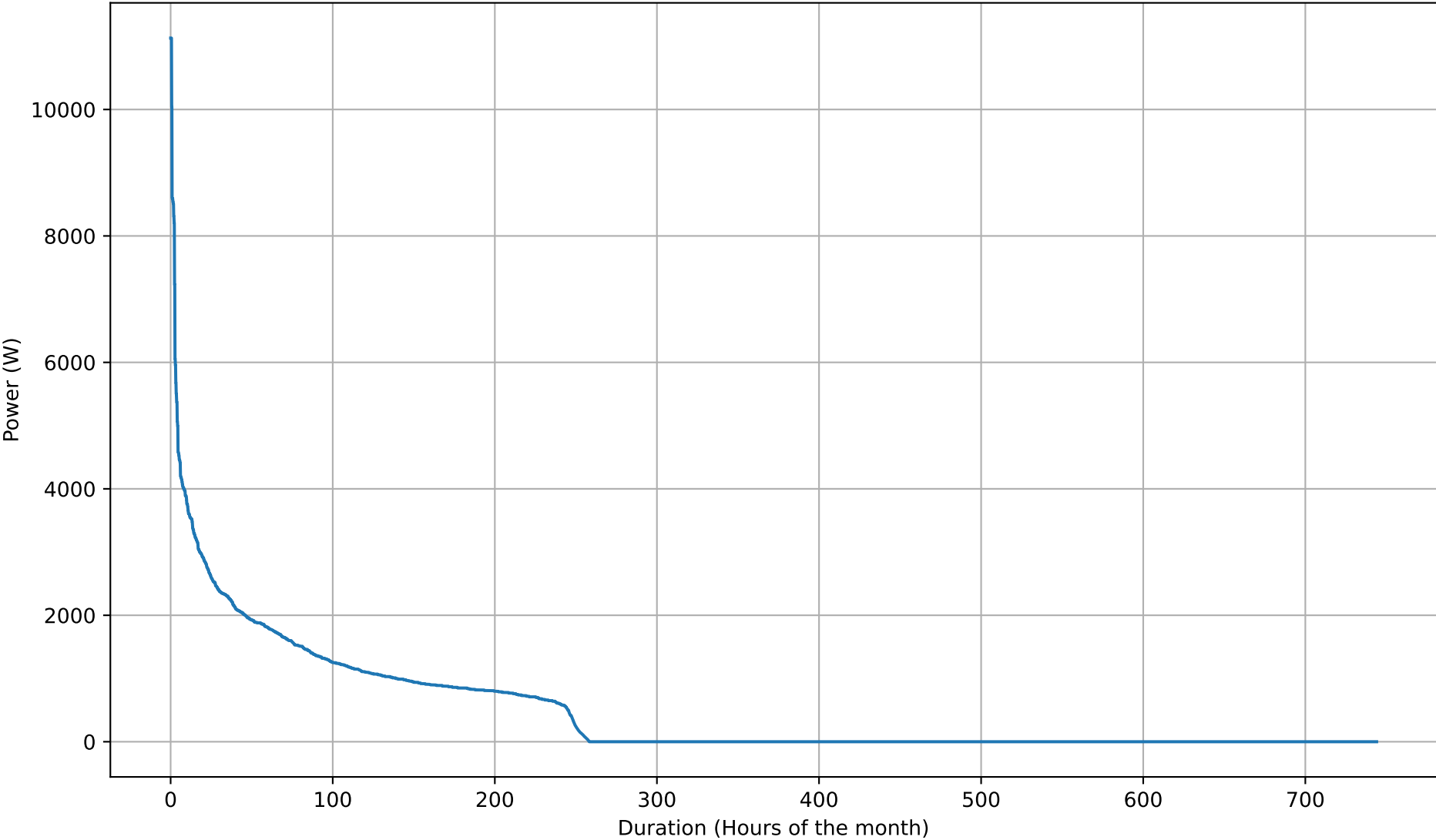
Battery Discharging Power Duration Curve - 15kWh - Jul
