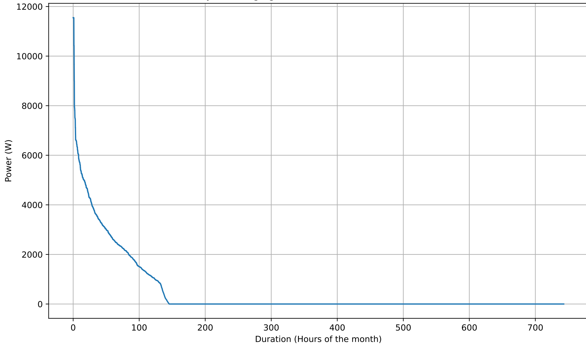
Battery Discharging Power Duration Curve - 15kWh - Mar
