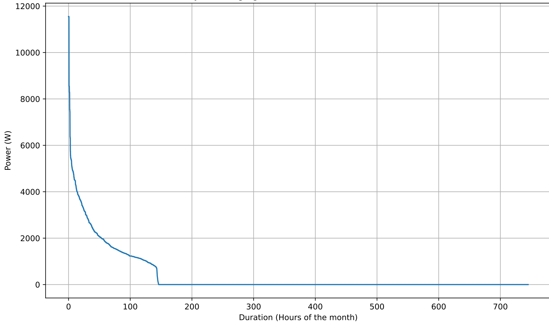
Battery Discharging Power Duration Curve - 15kWh - Oct
