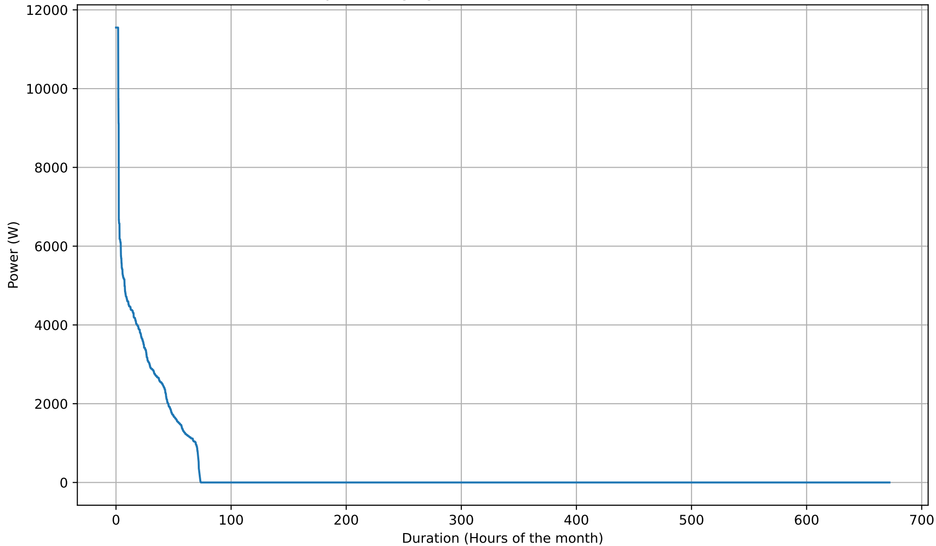
Battery Discharging Power Duration Curve - 15kWh - Feb
