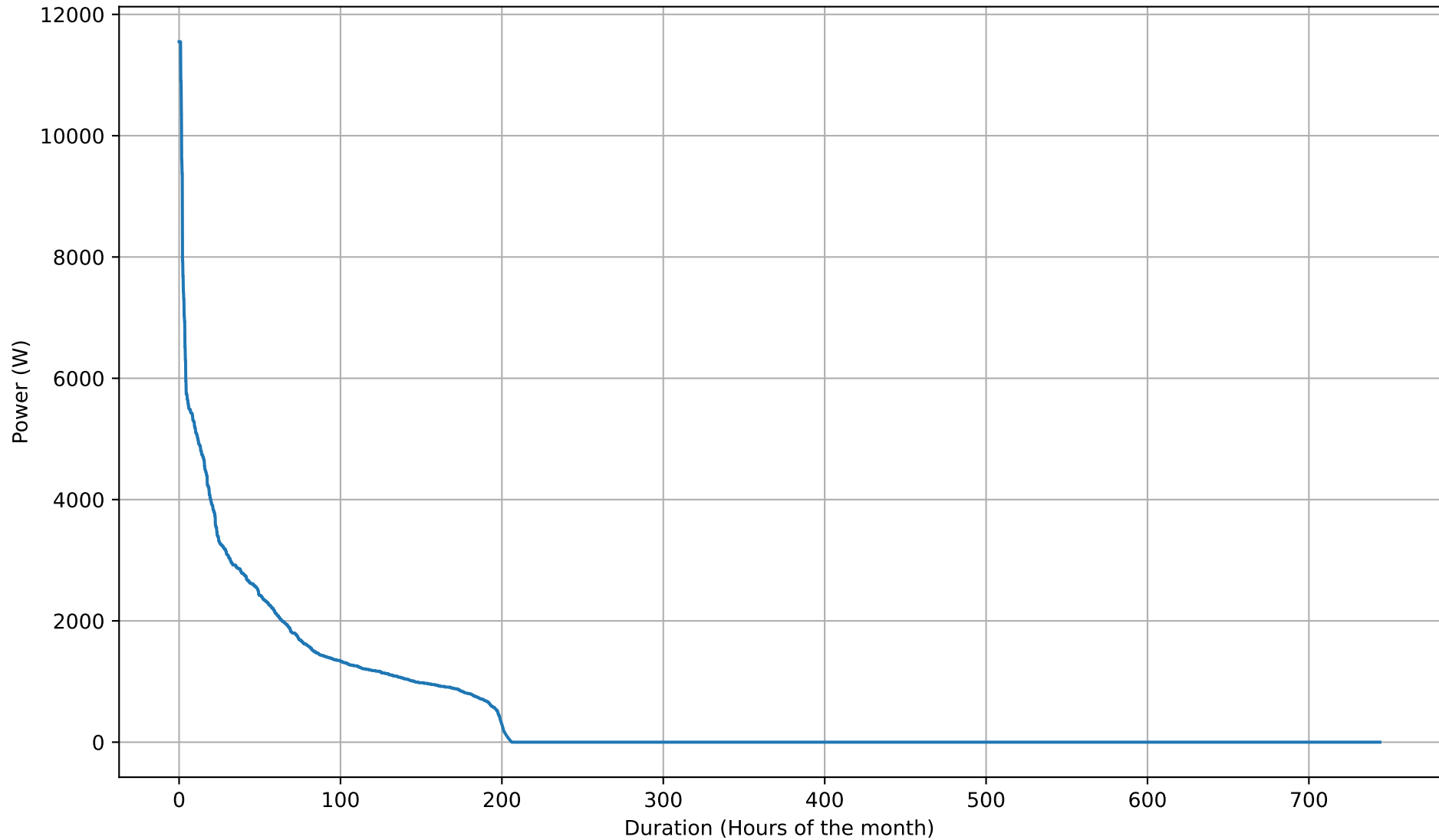
Battery Discharging Power Duration Curve - 15kWh - May
