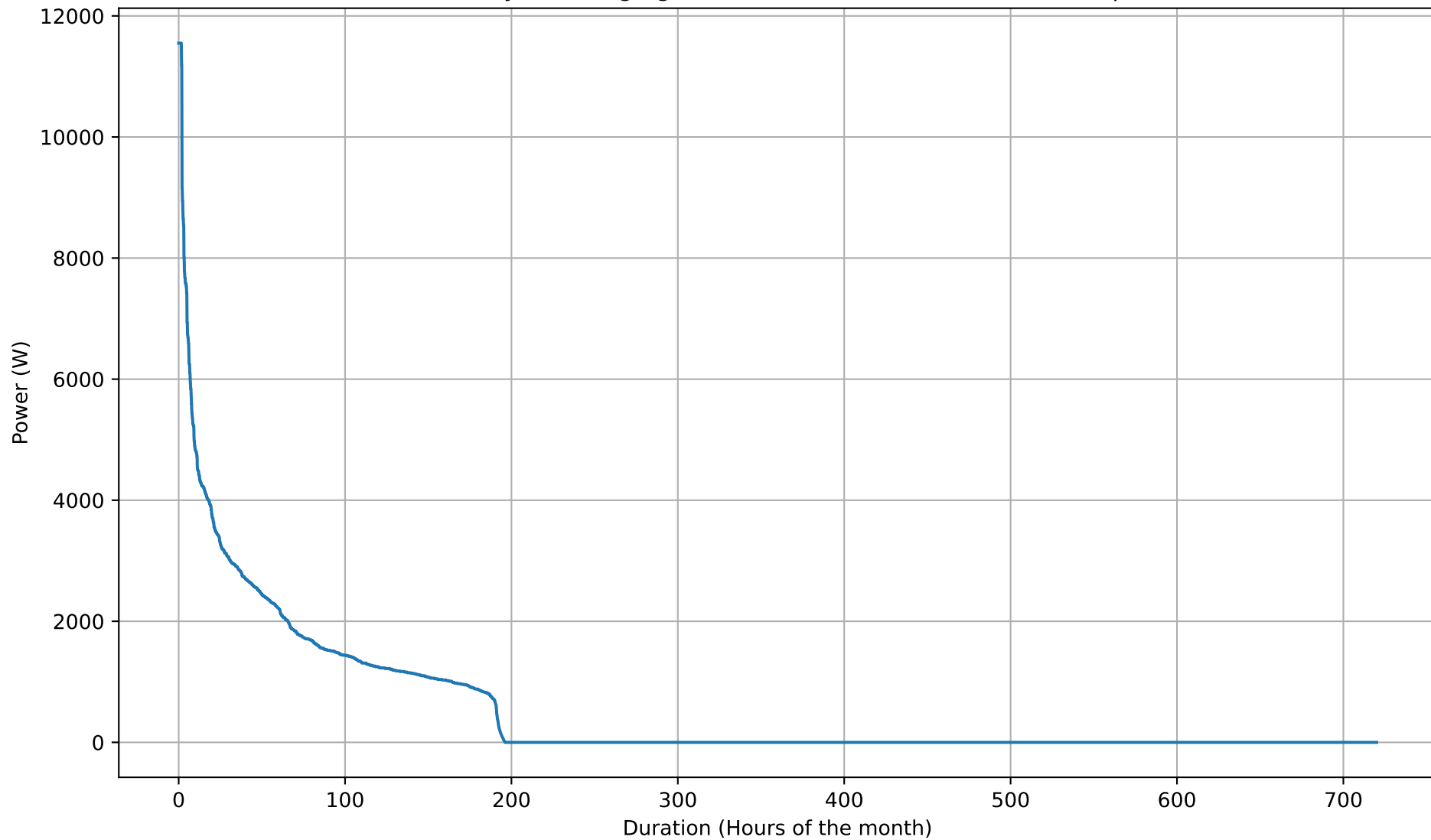
Battery Discharging Power Duration Curve - 15kWh - Sep
