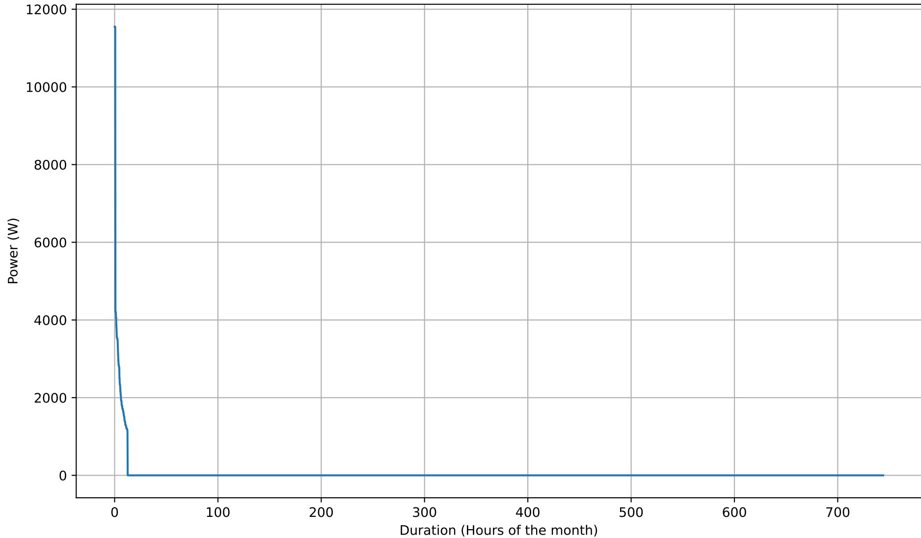
Battery Discharging Power Duration Curve - 15kWh - Dec
