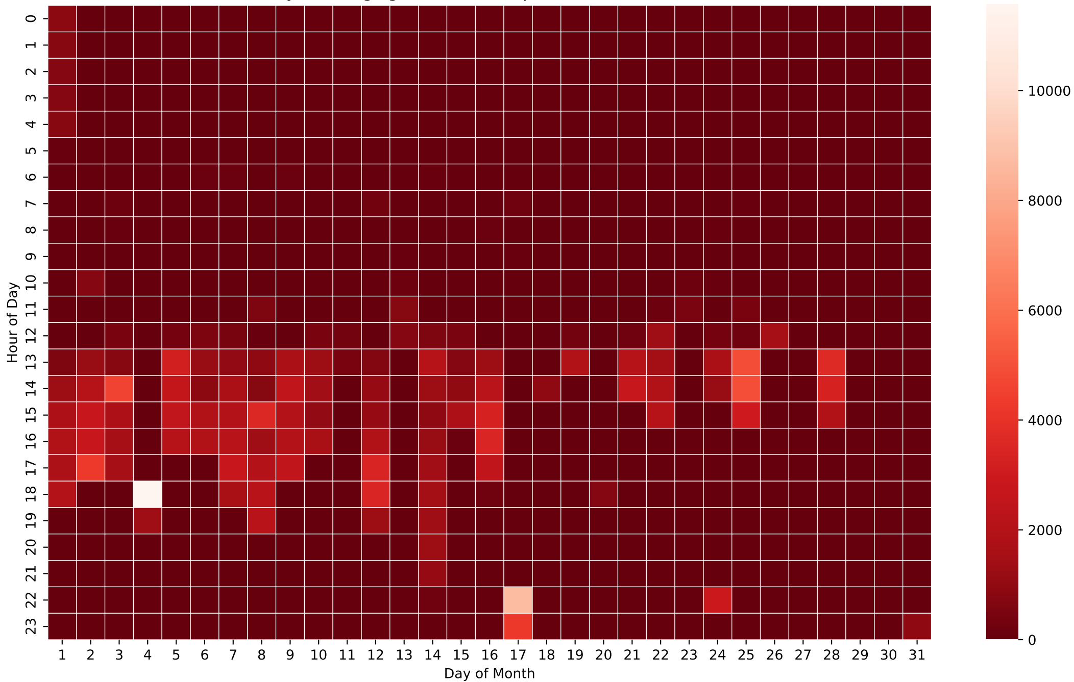
Battery Discharging Power Heatmap (Wh/Hour) - 15kWh - Nov
