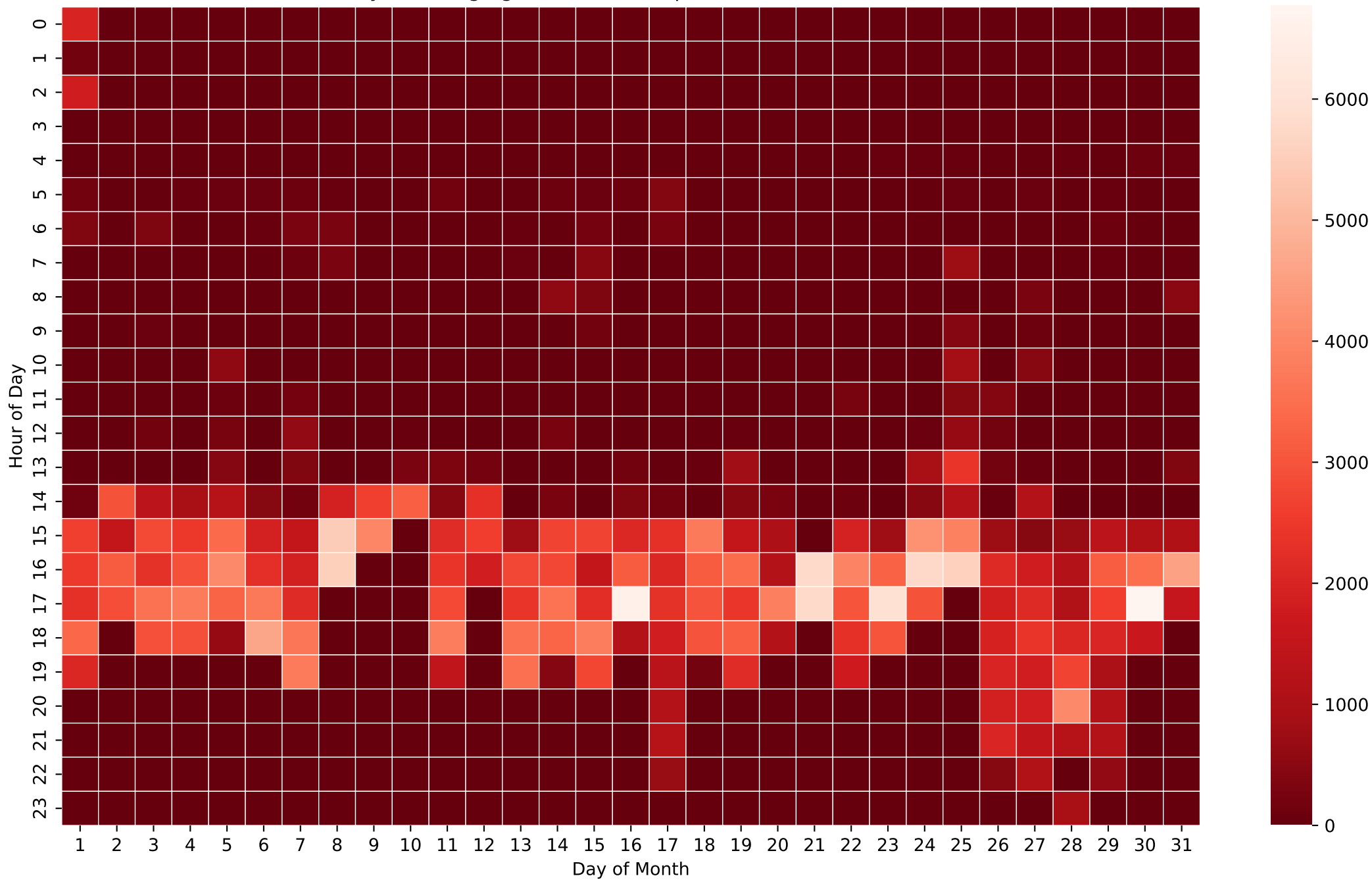
Battery Discharging Power Heatmap (Wh/Hour) - 15kWh - Mar
