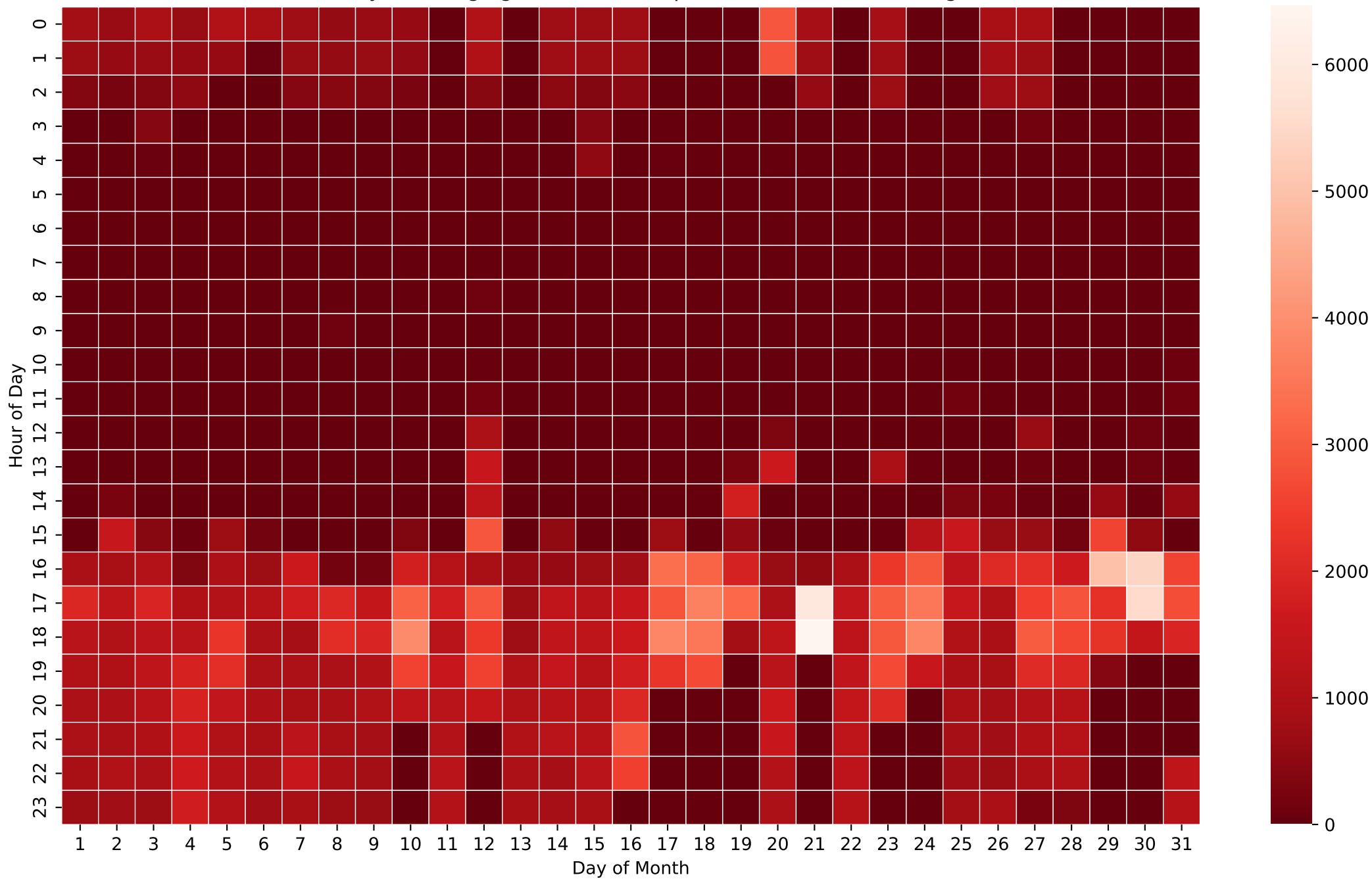
Battery Discharging Power Heatmap (Wh/Hour) - 15kWh - Aug
