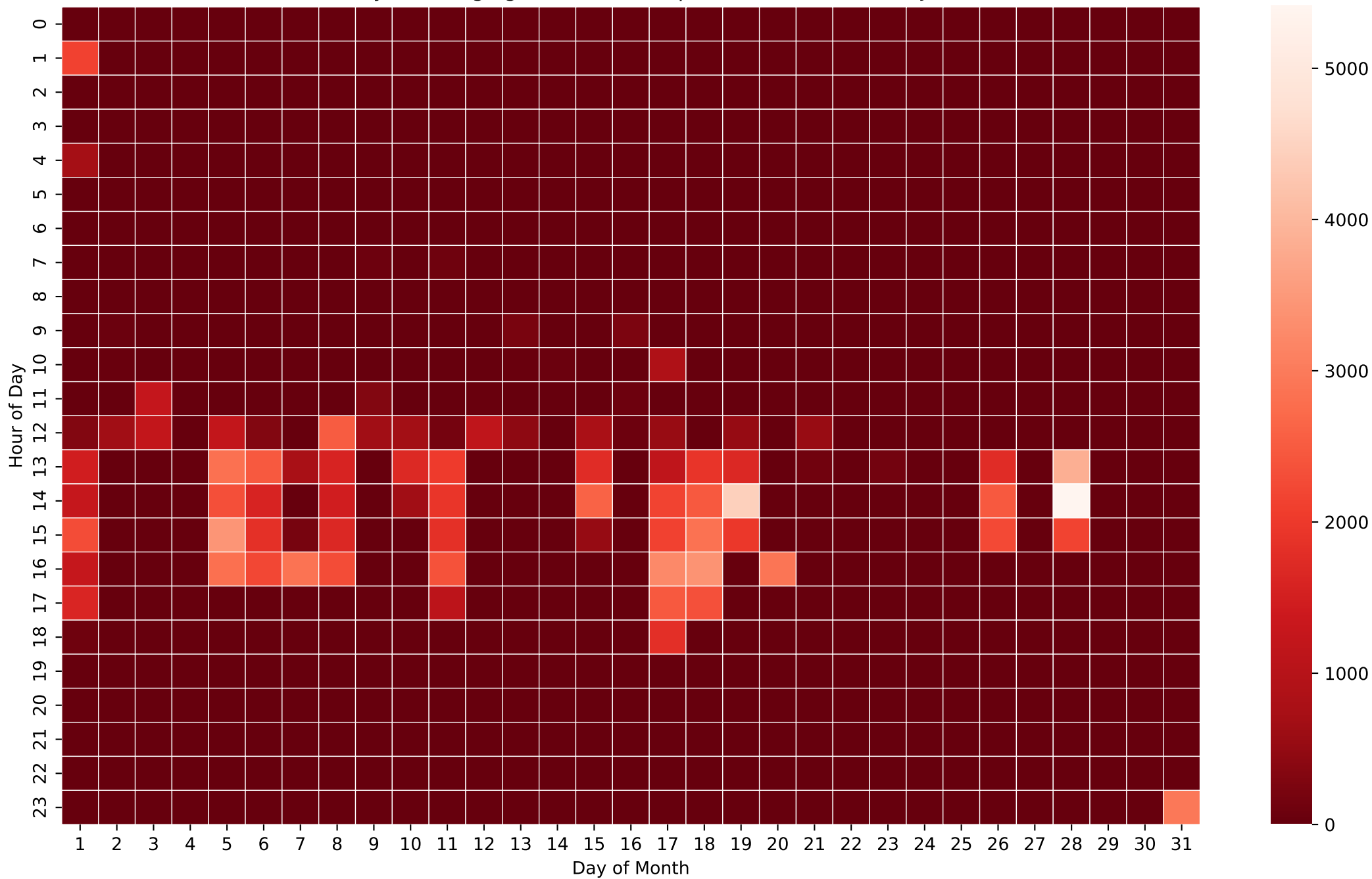
Battery Discharging Power Heatmap (Wh/Hour) - 15kWh - Jan
