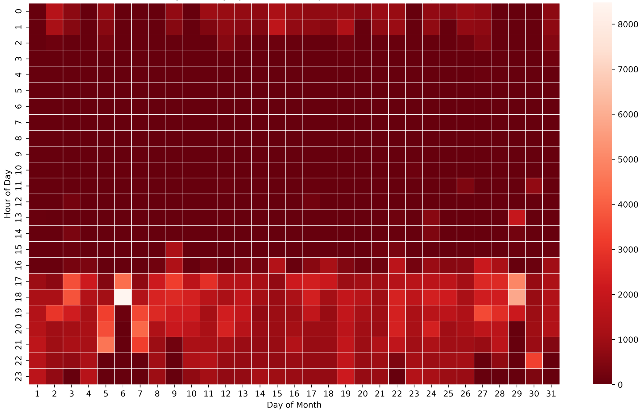
Battery Discharging Power Heatmap (Wh/Hour) - 15kWh - Jul
