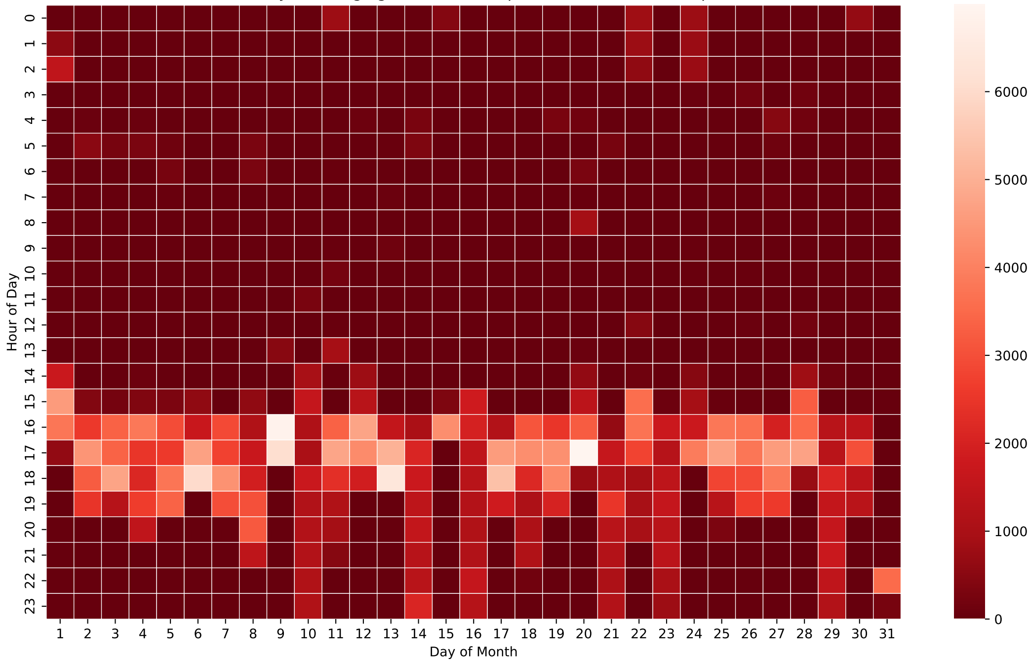
Battery Discharging Power Heatmap (Wh/Hour) - 15kWh - Apr
