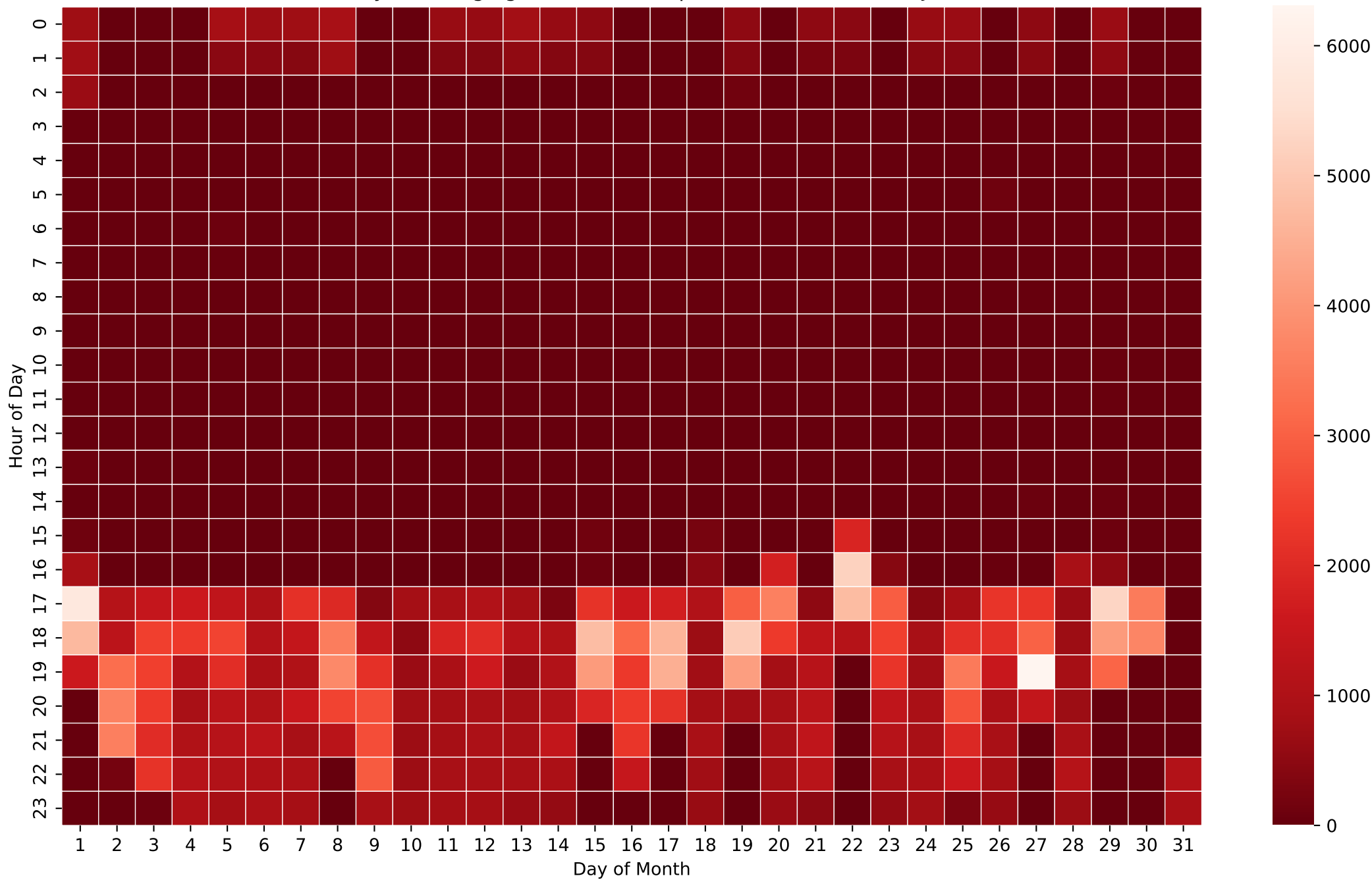
Battery Discharging Power Heatmap (Wh/Hour) - 15kWh - Jun
