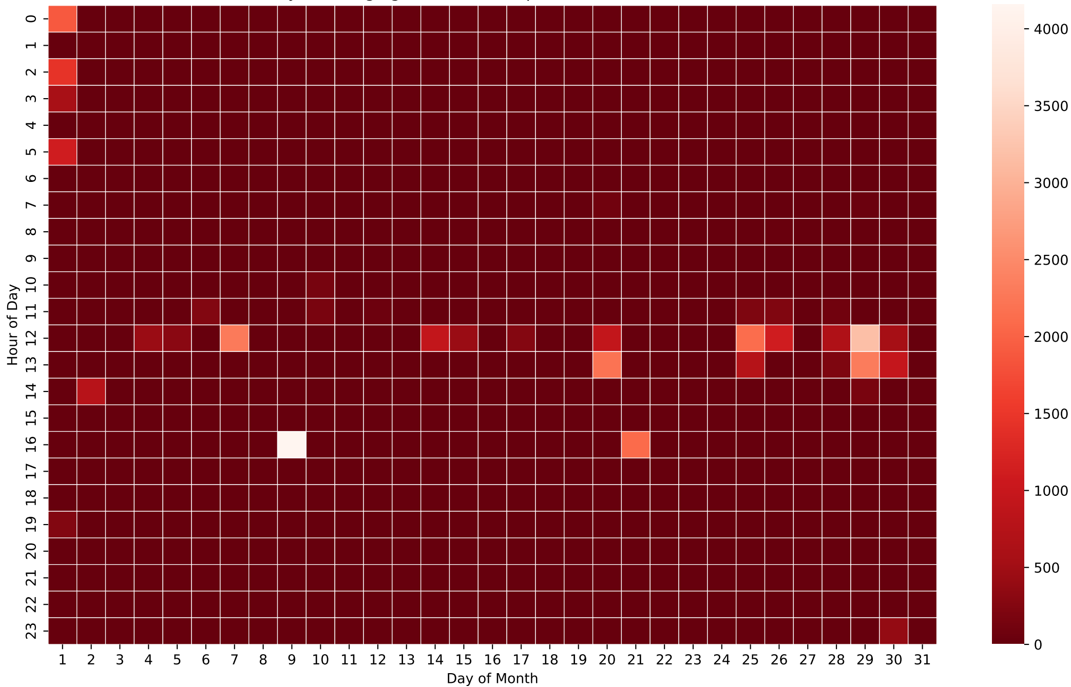
Battery Discharging Power Heatmap (Wh/Hour) - 15kWh - Dec
