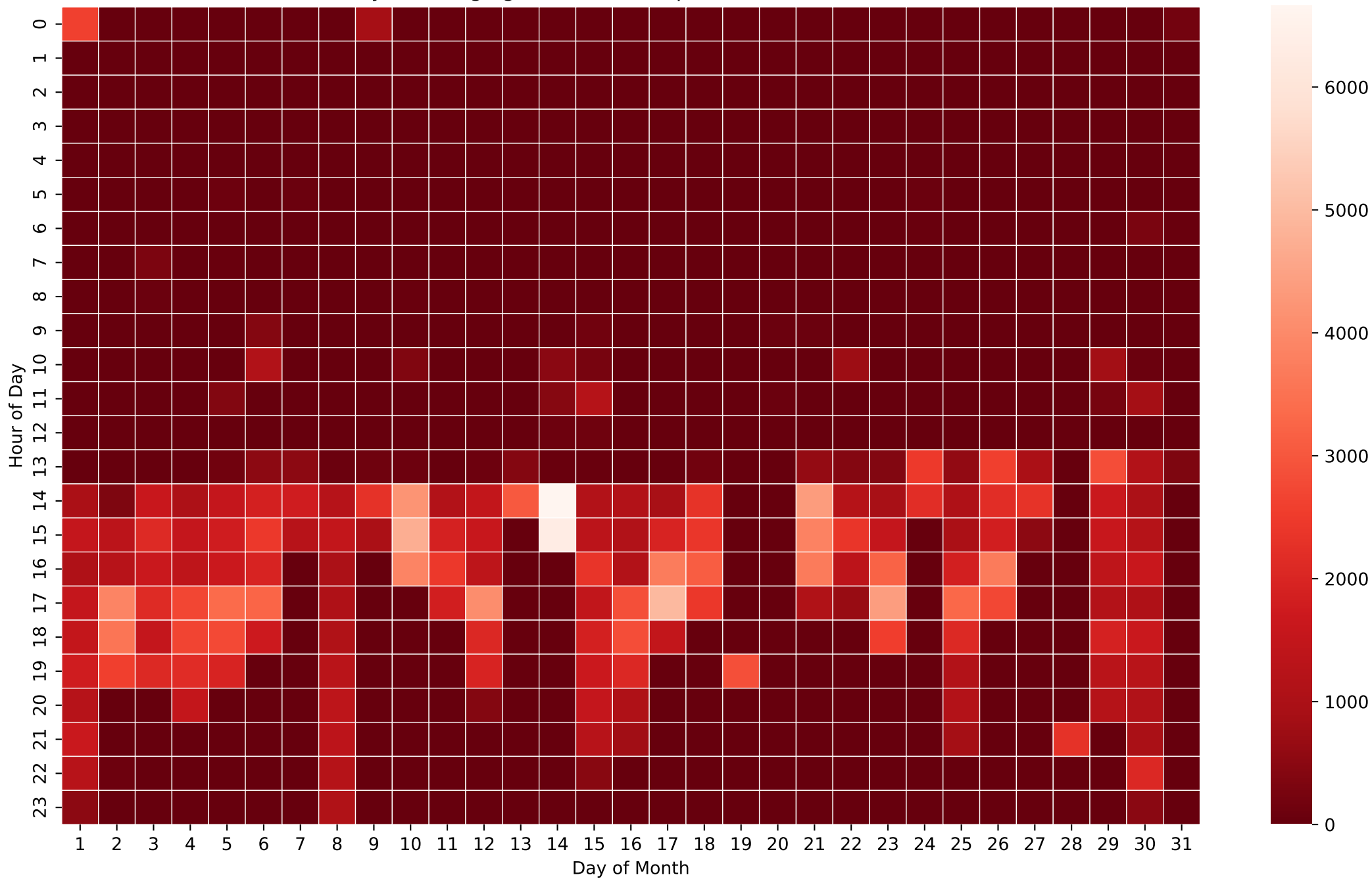
Battery Discharging Power Heatmap (Wh/Hour) - 15kWh - Oct
