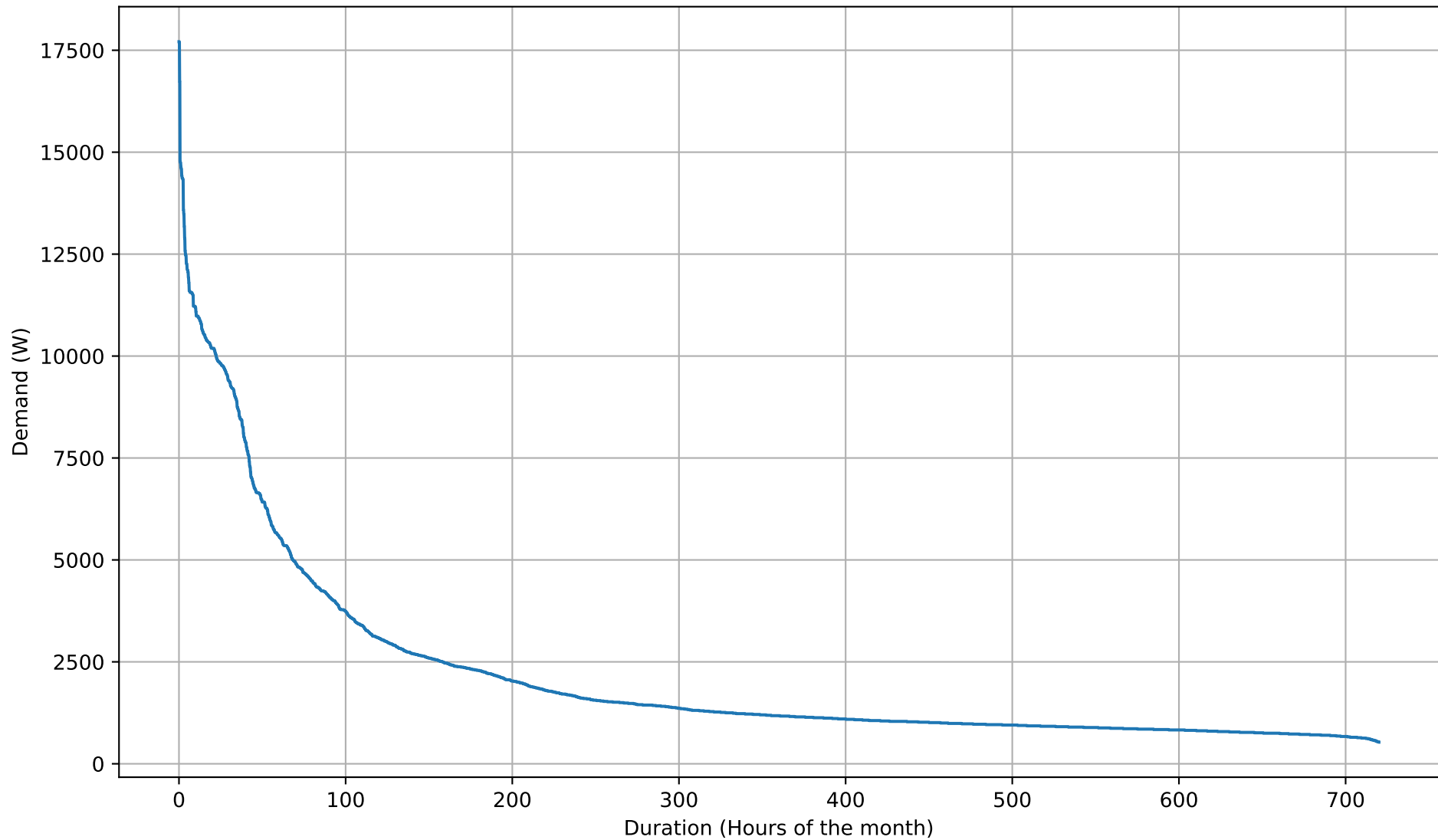
Electricity Demand Duration Curve - 15kWh - Sep
