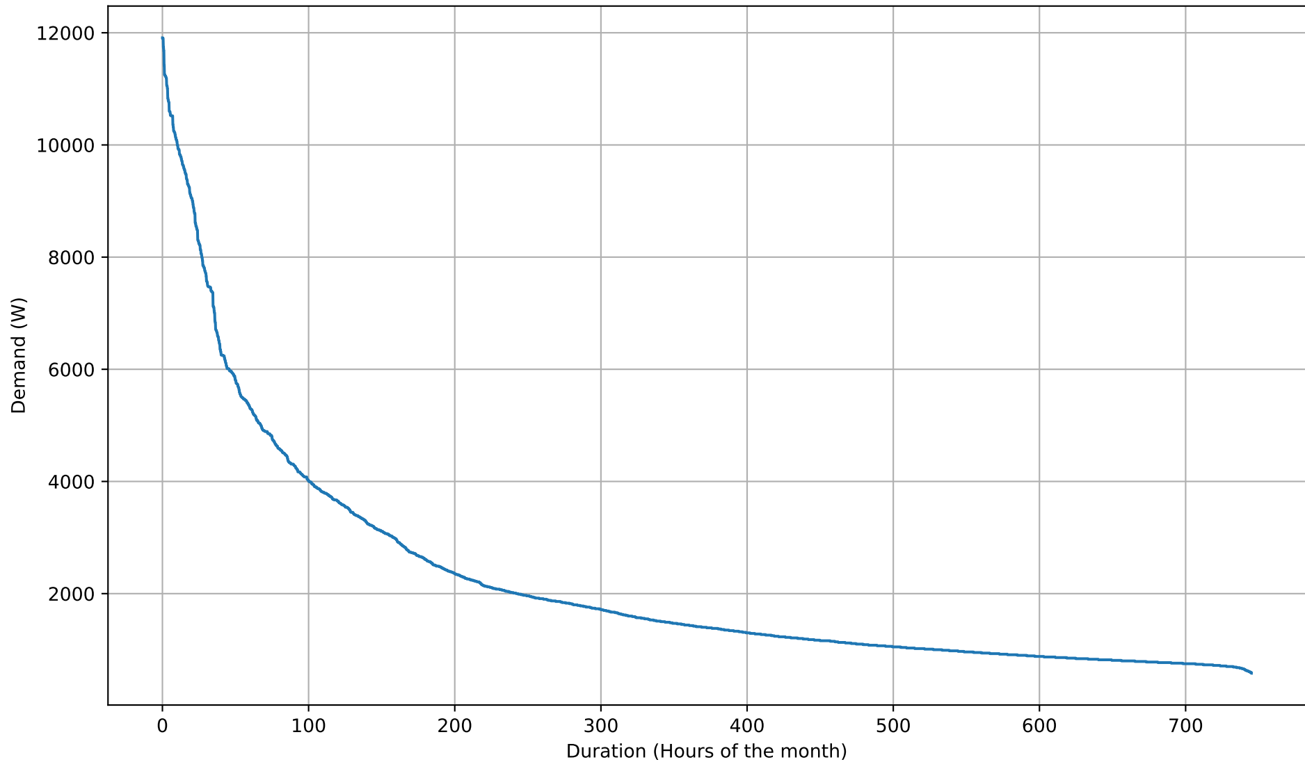
Electricity Demand Duration Curve - 15kWh - Oct
