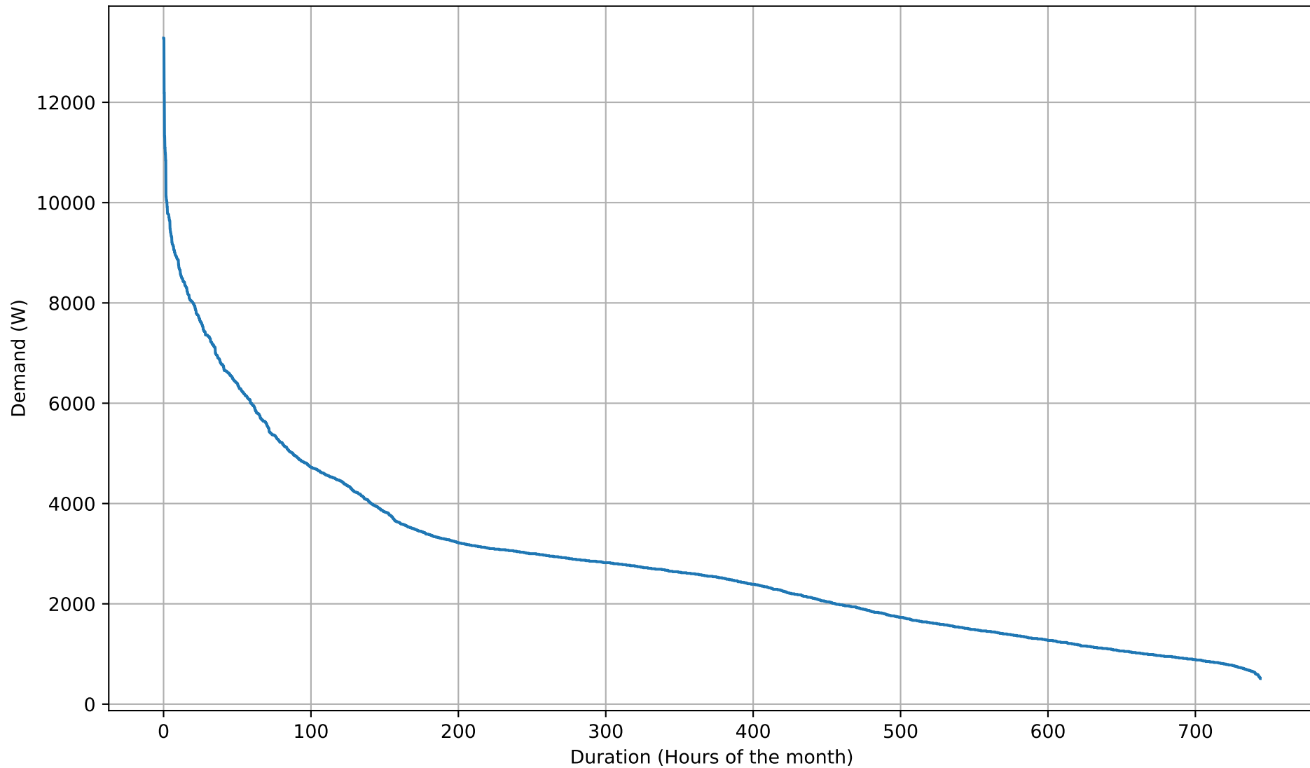
Electricity Demand Duration Curve - 15kWh - Jan
