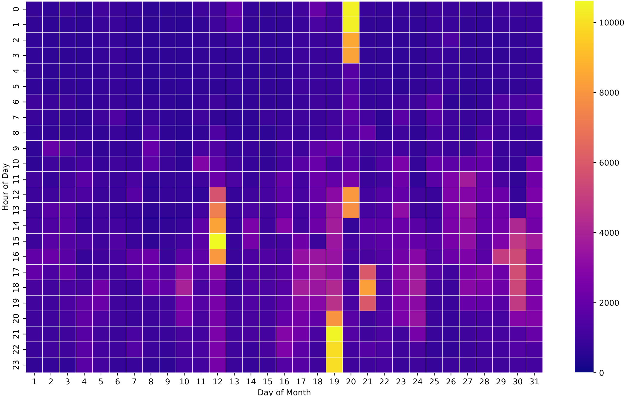
Electricity Demand Heatmap (Wh/Hour) - 15kWh - Aug
