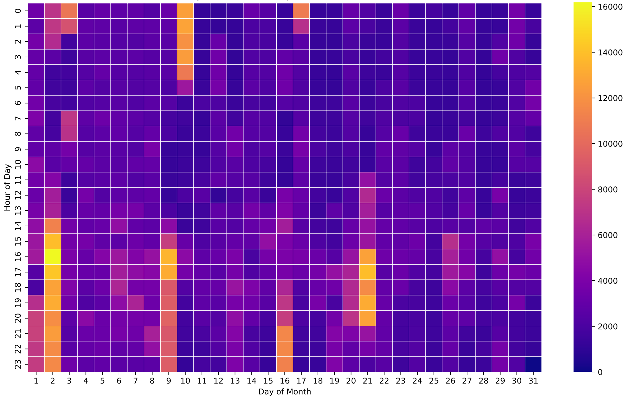
Electricity Demand Heatmap (Wh/Hour) - 15kWh - Dec
