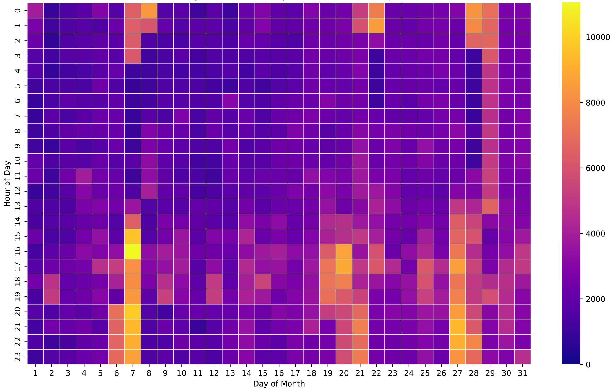
Electricity Demand Heatmap (Wh/Hour) - 15kWh - Jan
