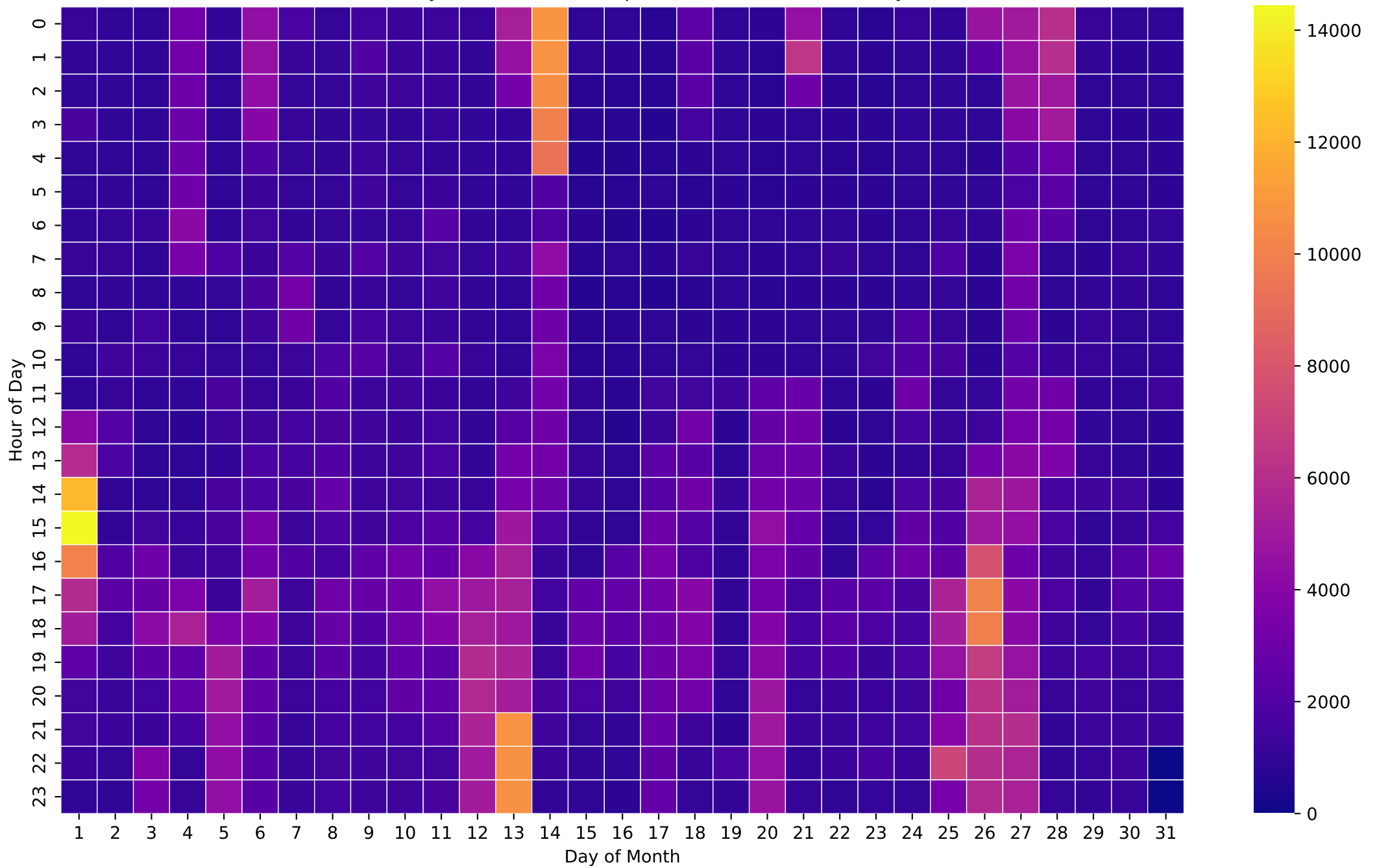
Electricity Demand Heatmap (Wh/Hour) - 15kWh - May
