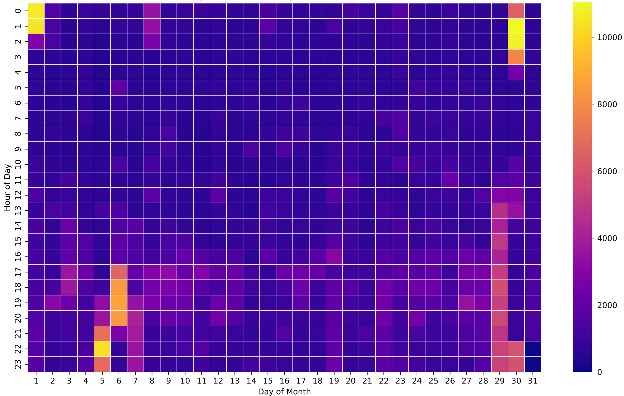
Electricity Demand Heatmap (Wh/Hour) - 15kWh - Jul
